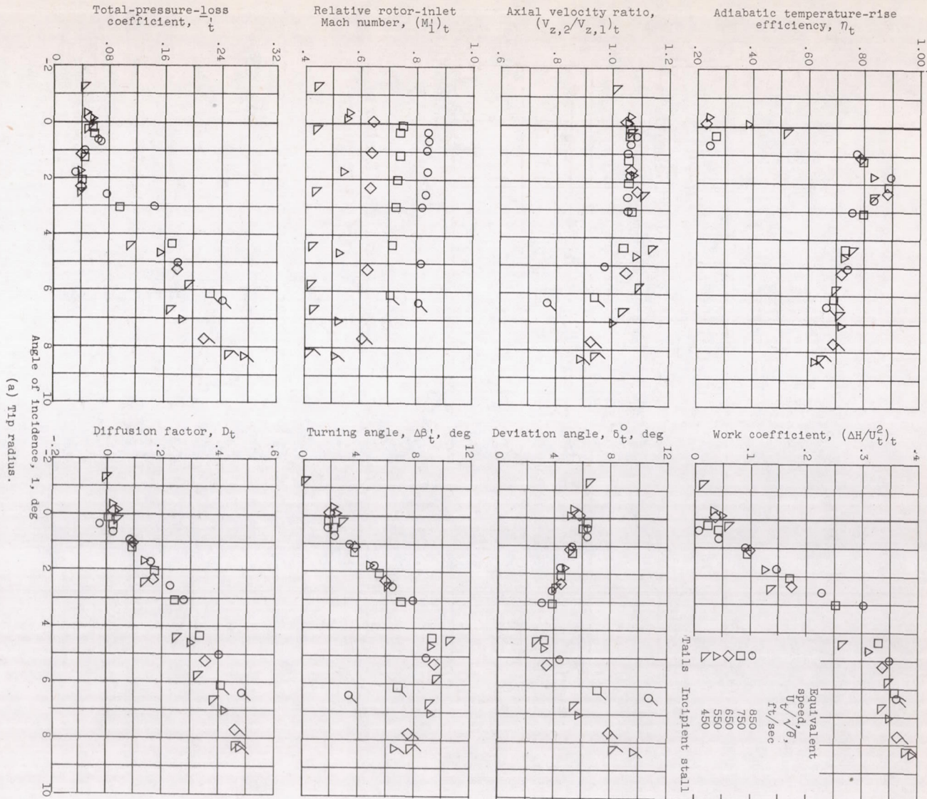
Figure 8. - Blade-element performance for short-chord rotor. Inlet pressure, 25 inches of mercury absolute.
