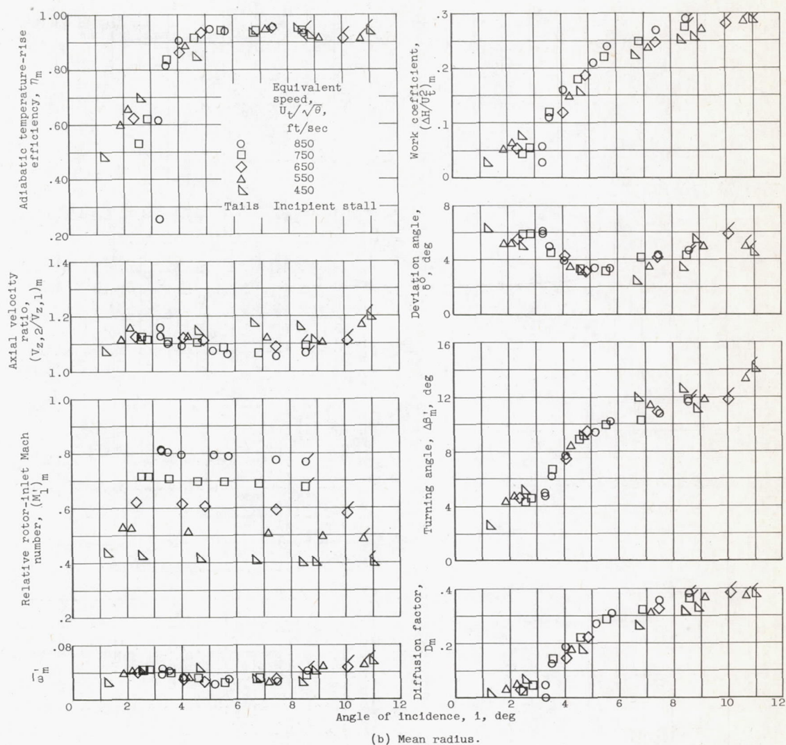
Figure 8. - Continued. Blade-element performance for short-chord rotor. Inlet pressure, 25 inches of mercury absolute.
