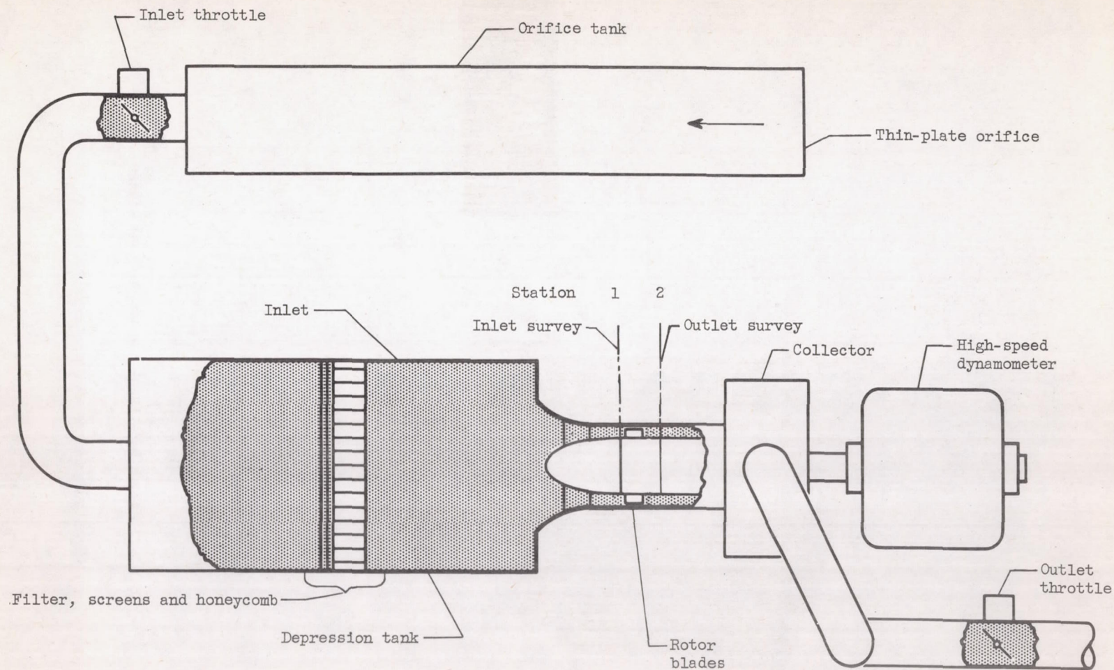
Figure 3. - Compressor installation.
