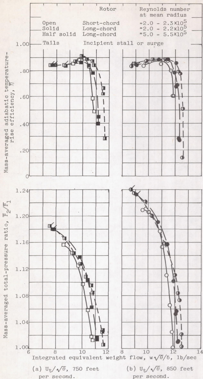
Figure 6. - Comparison of performance of short- and long-chord rotors during unstalled operation. Long-chord rotor at two Reynolds number ranges.
