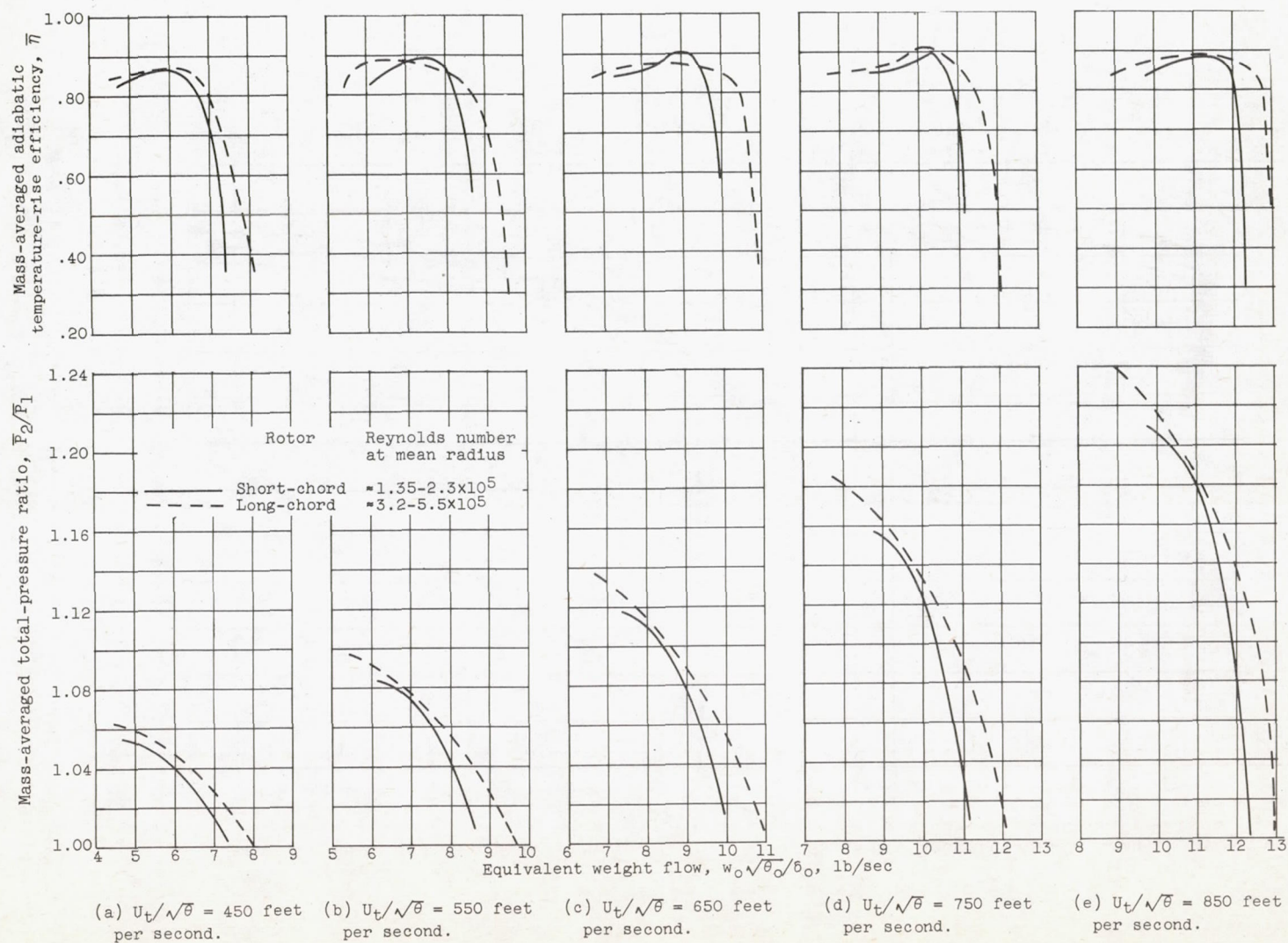
Figure 5. - Comparison of over-all performances of short- and long-chord rotors during unstalled operation. Inlet pressure, 25 inches of mercury absolute.
