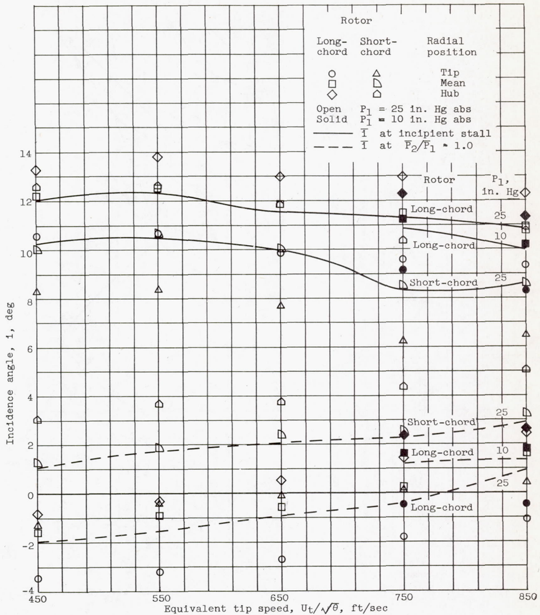
Figure 11. - Incidence angle at end points of unstalled performance data for long- and short-chord rotors at speeds tested.
