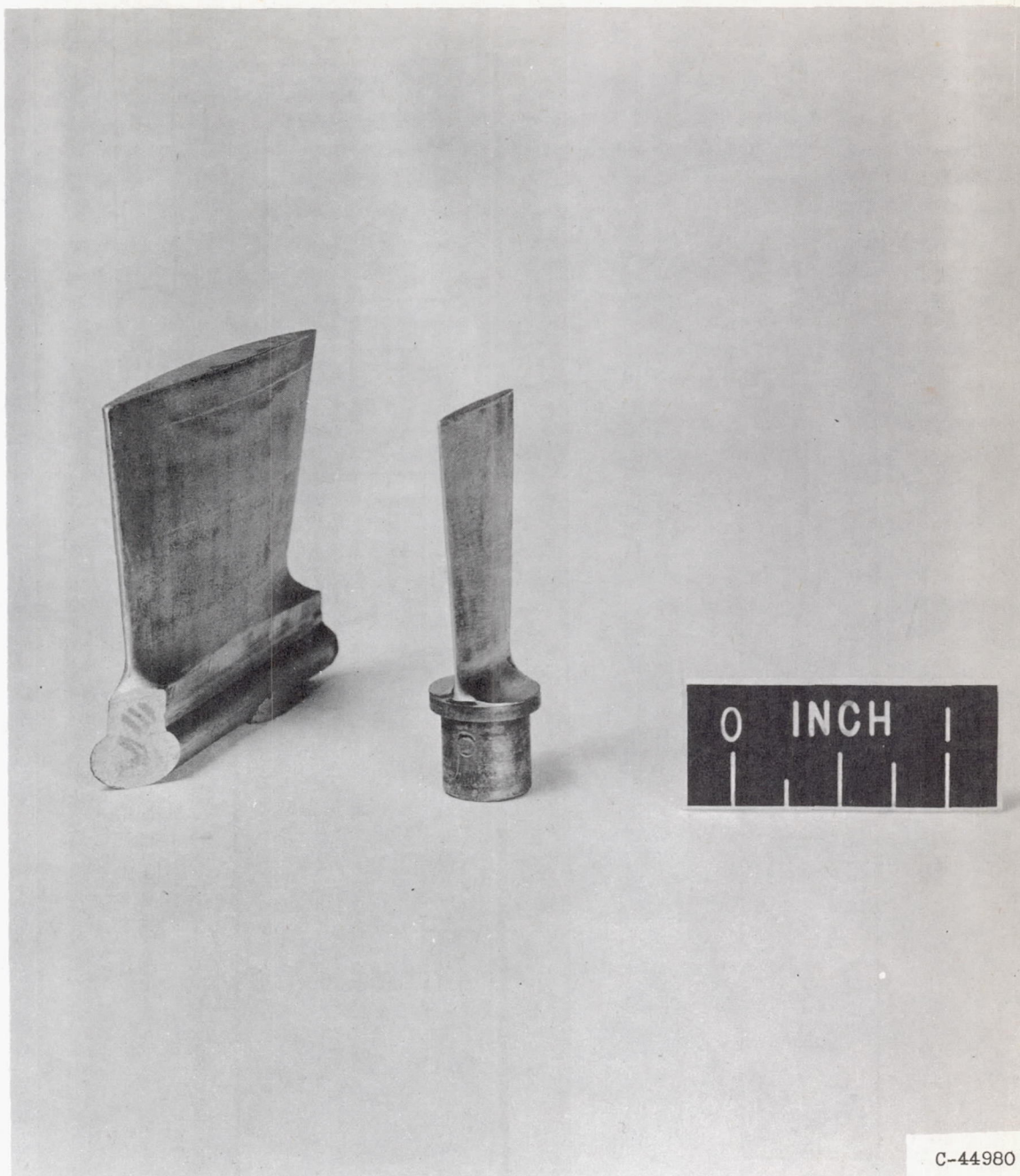
Figure 2. - Long- and short-chord blades.
