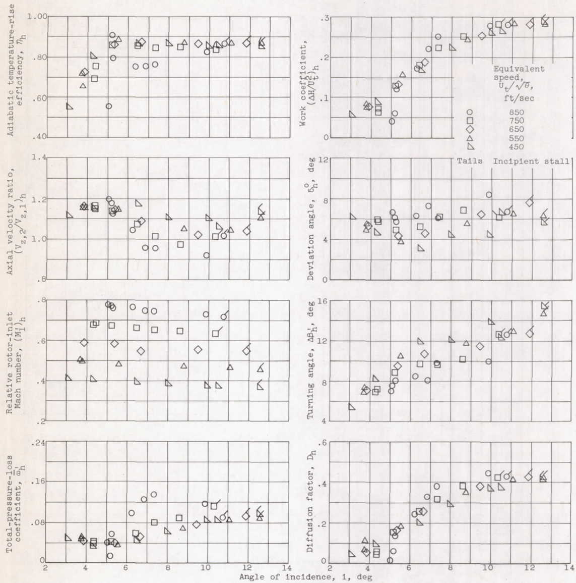
Figure 8. - Concluded. Blade-element performance for short-chord rotor. Inlet pressure, 25 inches of mercury absolute.
