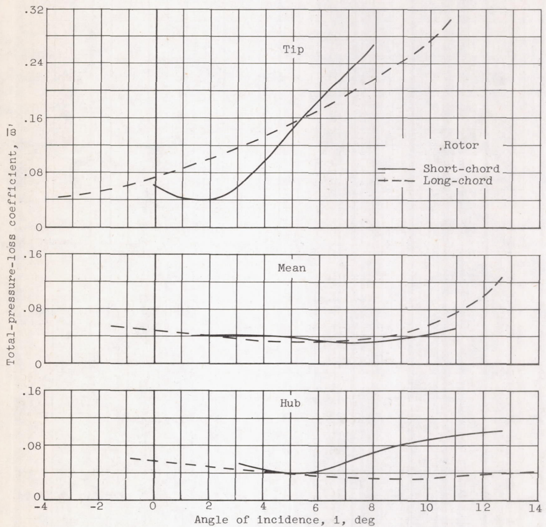
Figure 10. - Comparison of total-pressure-loss coefficients for long- and short-chord rotors.
