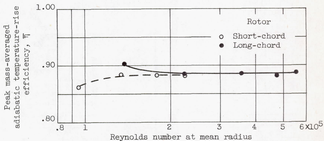
Figure 7. - Design-speed peak efficiencies of short- and long-chord rotors for various inlet pressures.
