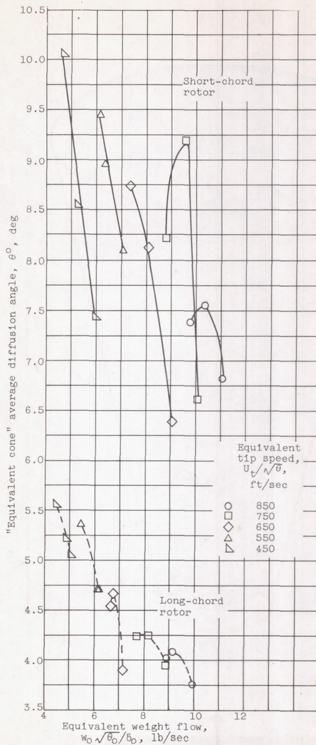
Figure 14. - Variation of equivalent cone angle with equivalent weight flow.
