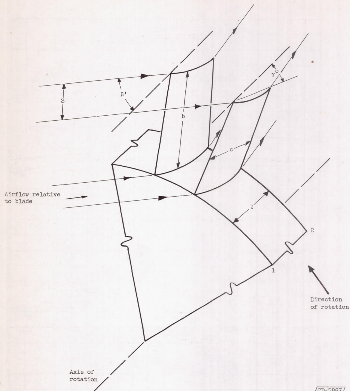
Figure 12. - Typical compressor blade passage.
