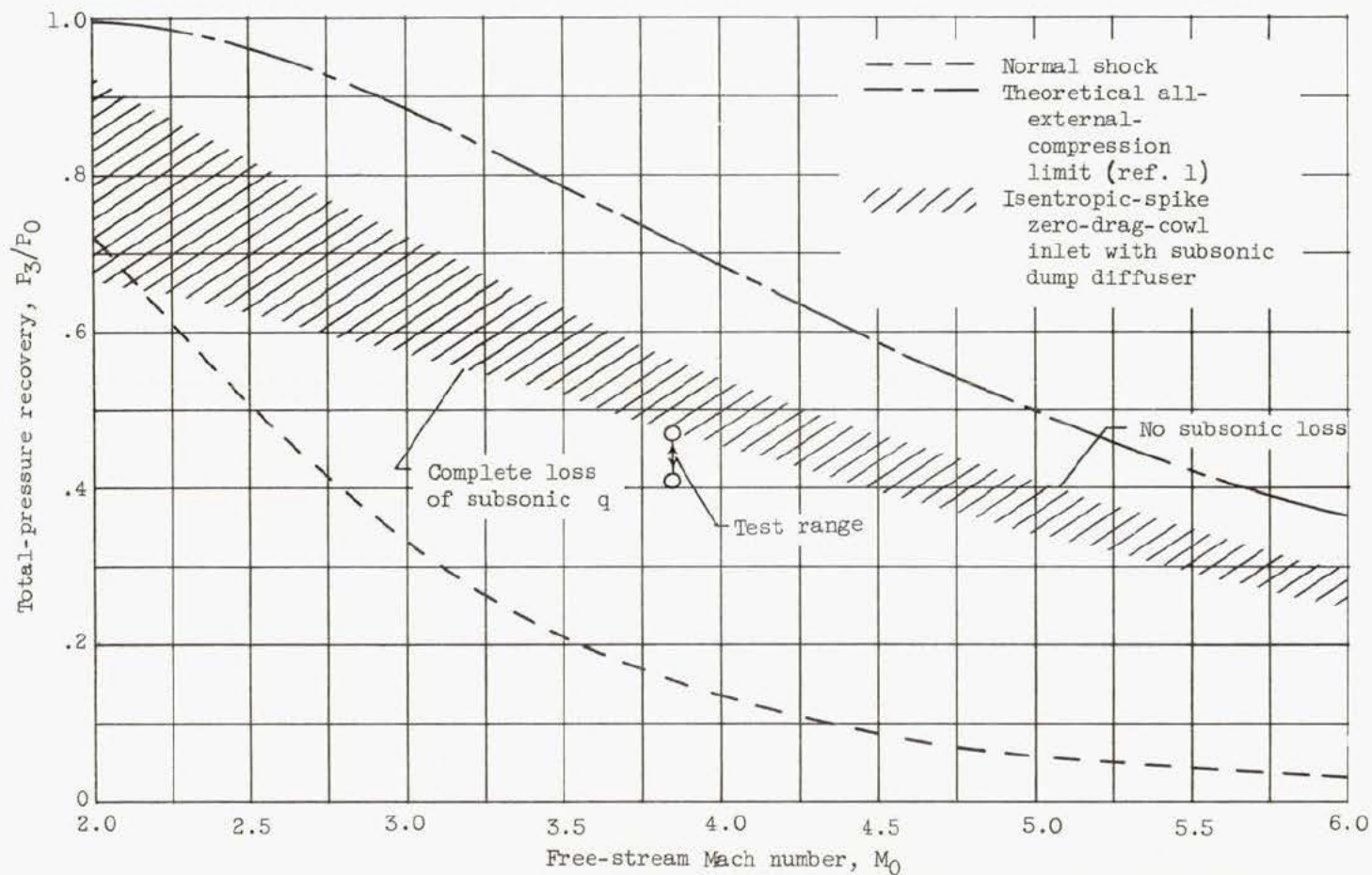
Figure 7. - Variation with Mach number of the performance of an isentropic-spike zero-drag-cowl with subsonic dump diffuser.
