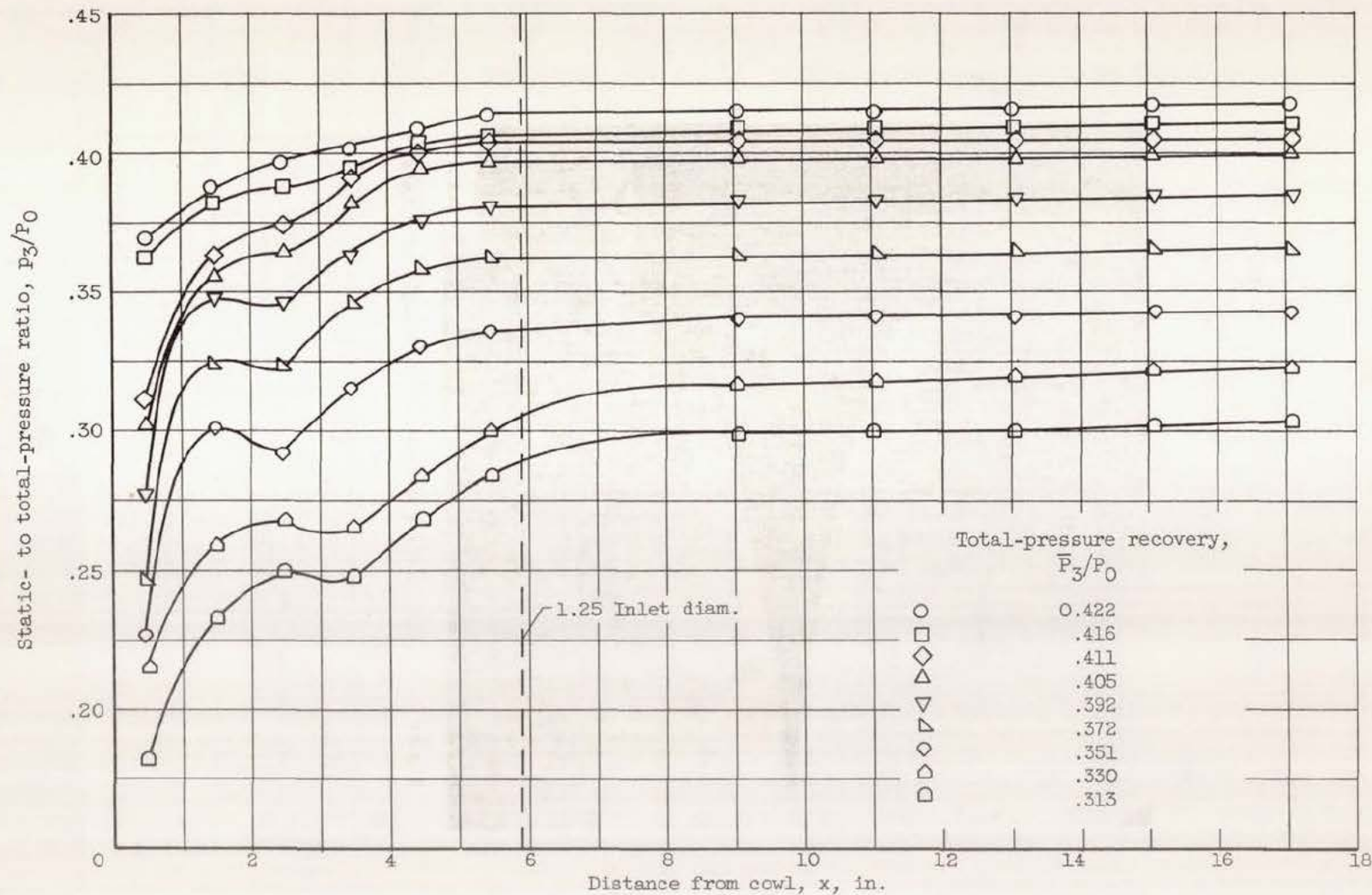
Figure 4. - Static-pressure distributions along the duct. Zero angle of attack; cowl-position parameter, 17^\circ 2.5' .
