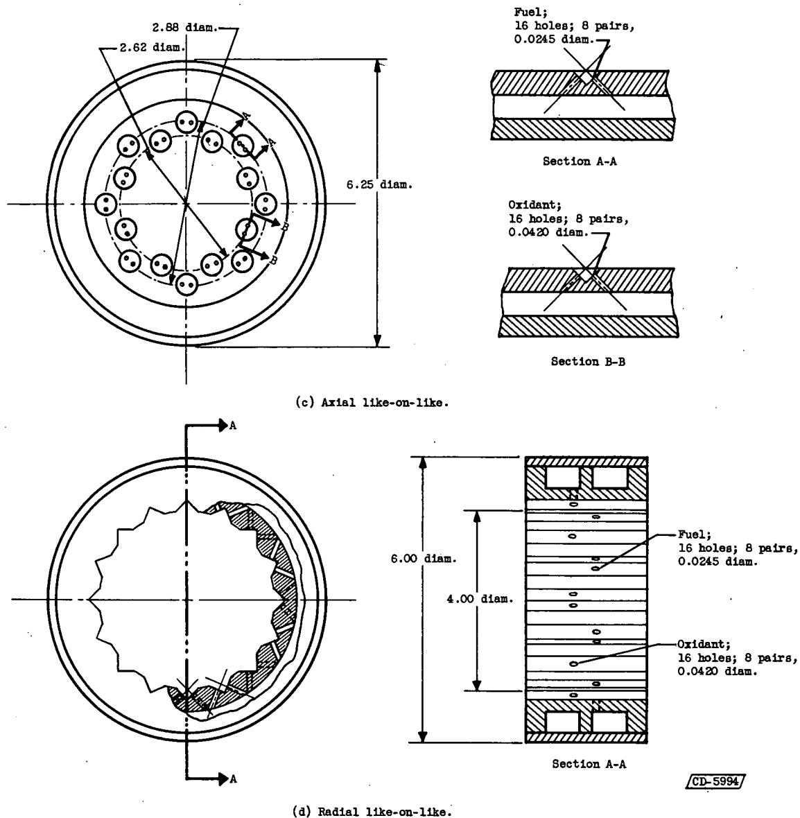
Figure 2. - Continued. Injectors. (All dimensions in inches.)
