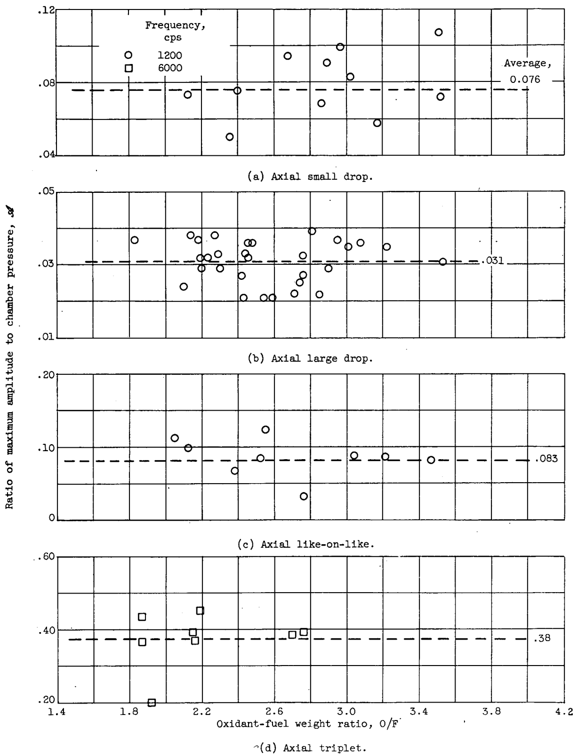
Figure 7. - Variation of screaming amplitude with oxidant-fuel ratio for each injector.
