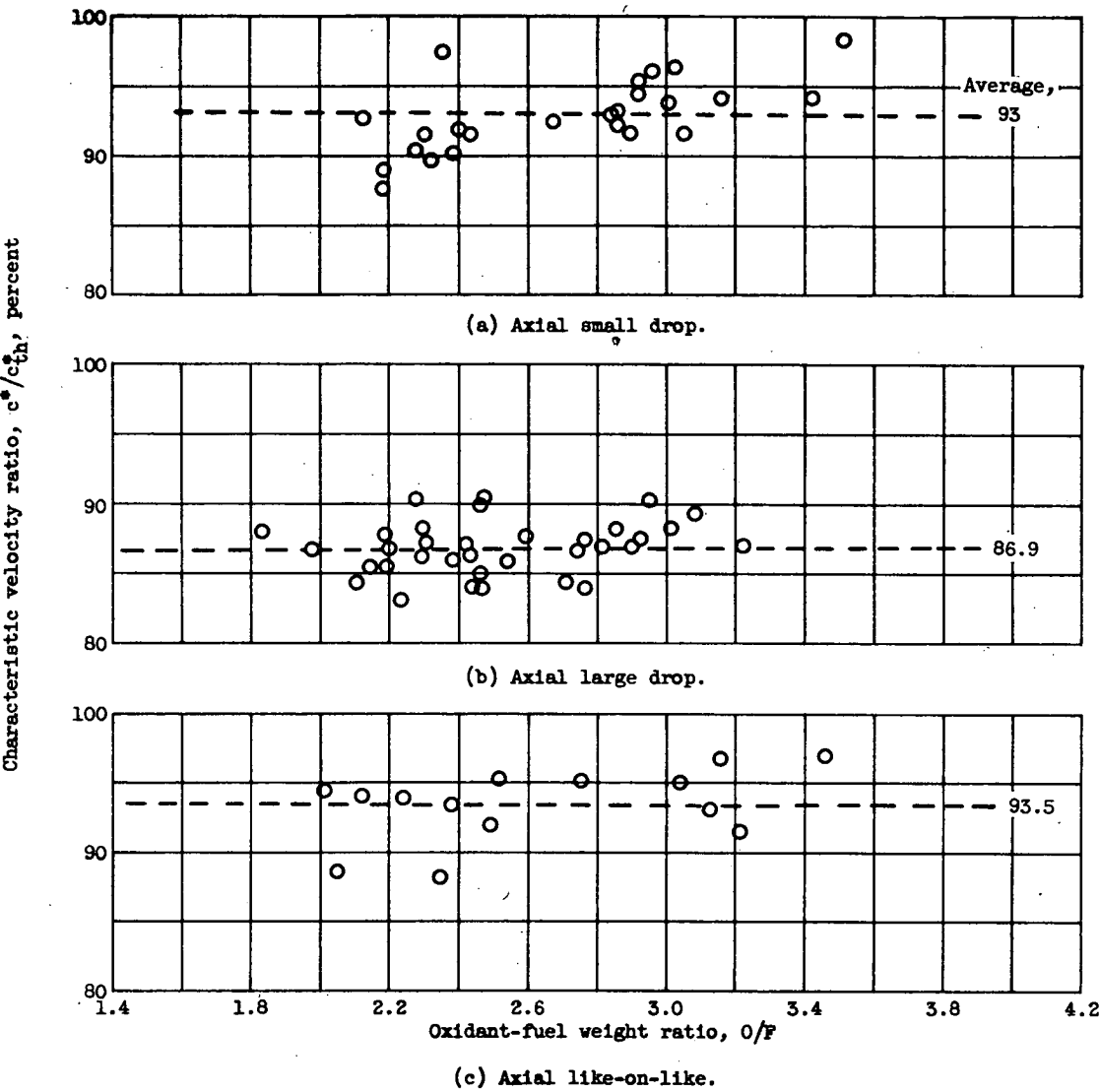
Figure 6. - Injector performance.
