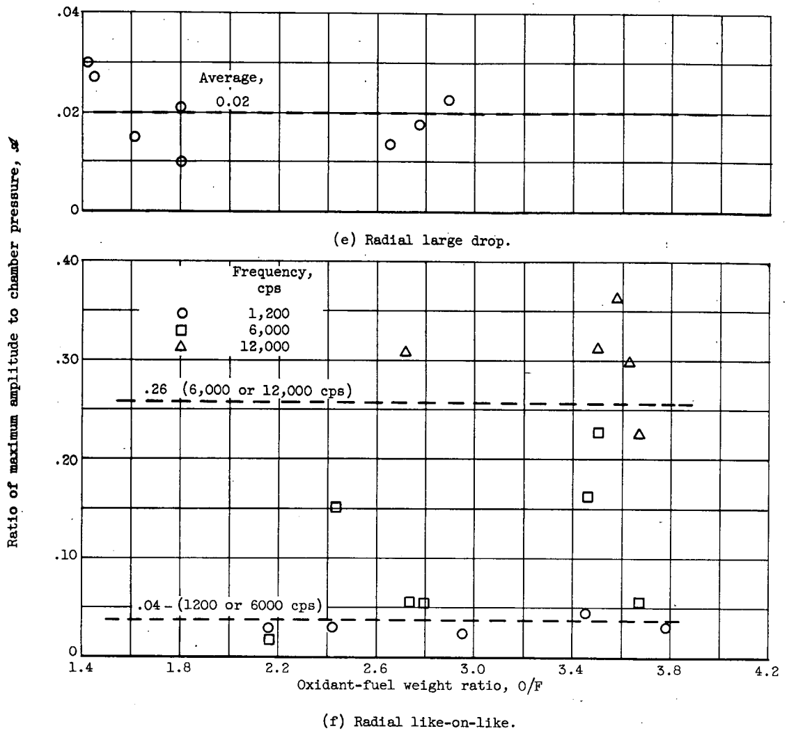
Figure 7. - Concluded. Variation of screaming amplitude with oxidant-fuel ratio for each injector.
