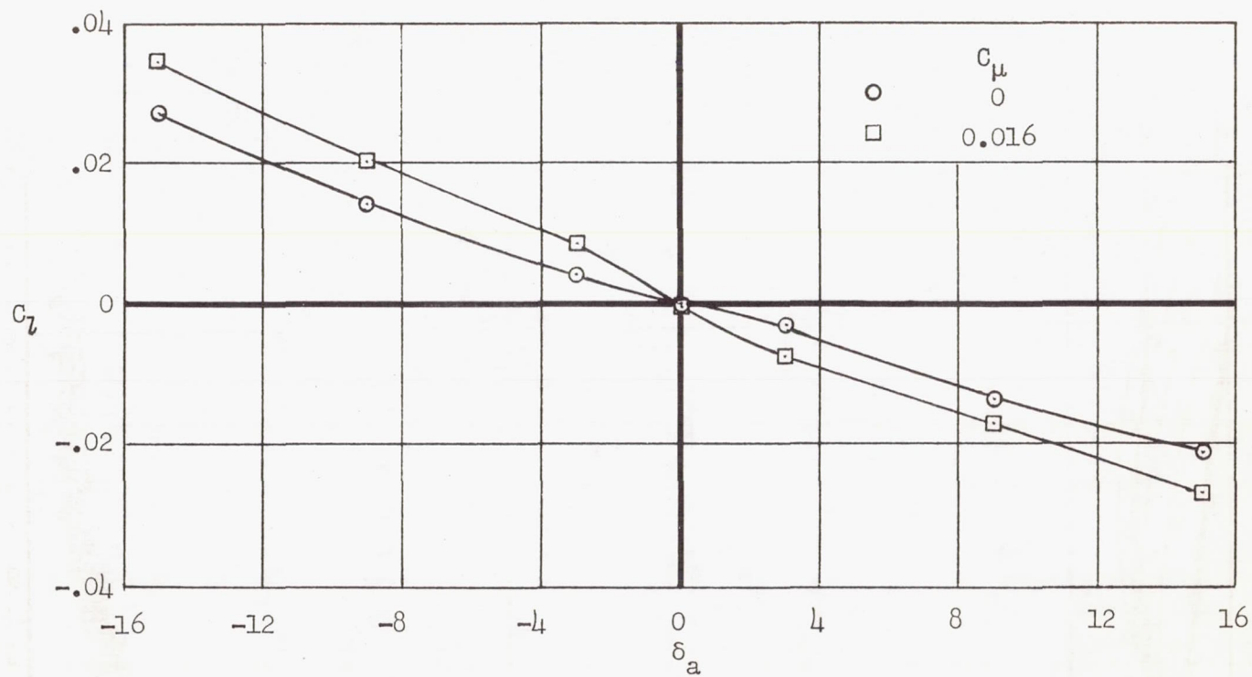
Figure 10.- Comparison of aileron effectiveness without and with flap blowing; \delta_F = 60^\circ .
