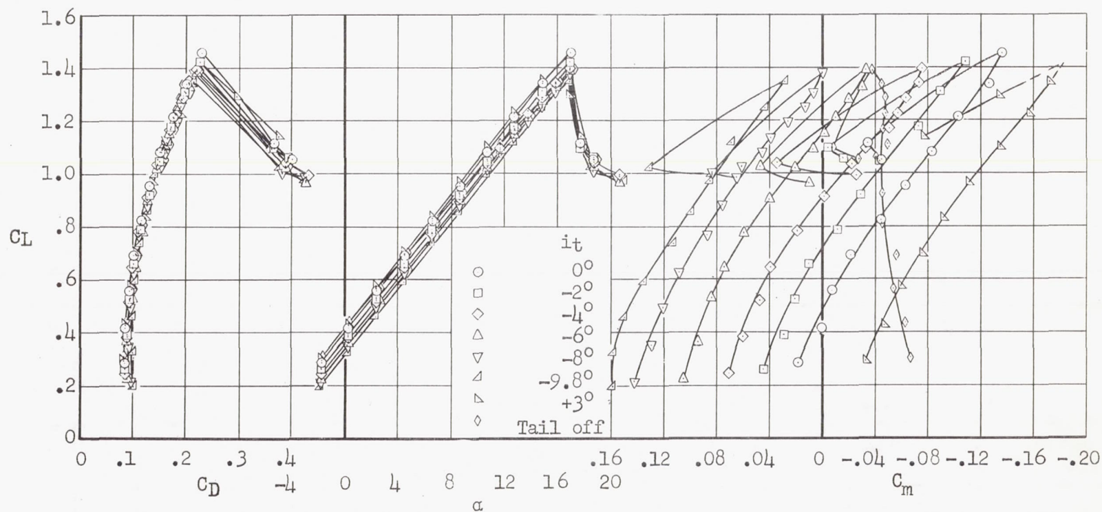
Figure 5.- Aerodynamic characteristics of the airplane with the horizontal tail; \delta_F = 45^\circ .
