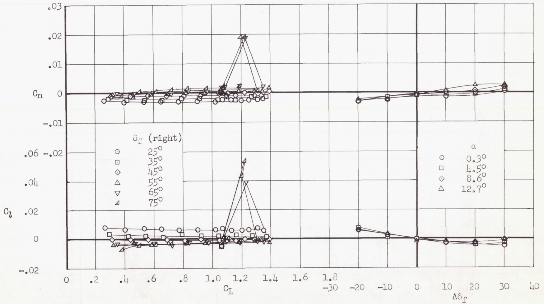
(b) Lateral characteristics.
