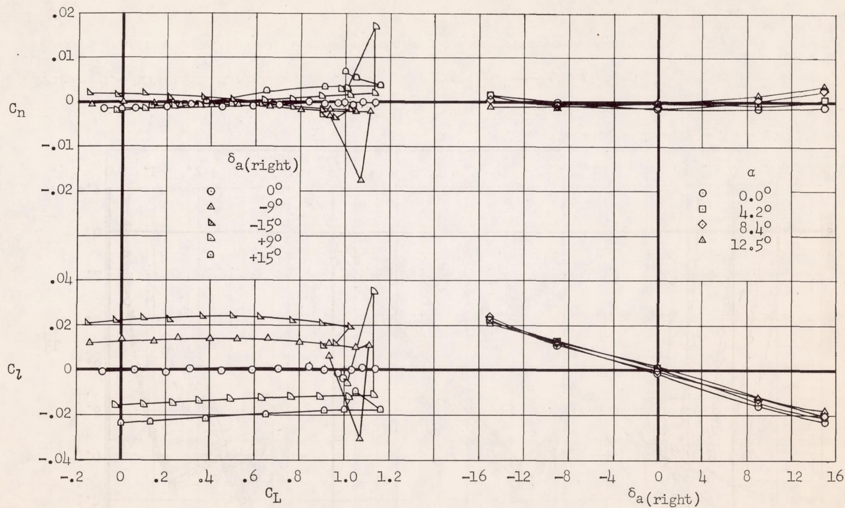
(b) Lateral characteristics.
