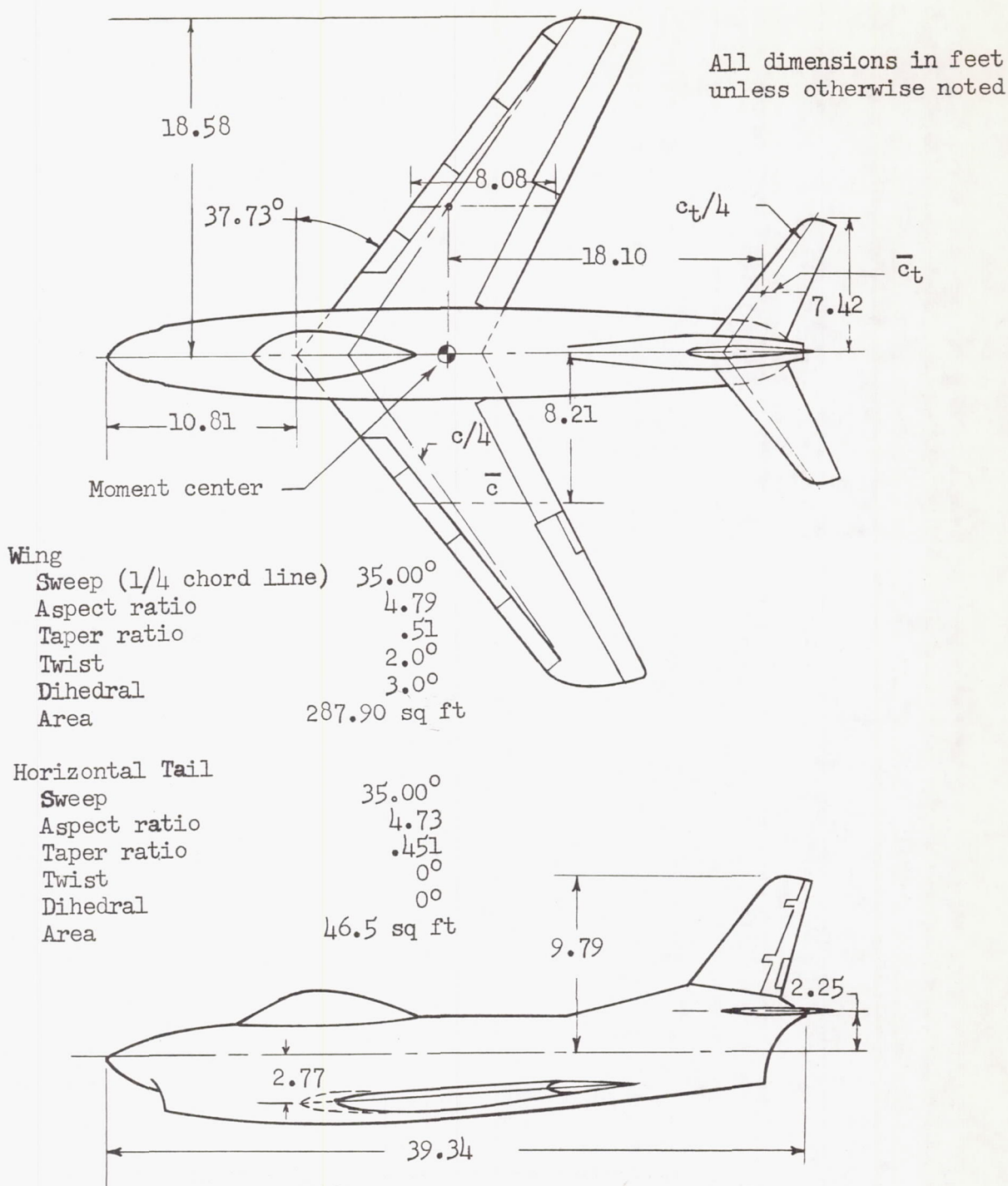
Figure 2.- General arrangement of YF-86D airplane.
