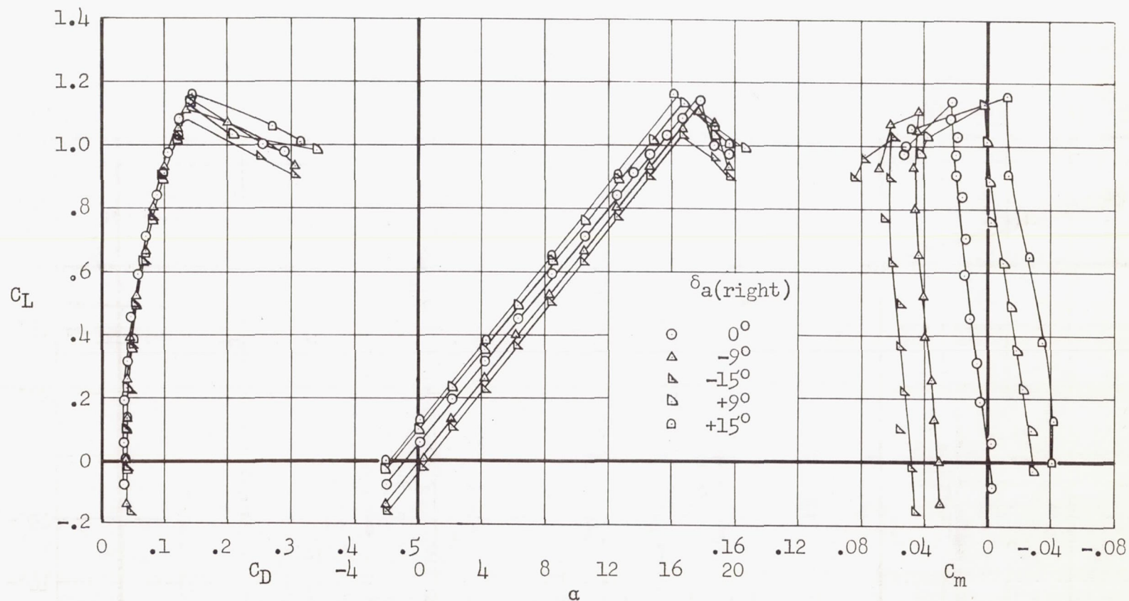
(a) Longitudinal characteristics.
