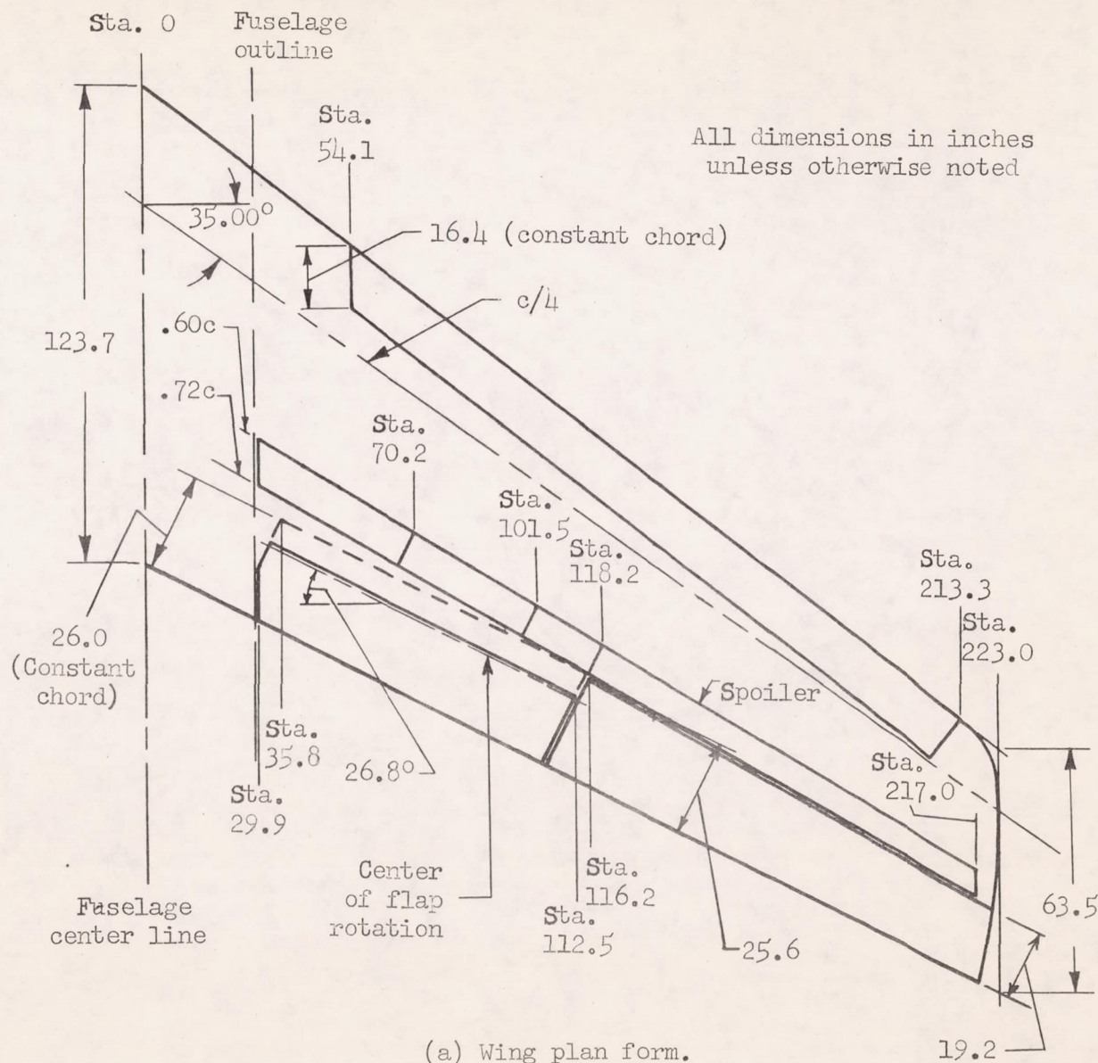
Figure 3.- Details of wing with lateral control devices and blowing flap.
