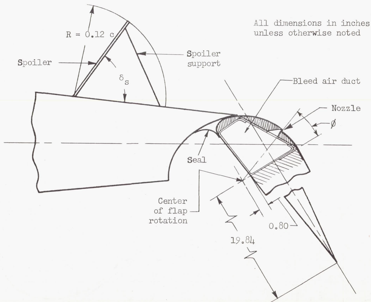
(b) Section view of blowing flap and spoiler.
