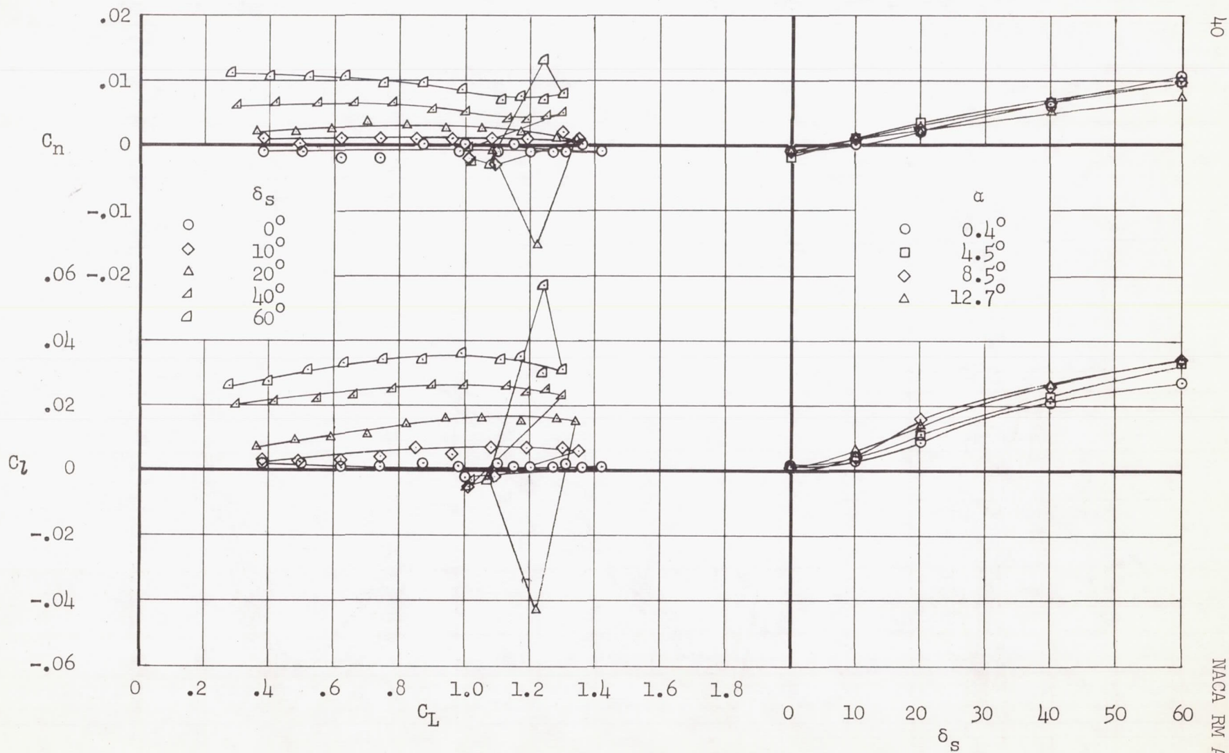
(b) Lateral characteristics.
