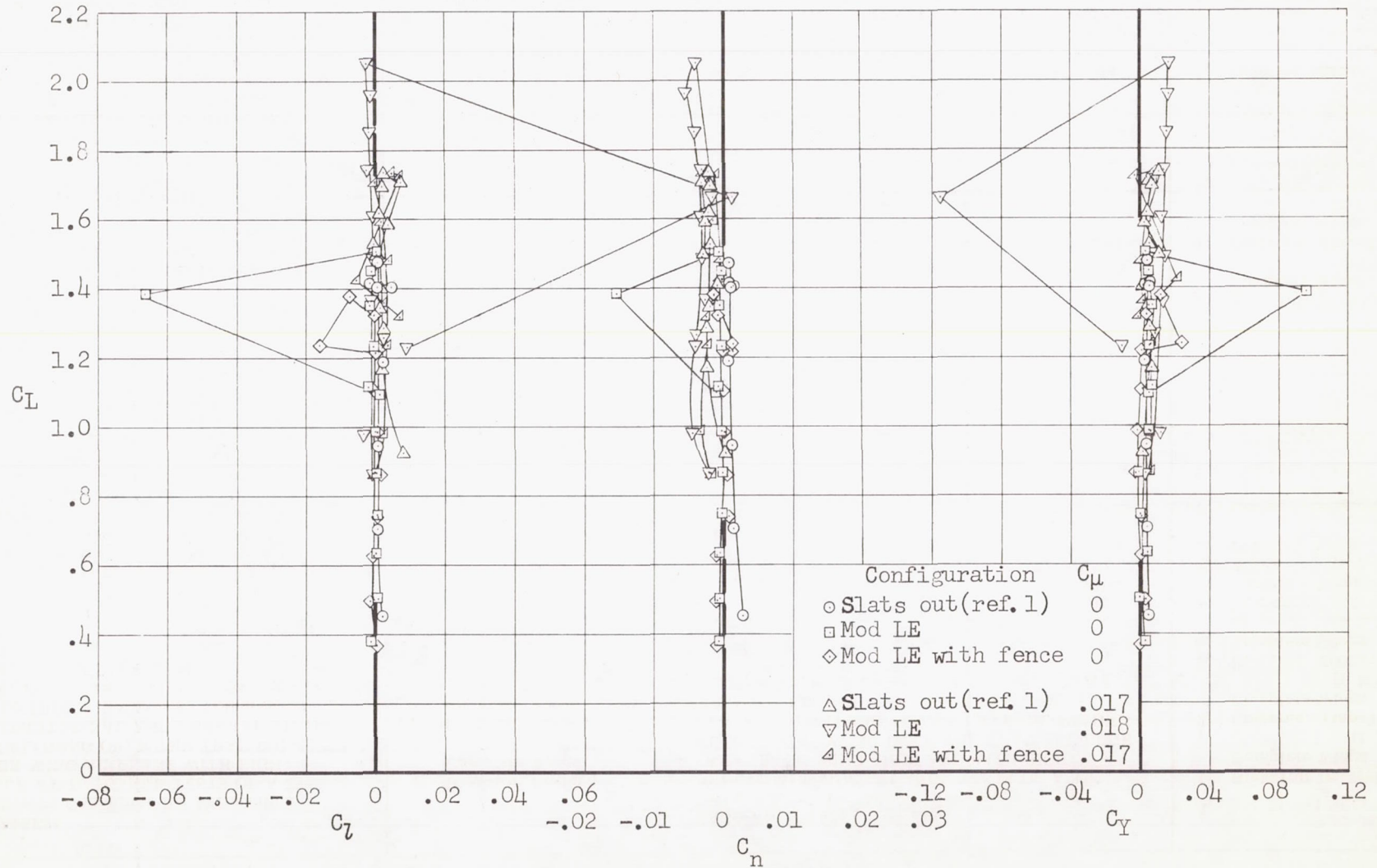
(b) Lateral characteristics.
