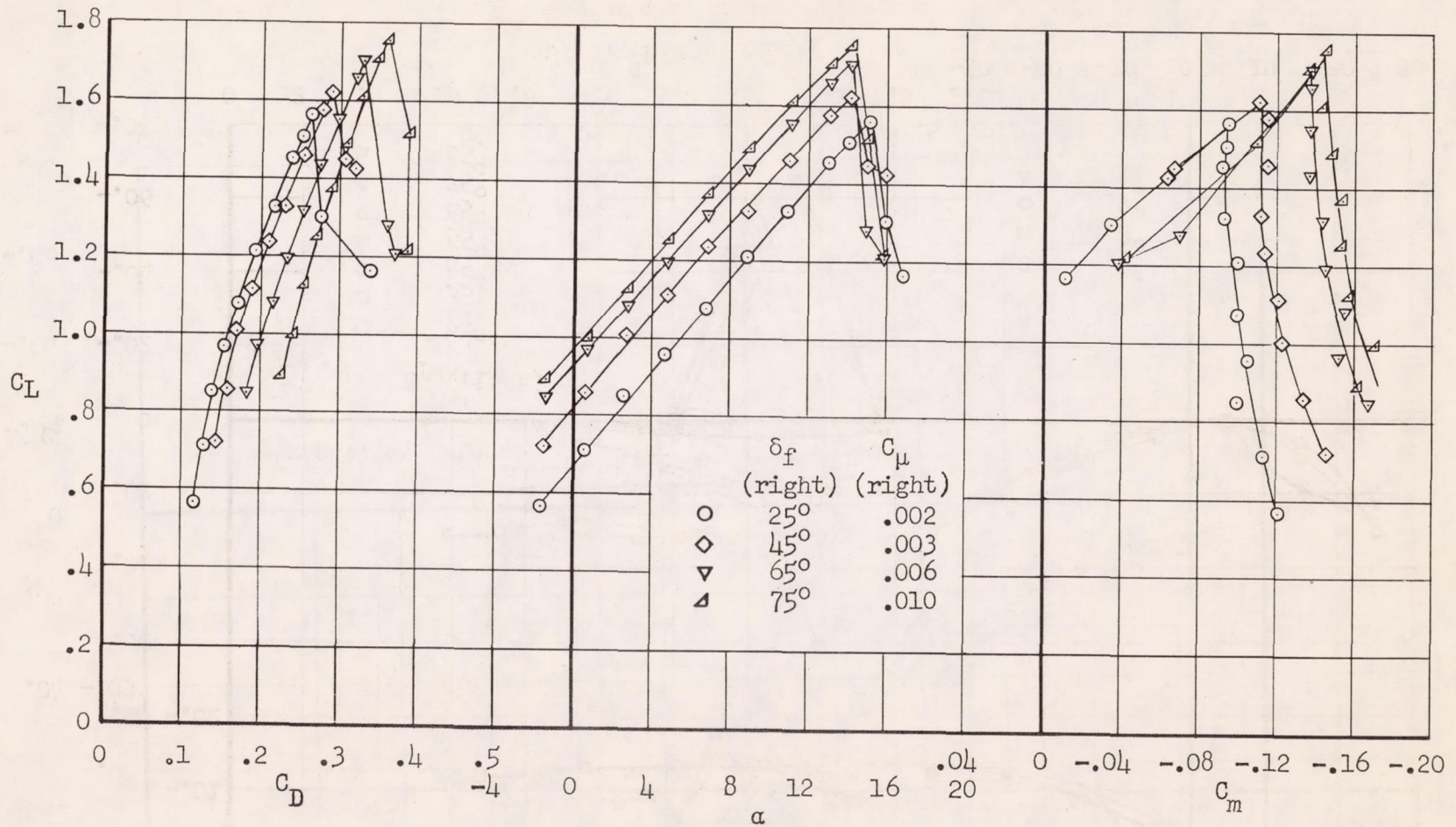
(a) Longitudinal characteristics.
