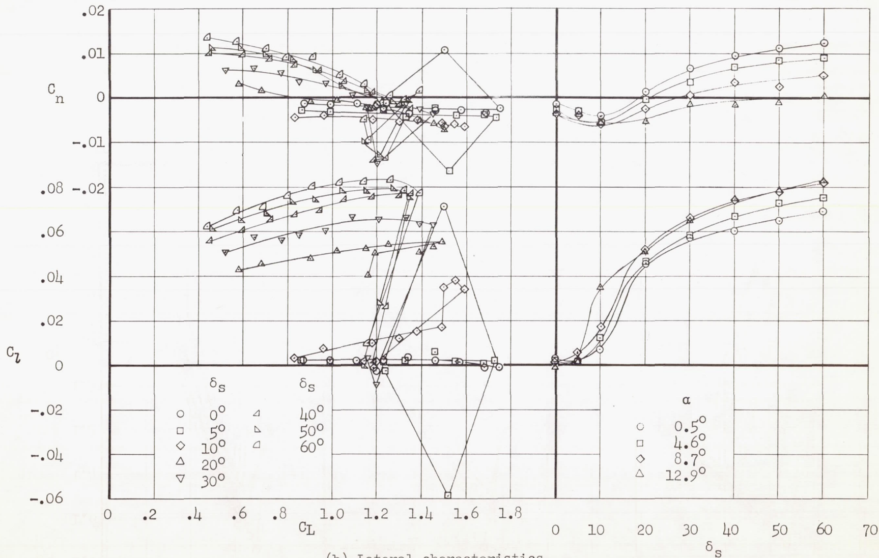
(b) Lateral characteristics.
