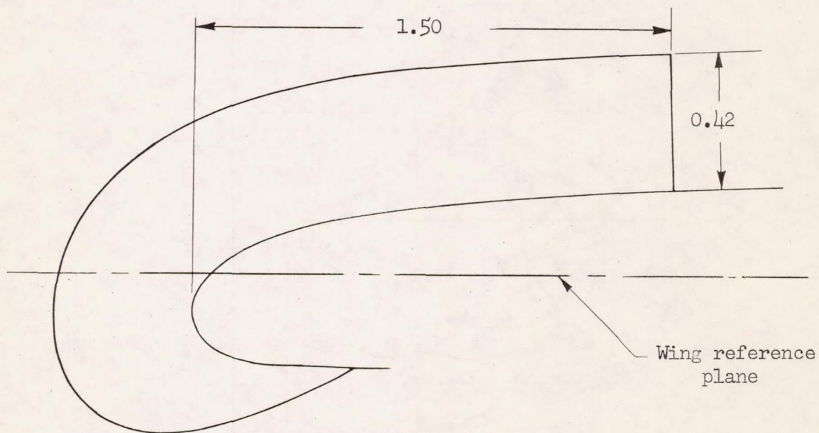
(b) Fence located at 0.628 semispan.
