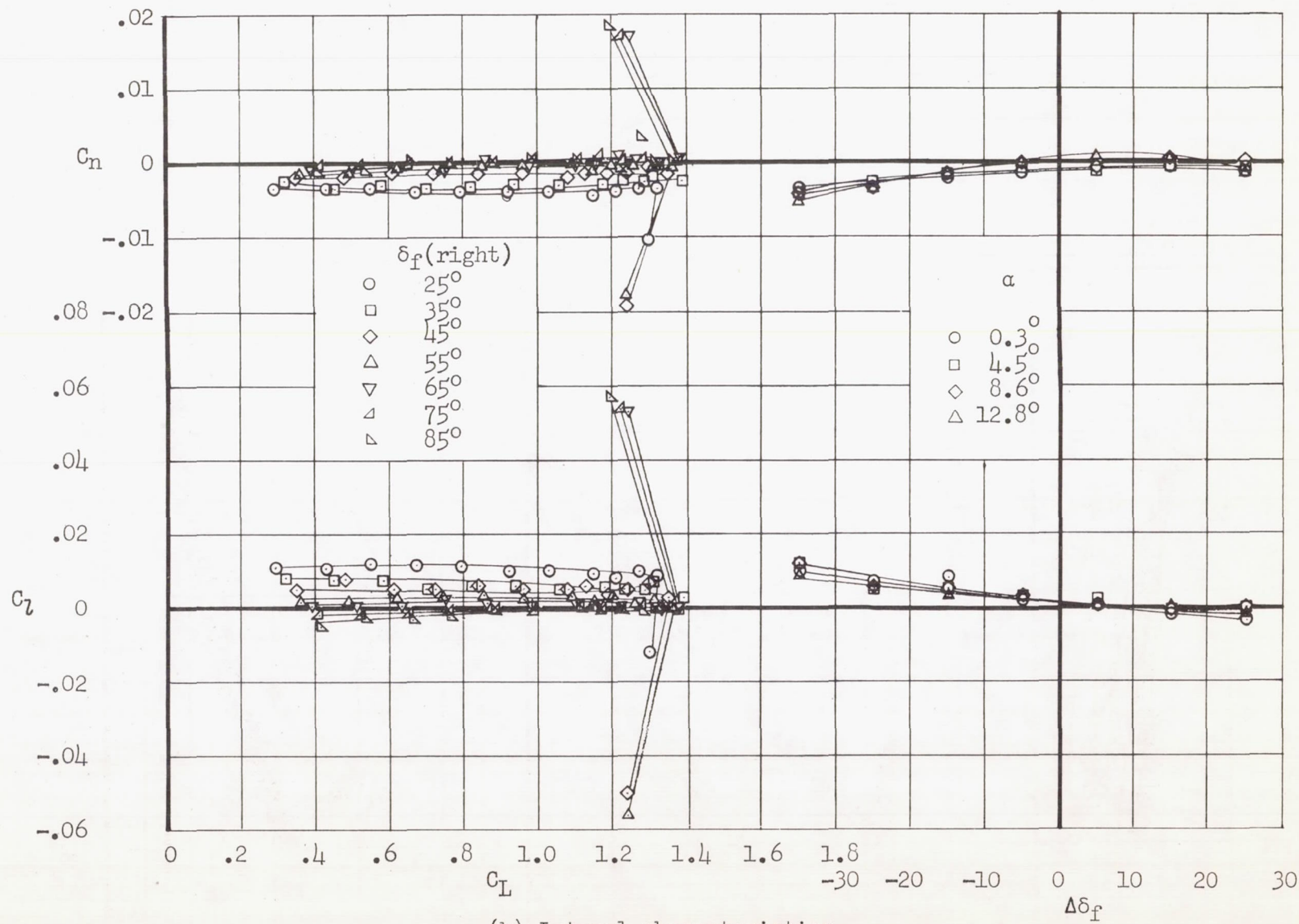
(b) Lateral characteristics.
