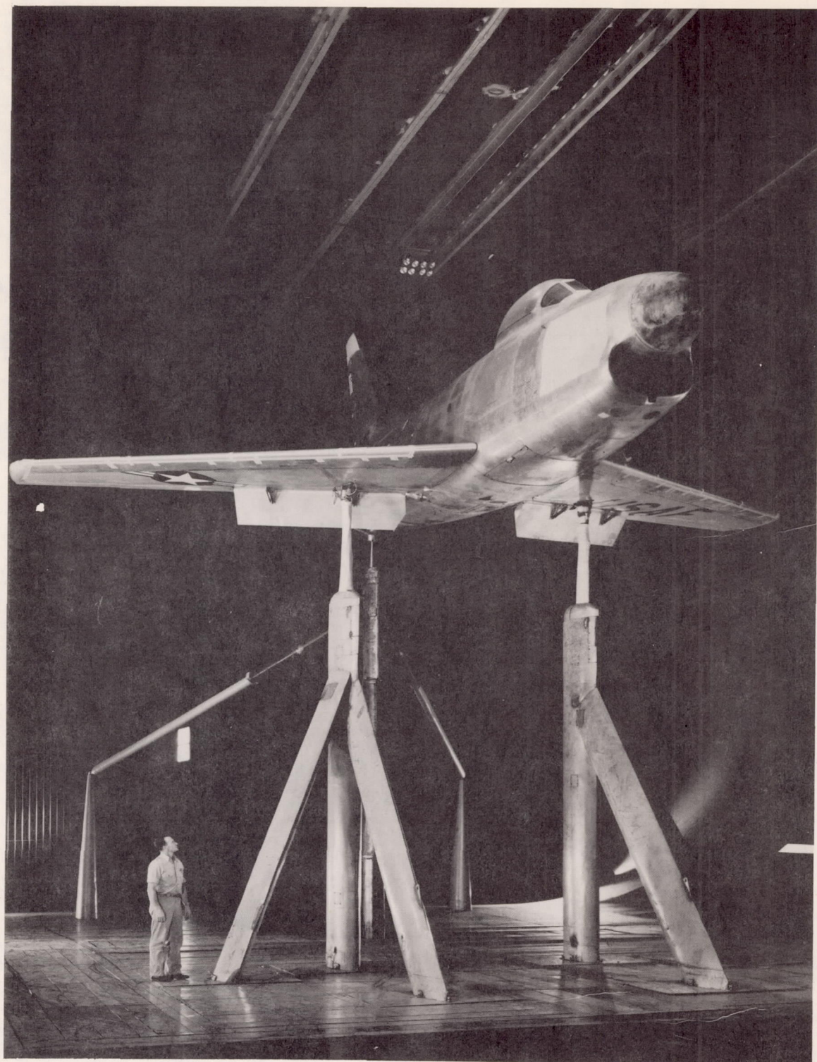
Figure 1.- Photograph of YF-86D airplane mounted in the Ames 40- by 80-foot wind tunnel.
