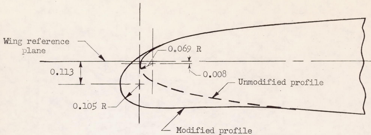
(a) Airfoil section at 0.857 semispan normal to wing quarter-chord line.
