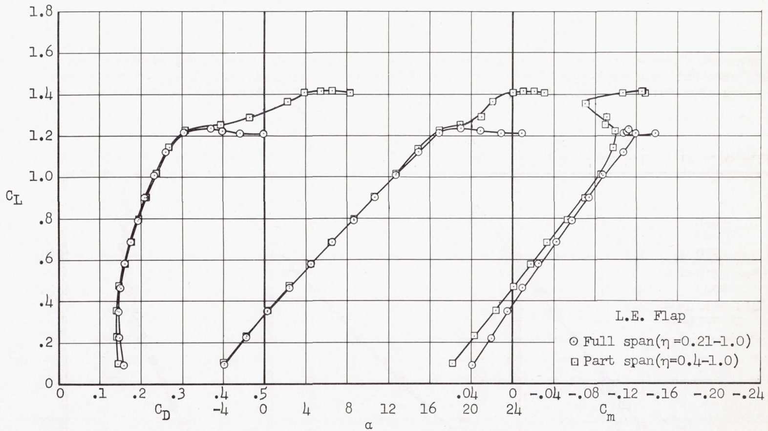
Figure 6.- Effect of a change in leading-edge flap span on the aerodynamic characteristics of the model with the small-span trailing-edge flap; suction on leading-edge flap; \delta_n = 50^\circ ; plain leading edge; suction on trailing-edge flap.
