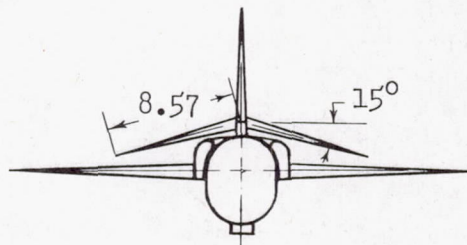
Figure 2.- Dimensional details of the model.
