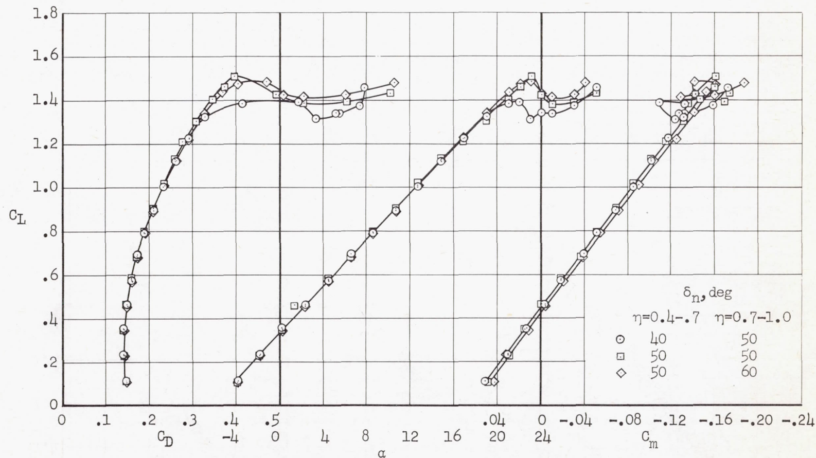
Figure 8.- Aerodynamic characteristics of the model with several outboard leading-edge flap configurations; small trailing-edge flap with area suction; leading-edge flap area suction ( \eta = 0.4 - 1.0 ); \delta_n = 30^\circ for \eta = 0.21 - 0.4 ; modified leading edge ( \eta = 0.7 - 1.0 ).
