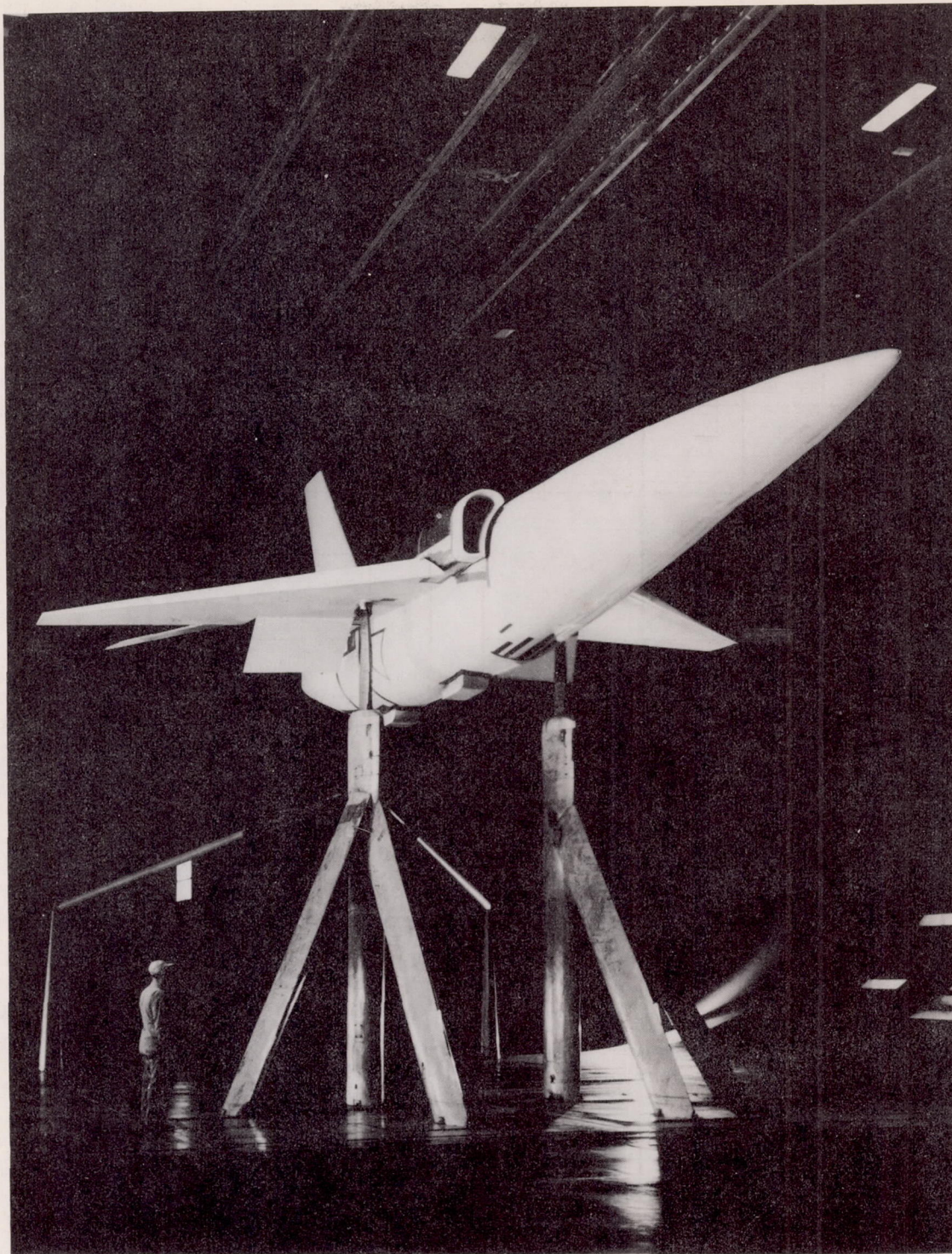
Figure 1.- Photograph of the model mounted in the Ames 40- by 80-foot wind tunnel.
