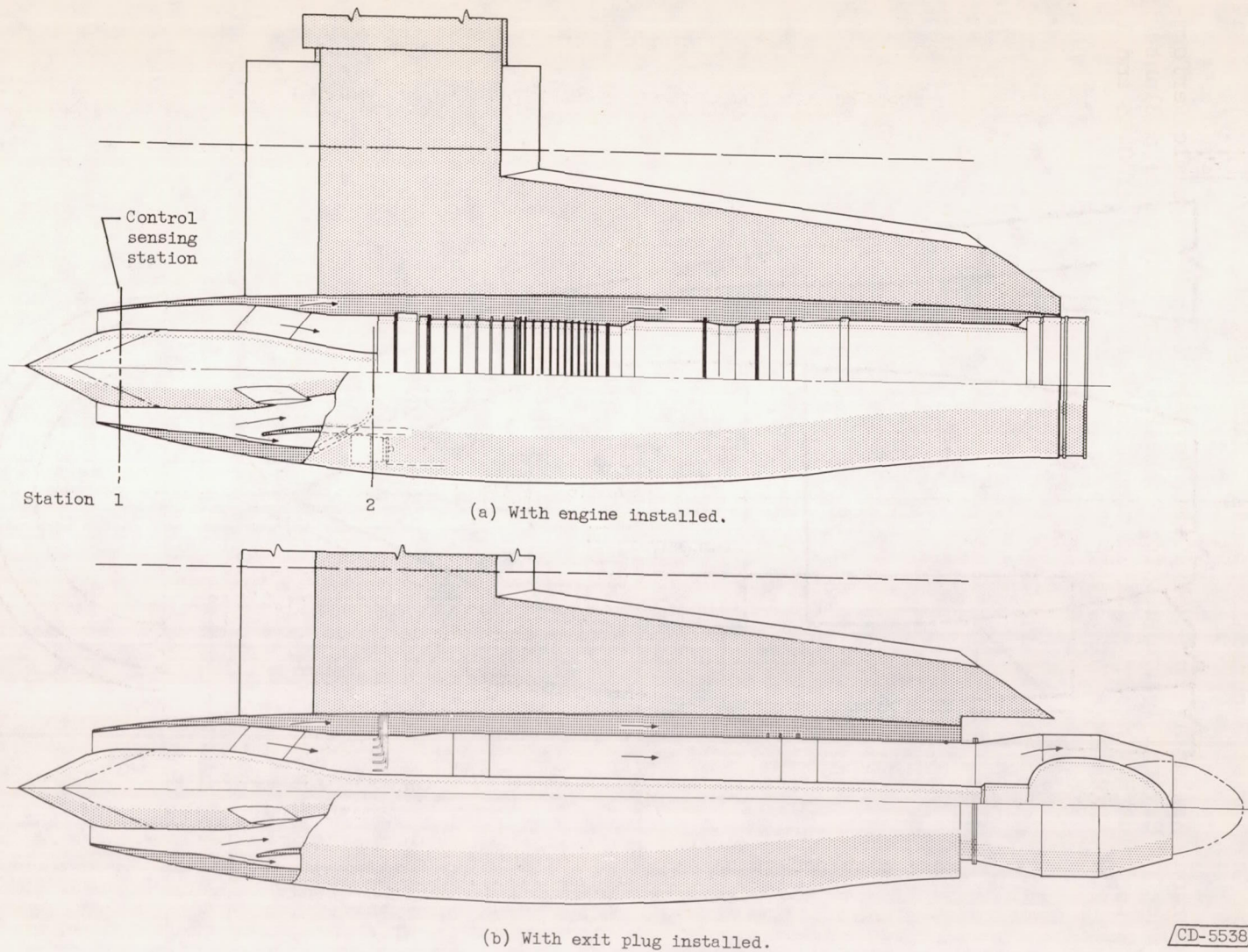
Figure 1. - Nacelle configuration.
