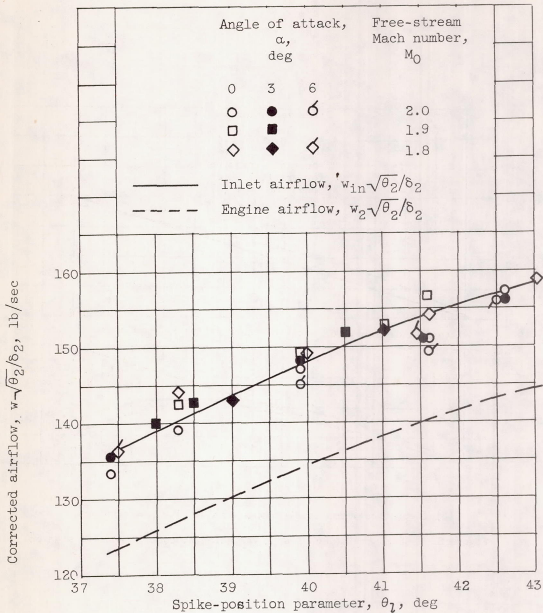
Figure 4. - Concluded. Critical inlet performance.
