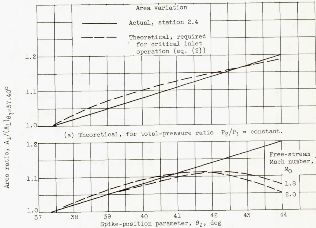
Figure 5. - Characteristics of area variation at control sensing station.
