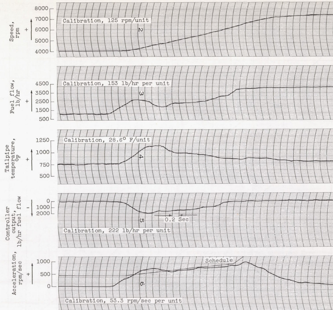
Figure 12. - Typical acceleration transient.
