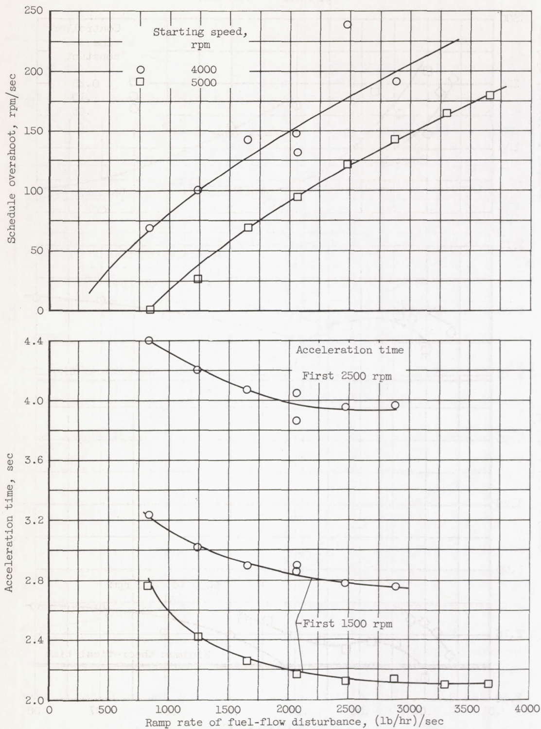
Figure 16. - Variation of schedule overshoot and acceleration time with ramp rate of fuel-flow disturbance at starting speeds of 4000 and 5000 rpm.
