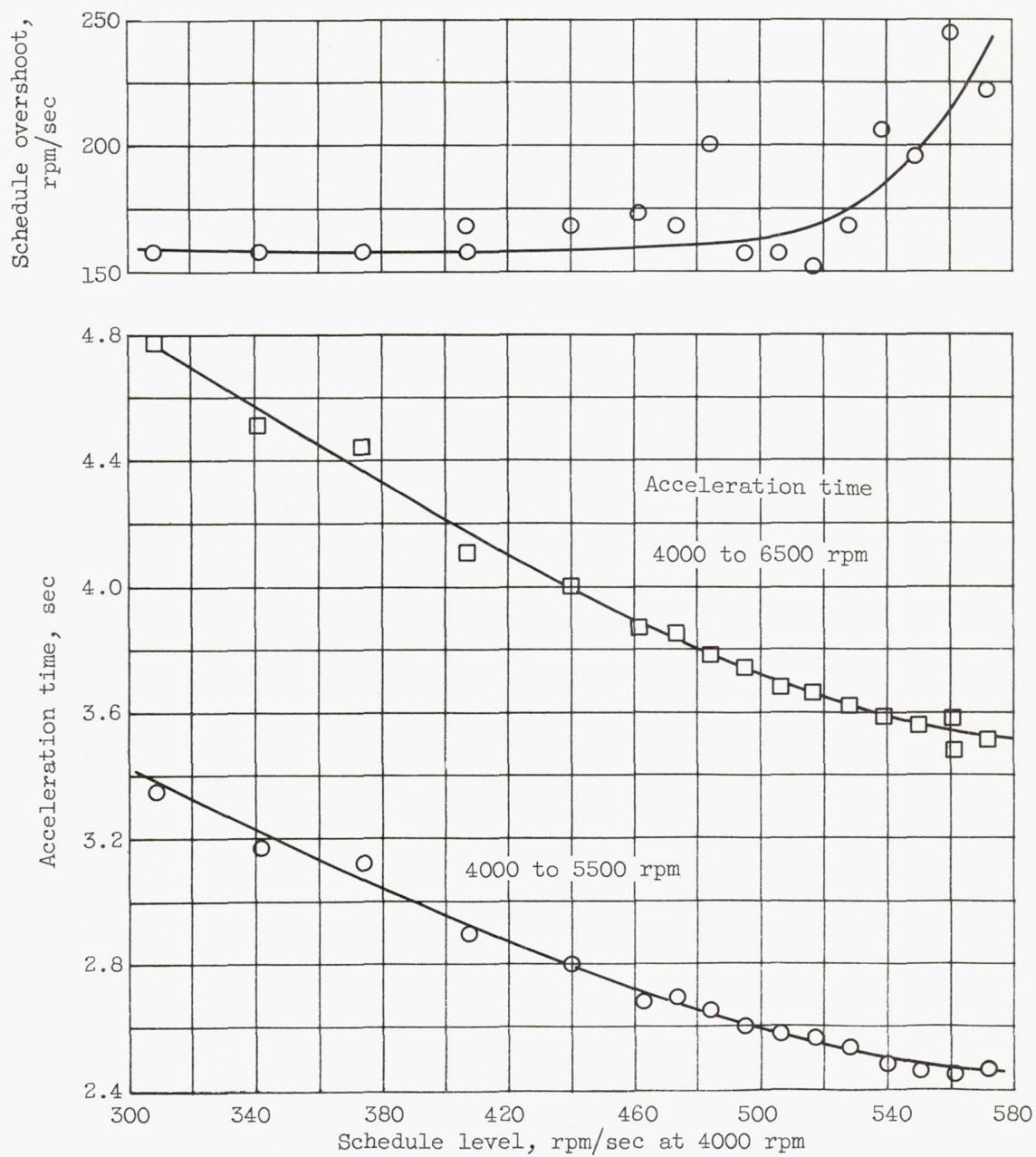
Figure 17. - Variation of schedule overshoot and acceleration time with schedule level.
