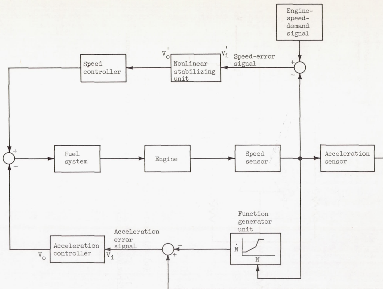
(a) Block diagram.
