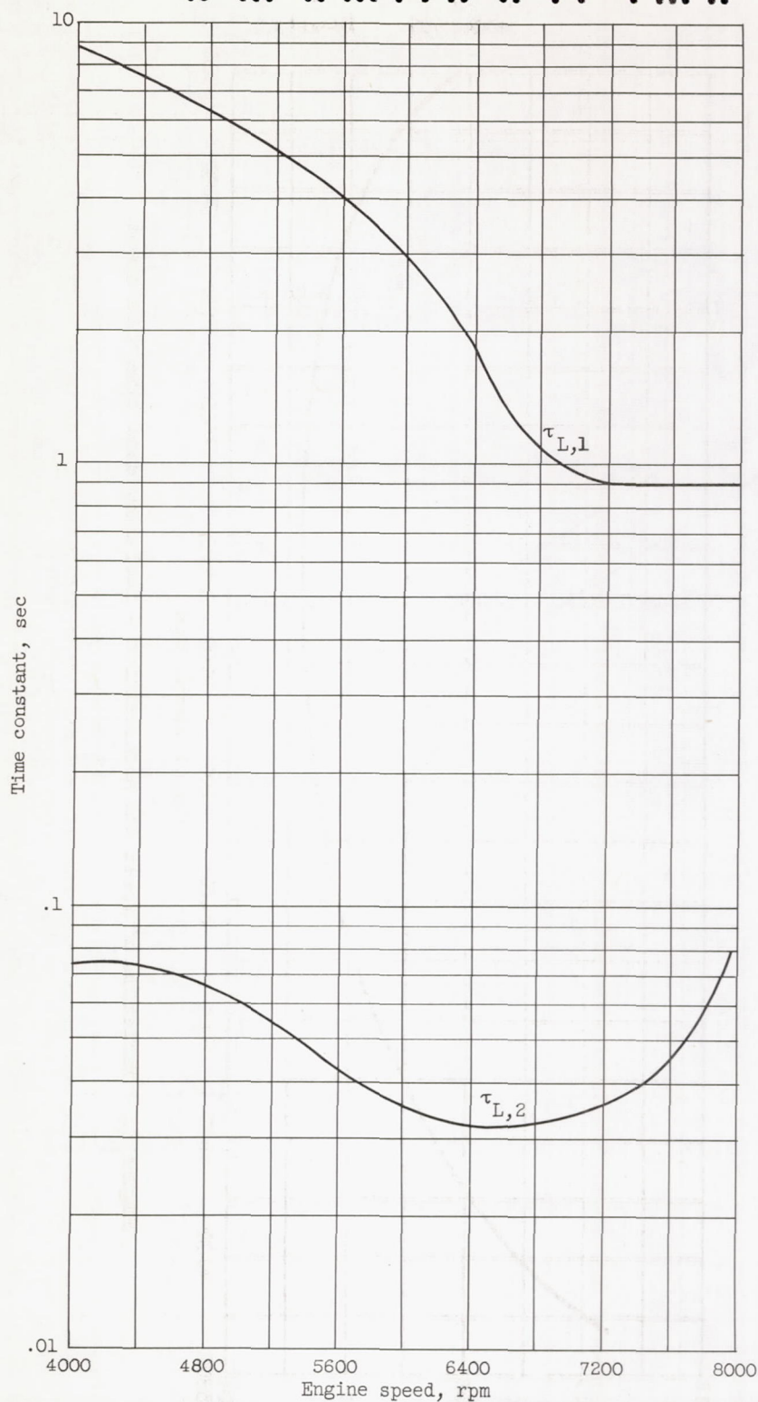
Figure 8. - Variation of engine-speed - fuel-flow time constants with speed.
