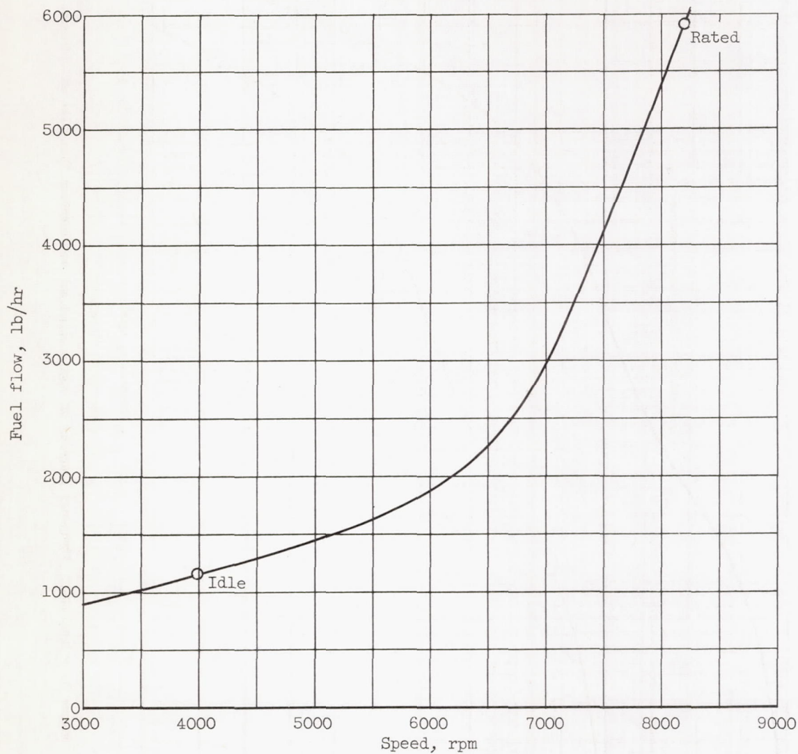
Figure 4. - Variation of steady-state fuel flow with speed.
