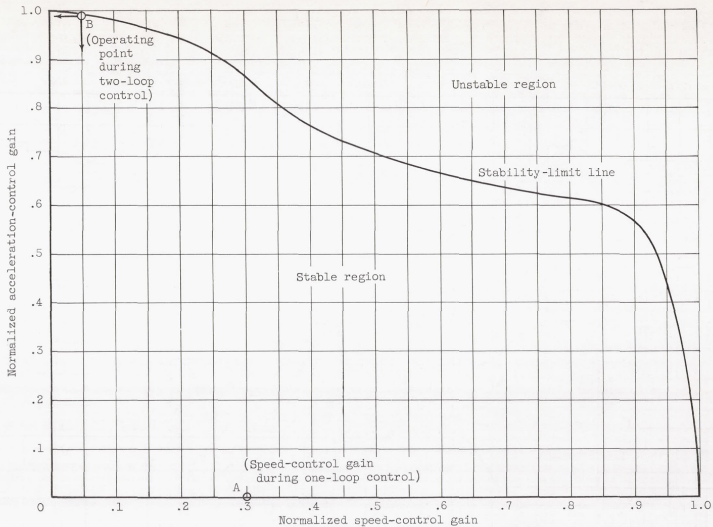
Figure 10. - Variation of acceleration loop stability-limit gain with speed loop gain (includes engine dynamics at 4500 rpm).
