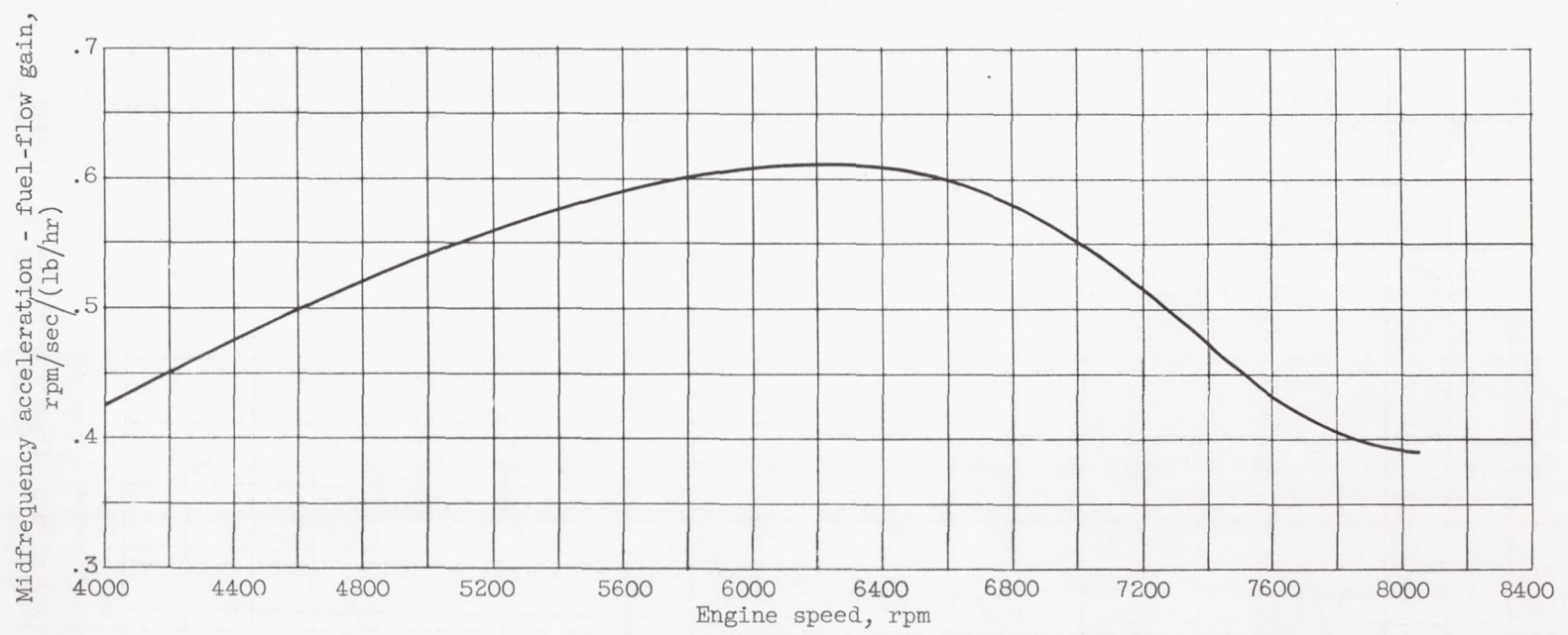
Figure 6. - Variation of midfrequency acceleration - fuel-flow gain with speed.
