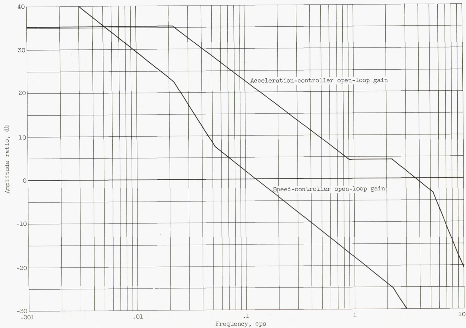
Figure 11. - Amplitude-frequency response of open-loop acceleration and speed controls at operating point chosen (straight-line approximation) (including engine dynamics at 4500 rpm).
