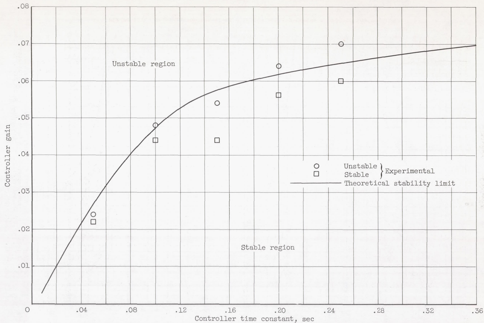
Figure 14. - Experimental- and theoretical-stability-limit gain variation with controller time constant.
