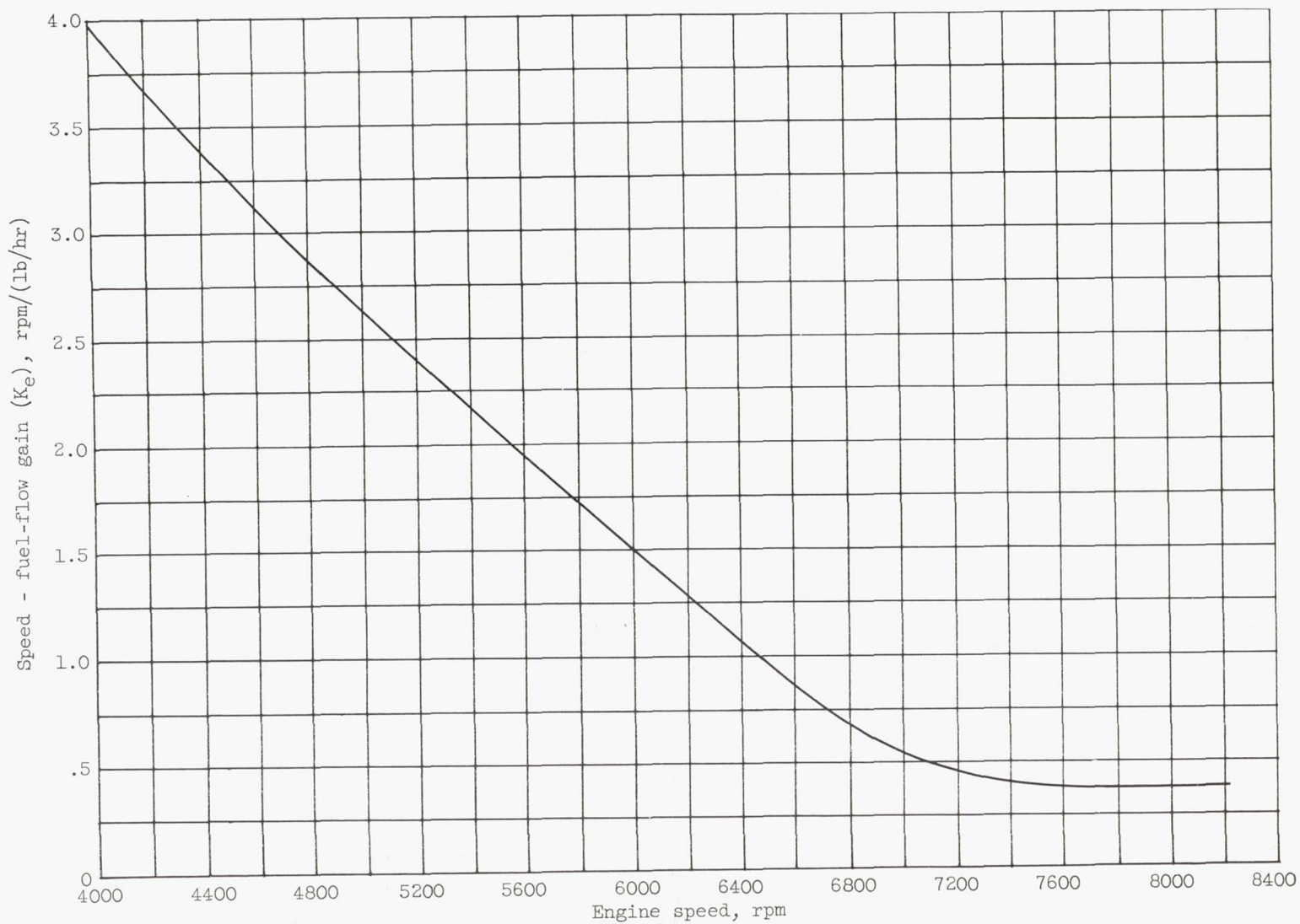
Figure 5. - Variation of steady-state speed - fuel-flow gain with speed.
