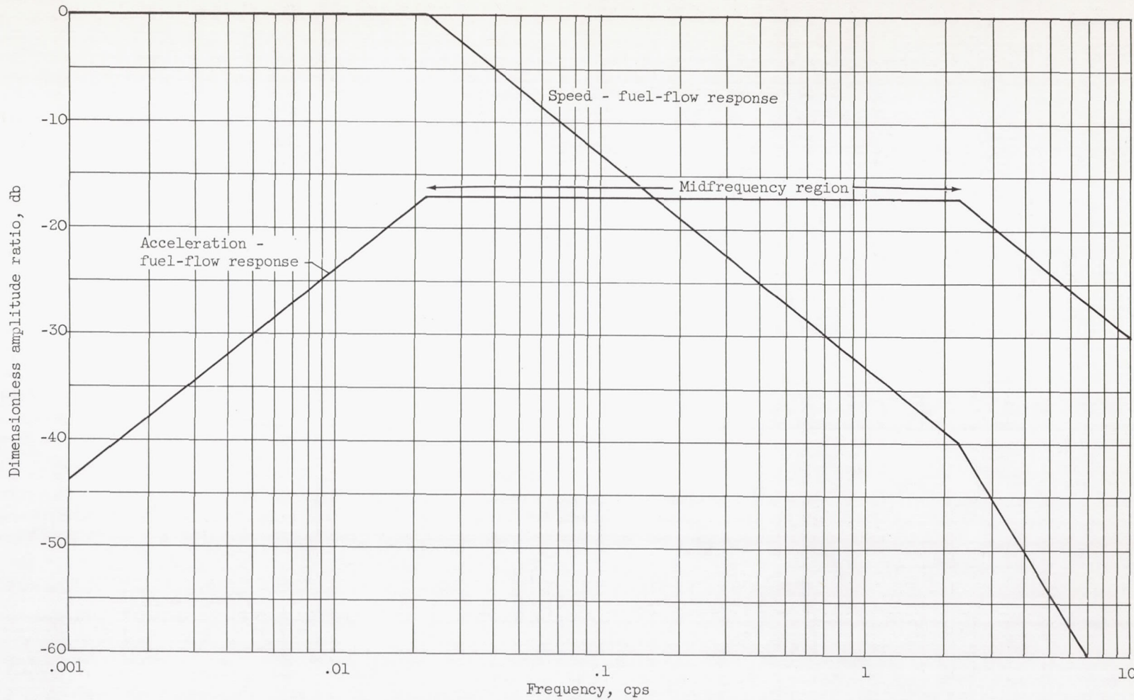
(a) Amplitude frequency.
