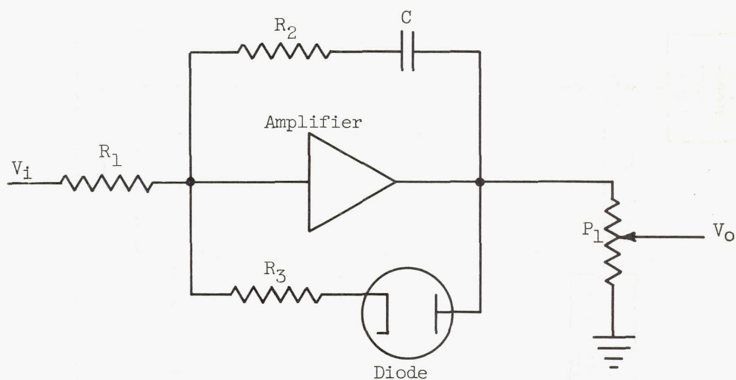
(b) Schematic diagram of nonlinear control.
