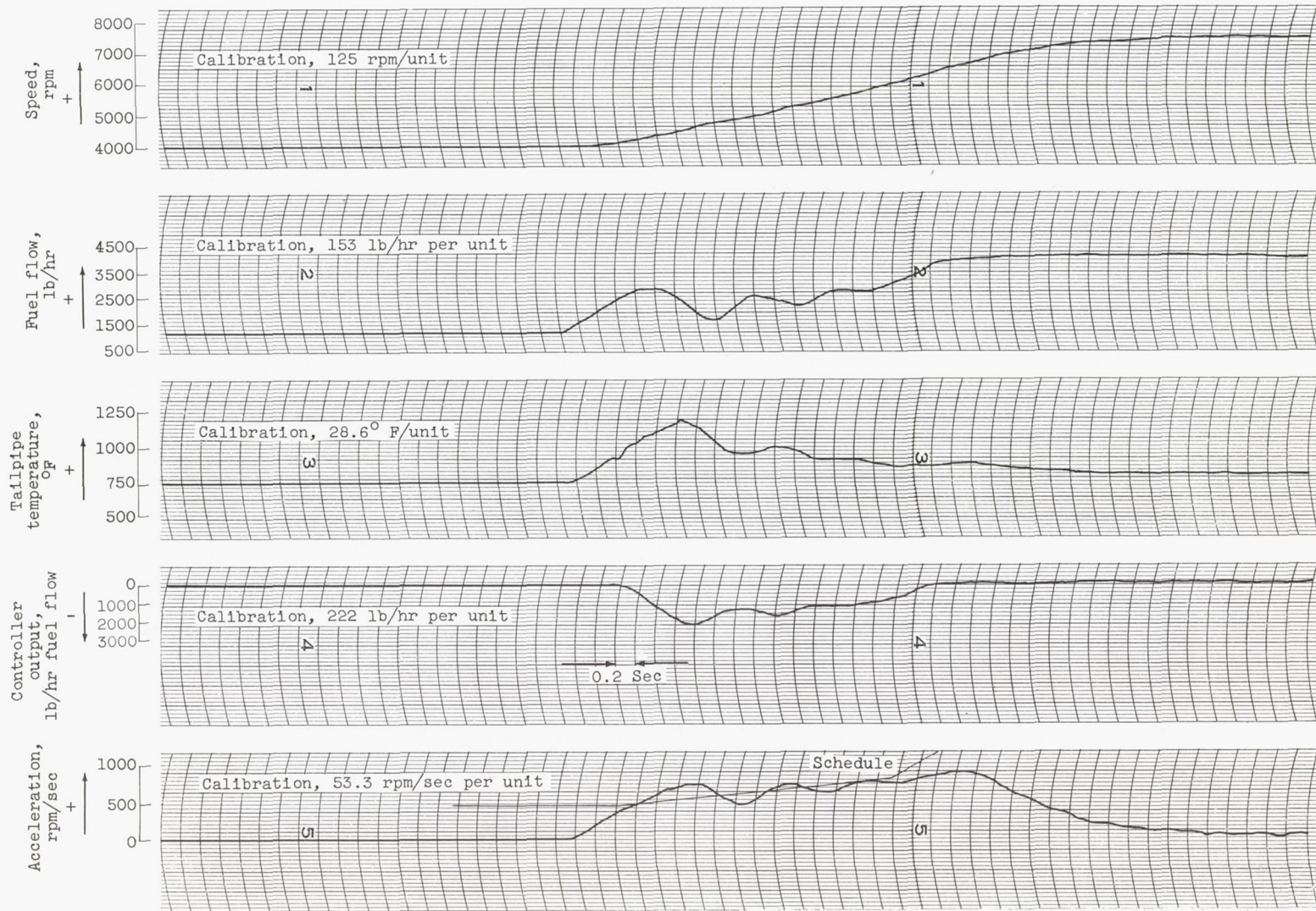
Figure 13. - Acceleration transient with instability during a part of the transient.
