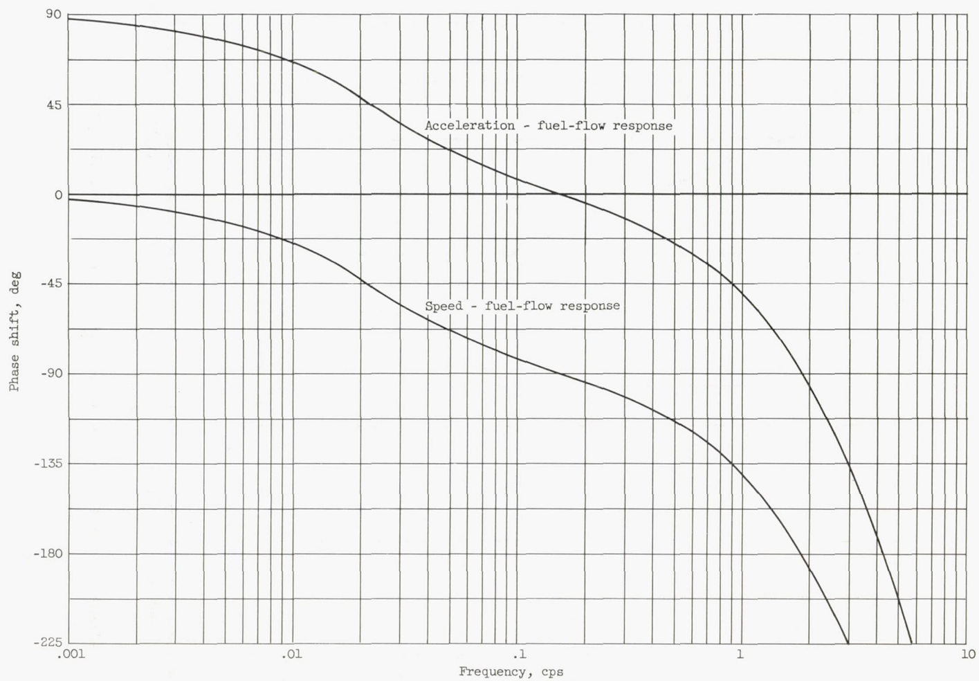
(b) Phase shift frequency.
