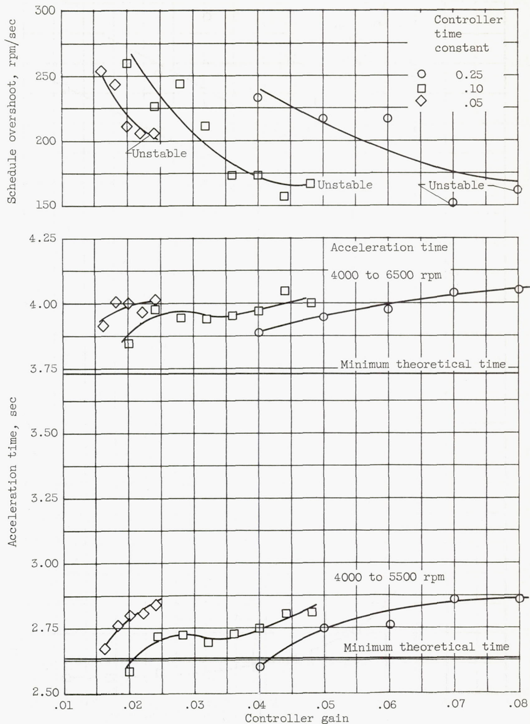
Figure 15. - Variation of schedule overshoot and acceleration time with controller gain and time constant.
