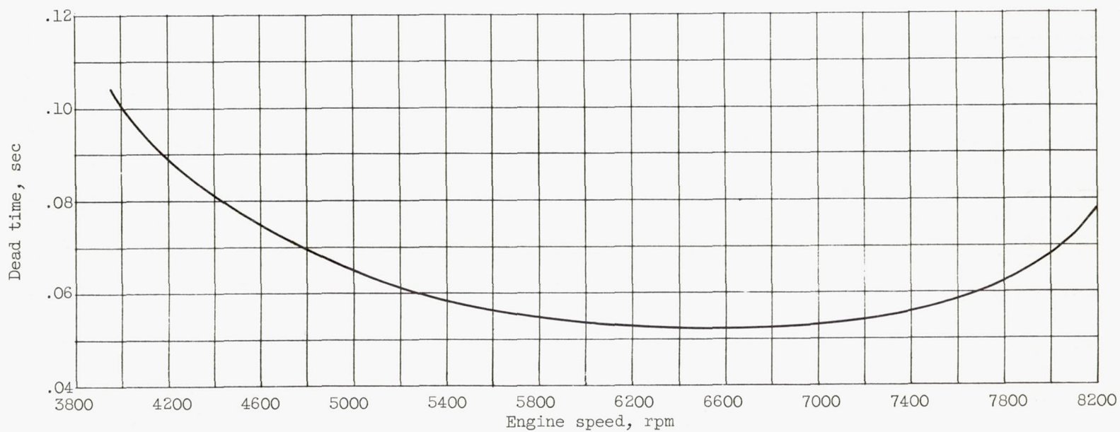
Figure 7. - Variation of speed and acceleration - fuel-flow dead time with speed.
