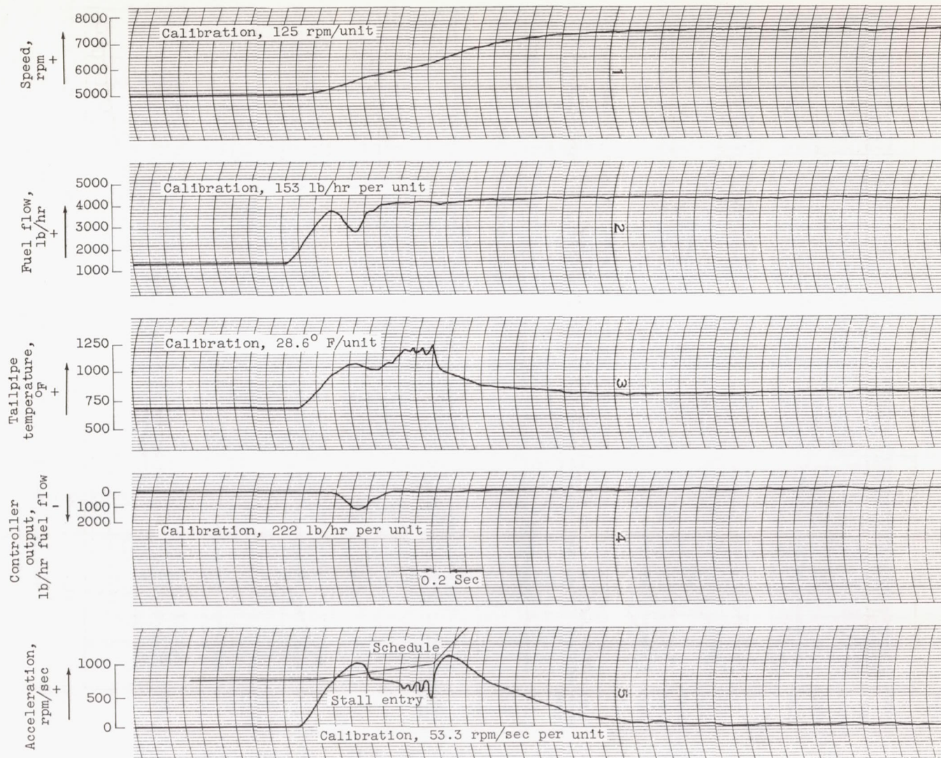
Figure 18. - Trace of acceleration transient with high schedule level resulting in engine stall.
