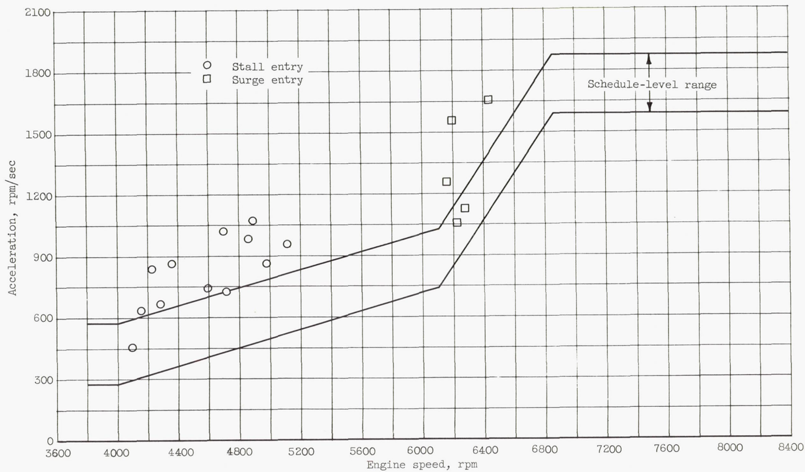
Figure 9. - Variation of stall and surge accelerations and schedule-level range used with speed.
