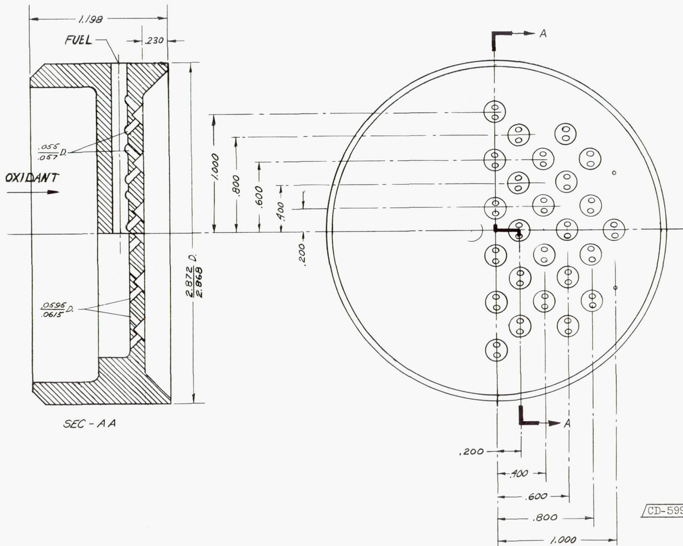
(a) RMI-1 injector; 22 pairs each of like-on-like fuel and oxidant holes with surface impingement at 90°.
