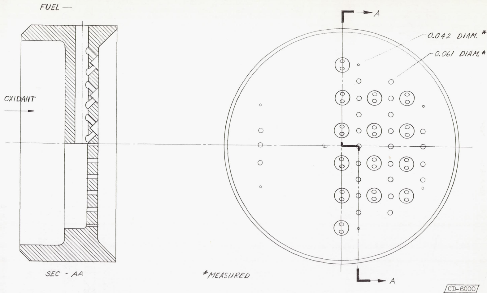
(b) RMI-2 injector; 22 pairs of like-on-like fuel holes with surface impingement at 90^\circ ; 22 showerhead oxidant holes.
