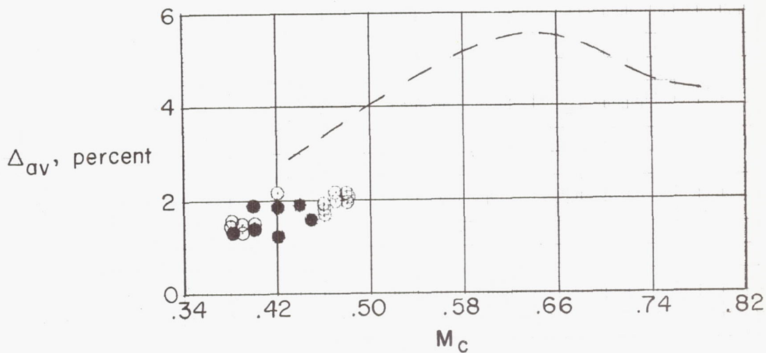
(b) Variation of distortion with compressor-face Mach number.
