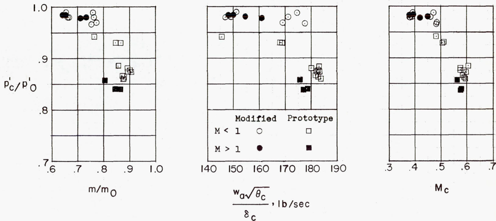
Figure 8.- Variation of compressor-face-pressure recovery with various flow-rate parameters; \alpha \approx 4^\circ .
