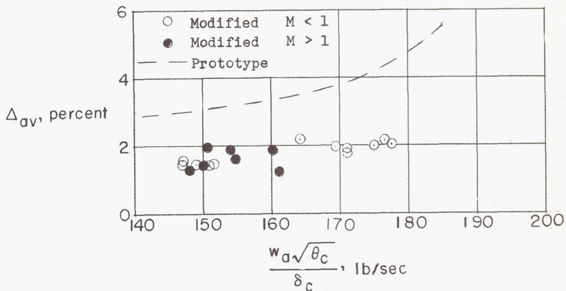
(a) Variation of distortion with normalized airflow rate.
