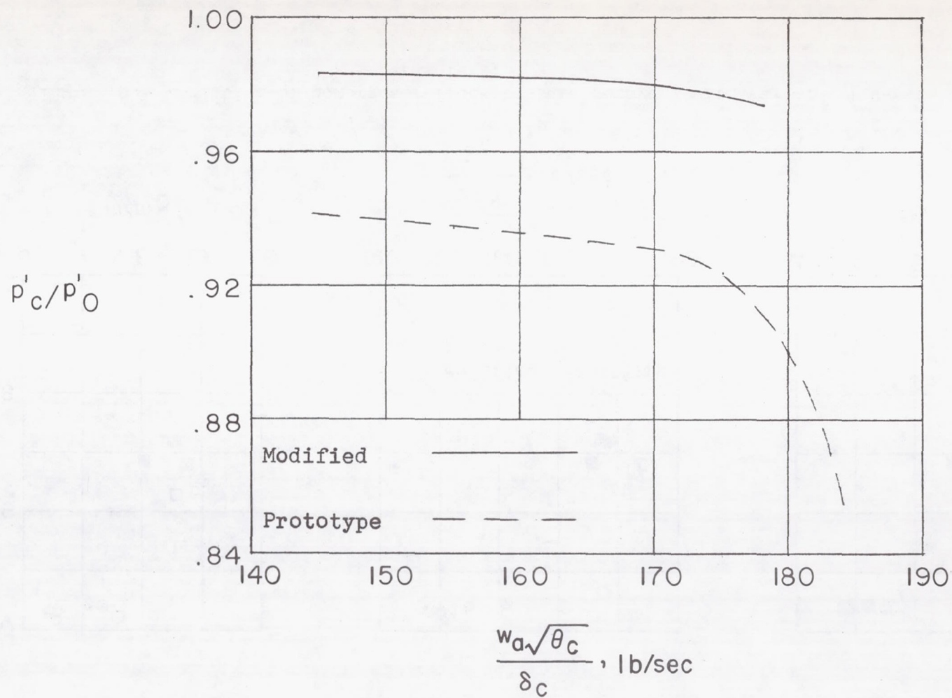
Figure 7.- Variation of compressor-face pressure recovery with normalized airflow rate; \alpha \approx 4^\circ ; M < 1 .
