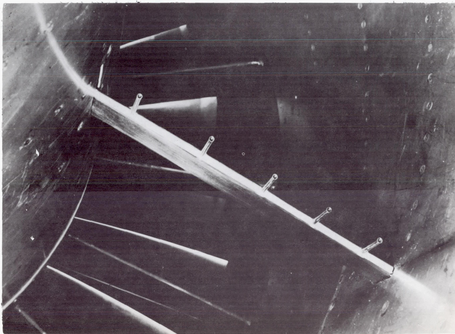
Figure 6.- Close-up view of survey rake, prototype installation. E-1585
