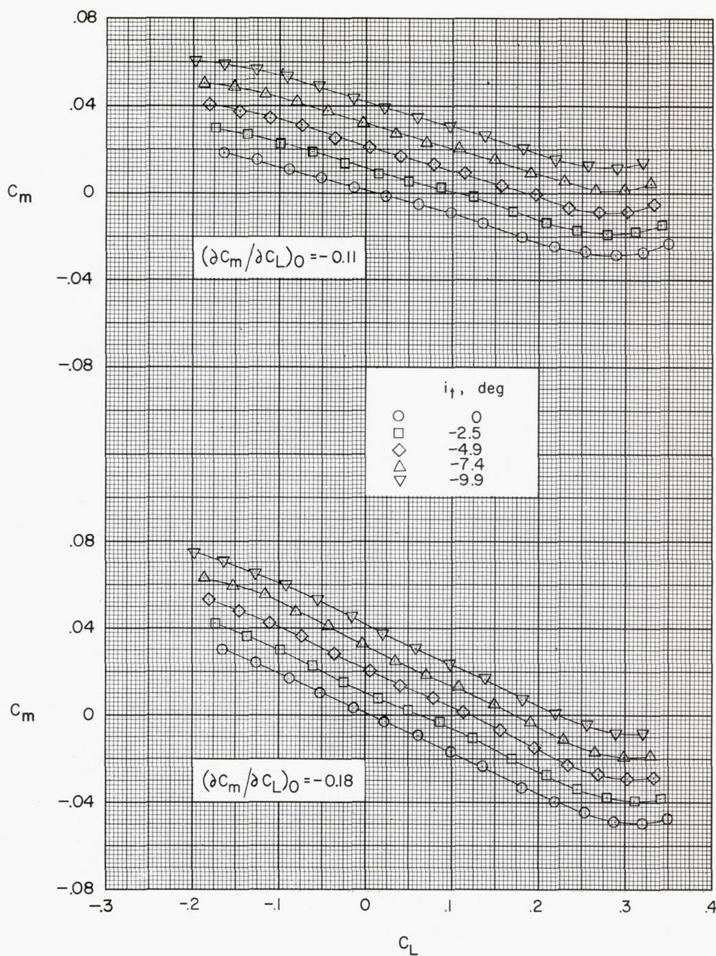
(b) (\partial C_m / \partial C_L)_0 = -0.11 and -0.18 .
