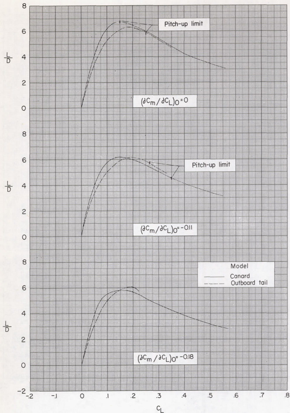
Figure 9.- Variation of trimmed L/D with lift coefficient for various longitudinal stability levels.
