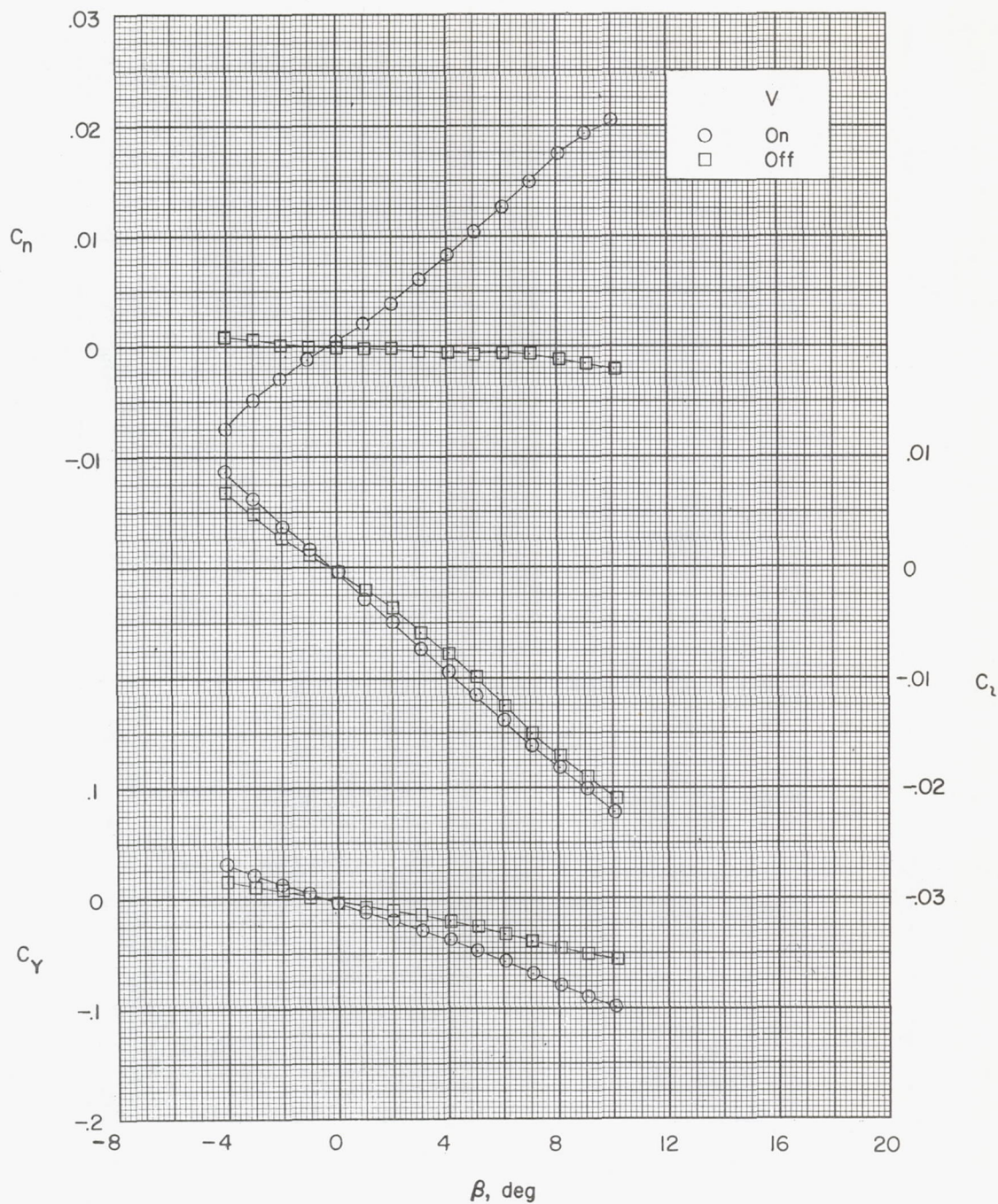
(a) Center of gravity at body station 21.97.
