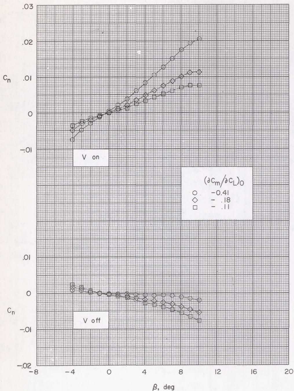
(b) Varying center-of-gravity position for different values of longitudinal stability.
