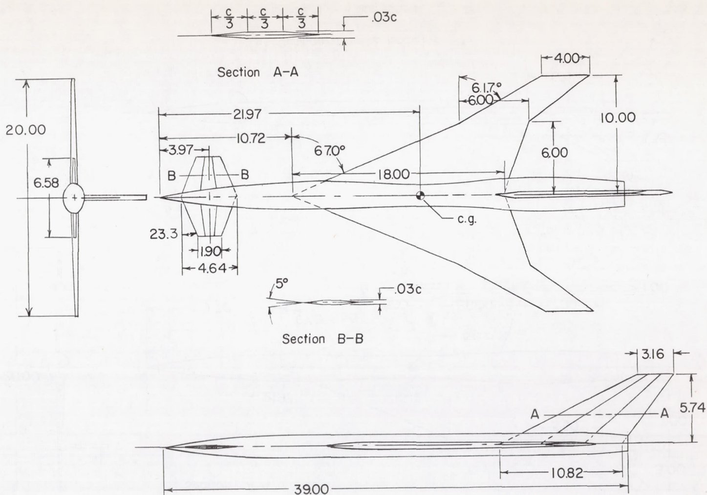
(a) Canard model.
