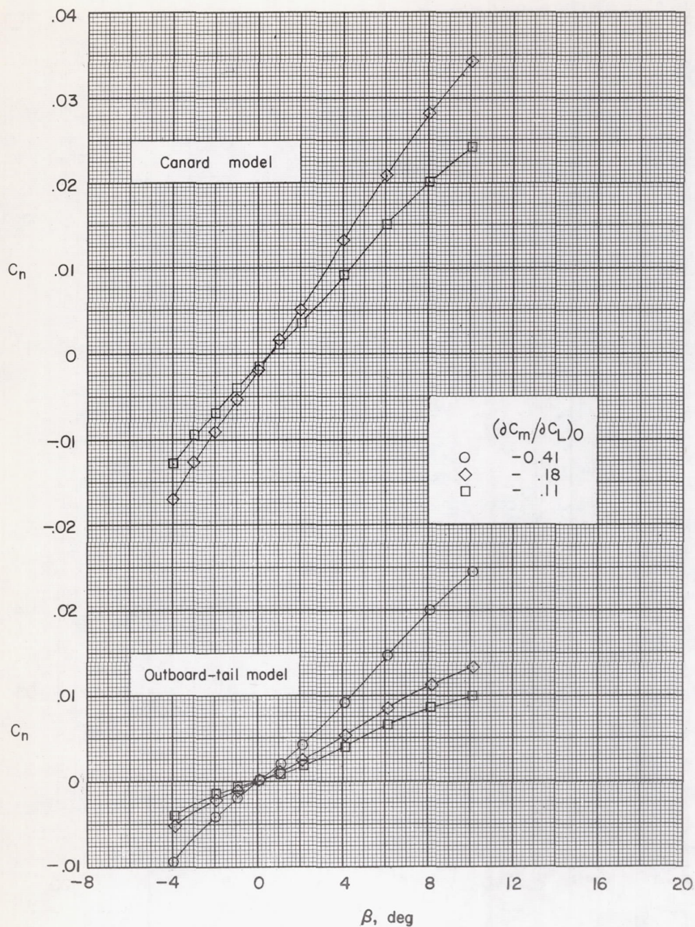
(b) Constant longitudinal stability.
