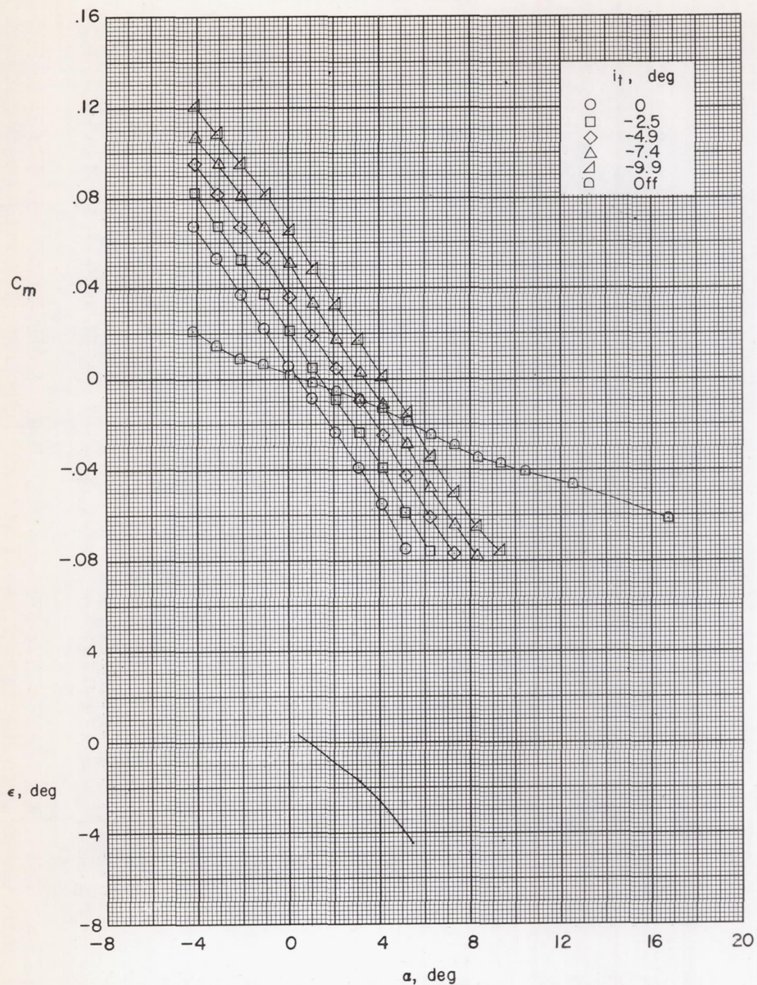
Figure 5.- Effective downwash characteristics for outboard-tail configuration.
