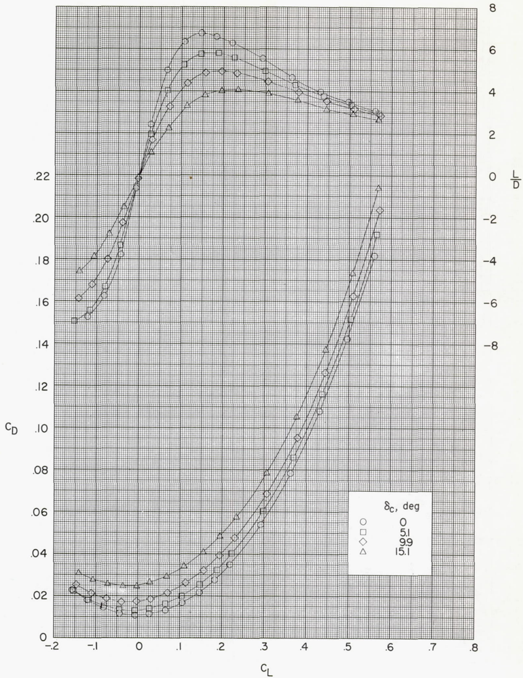
(c) Variation of L/D and C_D with C_L .
