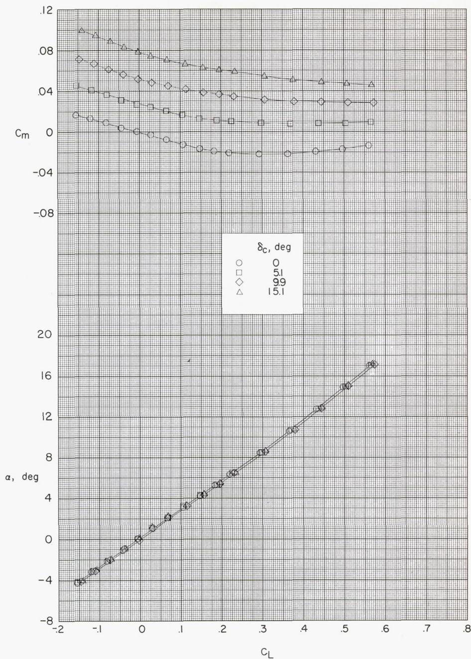
(a) Variation of C_m and \alpha with C_L . \partial C_m / \partial C_L = -0.11 .
