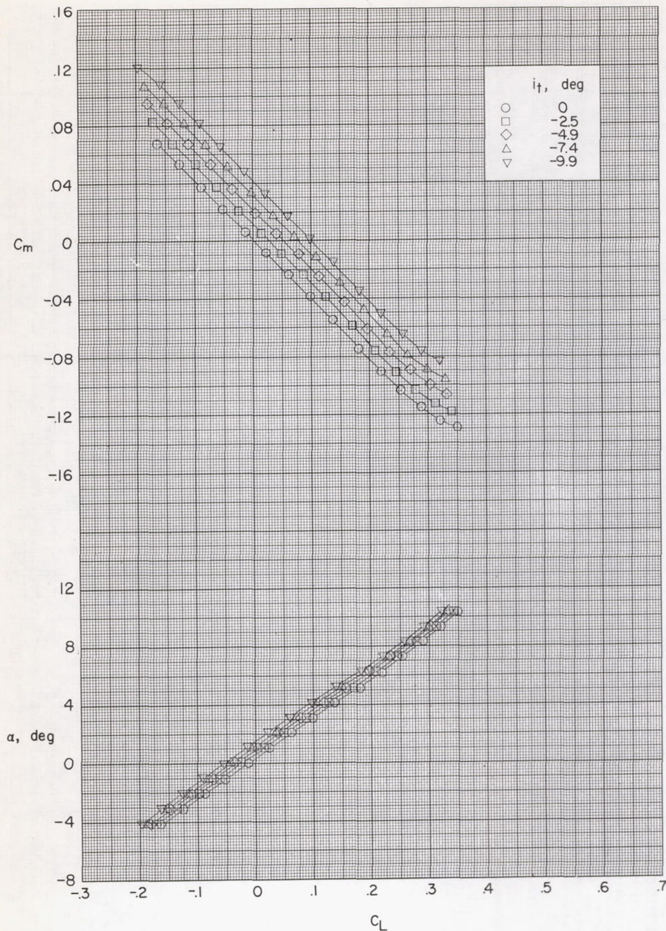
(a) Variation of C_m and \alpha with C_L . \partial C_m / \partial C_L = -0.41 .
