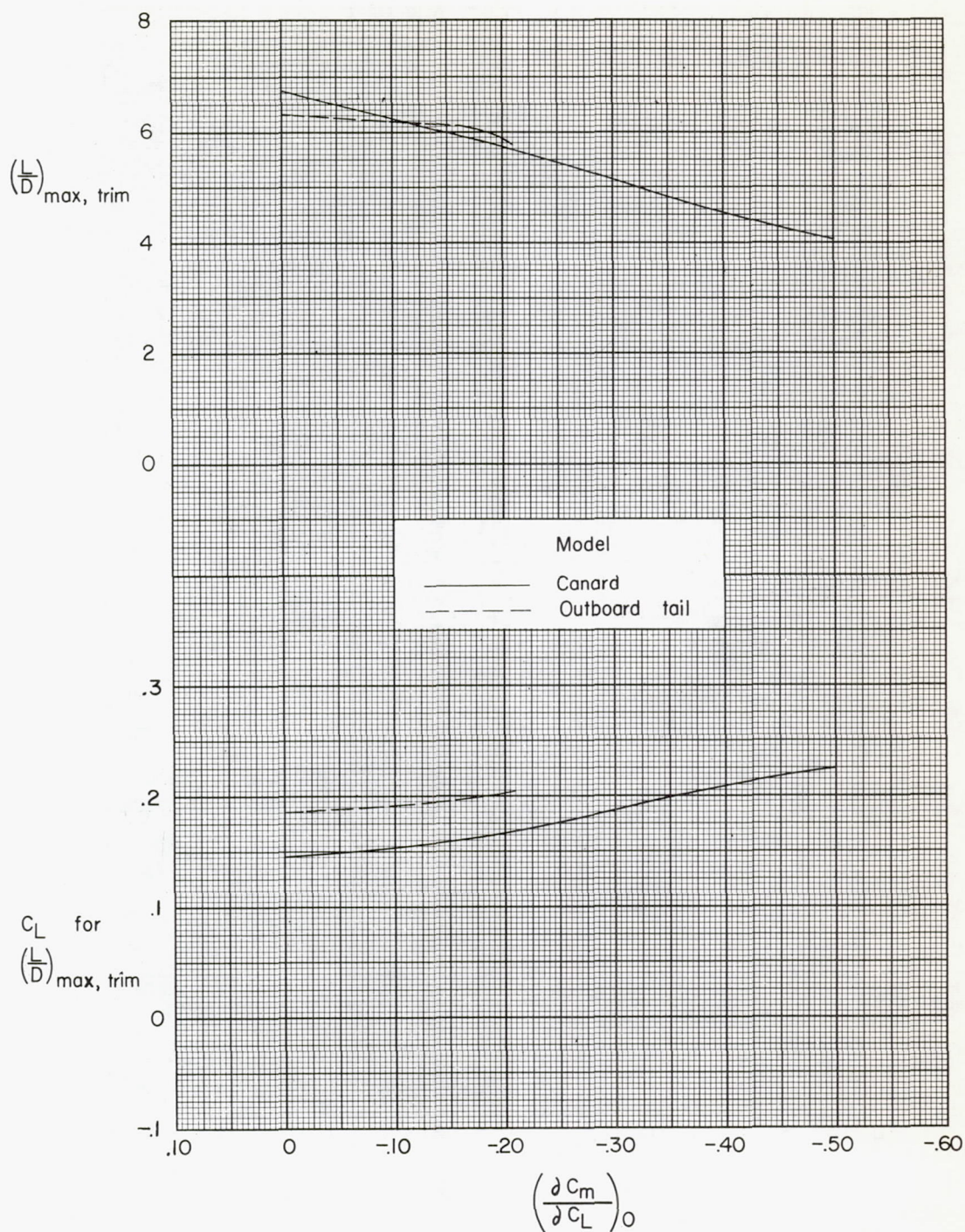
Figure 8.- Trimmed maximum L/D characteristics as a function of longitudinal stability.
