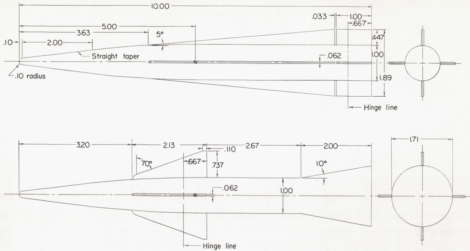
Figure 1.- Details of models. All linear dimensions are in calibers.
