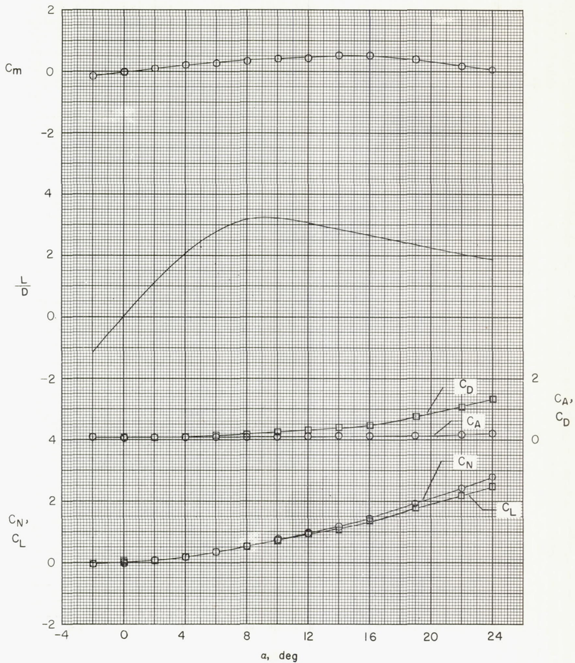
Figure 2.- Aerodynamic characteristics in pitch for body alone.
