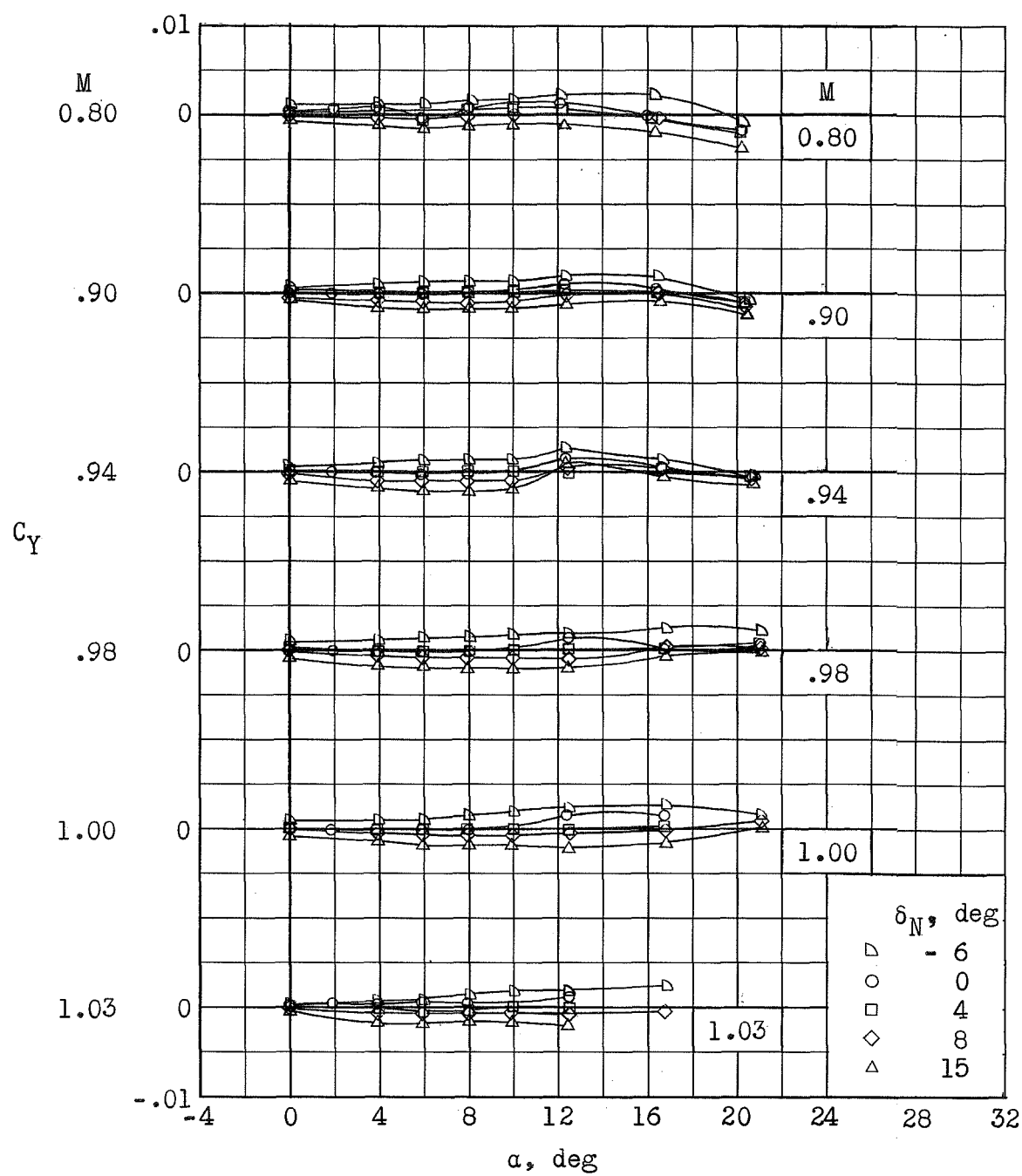
(e) C_Y against \alpha .
