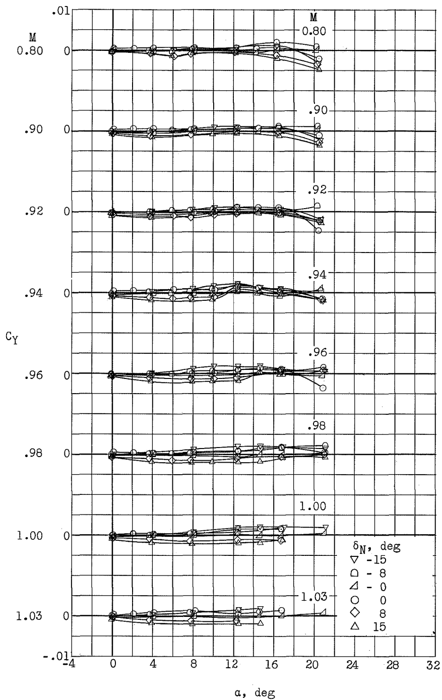
(e) C_L against \alpha .
