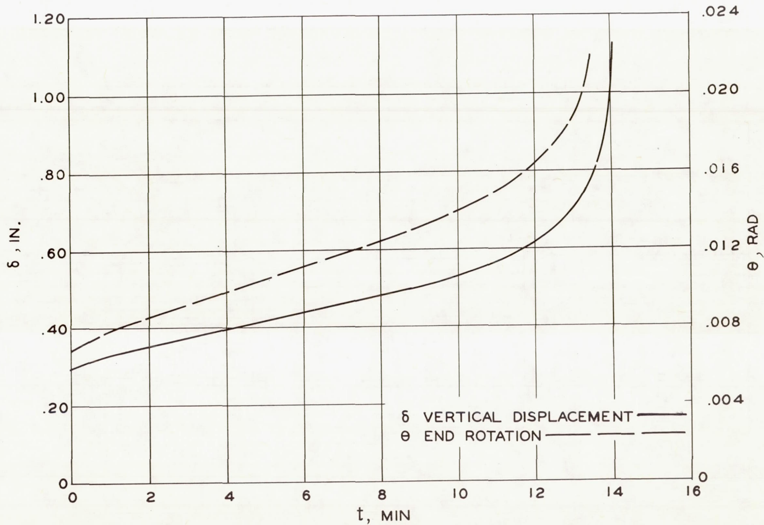
(a) Cylinder 17. Load, 580 pounds; bending moment, 62,700 inch-pounds; thickness, 0.051 inch.
