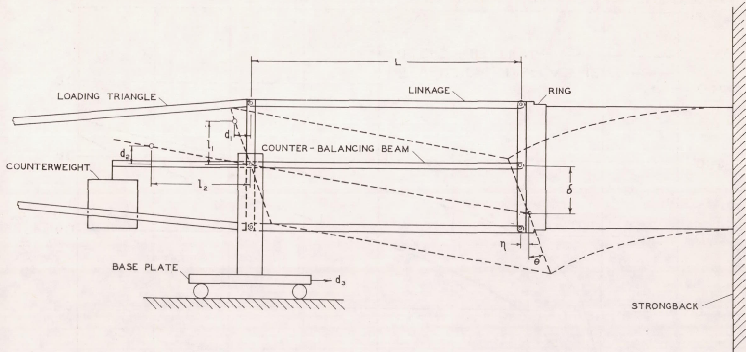
Figure 7.- Schematic drawing of equipment to measure deflections.
