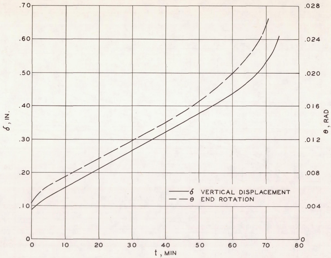
(b) Cylinder 29. Load, 380 pounds; bending moment, 41,000 inch-pounds; thickness, 0.040 inch.
