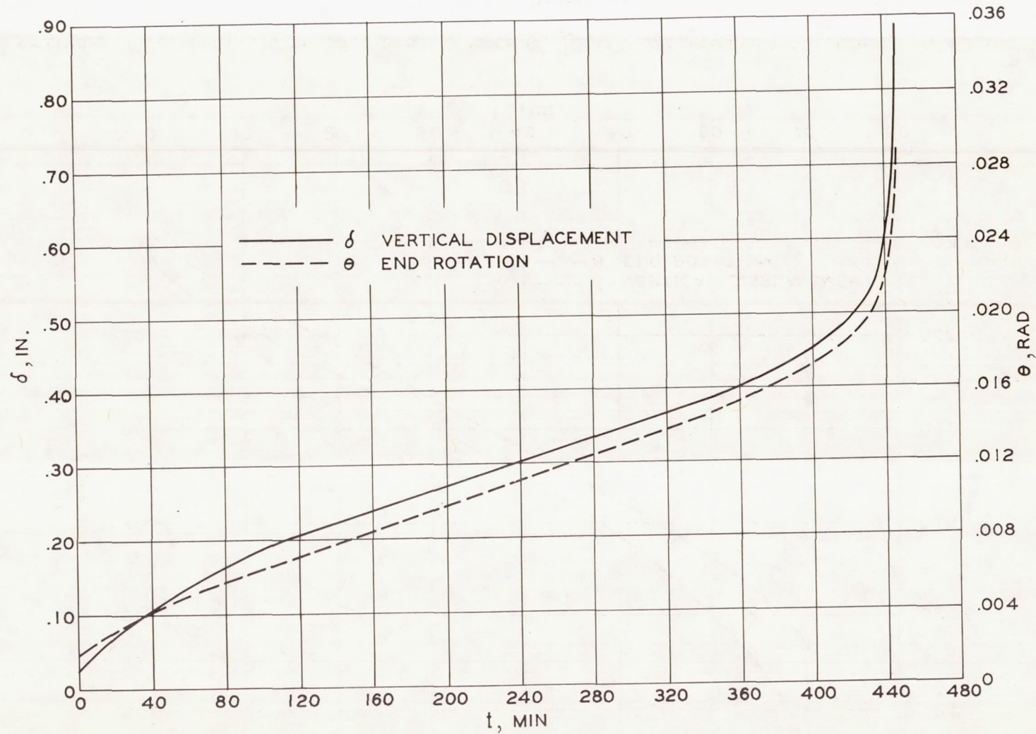
(c) Cylinder 42. Load, 190 pounds; bending moment, 20,500 inch-pounds; thickness, 0.032 inch.
