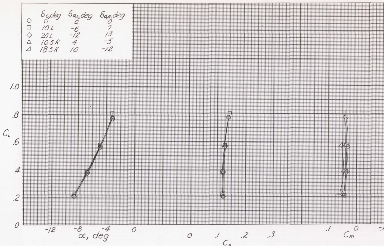
Figure 17.- Effect of aileron deflection on aerodynamic characteristics. Original configuration; normal inflation pressure (7 lb/sq in.); canopy installed; wind velocity approximately 64 mph ( q_{av} = 10 lb/sq ft).
