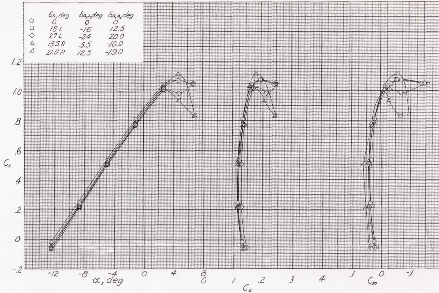
Figure 16.- Effect of aileron deflection on aerodynamic characteristics of the Goodyear Inflatoplane. Original configuration; normal inflation pressure (7 lb/sq in.); canopy installed; wind velocity approximately 41 mph ( q_{av} = 4 lb/sq ft).
