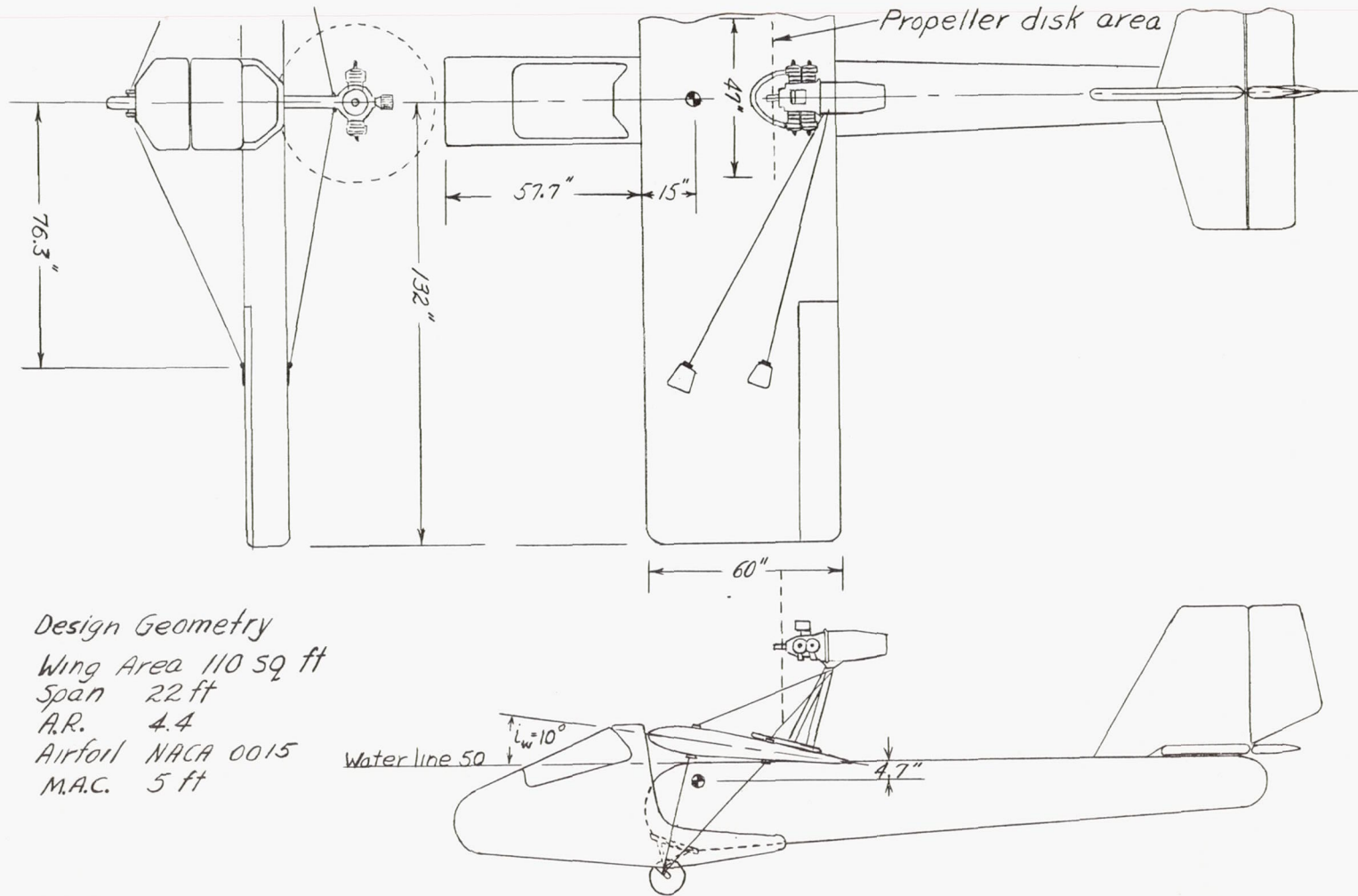
Figure 1.- Geometric characteristics of the Goodyear Inflatoplane.
