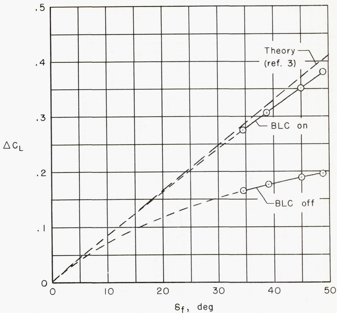
Figure 10.- Variation of flap lift increment with flap angle; \alpha = 12^\circ ; engine speed = 92 percent.
