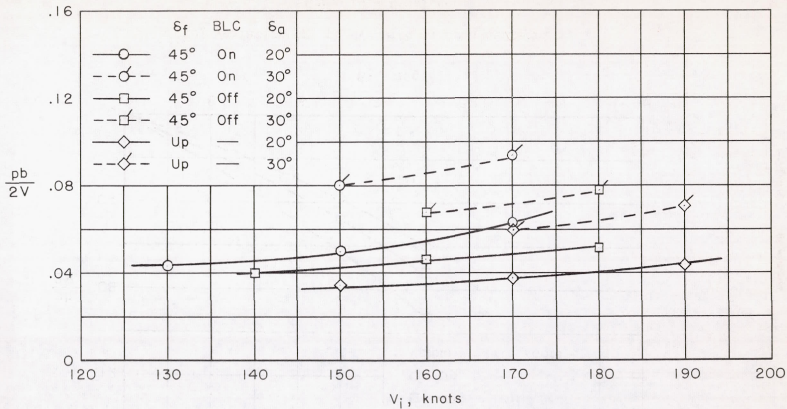
(a) Variation of \frac{pb}{2V} with airspeed.
