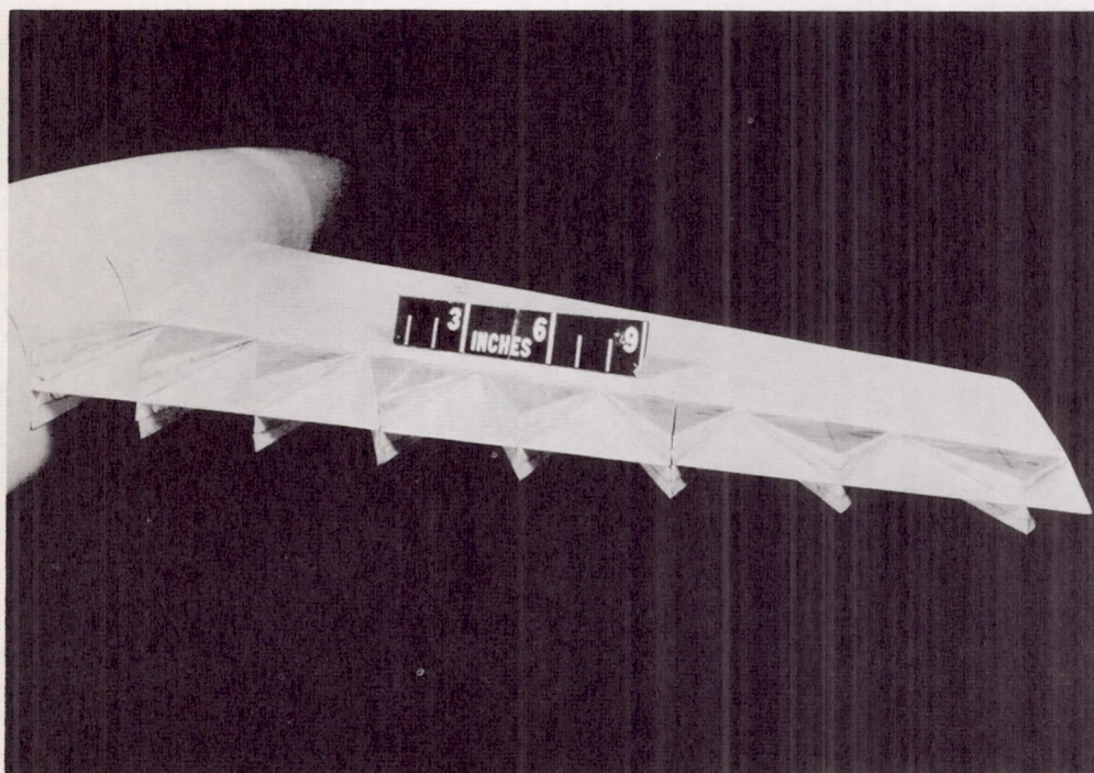
(b) Short-chord wedges; ramp angle = 3\frac{1}{2}^\circ .
