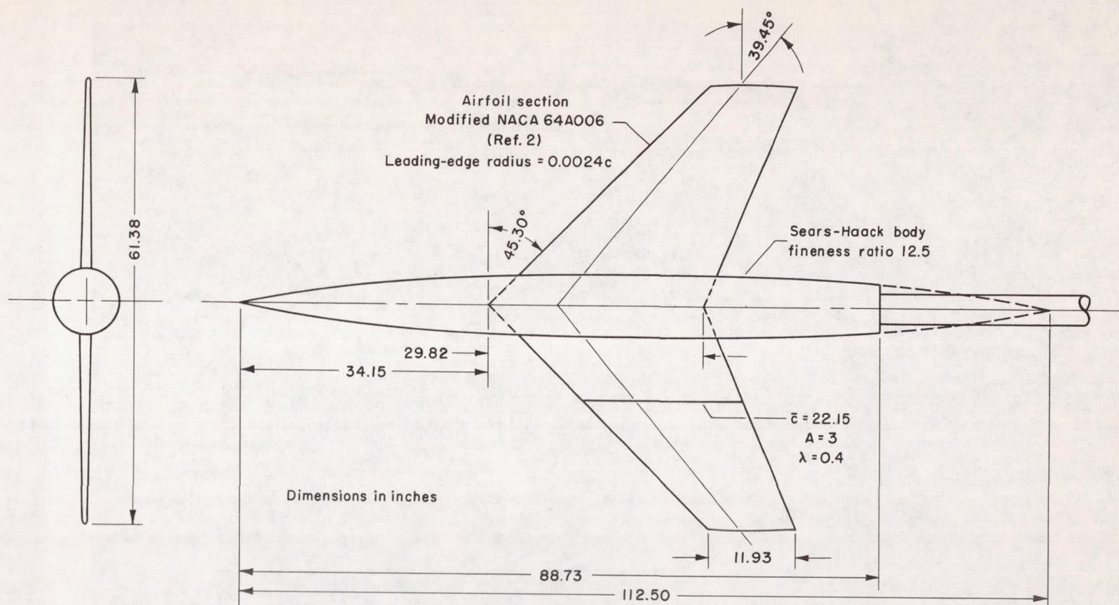
Figure 1.- Sketch of basic wing-body combination.
