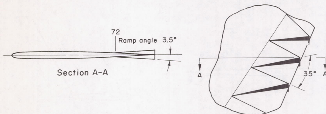
(b) Short-chord wedges; ramp angle = 3.5^\circ
