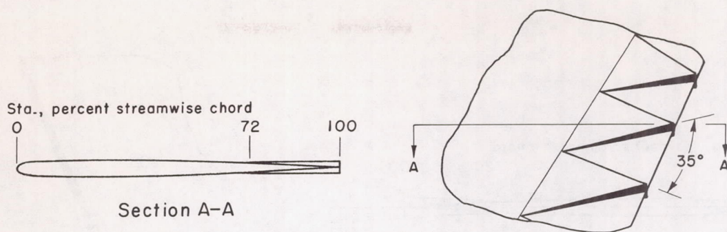
(a) Short-chord wedges; ramp angle = 0^\circ .
