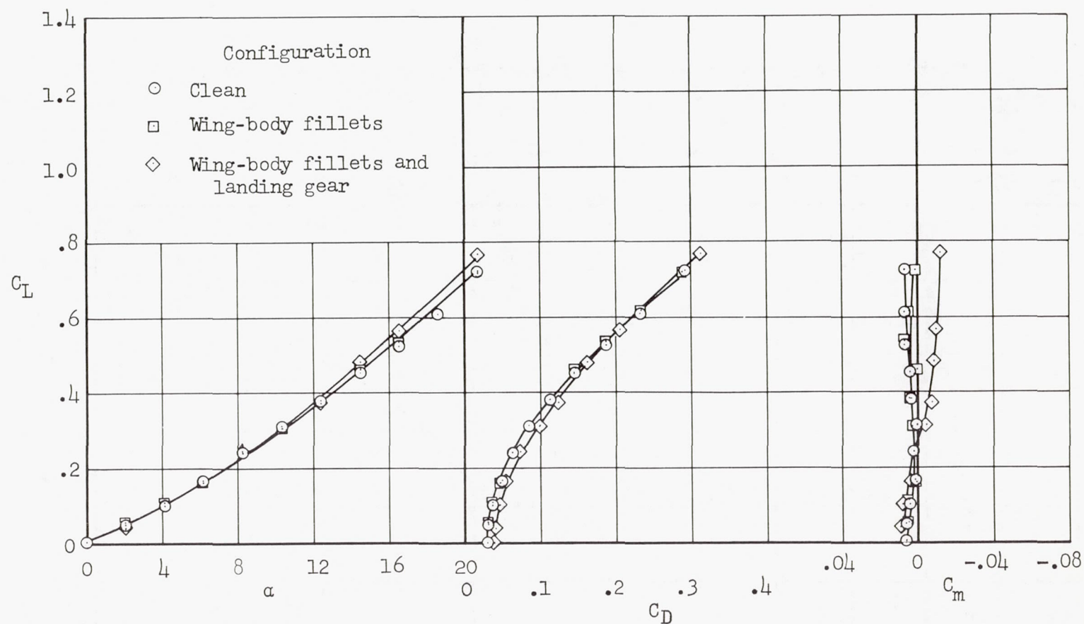
Figure 6.- Effects of adding wing-body fillets and landing gear on longitudinal stability; plan form C with 3/4-power fuselage and afterbody, \delta_t = 45^\circ .
