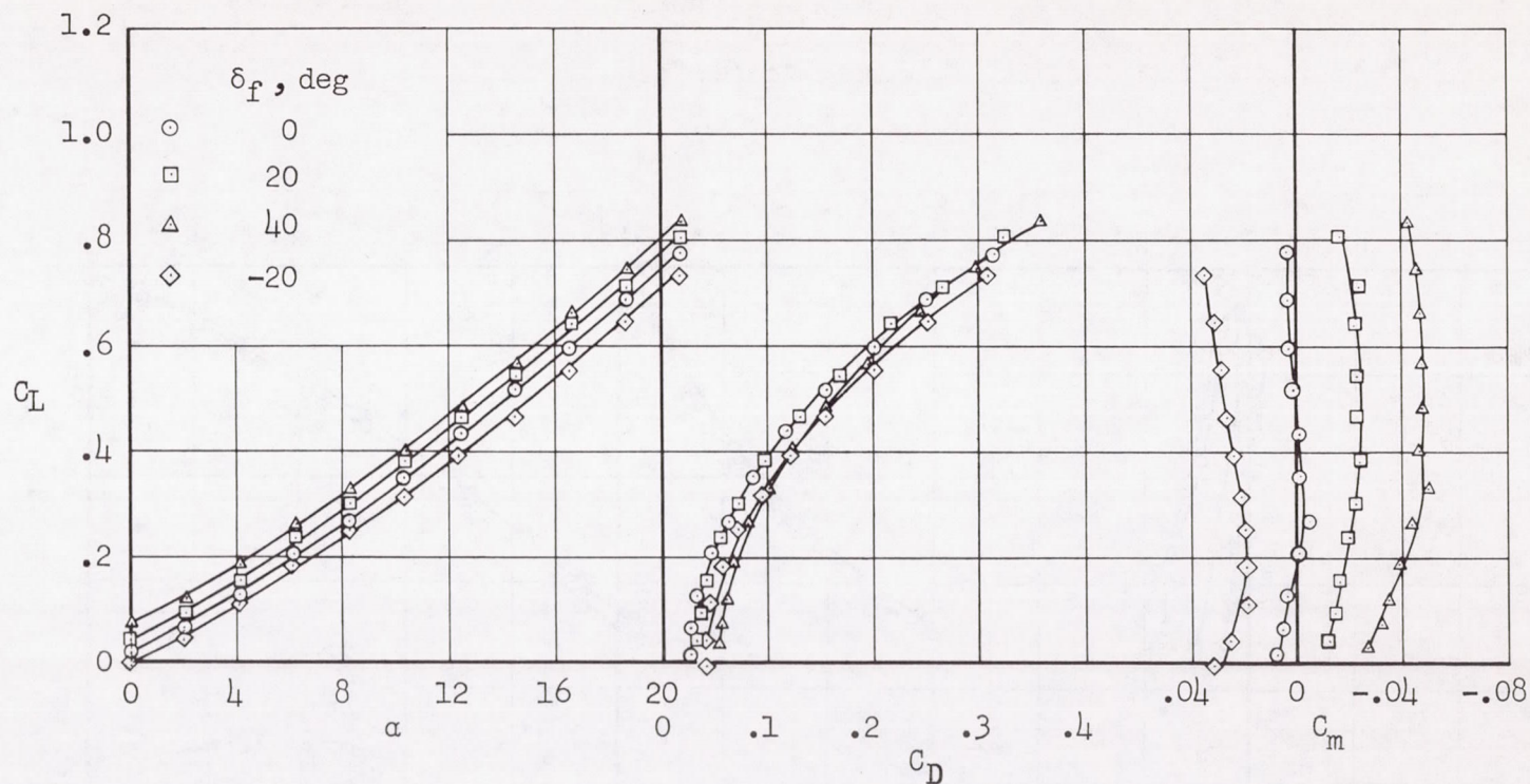
Figure 7.- Effects of flap deflection on the longitudinal characteristics of plan form C.
