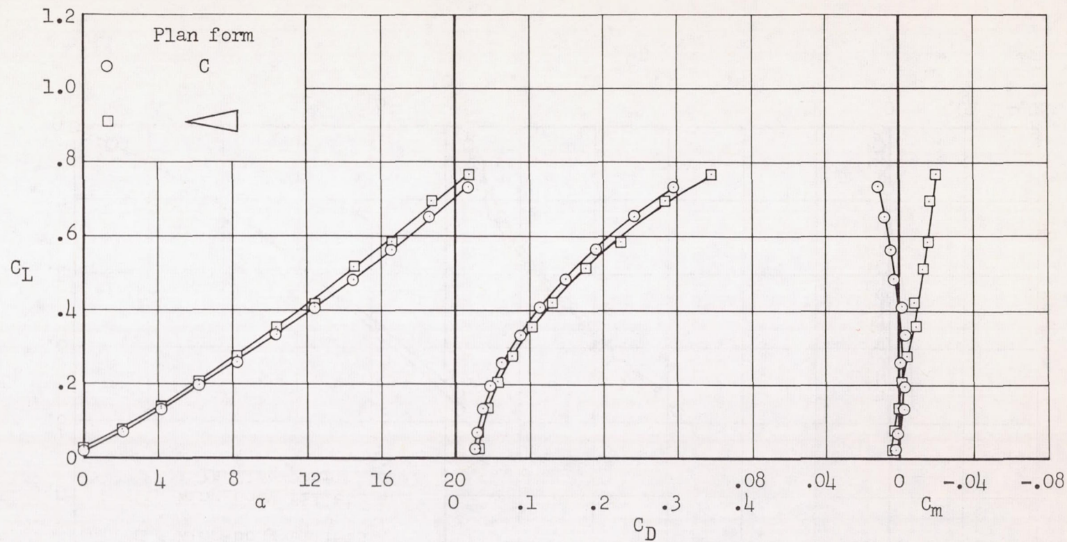
Figure 5.- Effect of changing wing plan form to a pure delta wing.
