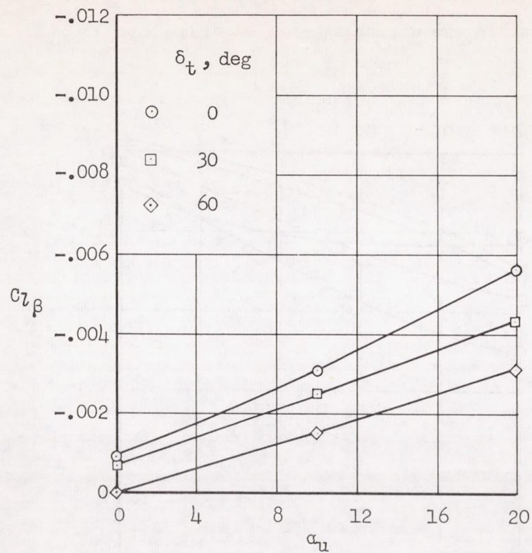
Figure 11.- Variation of C_{l\beta} and C_{n\beta} with \alpha_u and \delta_t ; plan form A.
