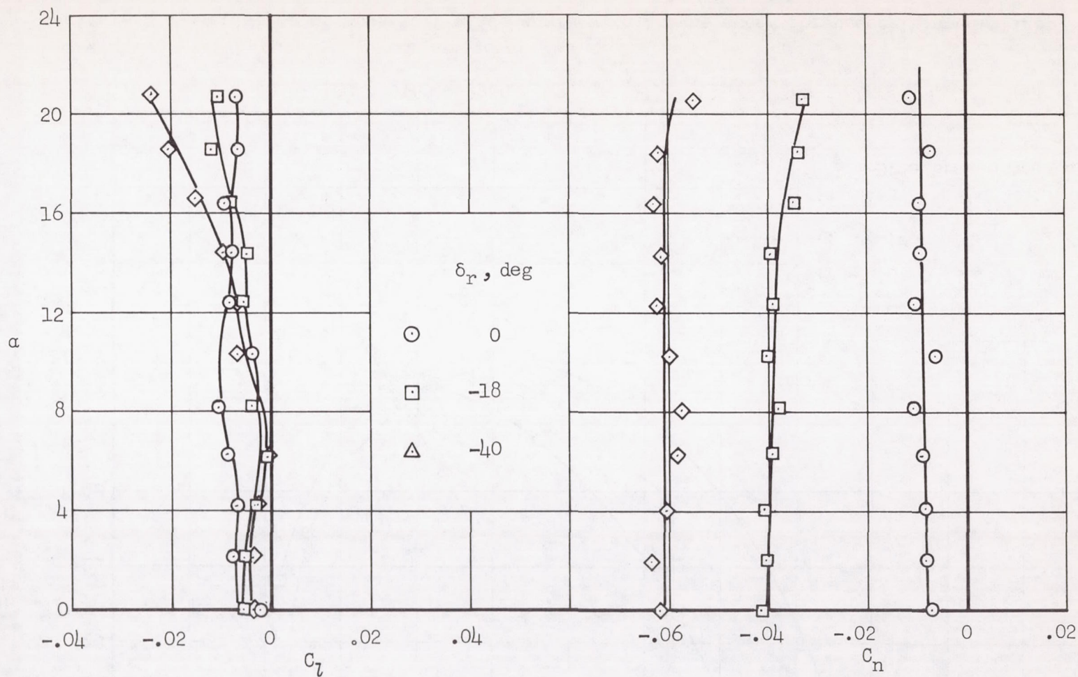
Figure 14.- Variation of C_L and C_N with \alpha_u and \delta_r ; plan form C with twin vertical fins.
