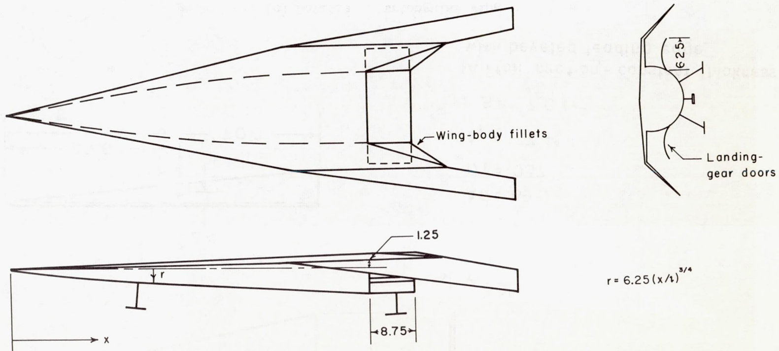
(d) Landing approach configuration (with 3/4-power fuselage and afterbody).
