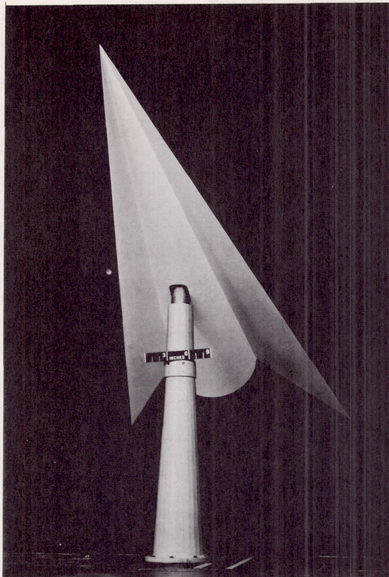
Figure 2.- Model of plan form A installed in Ames 7- by 10-foot wind tunnel.
