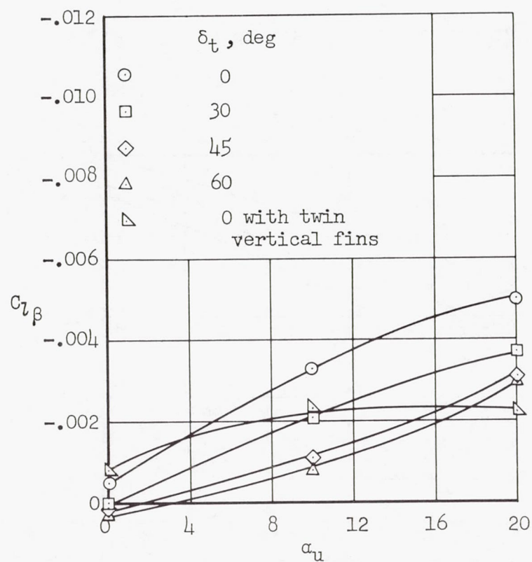
Figure 12.- Variation of C_{l\beta} and C_{n\beta} with \alpha_u and \delta_t ; plan form C.
