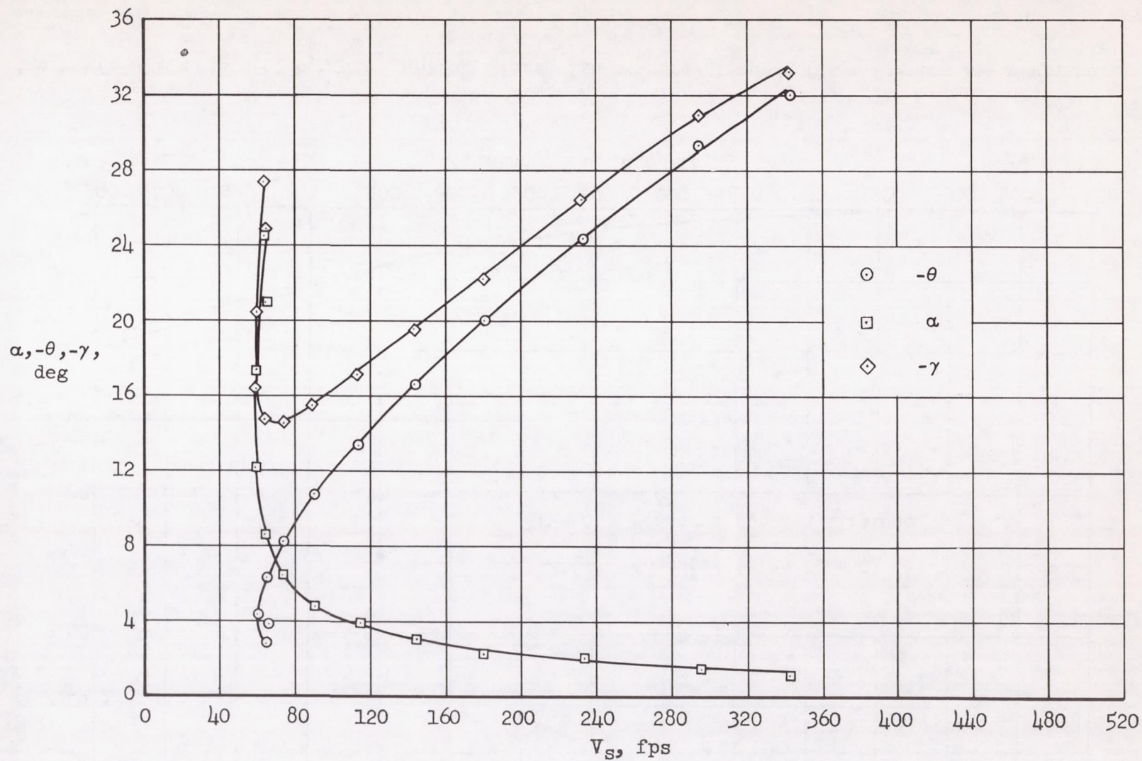
Figure 16.- Variation of angle of attack, glide angle, and attitude angle with sinking speed for unaccelerated flight; plan form C, W/S = 20 psf.
