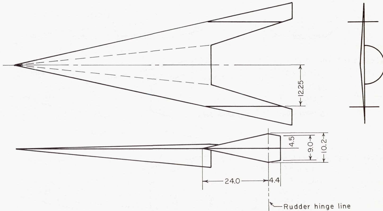
(b) Vertical-fin configuration.
