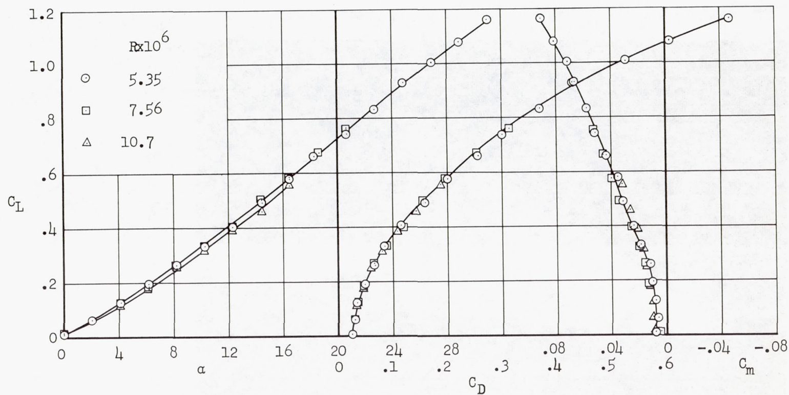
Figure 3.- The effects of Reynolds number on the longitudinal characteristics of plan form A; \delta_t = 30^\circ .
