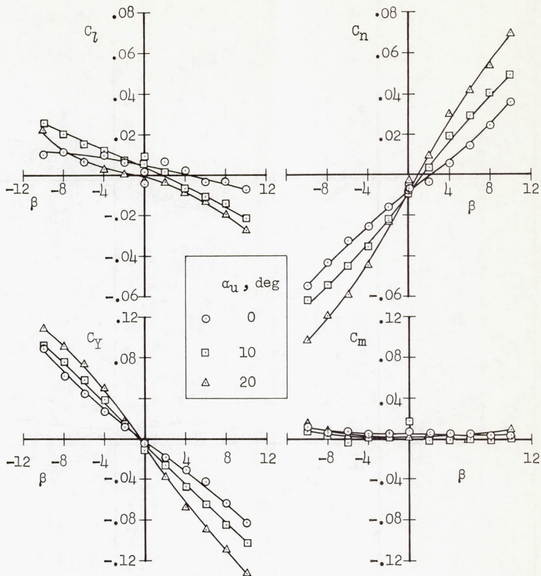
Figure 10.- Lateral characteristics of plan form C with twin vertical fins; \delta_t = 0^\circ .
