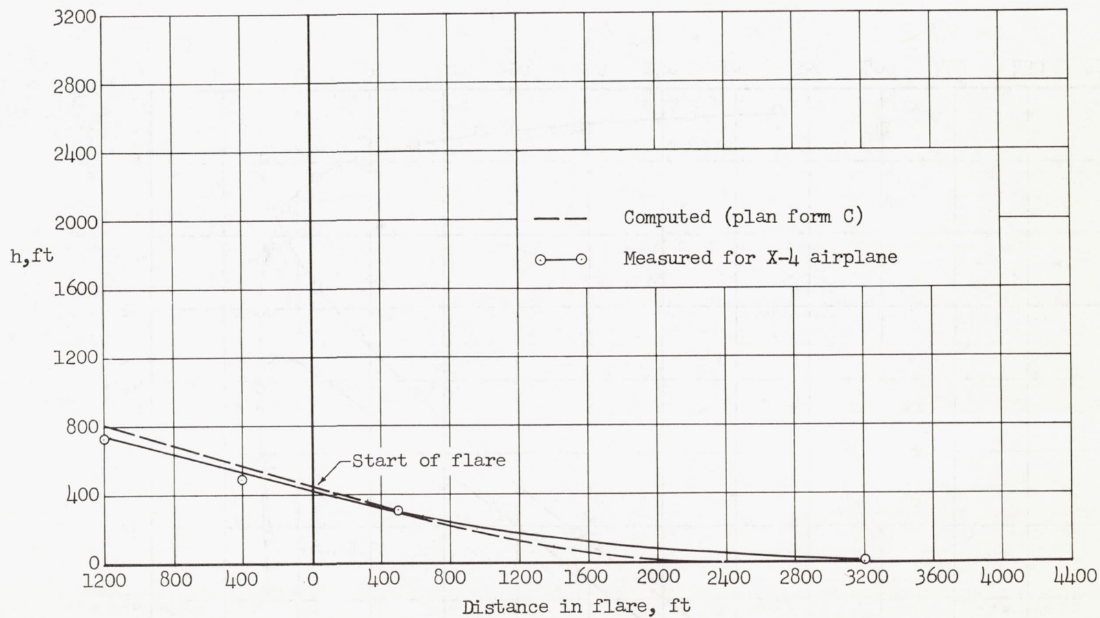
Figure 17.- Comparison of computed landing flare with measured landing flare for the X-4 airplane.
