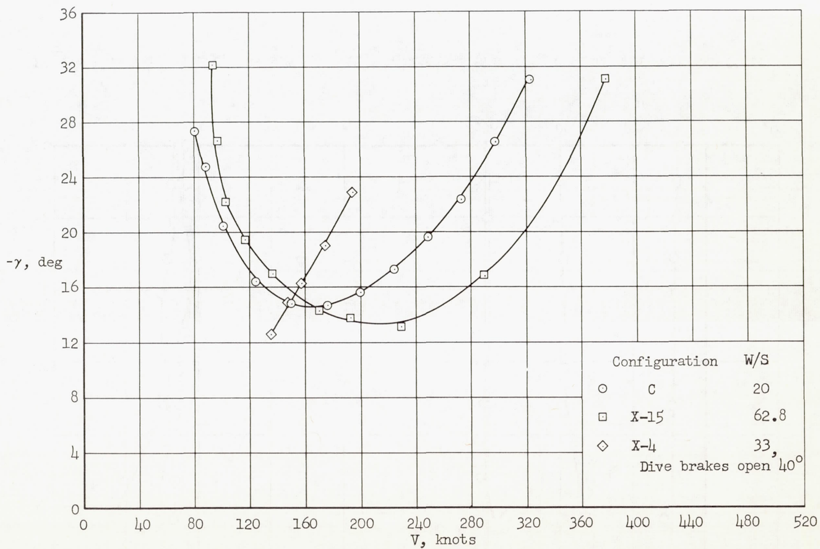
Figure 15.- Variation of power-off glide angle with flight speed for unaccelerated flight.
