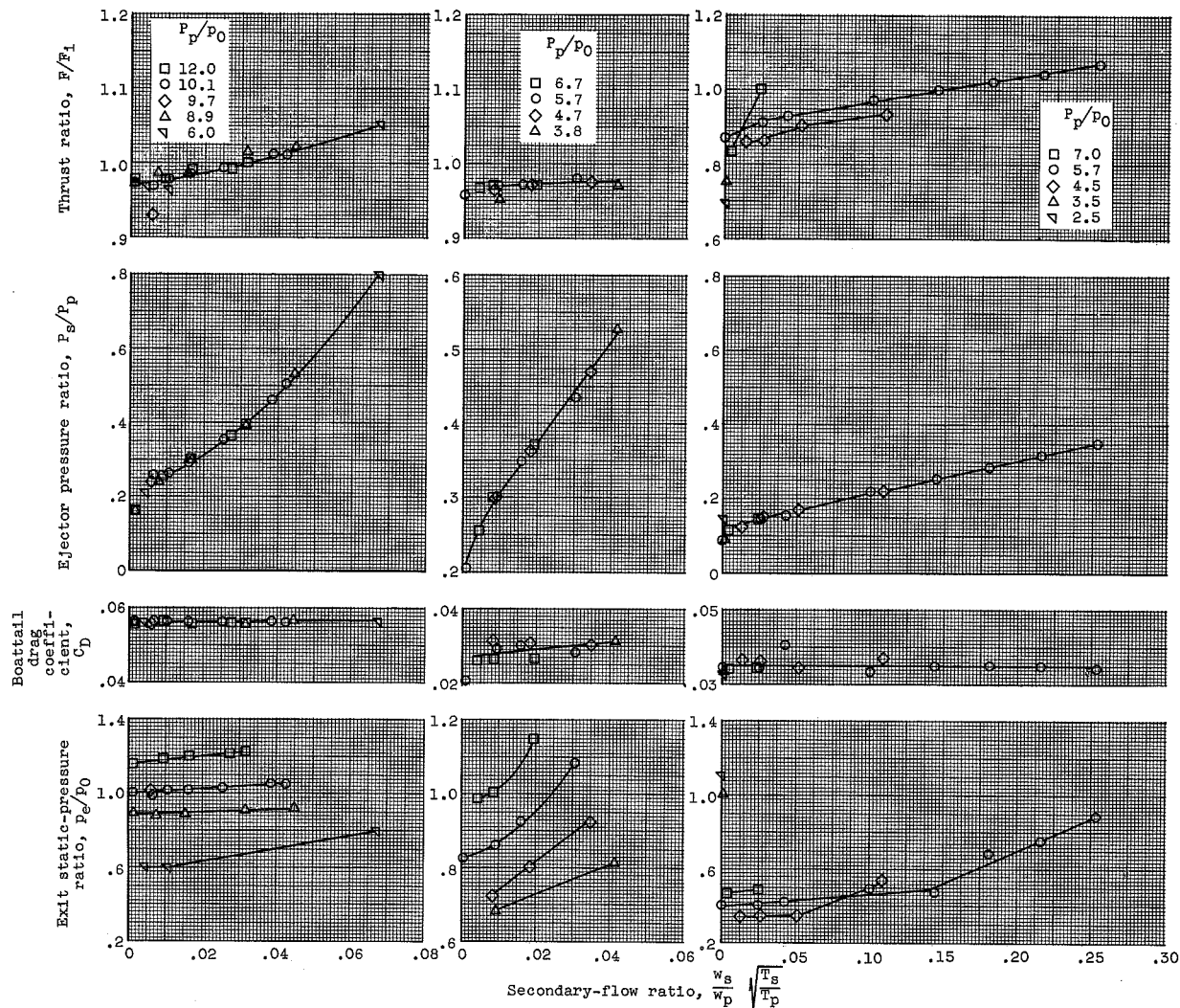
(a) Afterburning; Mach number, 2.0; d_e/d_p , 1.4.
