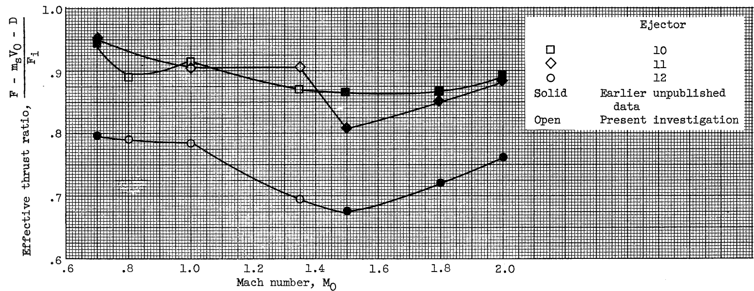
Figure 38. - Effect of Mach number on performance of fixed ejectors 10 to 12. Secondary-flow ratio, 0.02.
