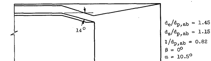
Figure 1. - Concluded. Ejector geometries.
