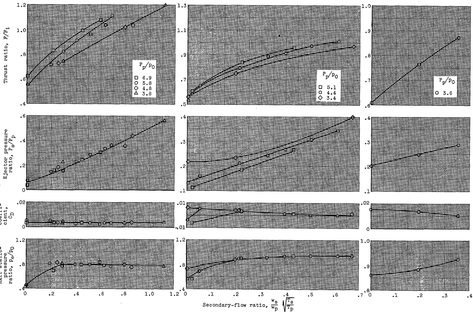
(a) No afterburning; Mach number, 1.35.
