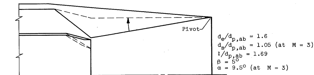
(h) Ejector 9: d_{p,nb}/d_{p,ab} = 0.75 ; d_m/d_{p,ab} = 2.0 .
