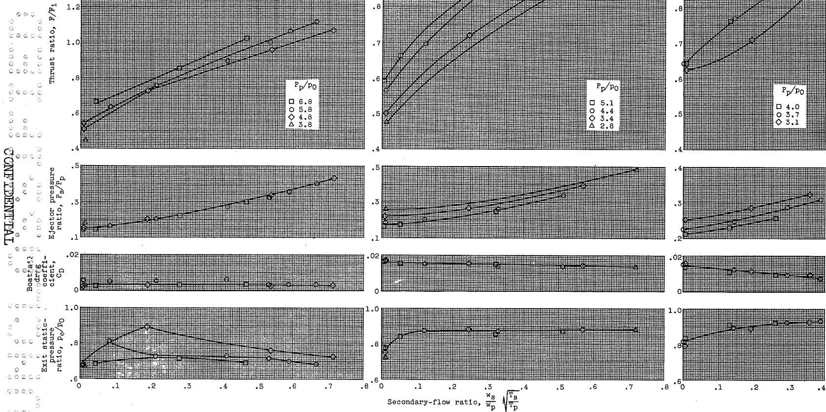
Figure 14. - Performance of ejector 1 with spoilers and air injection.
