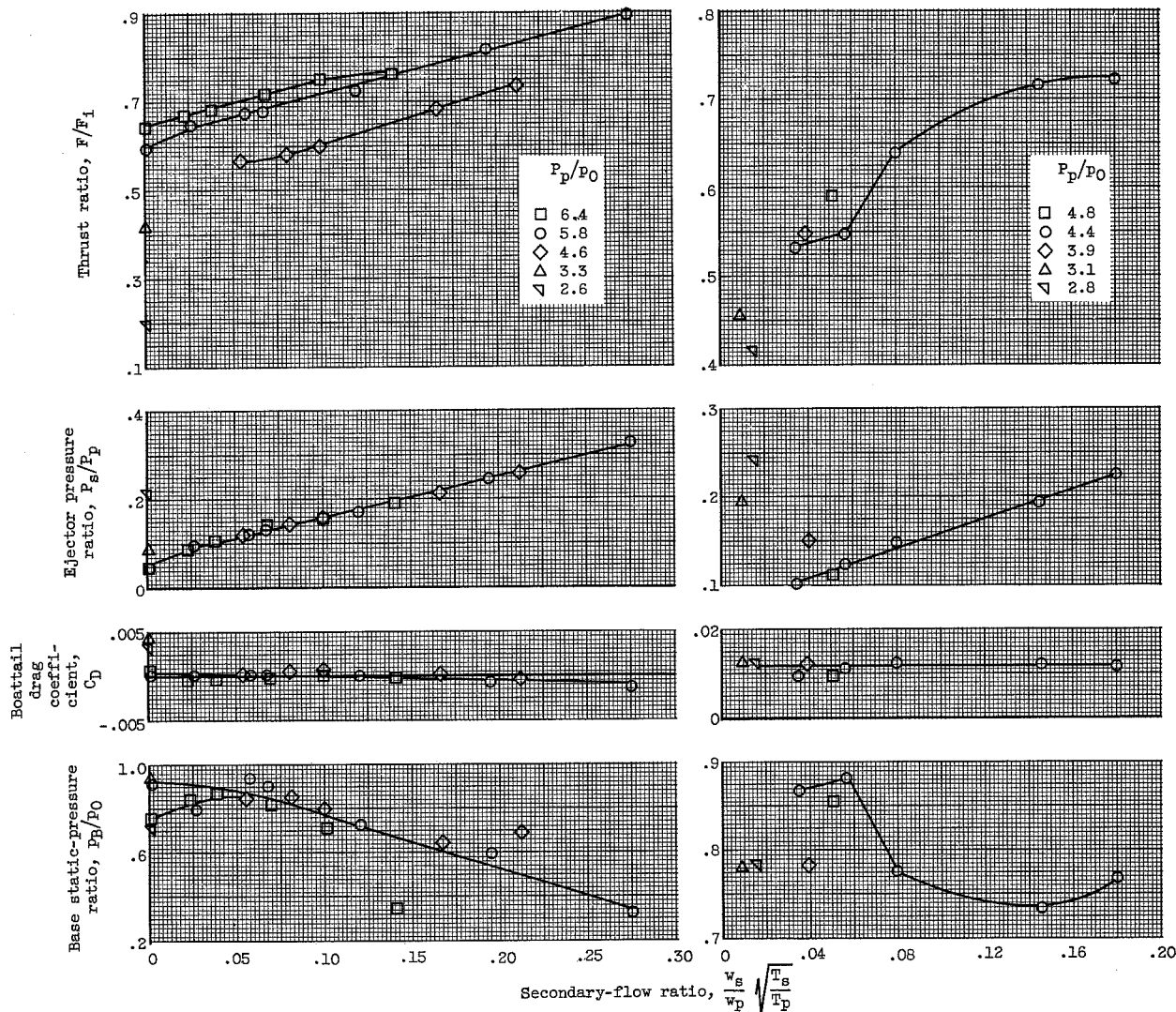
(b) No afterburning; Mach number, 1.0.
