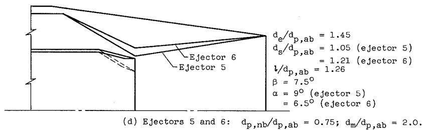
Figure 1. - Ejector geometries.
