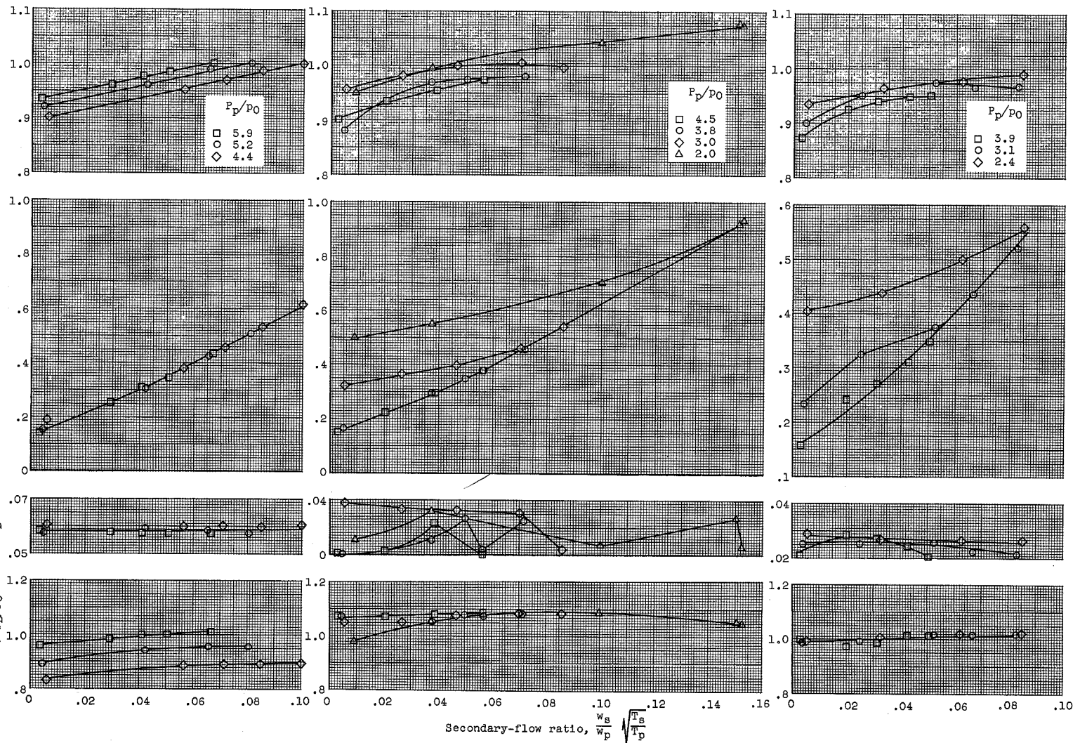
(a) Mach number, 1.35.
