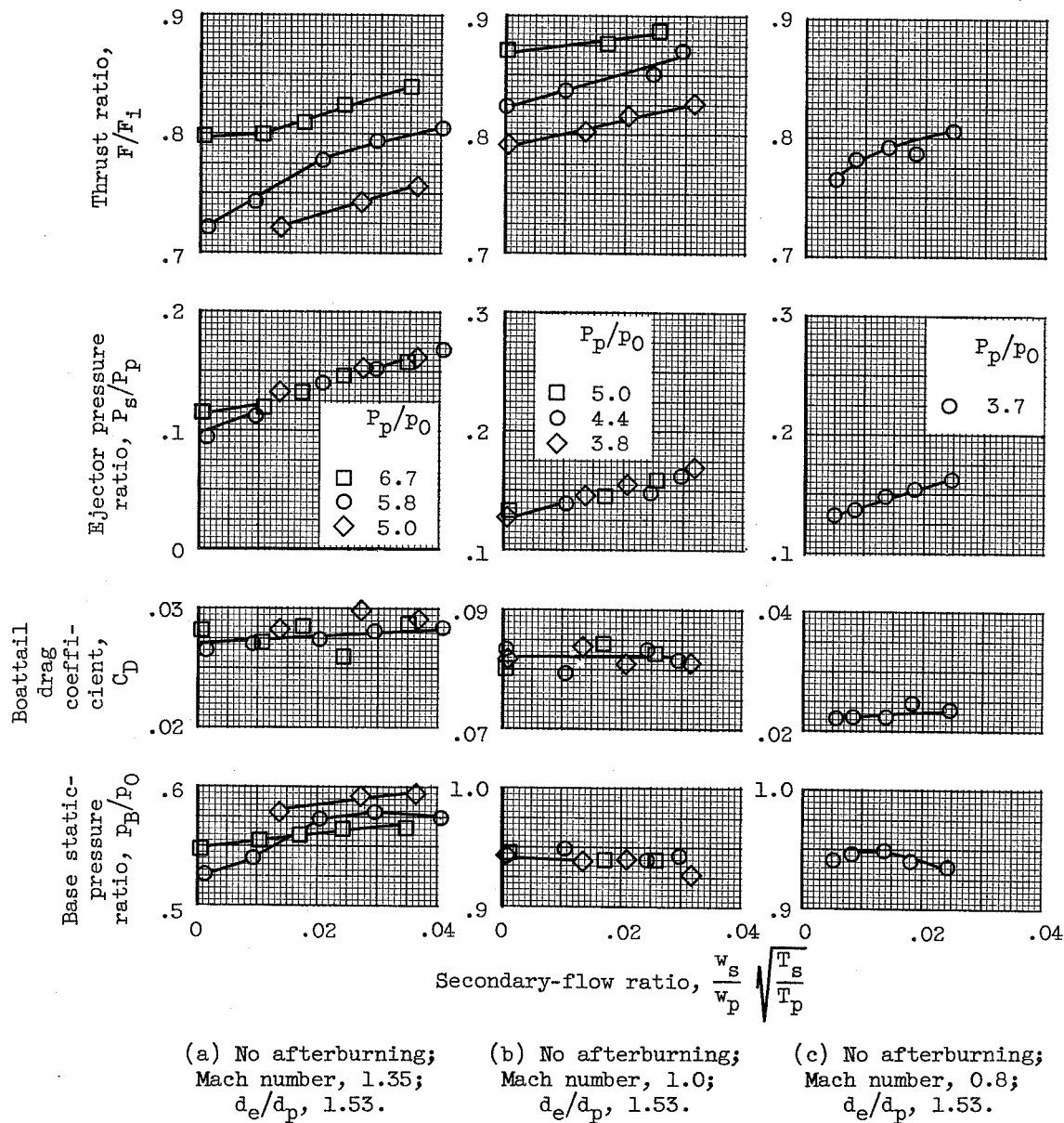
Figure 17. - Performance of ejector 8 without base flow.
