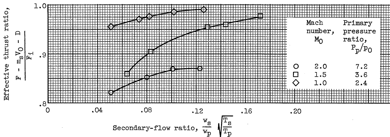
Figure 40. - Effect of secondary flow on performance of ejector 13.
