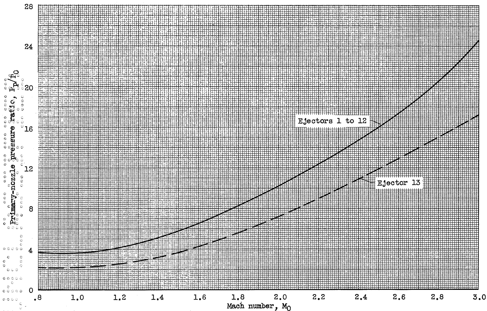
Figure 23. - Schedule of primary-nozzle pressure ratio.
