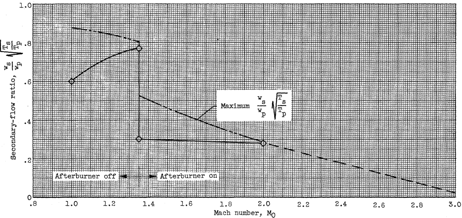
Figure 36. - Performance of variable-geometry ejector 9.
