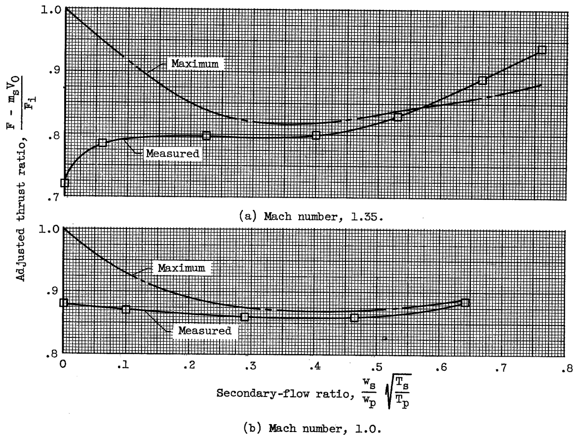
Figure 5. - Comparison of measured and maximum thrust ratios for ejector 8 with no afterburning.
