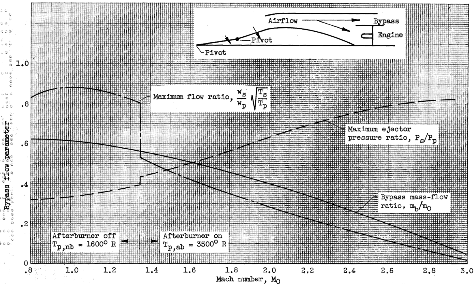
Figure 27. - Schedule of inlet bypass air available for ejector.
