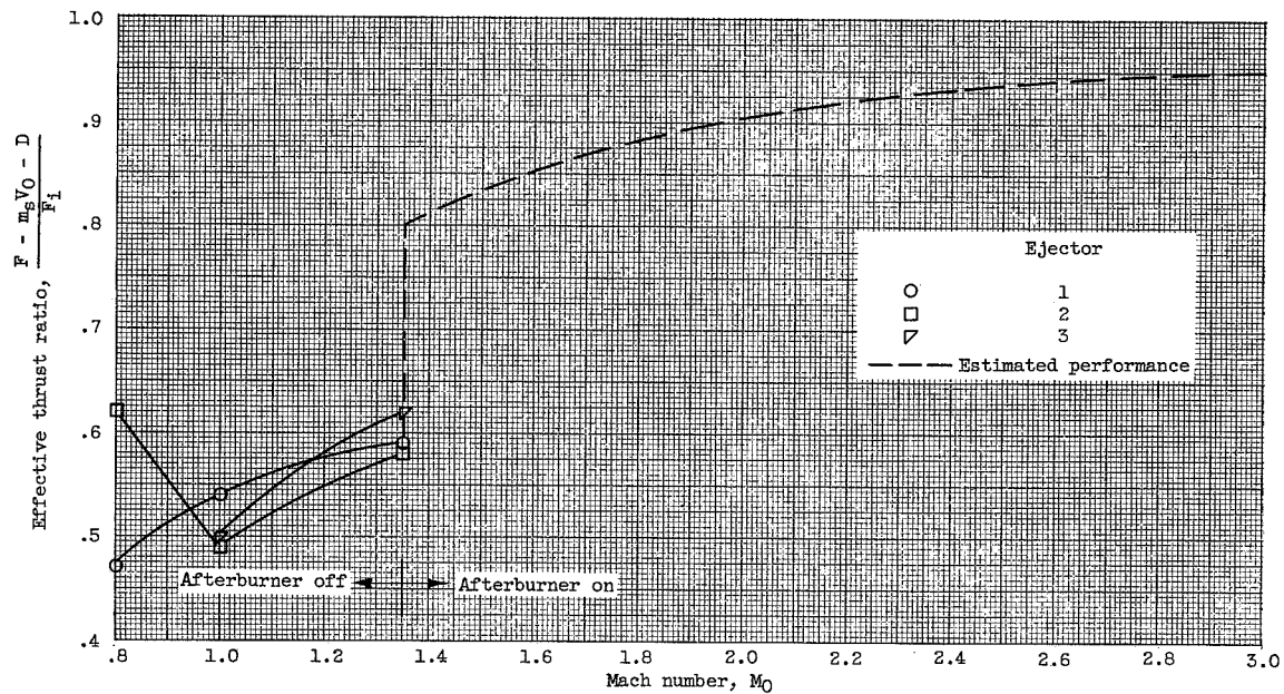
Figure 24. - Effect of flight Mach number on fixed ejector performance. Secondary-flow ratio, 0.02.
