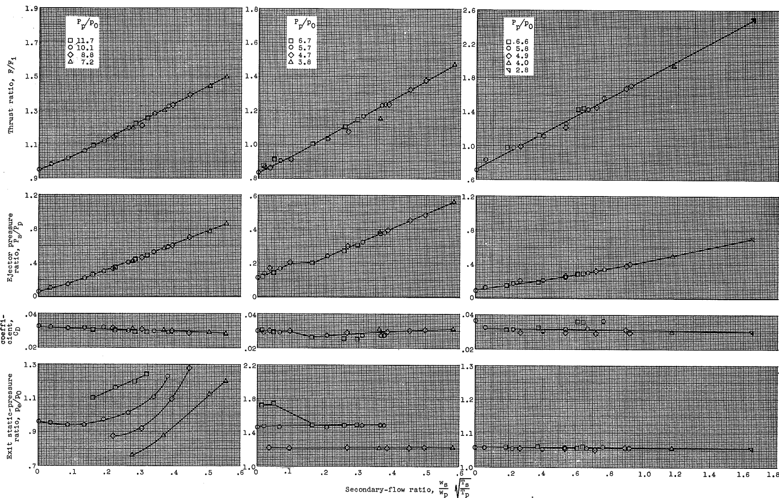
Figure 16. - Performance of ejector 8 with base flow.
