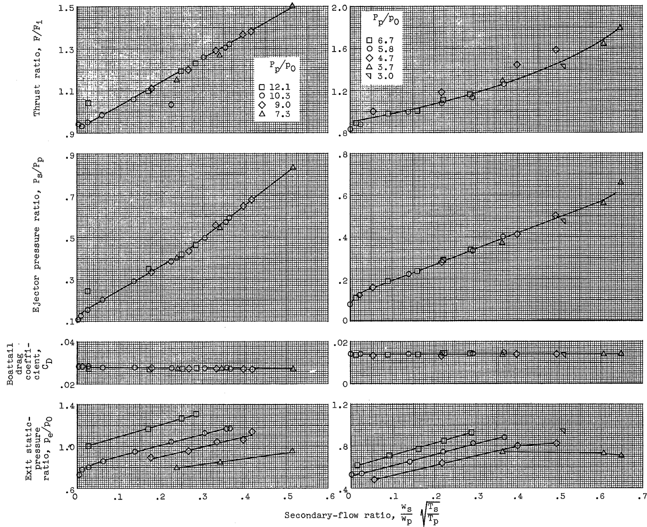
Figure 18. - Performance of ejector 9.
