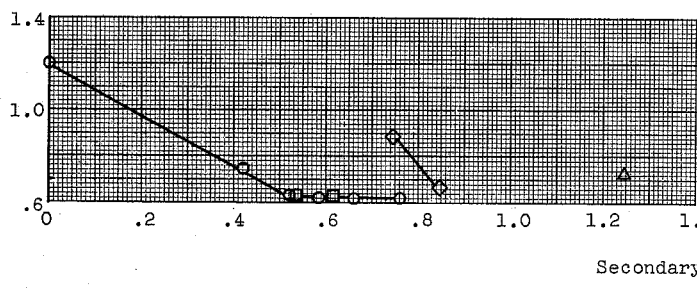
(c) No afterburning; Mach number, 1.35; d_s/d_p , 1.94.
