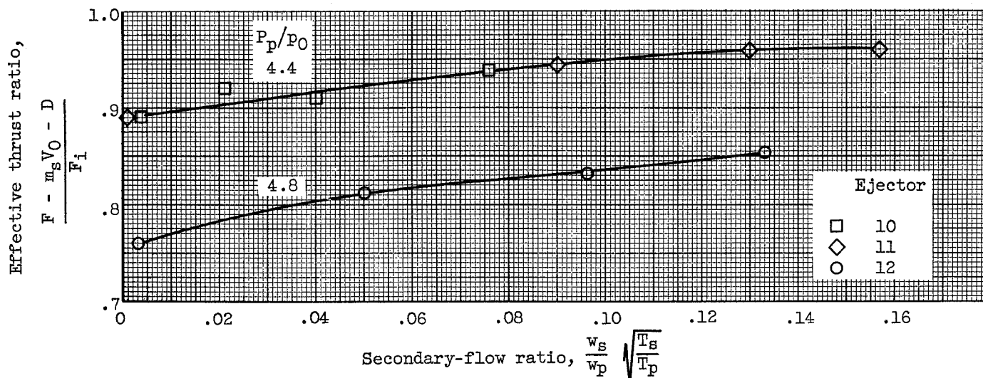
Figure 39. - Effect of secondary flow on performance of fixed ejectors 10 to 12 at Mach number 1.0.
