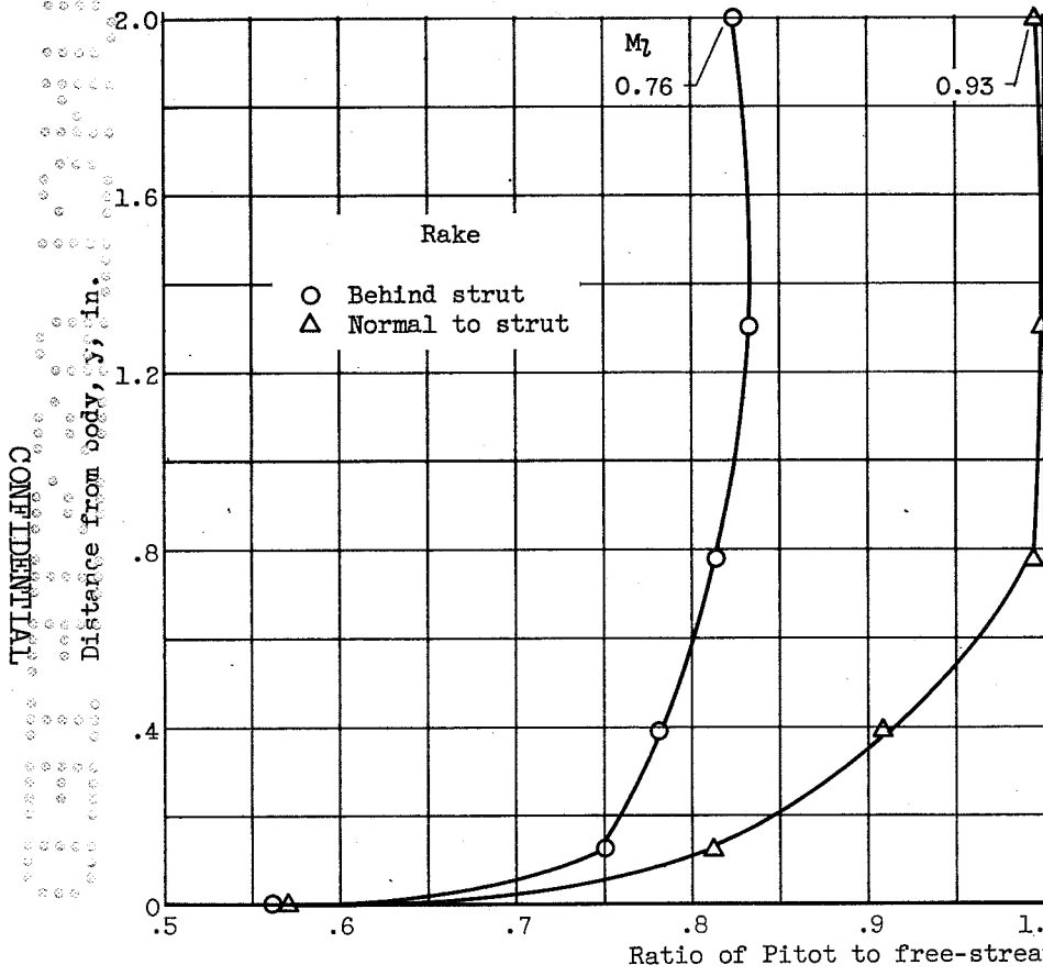
(c) Mach number, 1.0.
