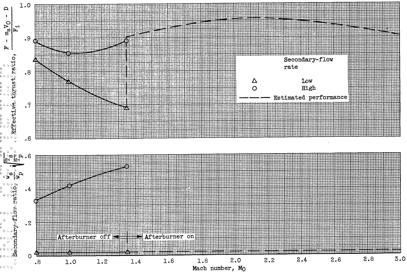
Figure 28. - Effect of secondary flow on performance of fixed ejector 6.
