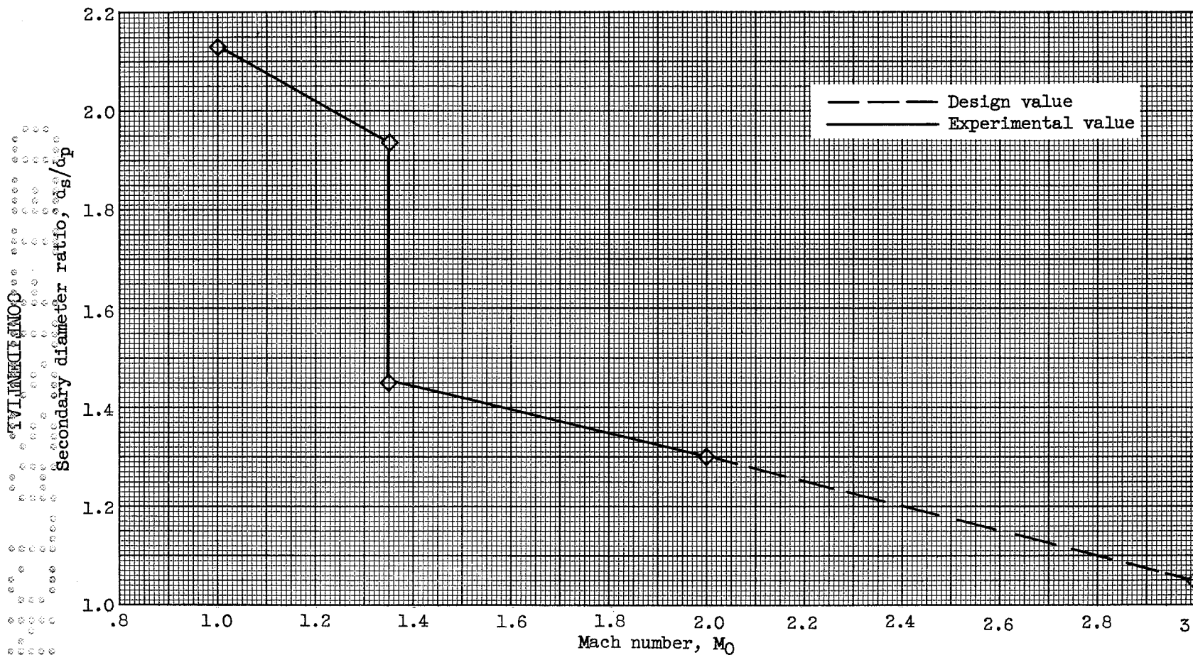
Figure 35. - Secondary-diameter-ratio schedule of ejector 9.
