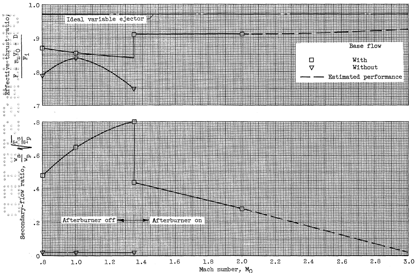
Figure 34. - Performance of variable-geometry ejector 8.
