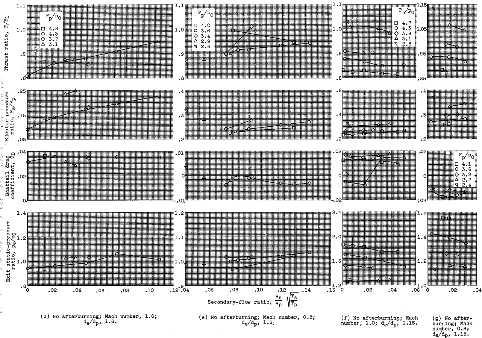
Figure 15. - Concluded. Performance of ejector 7.
