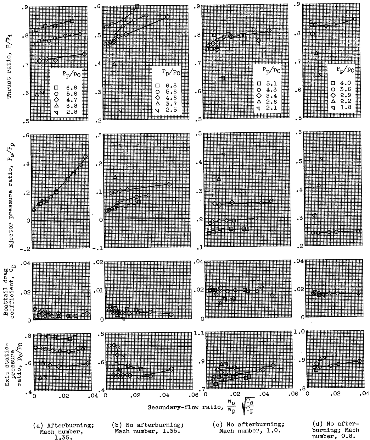
Figure 9. - Performance of ejector 4.
