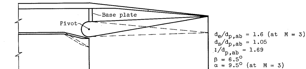
(g) Ejector 8: d_{p,nb}/d_{p,ab} = 0.75 ; d_m/d_{p,ab} = 2.0 .
