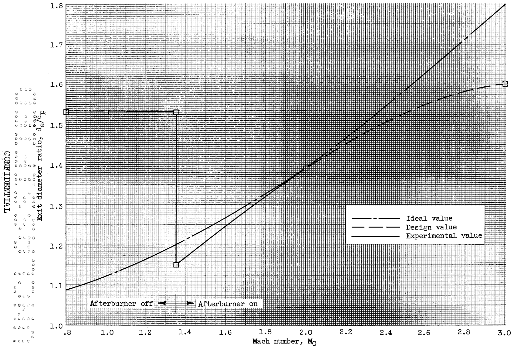
Figure 33. - Expansion-ratio schedule of ejector 8.
