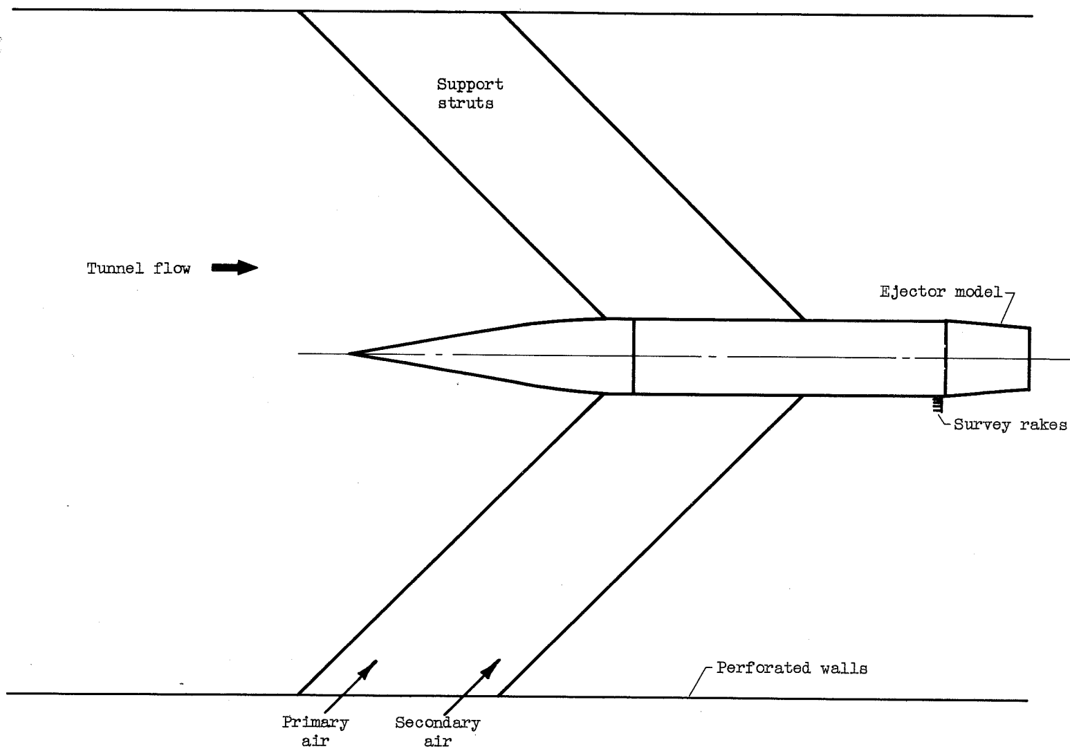
Figure 2. - Tunnel installation.
