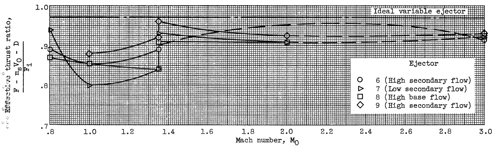
Figure 37. - Summary of performance of best ejector types.
