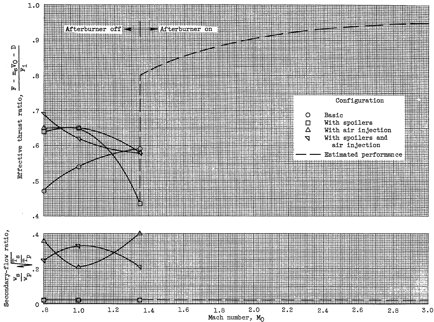
Figure 29. - Effect of spoilers and air injection on performance of fixed ejector 1.
