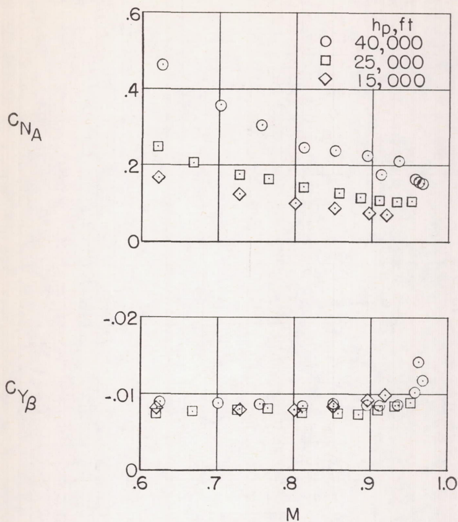
Figure 9.- Variation of C_{Y_B} and C_{N_A} determined in sideslip maneuvers at several altitudes.
