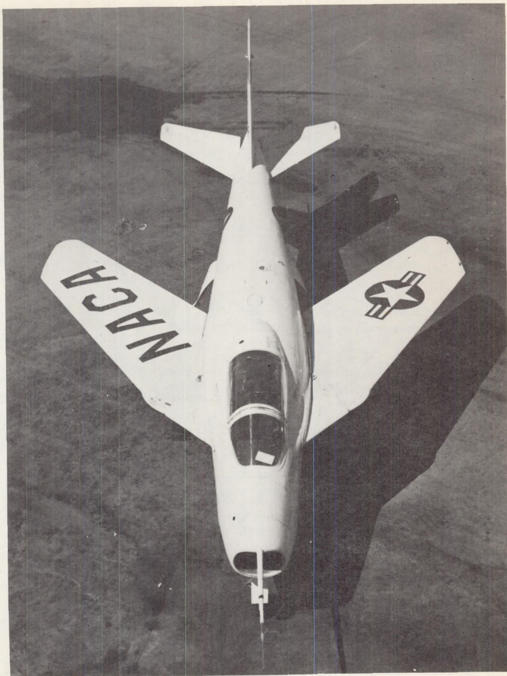
E-813 Figure 1.- Photograph of the Bell X-5 research airplane at 58.7^\circ sweepback.
