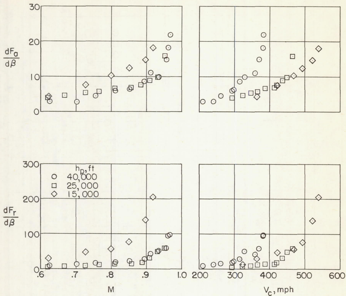
Figure 8.- Variation of control-force characteristics in sideslip with Mach number and calibrated airspeed.
