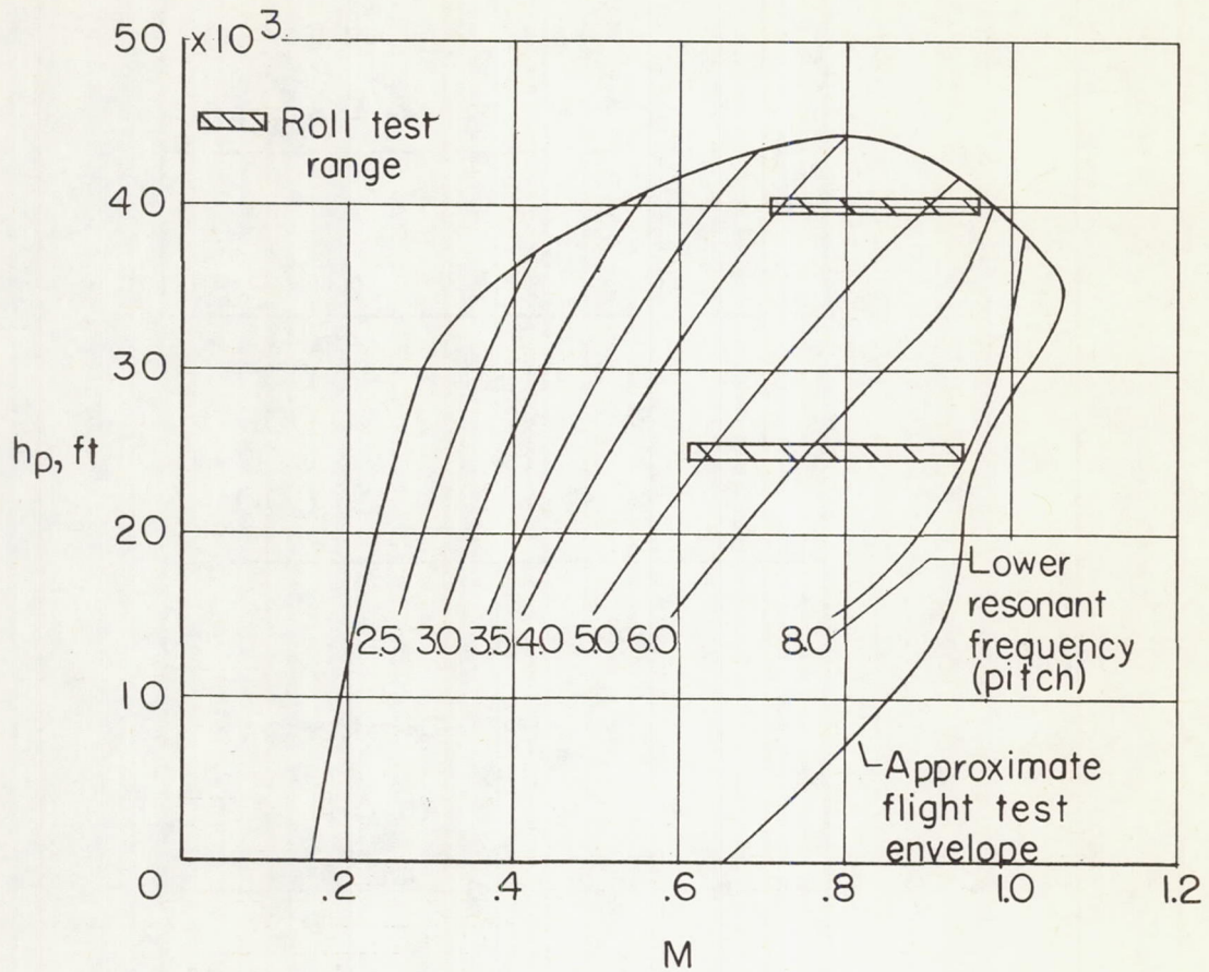
Figure 13.- Approximate flight test envelope of X-5 airplane showing lines of constant lower resonant frequency (pitch).
