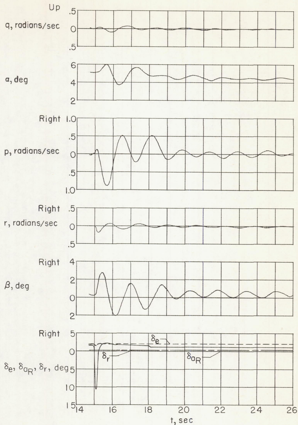
Figure 3.- Time history of lateral oscillation resulting from a rudder pulse at M = 0.90 ; h_p = 40,000 feet.
