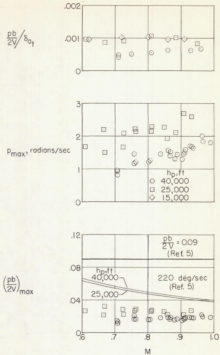
Figure 11.- Variation of aileron effectiveness, maximum rolling velocity, and maximum wing-tip helix angle with Mach number and comparison with the Military Specification.
