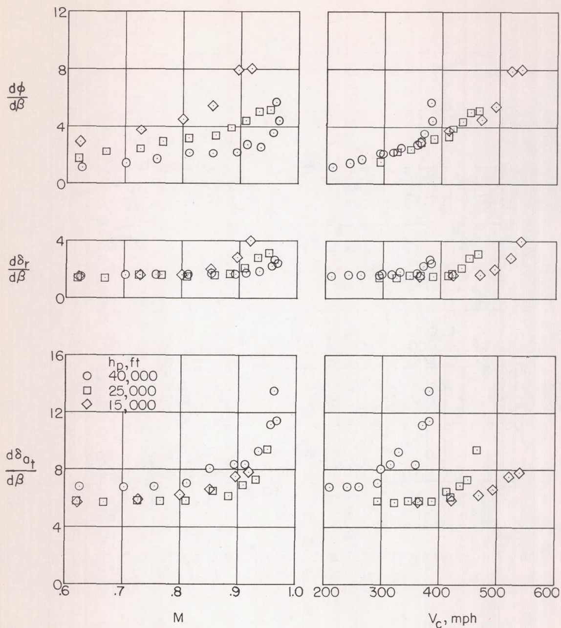
Figure 7.- Variation of several apparent lateral stability parameters with Mach number and calibrated airspeed.
