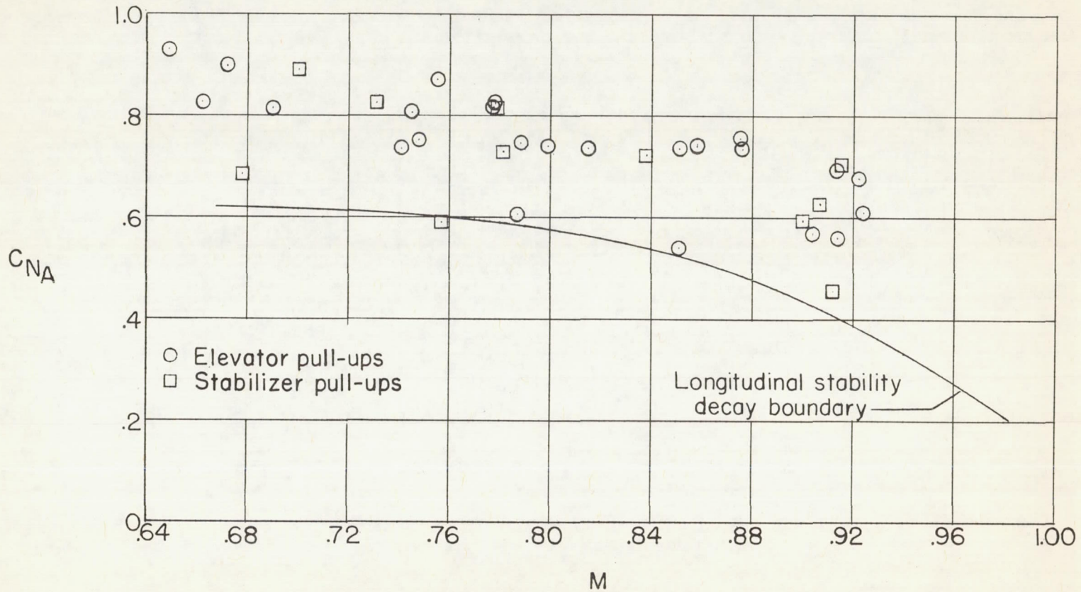
Figure 15.- Variation of C_{NA} with M for occurrence of directional divergence as compared with the longitudinal stability decay boundary. h_p = 40,000 feet.
