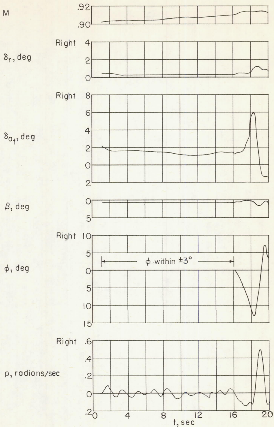
Figure 19.- Example of wing dropping at an altitude of 40,000 feet.
