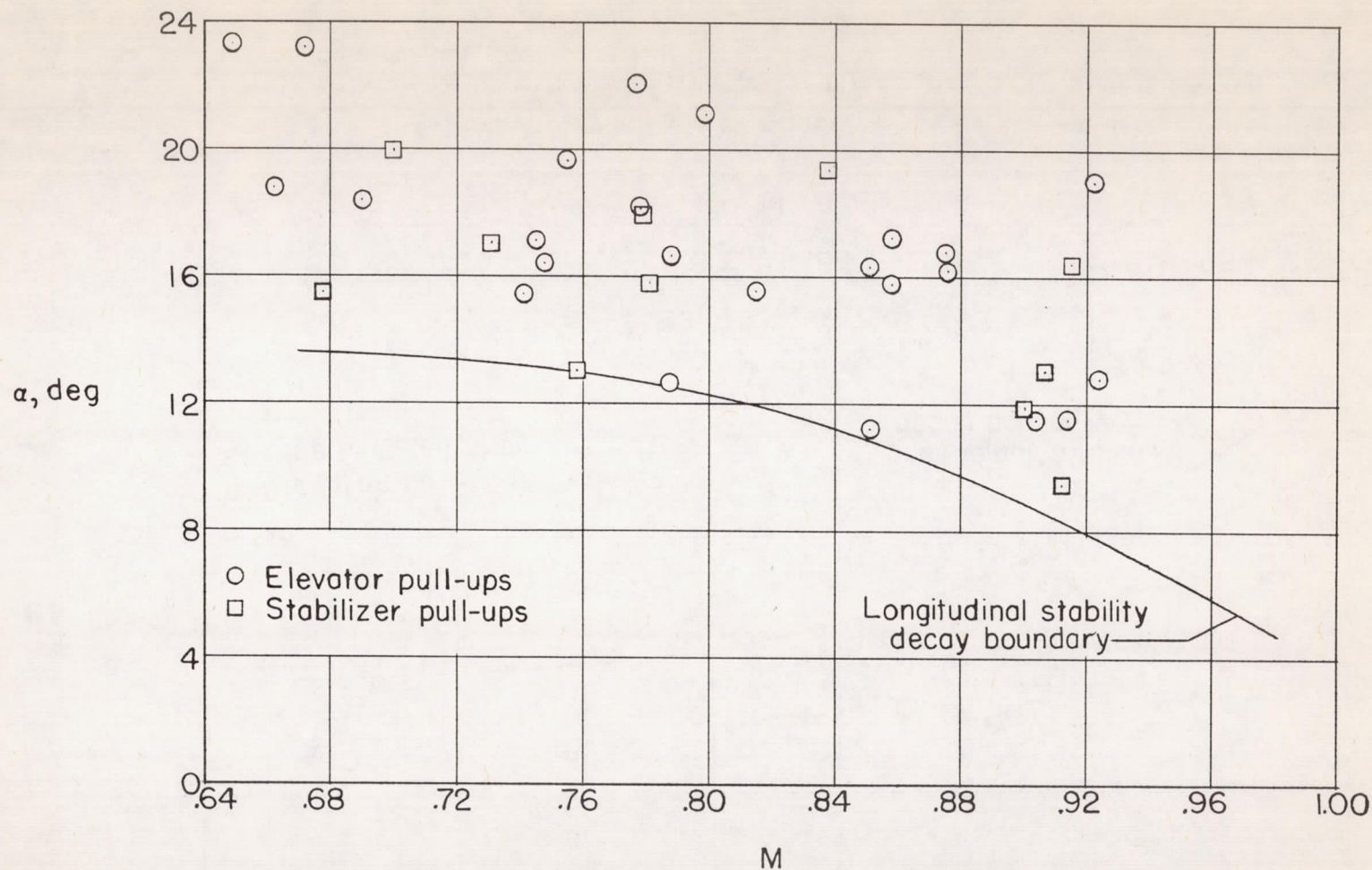
Figure 16.- Variation of \alpha with M for occurrence of directional divergence as compared with the longitudinal stability decay boundary. h_p = 40,000 feet.
