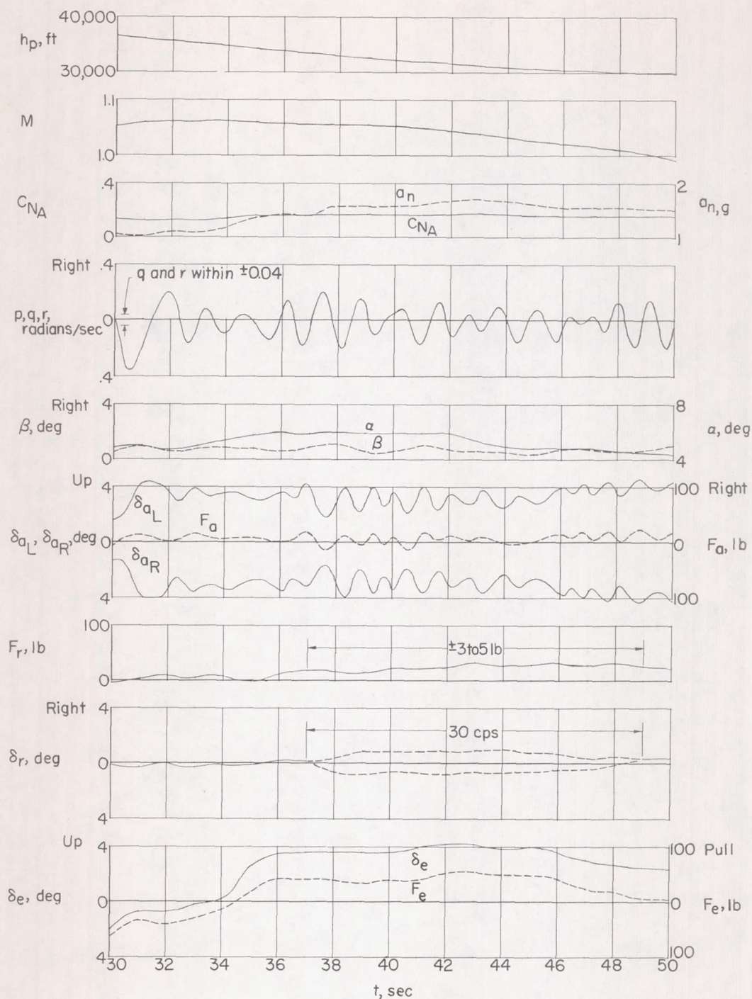
Figure 20.- Time history of quantities measured during single-degree-of-freedom flutter of the rudder.
