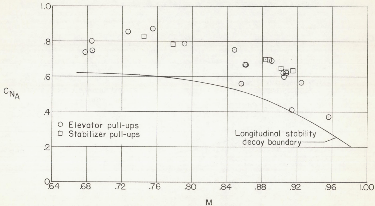
Figure 17.- Variation of C_{NA} with M for occurrence of aileron overbalance as compared with the longitudinal stability decay boundary. h_p = 40,000 feet.
