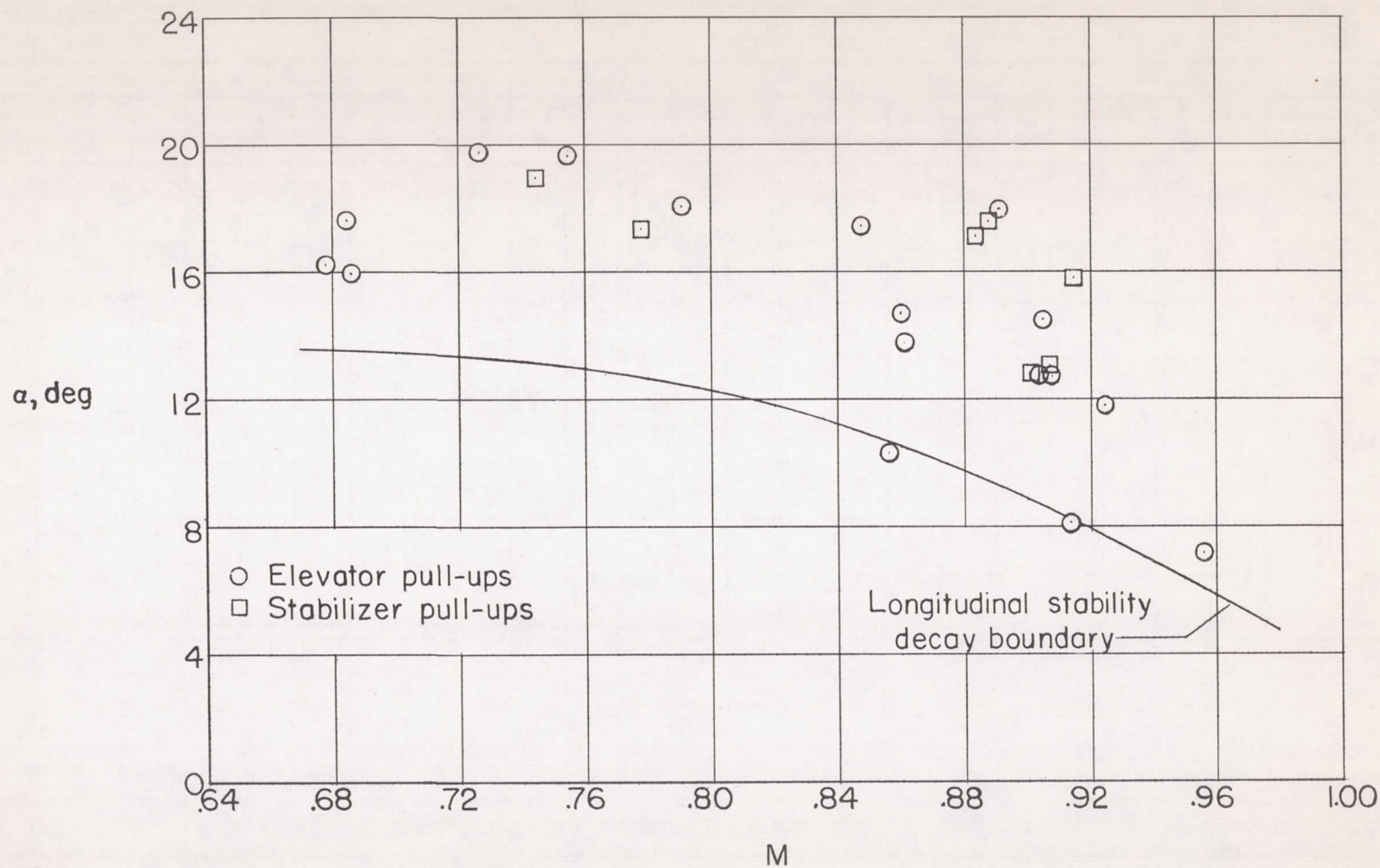
Figure 18.- Variation of \alpha with M for occurrence of aileron overbalance as compared with the longitudinal stability decay boundary. h_p = 40,000 feet.
