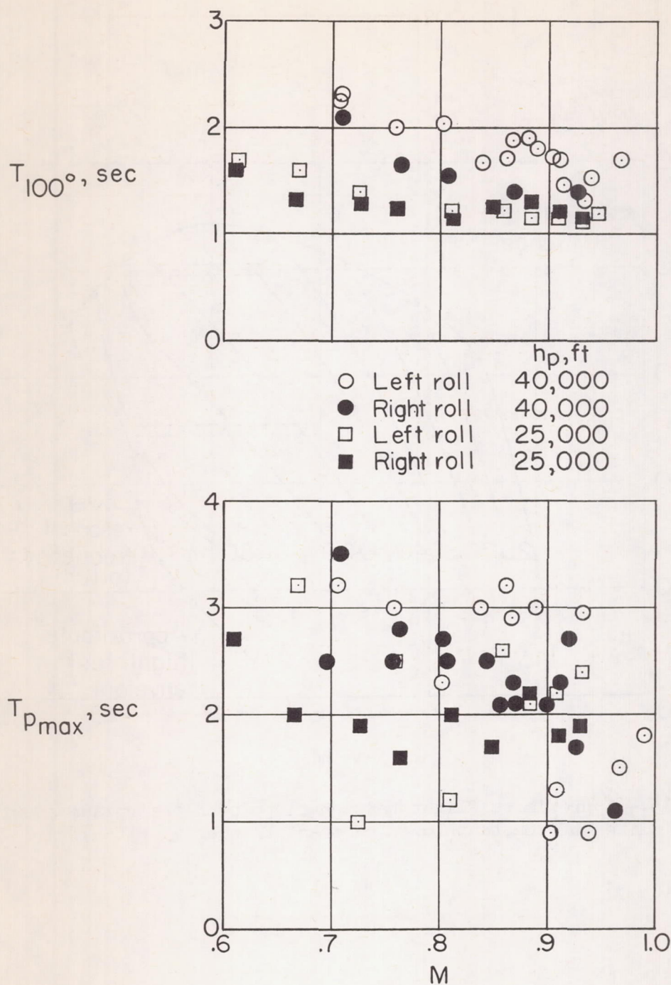
Figure 12.- Variation of time to bank to 100^\circ and time to bank to maximum rolling velocity with Mach number for full-deflection rolls.
