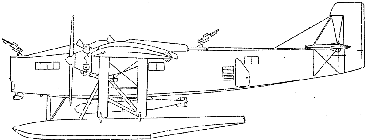
Fig.1 General arrangement drawing of the C.A.M.S.60 seaplane.
