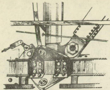
Fig. 4 Fitting on lower longeron of fuselage.
