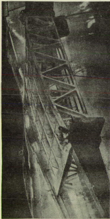
Figure 7.- View showing special ribs in the wing root.
