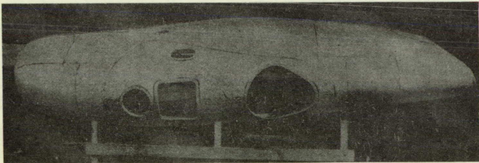
Figure 4.- View of the Scapa engine nacelle, which has been placed on its side in order to show the inspection doors in the floor by which engineers reach the engines. The nacelle is of all-metal construction. " Flight "
