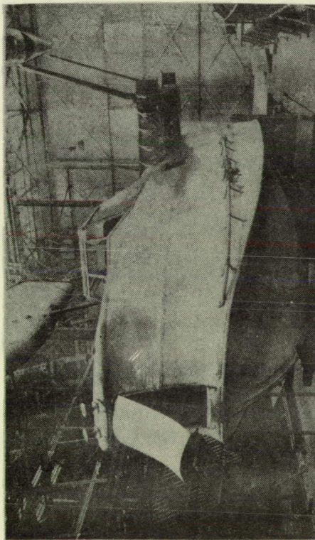
Figure 8.- View of hull with wing root in place.
