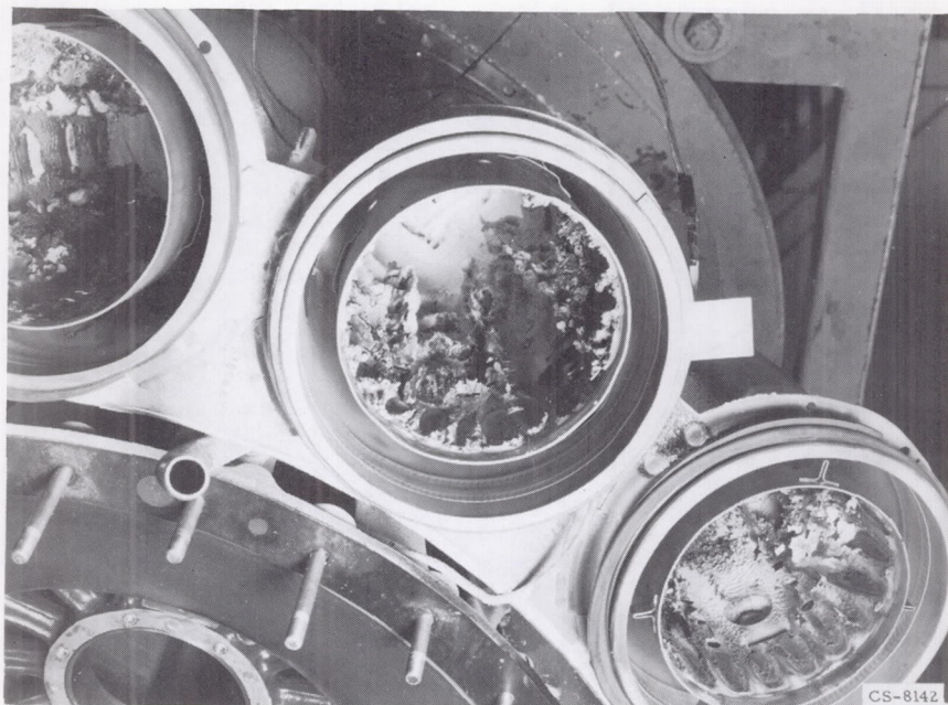
Figure 17. - Deposits from trimethylborate in upstream end of combustor. Domes have been removed.
