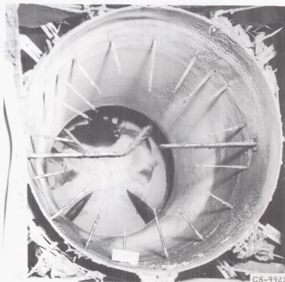
PRIMARY COMBUSTOR OPERATION WITH B_5H_9 + 100 MIN JP-4
