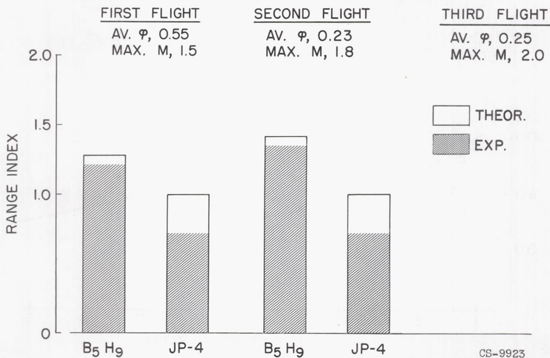
Figure 38. - Relative performance of pentaborane and JP-4 in ram-jet flights.
