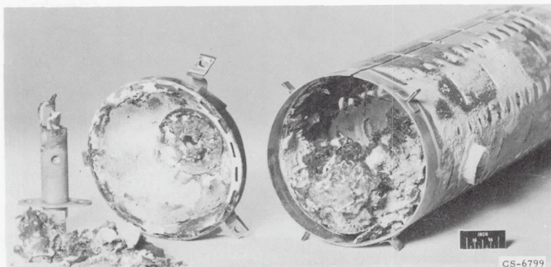
Figure 7. - Boron oxide deposits from diborane in combustor configuration 1.
