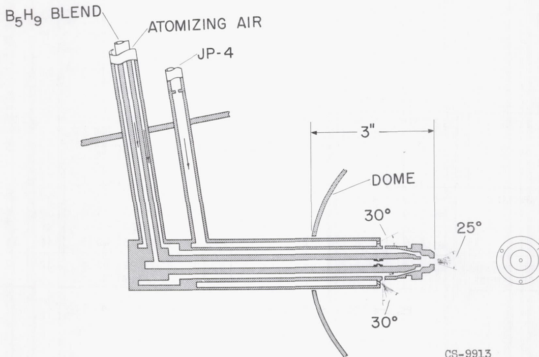
Figure 14. - Dual-fuel injector.
