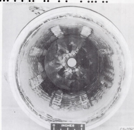
FUEL INJECTOR ON WALL 330 LB B_2O_3 1\frac{1}{2} HR OPERATION WITH JP-4
