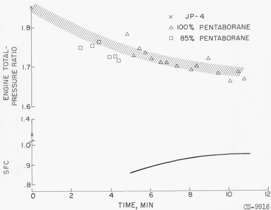
Figure 26. - Effect of operating time on engine performance. Variable-area exhaust nozzle; altitude, 50,000 feet; Mach number, 0.8.
