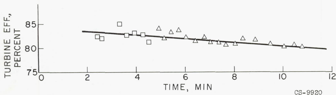
Figure 27. - Effect of operating time on component performance. Variable-area exhaust nozzle; injectors located on combustor wall; altitude, 50,000 feet; Mach number, 0.8.
