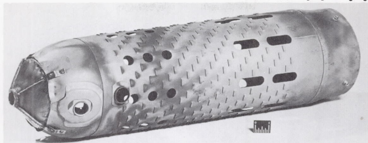
MODIFIED J47 COMBUSTOR
