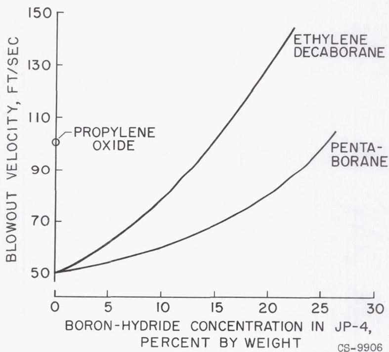
Figure 5. - Blowout velocities of boron hydride - JP-4 fuel mixtures. Equivalence ratio, 1.0.
