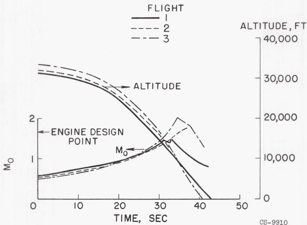
Figure 37. - Ram-jet flights with pentaborane.
