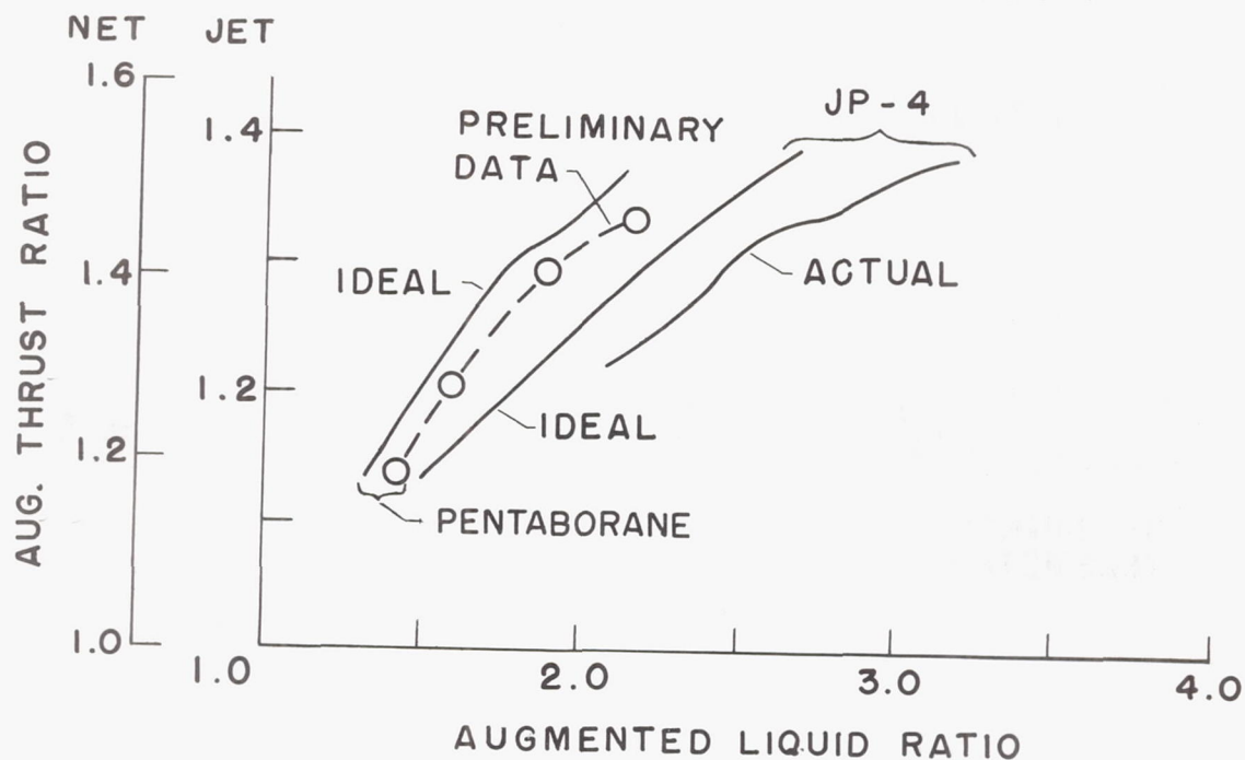
Figure 33. - Afterburner performance. Altitude, 50,000 feet; Mach number, 0.6.
