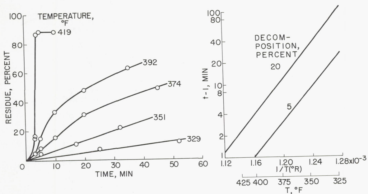
Figure 3. - Thermal decomposition of pentaborane.
