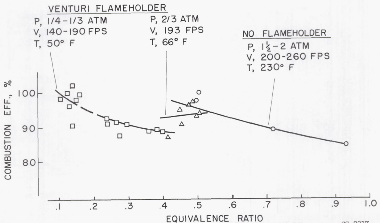
Figure 36. - Pentaborane performance in connected-pipe combustor.
