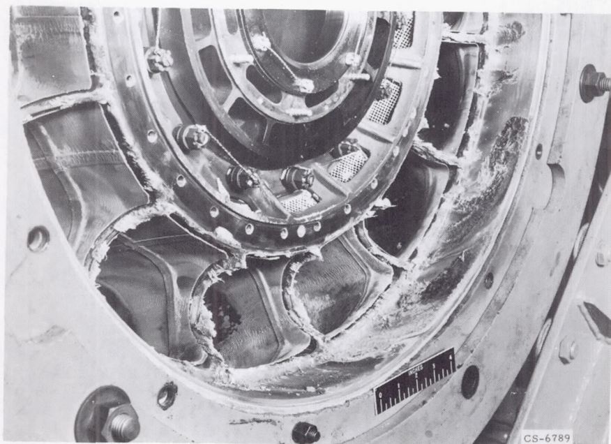
Figure 18. - Buildup of deposits at combustor exit.
