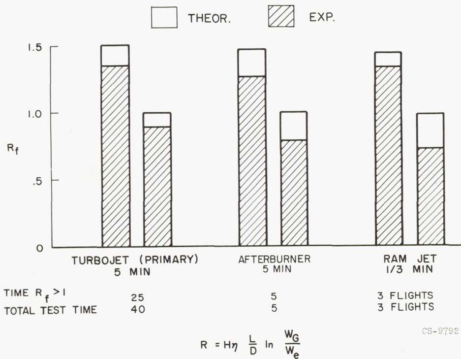
Figure 39. - Summary of pentaborane data.
