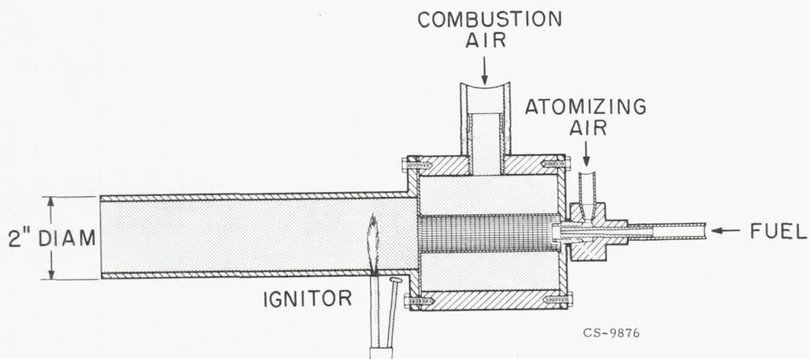
Figure 4. - Blowout-velocity apparatus.
