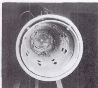
COMBUSTOR
