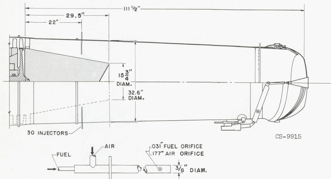
Figure 32. - Pentaborane afterburner.
