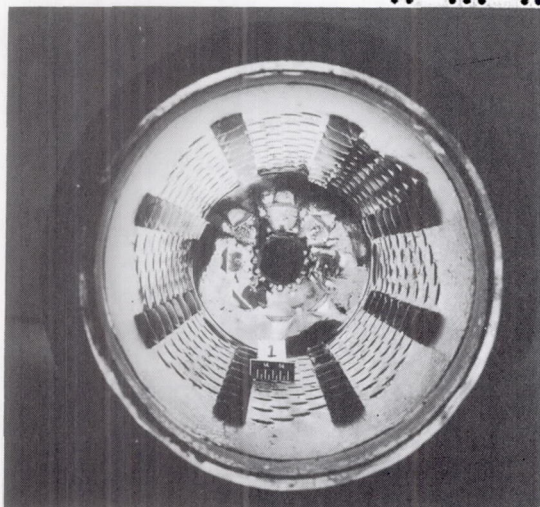
AIR-ATOMIZING FUEL INJECTOR 220 LB B_2O_3 8 MIN OPERATION WITH JP-4
