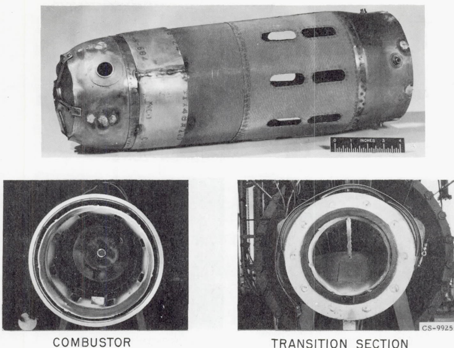
Figure 11. - Wire-cloth combustor liner for pentaborane. Operating time, 13.3 minutes; pressure, 1/2 atmosphere; outlet temperature, 925^{\circ} F.
