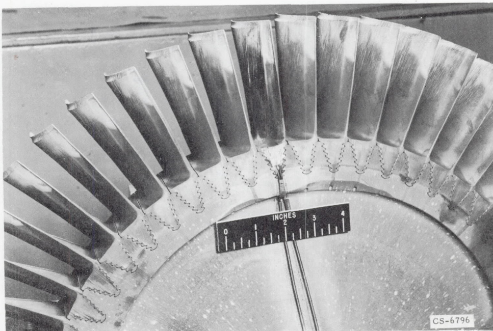
Figure 20. - Buildup of deposits on turbine rotor. Downstream view.
