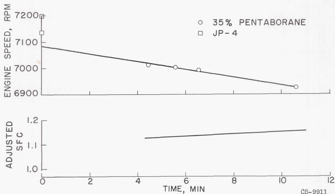
Figure 25. - Effect of operating time on engine performance. Fixed-area exhaust nozzle; altitude, 50,000 feet; Mach number, 0.8.
