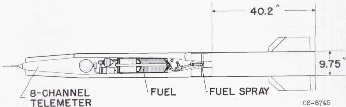
Figure 35. - Free-flight ram jet.
