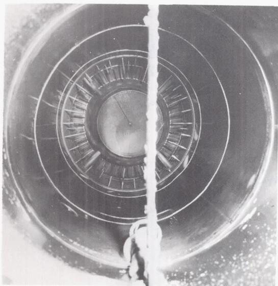
AFTERBURNER OPERATION WITH B_5H_9 + 10 MIN JP-4
