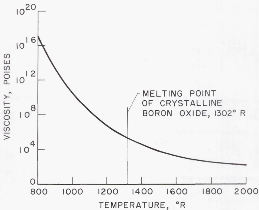
Figure 6. - Viscosity of vitreous boron oxide B_2O_3 (ref. 11).
