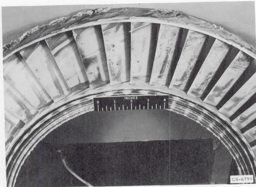
Figure 19. - Buildup of deposits on nozzle diaphragm. Downstream view.
