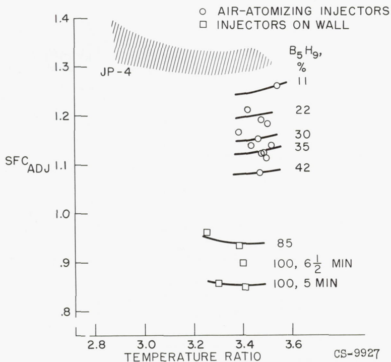
Figure 24. - Engine performance of pentaborane and JP-4 fuel mixtures. Altitude, 50,000 feet; Mach number, 0.8.
