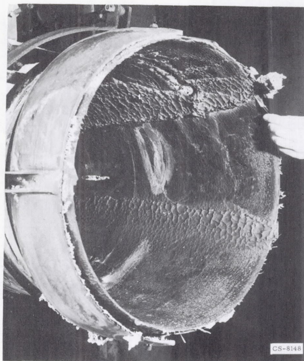
Figure 21. - Deposits on tailpipe.
