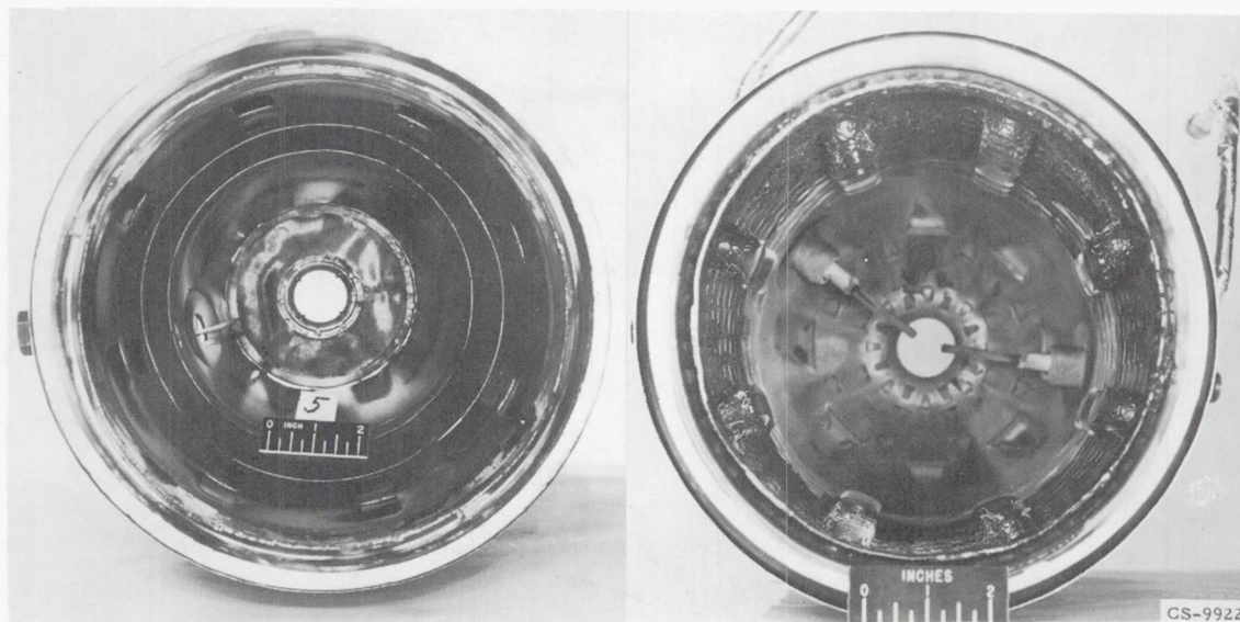
CONVENTIONAL COMBUSTOR INJECTORS ON WALL
