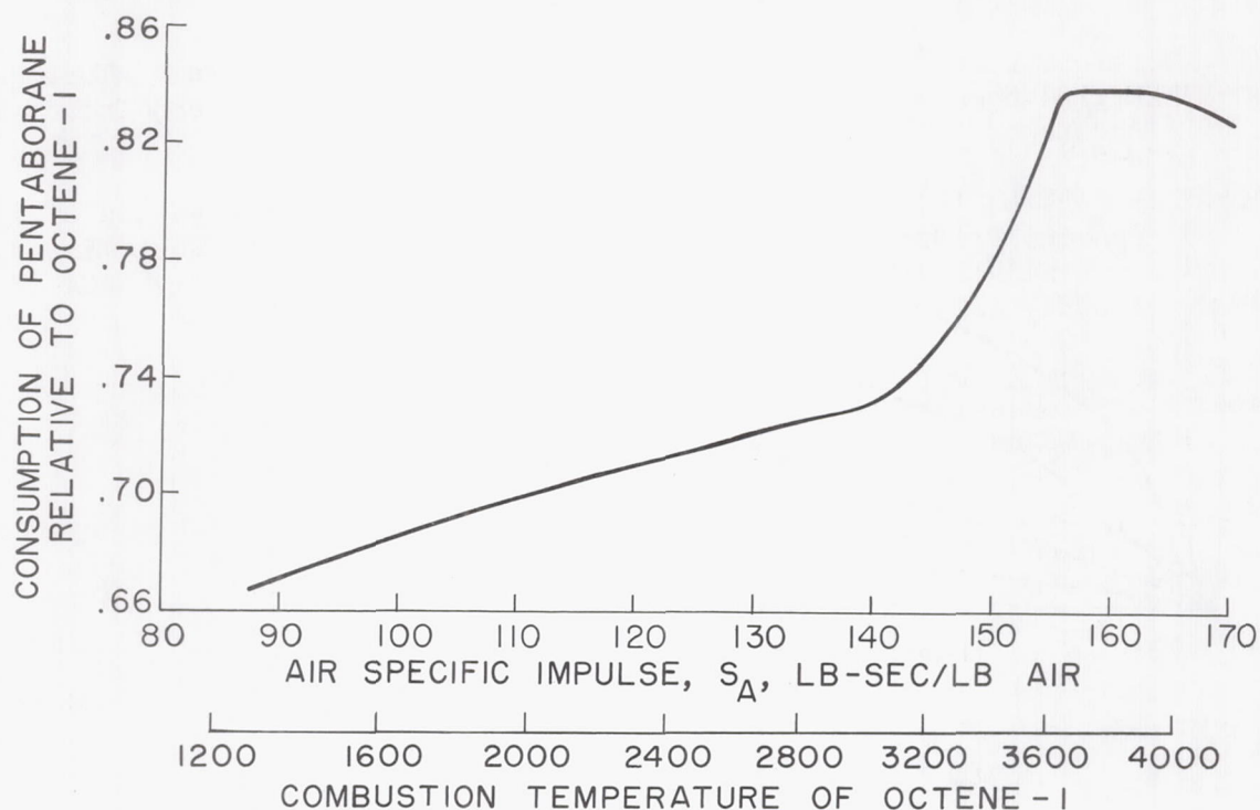
Figure 1. - Consumption of pentaborane relative to octene-1 against air specific impulse for combustion pressure of 2 atmospheres. Frozen composition; Mach number in combustor, 2.
