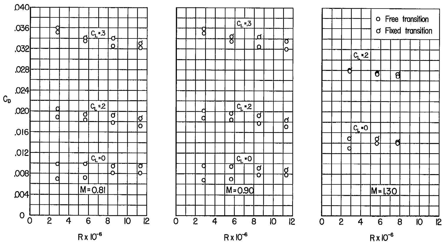
(b) C_D vs. Reynolds number.
