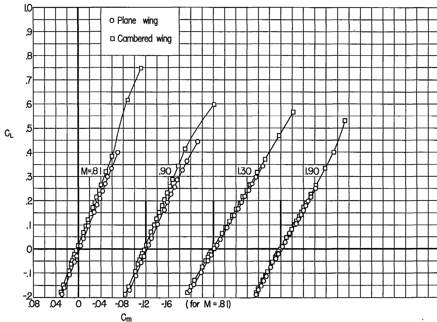
(b) C_L vs. C_m Figure 15.- Concluded.
