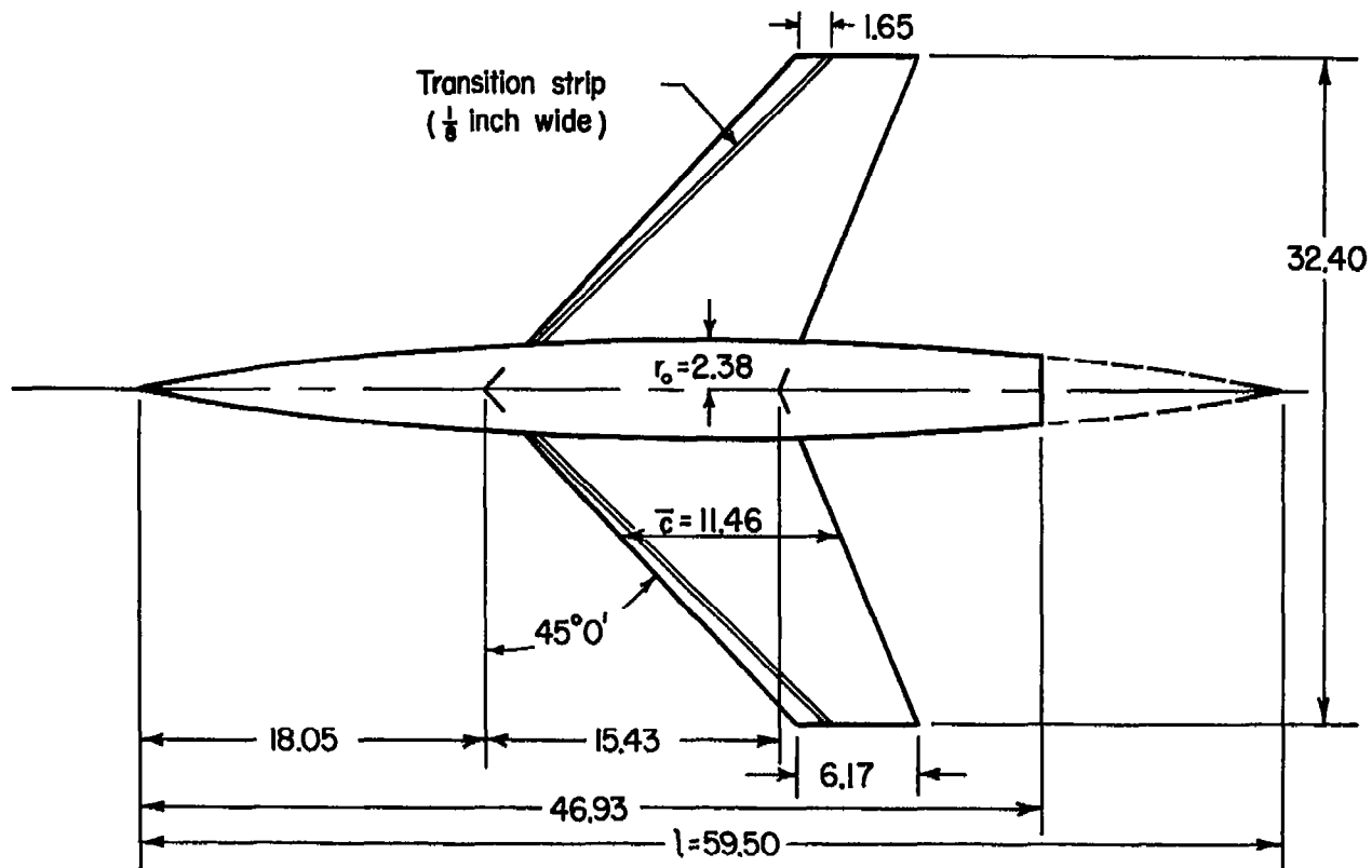
(b) Sweptback wing.
