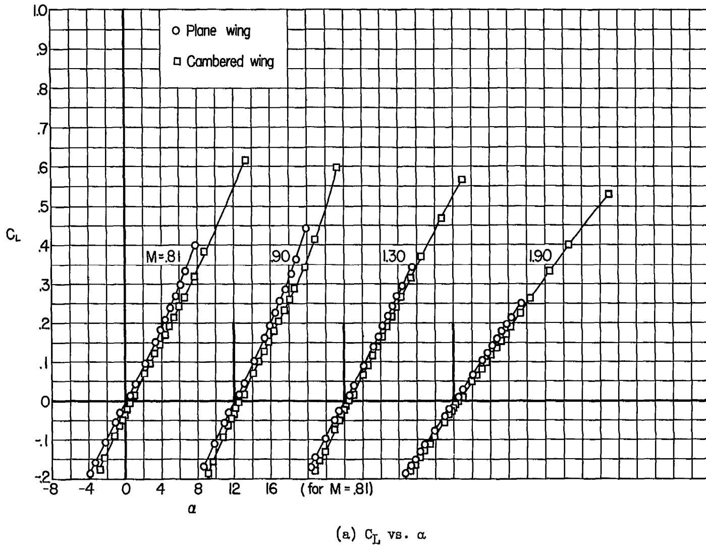
Figure 15.- Effect of conical camber on the lift and pitching-moment characteristics of a 3-percent-thick triangular wing with fixed transition; R = 5.6 \times 10^6 .
