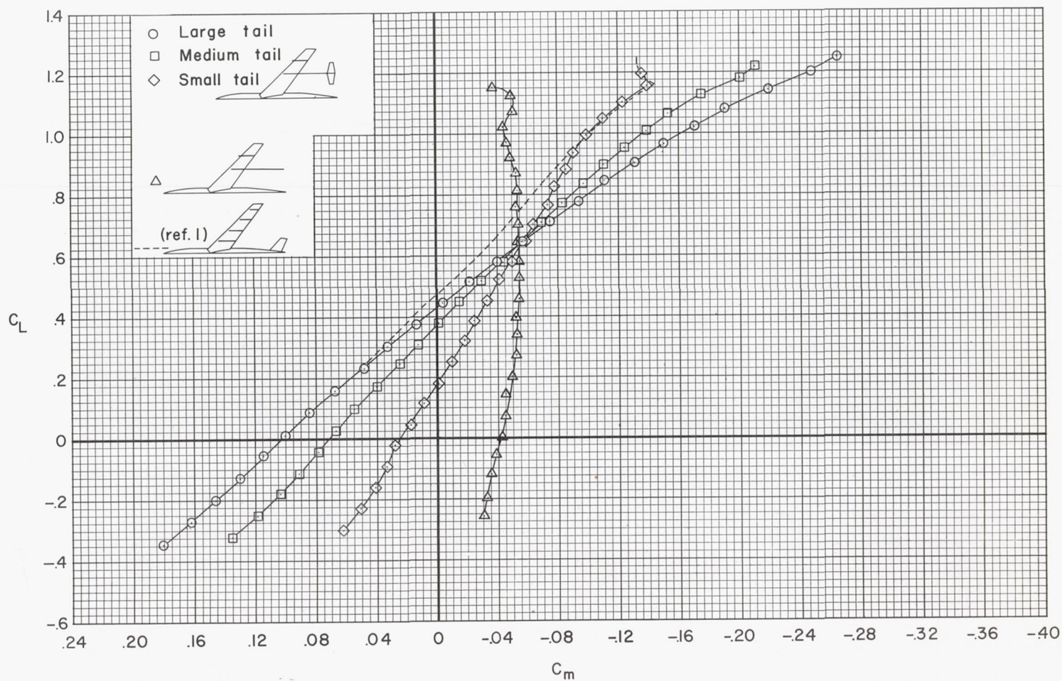
Figure 11.- The effects of tail size on the pitching-moment characteristics of the model; tails in low position at 0.5 b/2 ; i_t = -6^\circ .
