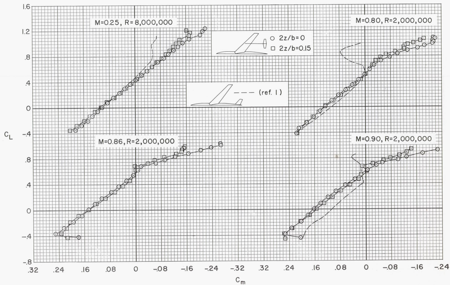
(a) Effects of changing vertical position of horizontal tail.
