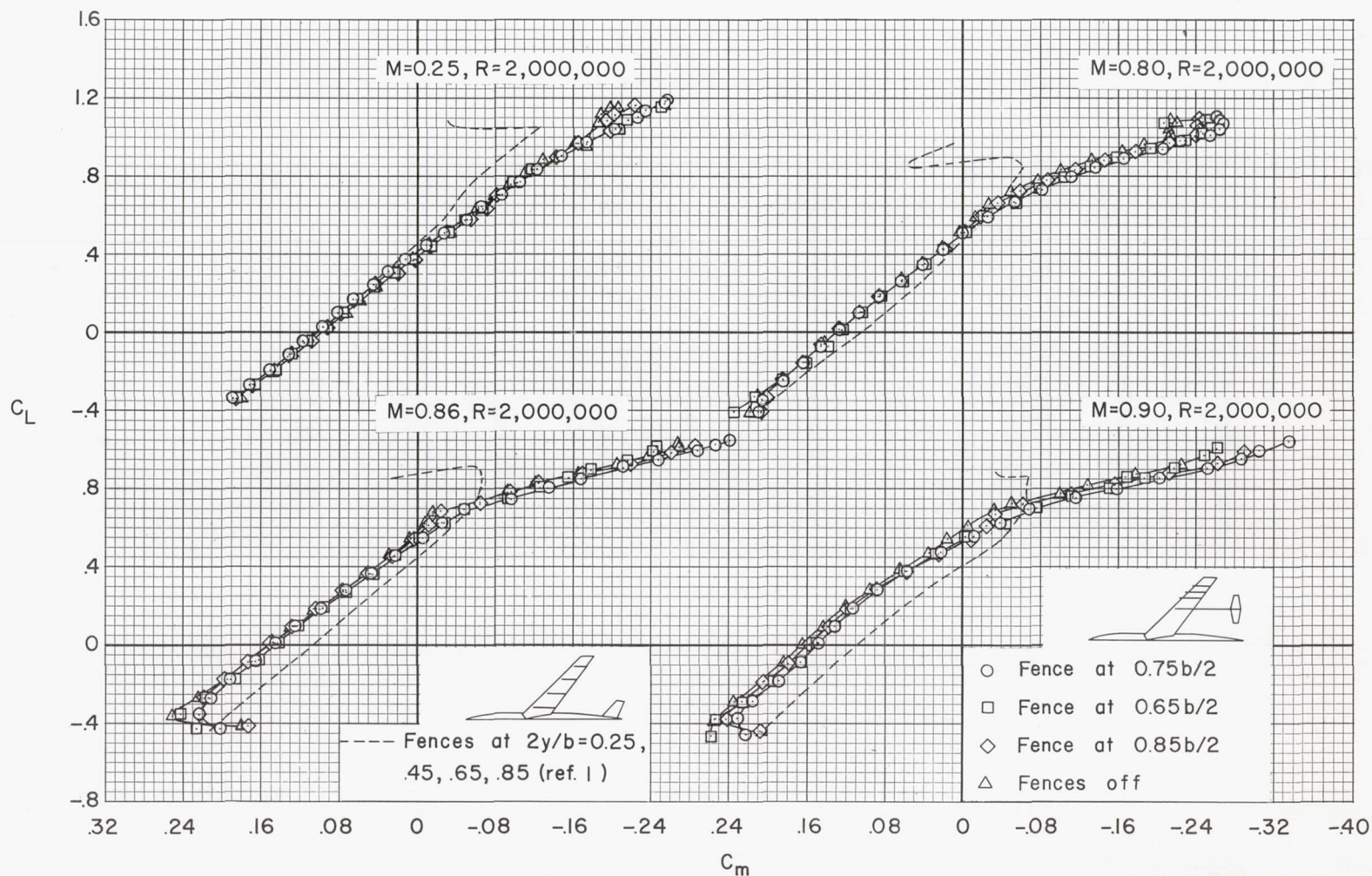
Figure 6.- The effects of a wing fence on the pitching-moment characteristics of the model with the large outboard tail in the low position at 0.5 b/2 ; i_t = -6^\circ .
