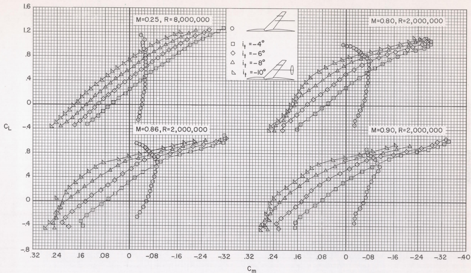
Figure 9.- The pitching-moment characteristics of the model with the large outboard tail at several incidences; tail in low position at 0.5 b/2 .
