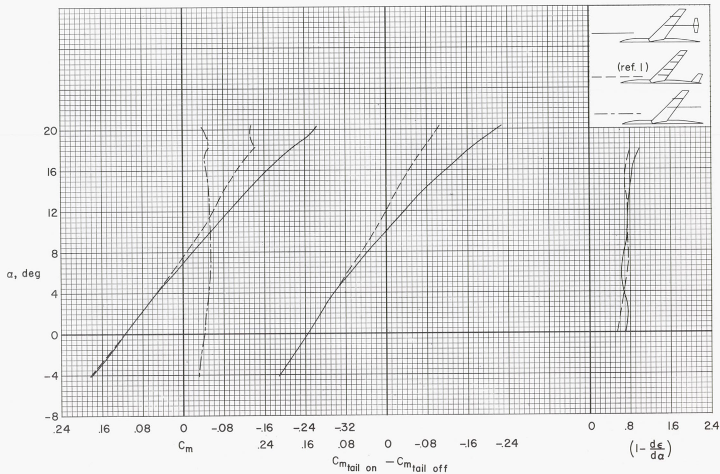
(a) M = 0.25 , R = 8,000,000
