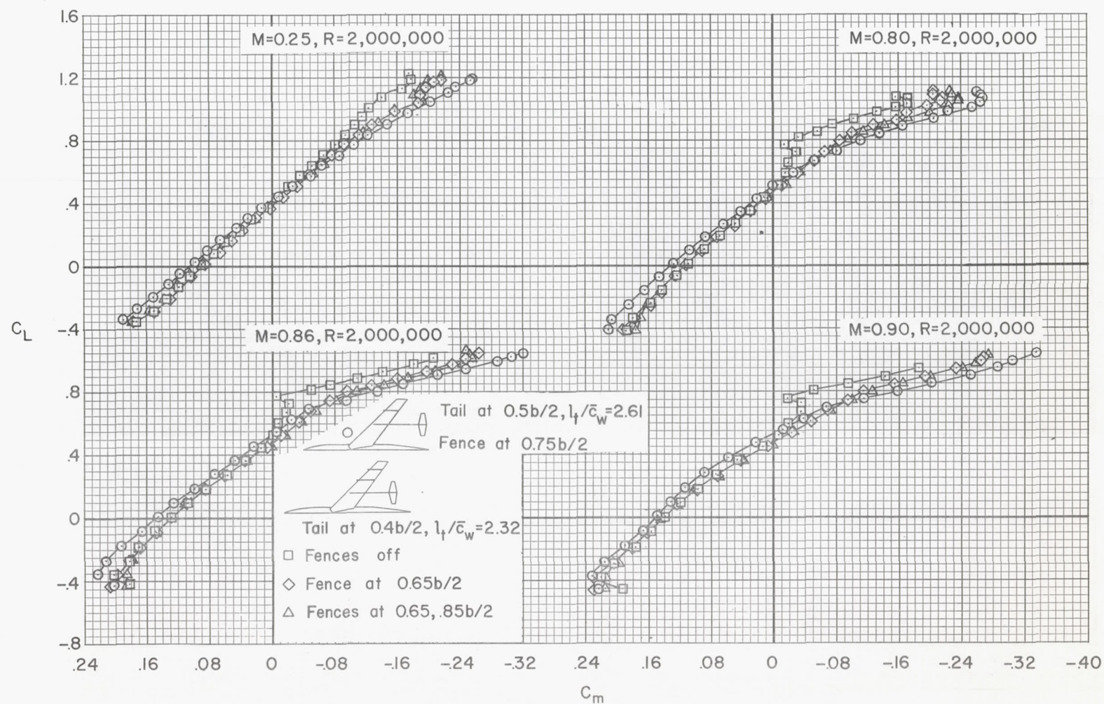
Figure 8.- A comparison of the effects of wing fences on the pitching-moment characteristics of the model for two lateral positions of the large outboard tail; i_t = -6^\circ .
