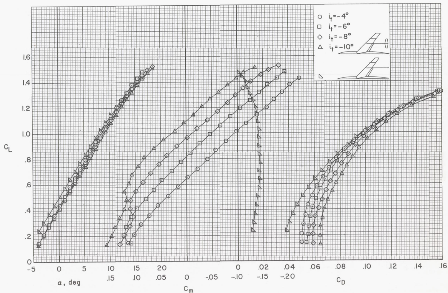
Figure 18.- The longitudinal characteristics of the model with large outboard tail at several incidences; tail in low position at 0.5 b/2 ; flaps deflected; M = 0.25 , R = 8,000,000 .
