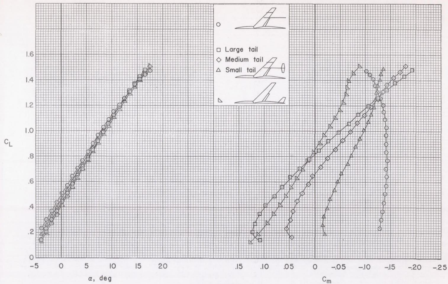
Figure 17.- The effects of tail size on the lift and pitching-moment characteristics of the model with flaps deflected; tails in low position at 0.5 b/2 ; i_t = -6^\circ , M = 0.25 , R = 8,000,000 .
