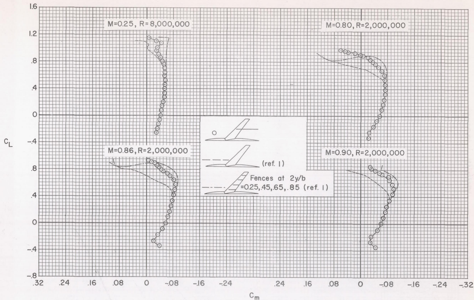
Figure 5.- The effectiveness of the tail-boom as a wing fence.
