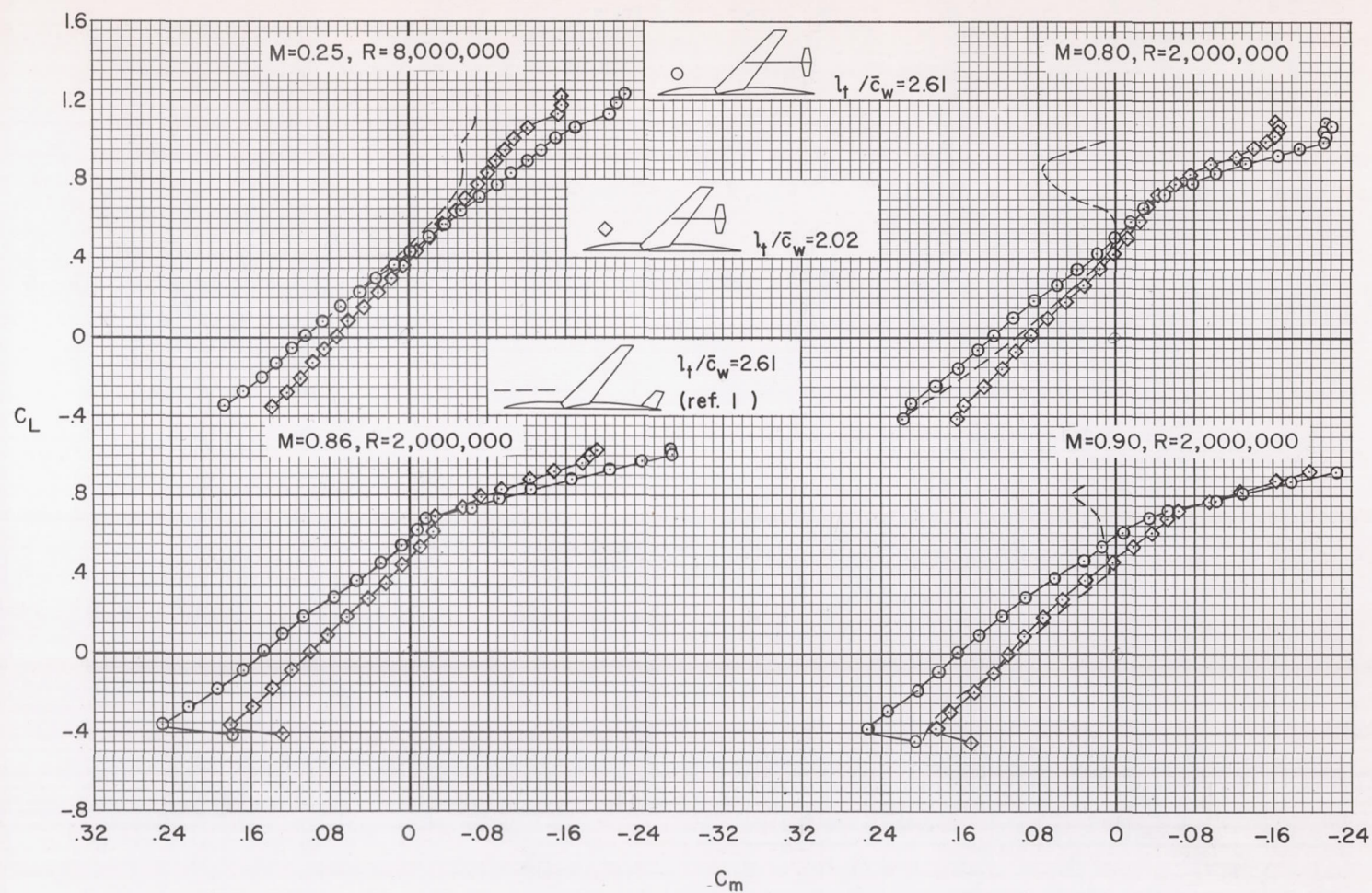
(b) Effects of changing longitudinal position of horizontal tail.
