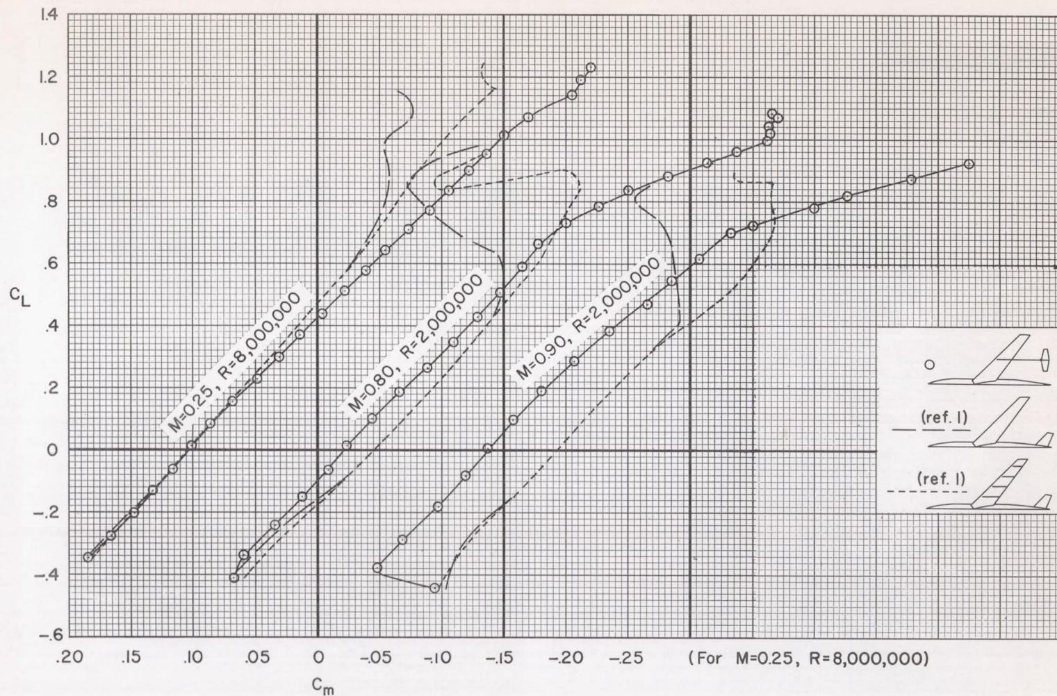
Figure 3.- A comparison of the pitching-moment characteristics of the model with a conventional sweptback tail and with the large outboard tail in the low position at 0.5 b/2 ; i_t = -6^\circ .
