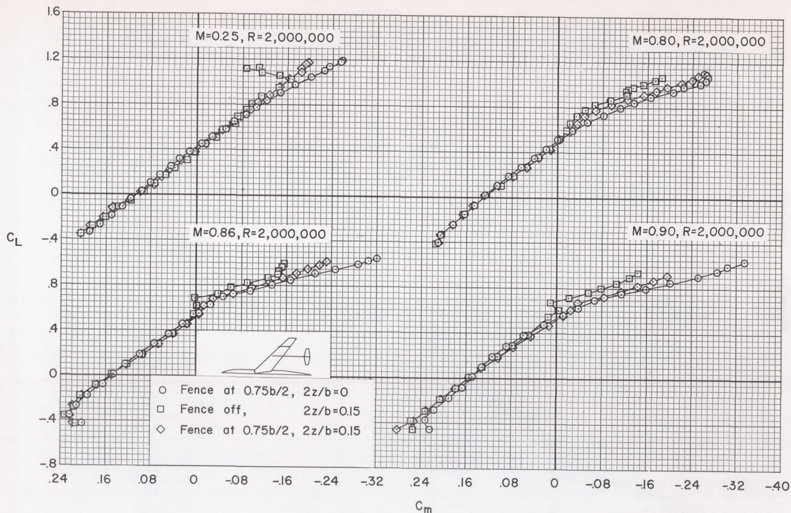
Figure 7.- A comparison of the effects of wing fences on the pitching-moment characteristics of the model for two heights of the large outboard tail at 0.5 b/2 ; i_t = -6^\circ .
