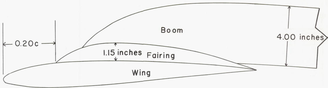
Wing-boom juncture
