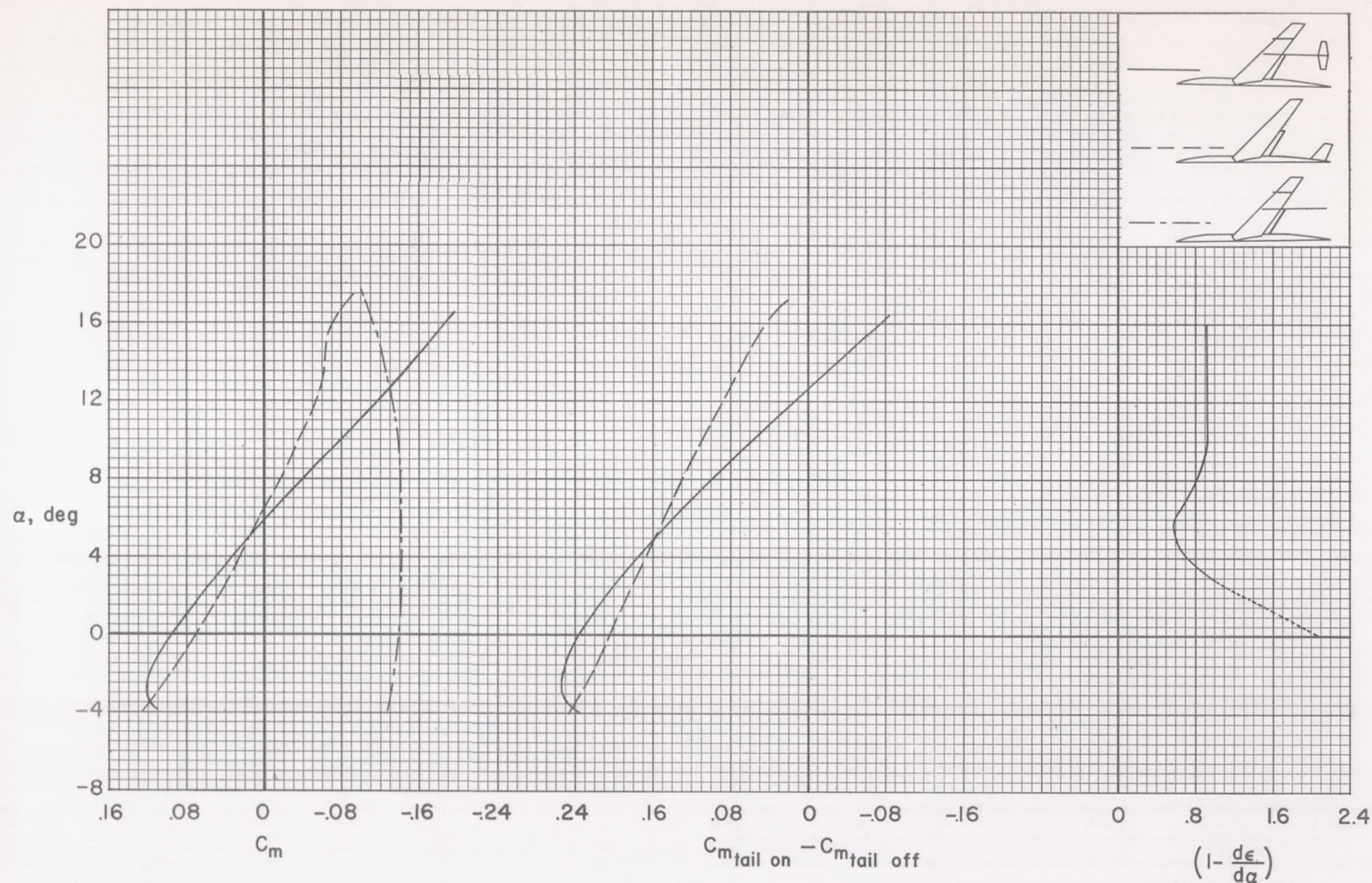
Figure 19.- The variations with angle of attack of total pitching-moment coefficient, pitching-moment coefficient due to horizontal tail, and downwash parameter for the model with a large outboard tail in low position at 0.5\ b/2 and with a conventional sweptback tail; flaps deflected; M = 0.25 , R = 8,000,000 , i_t = -6^\circ .
