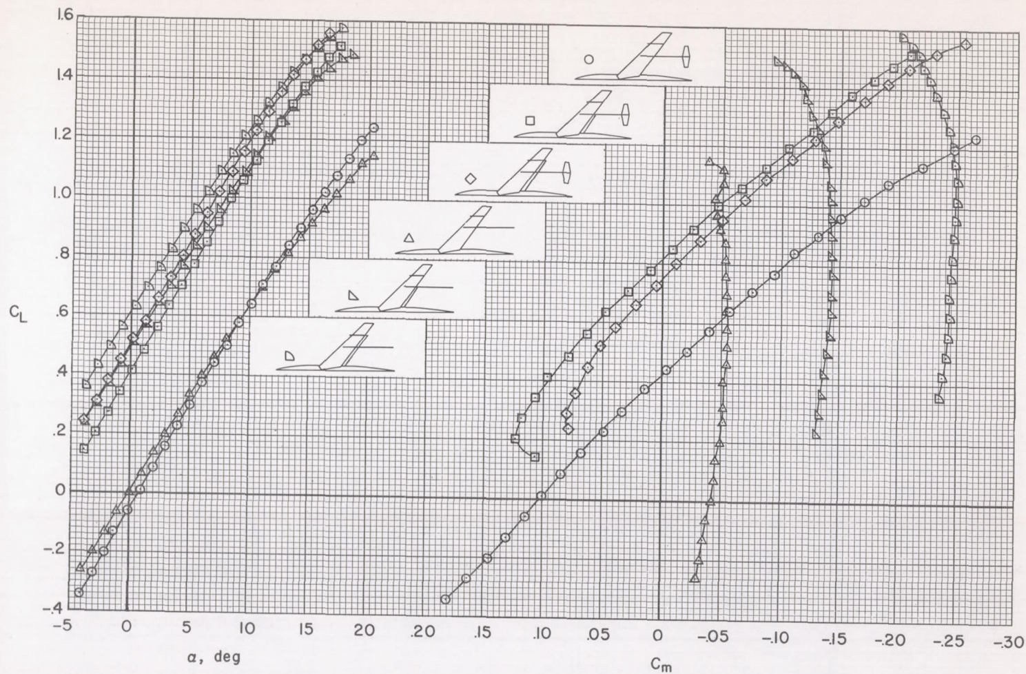
Figure 15.- The effects of flaps on the lift and pitching-moment characteristics of the model with and without the large outboard horizontal tail in low position at 0.5 b/2 ; M = 0.25 , R = 8,000,000 , i_t = -6^\circ .
