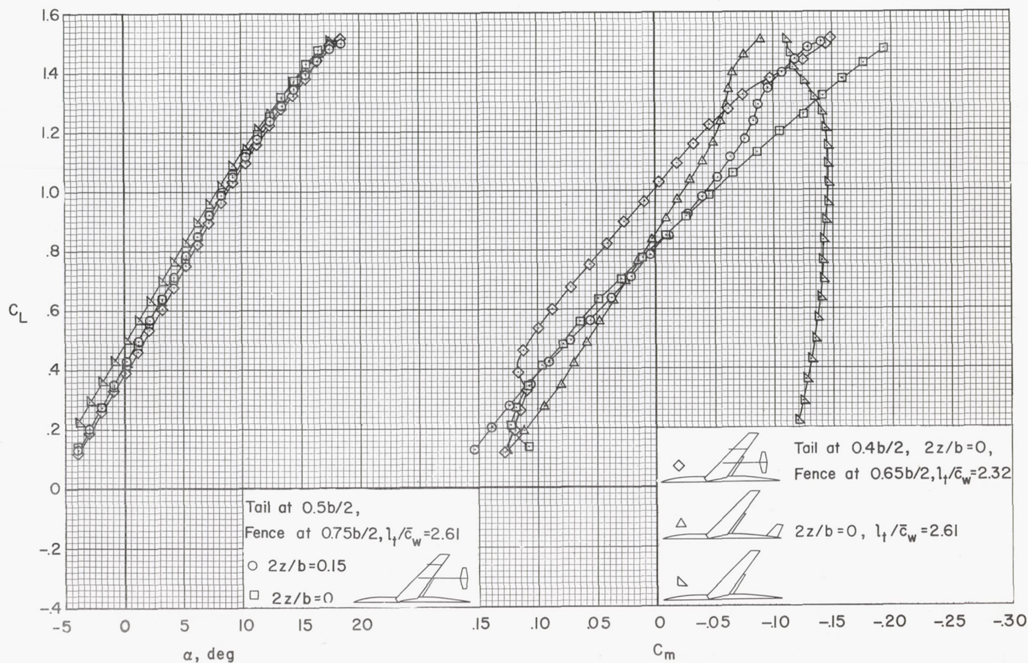
Figure 16.- The effects of tail position on the lift and pitching-moment characteristics of the model with flaps deflected; M = 0.25 , R = 8,000,000 , i_t = -6^\circ .
