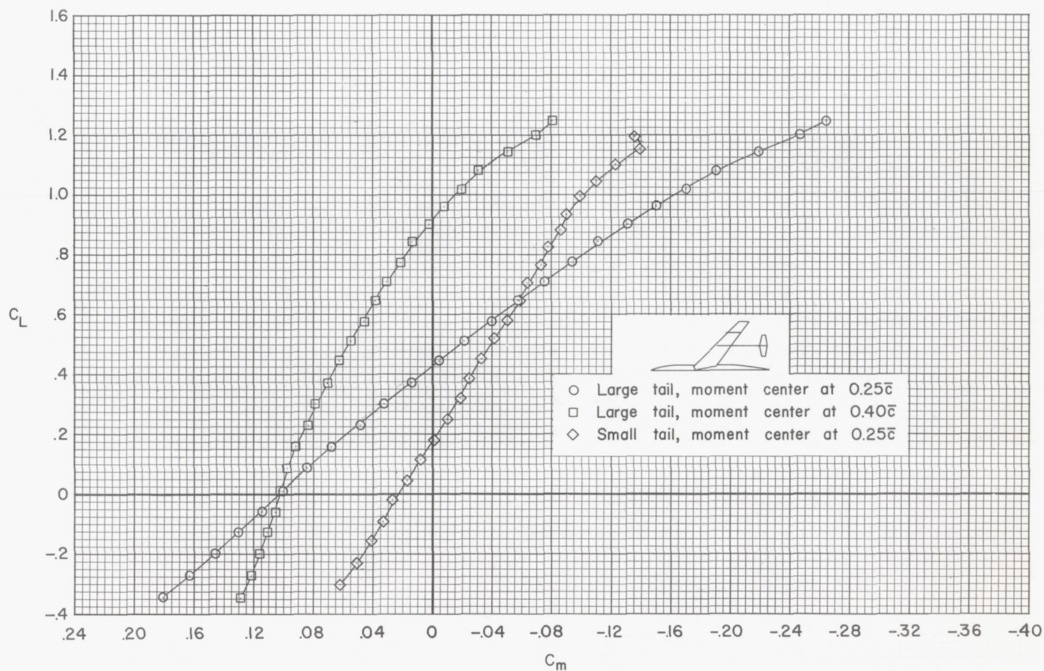
Figure 13.- A comparison of the changes in pitching-moment characteristics resulting from rearward movement of the moment center and from a reduction of tail size; tails at 0.5 b/2 ; i_t = -6^\circ .
