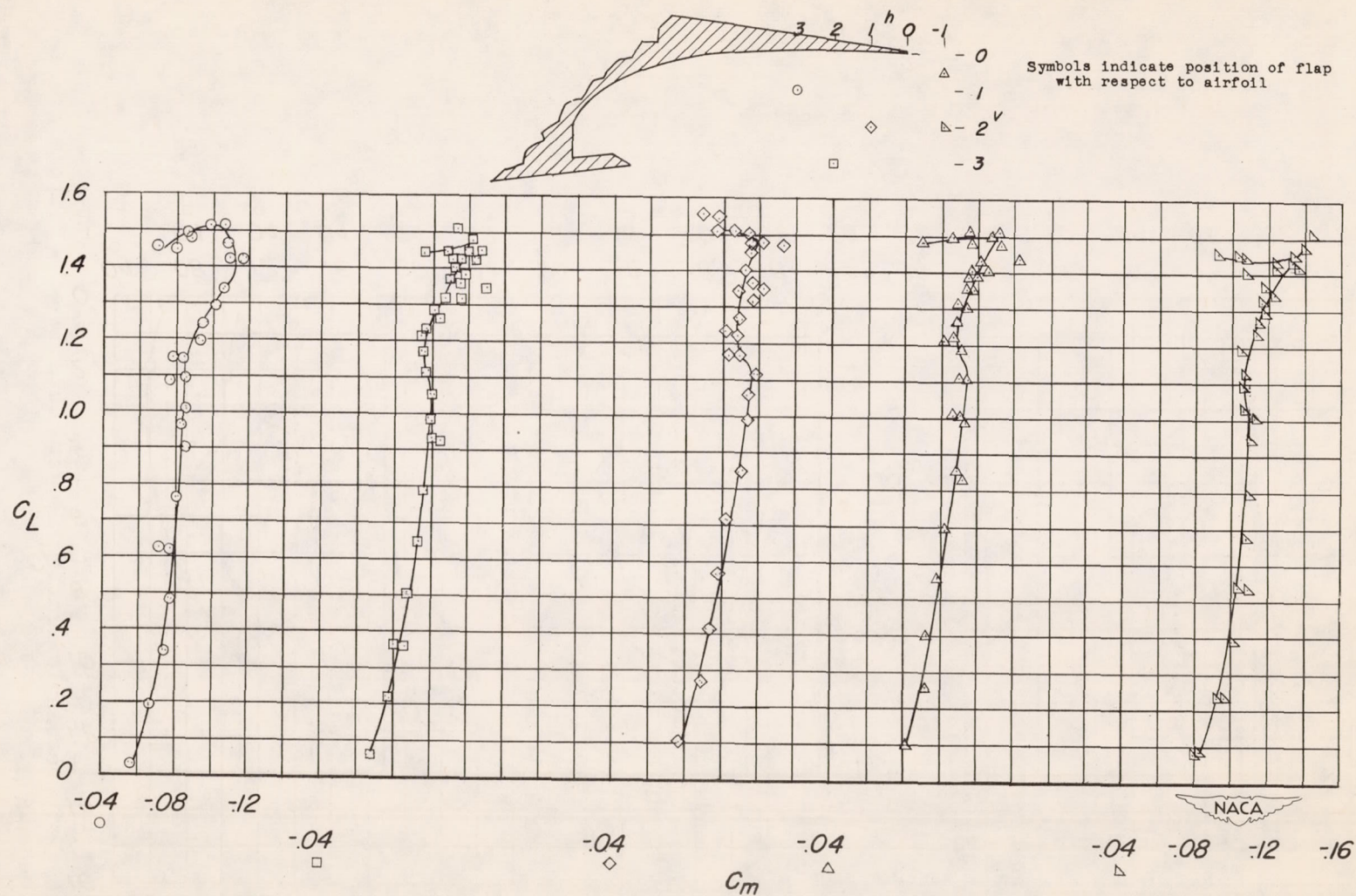
(c) C_L against C_m .
