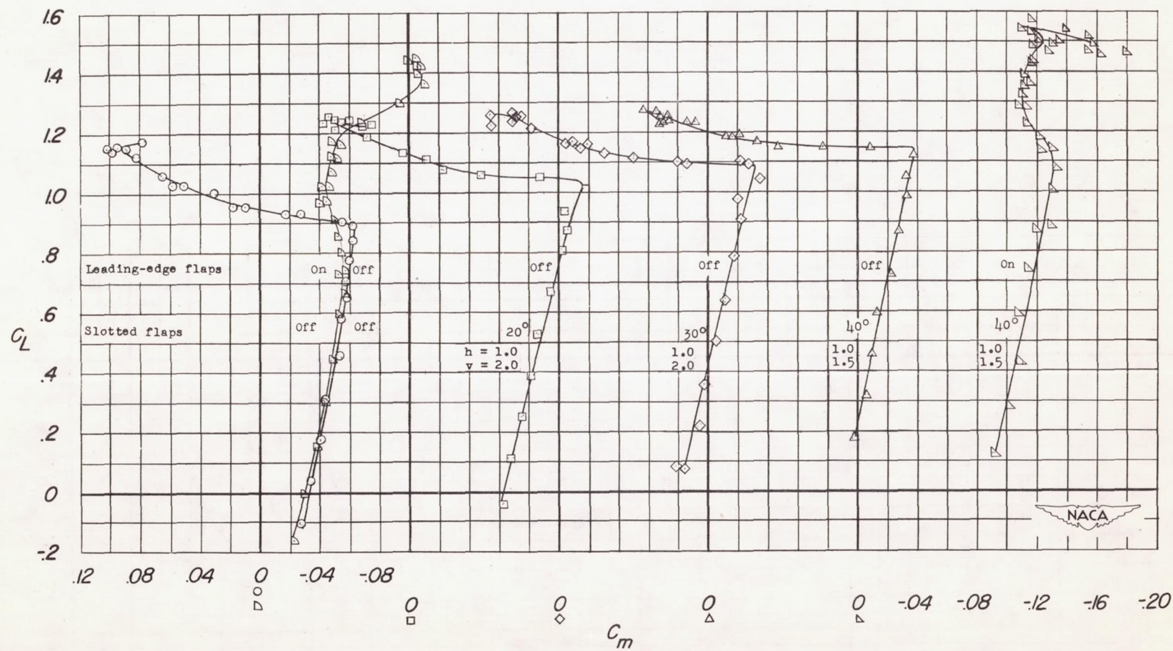
(c) C_L against C_m .
