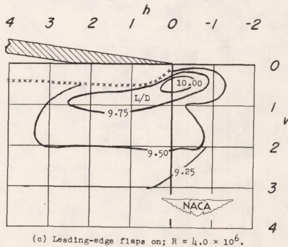
Figure 12.- Values of L/D at C_L = 0.8 for various positions of the single slotted flaps. \delta_f = 40^\circ .
