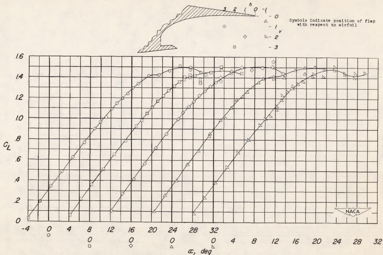
(a) C_L against \alpha .
