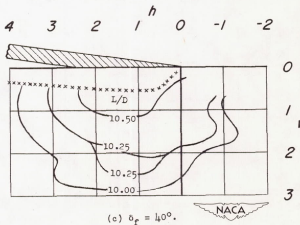
Figure 11.- Values of L/D at C_L = 0.8 for various positions of the single slotted flaps. Leading-edge flaps off; R = 4.0 \times 10^6 .
