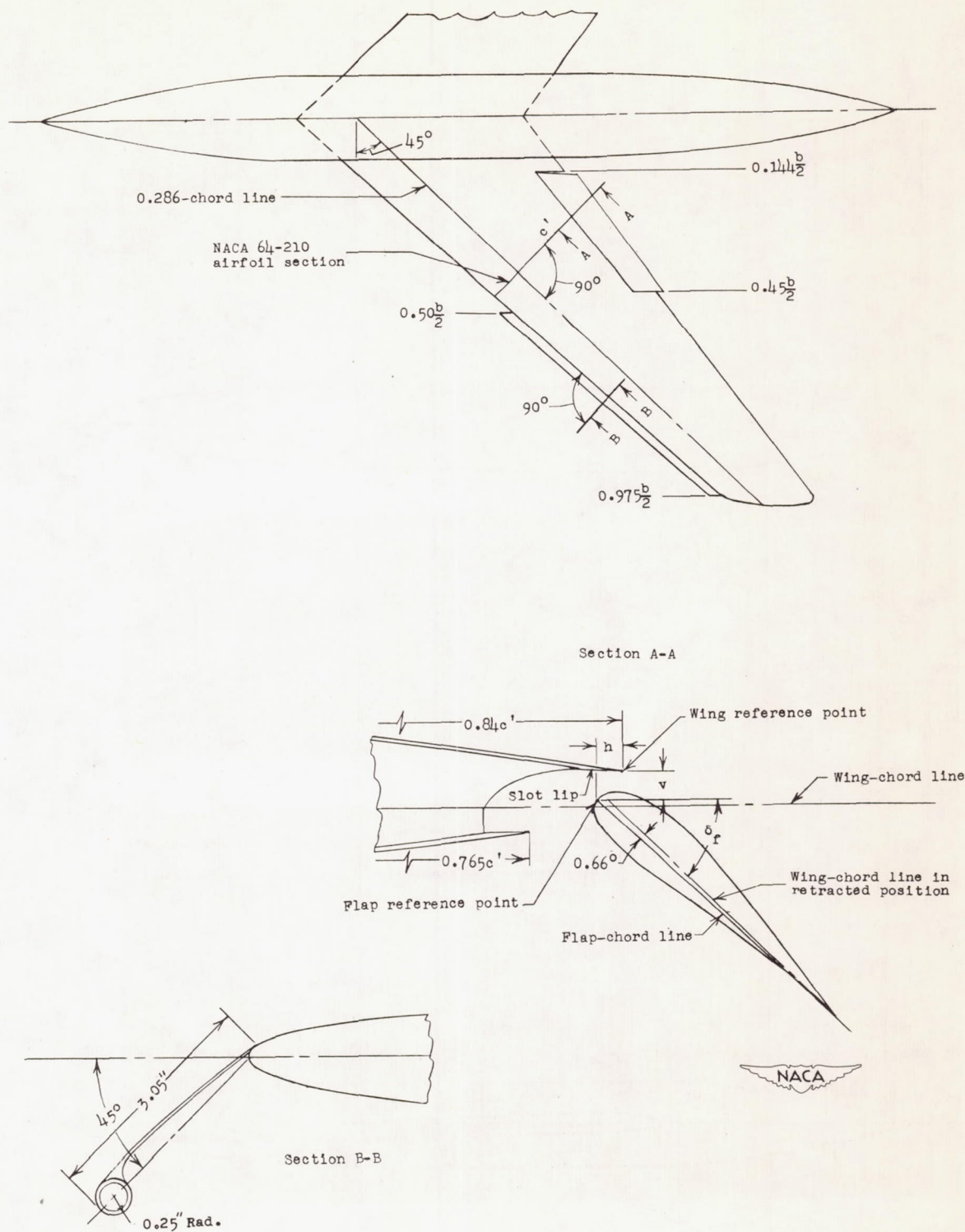
Figure 2.- Details of leading-edge and trailing-edge flaps.
