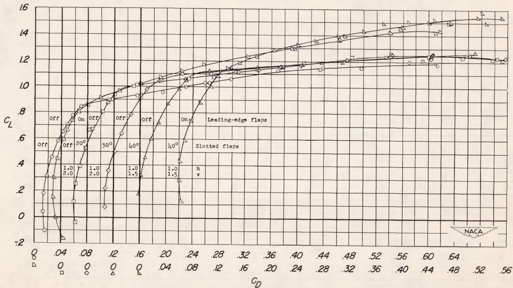
(b) C_L against C_D .
