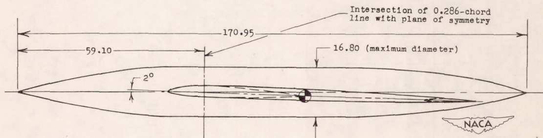
Figure 1.- Geometry of the 47.7° sweptback-wing - fuselage combination. All dimensions are in inches.
