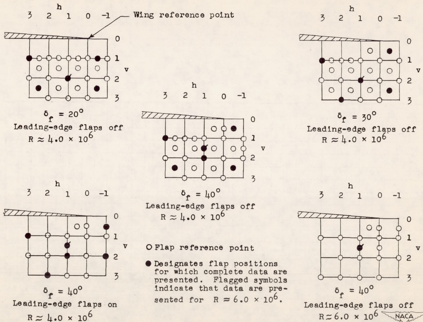
Figure 4.- Index of flap positions investigated.
