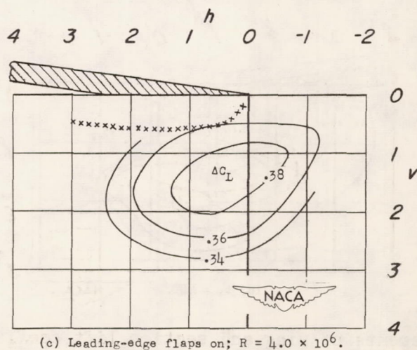
Figure 10.- Increments of wing lift coefficient at various positions of the single slotted flaps. \delta_f = 40^\circ .
