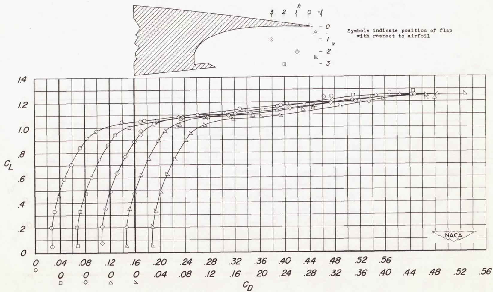
(b) C_L against C_D .
