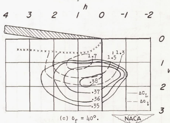
Figure 9.- Increments of wing and section lift coefficient at various positions of the single slotted flaps. Leading-edge flaps off; R = 4.0 \times 10^6 .
