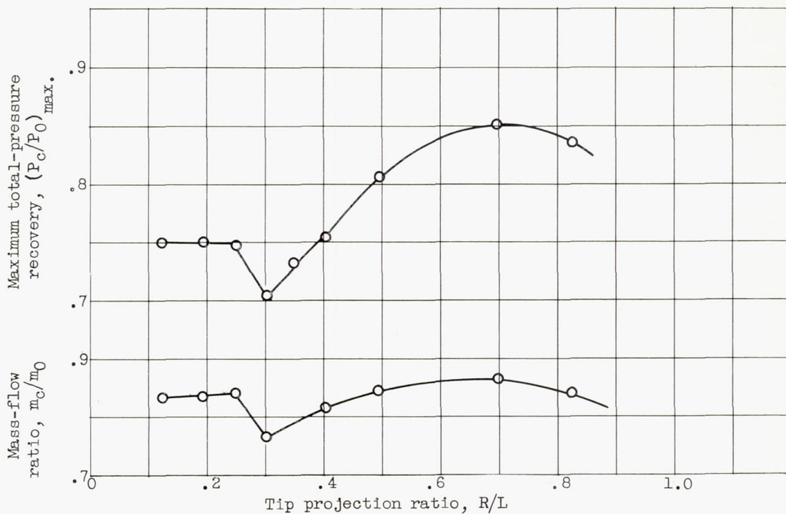
(a) Maximum total-pressure recovery and corresponding mass-flow ratio as function of tip projection.
