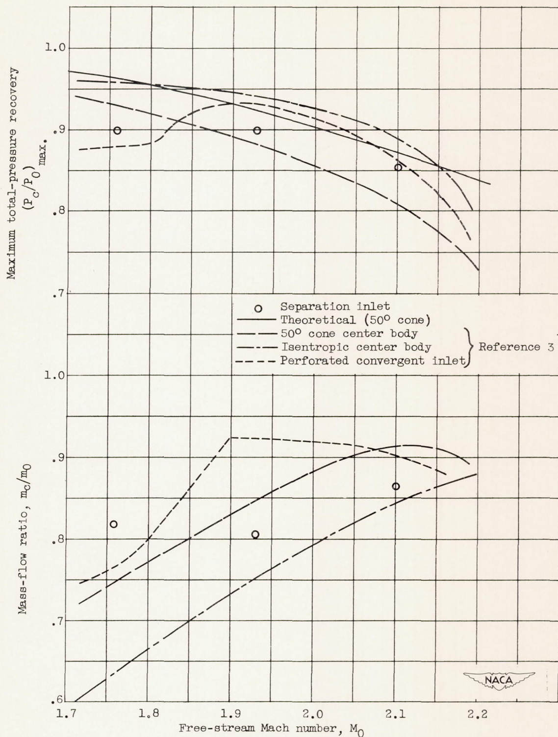
Figure 9. - Maximum total-pressure recovery and corresponding mass-flow ratio for separation inlet and several solid-body inlets.
