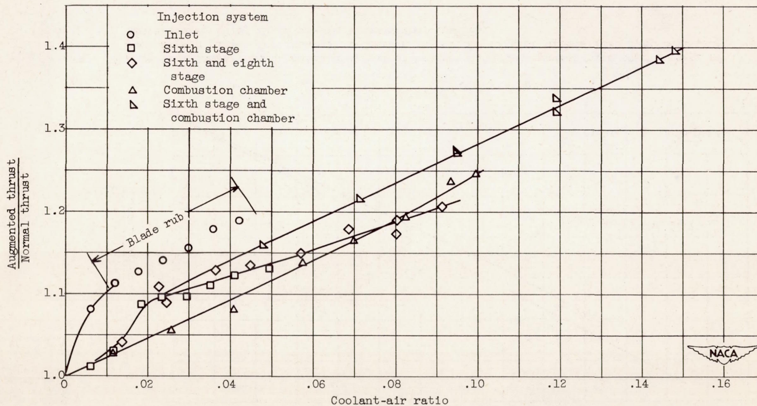
Figure 6. - Variation of ratio of augmented to normal thrust with coolant-air ratio for various injection systems. Engine speed, 7890 rpm; tail-pipe temperature, 1275° F; inlet-air temperature, 100° F.
