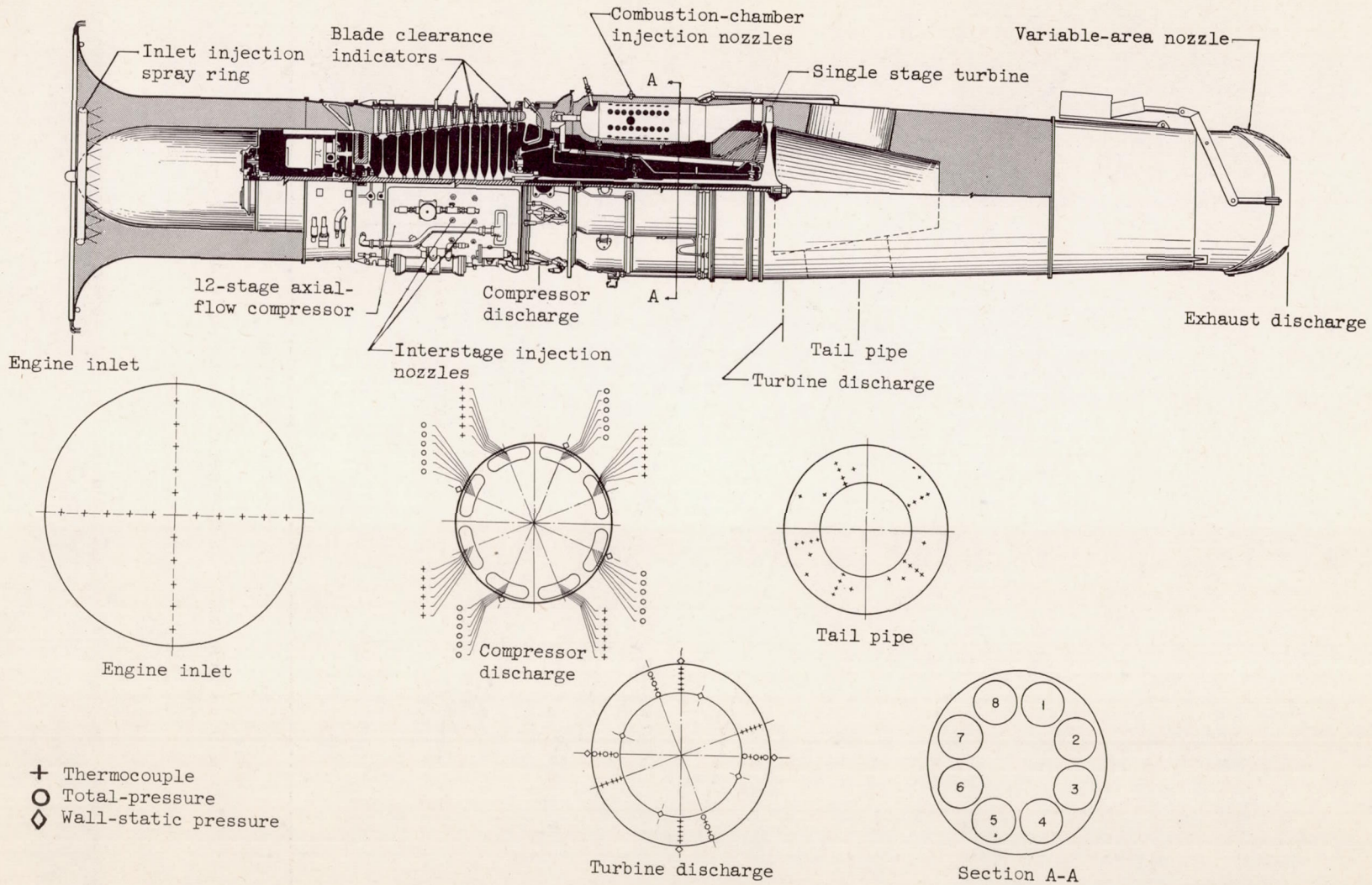
Figure 4. - Engine instrumentation.
