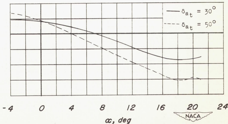
(d) Fuselage on, \delta_f = 50^\circ ( 0.35b flap), \delta_n = 30^\circ , 0.40b/2 aileron, t = 0 .
