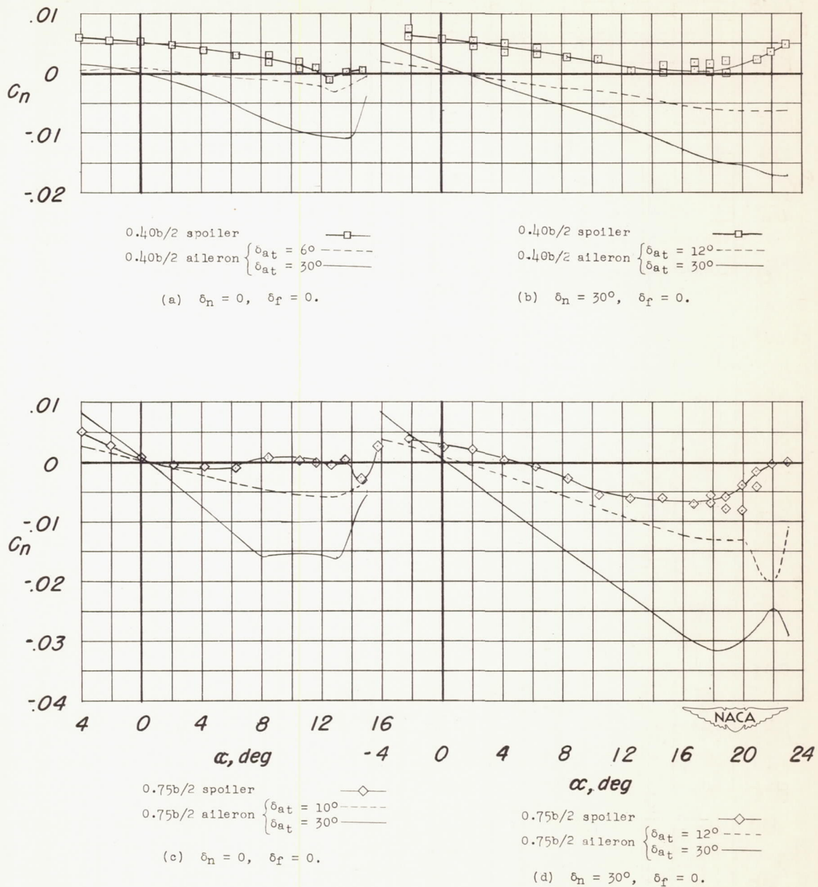
Figure 22.- Comparison of spoiler and aileron yawing-moment coefficients for various configurations. Fuselage on, t = 0 .
