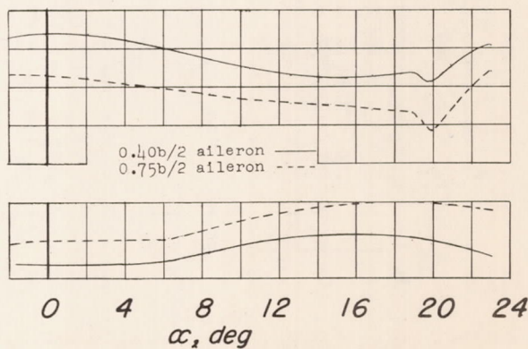
(e) Effect of aileron span; fuselage on, t = 0 , 0.005c vent, \delta_f = 0 , \delta_n = 30^\circ .
