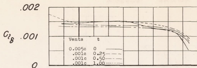
(a) Effect of blunt ailerons; plain wing, 0.40b/2 ailerons.
