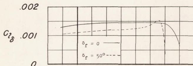
(c) Effect of 0.35b flap; fuselage on, 0.40b/2 aileron, t = 0 , 0.005c vent, \delta_n = 0 .
