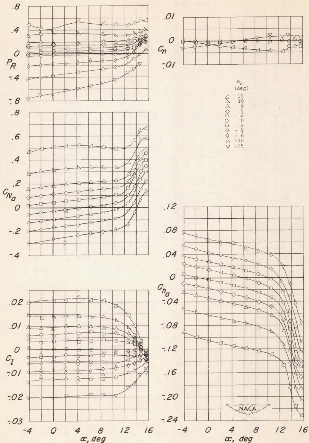
Figure 7.- Variation of P_R , C_{N_a} , C_l , C_n , and C_{h_a} with \alpha ; plain wing, 0.40b/2 aileron, t = 0.25 , 0.00lc vent, \delta_f = 0 , \delta_n = 0 .
