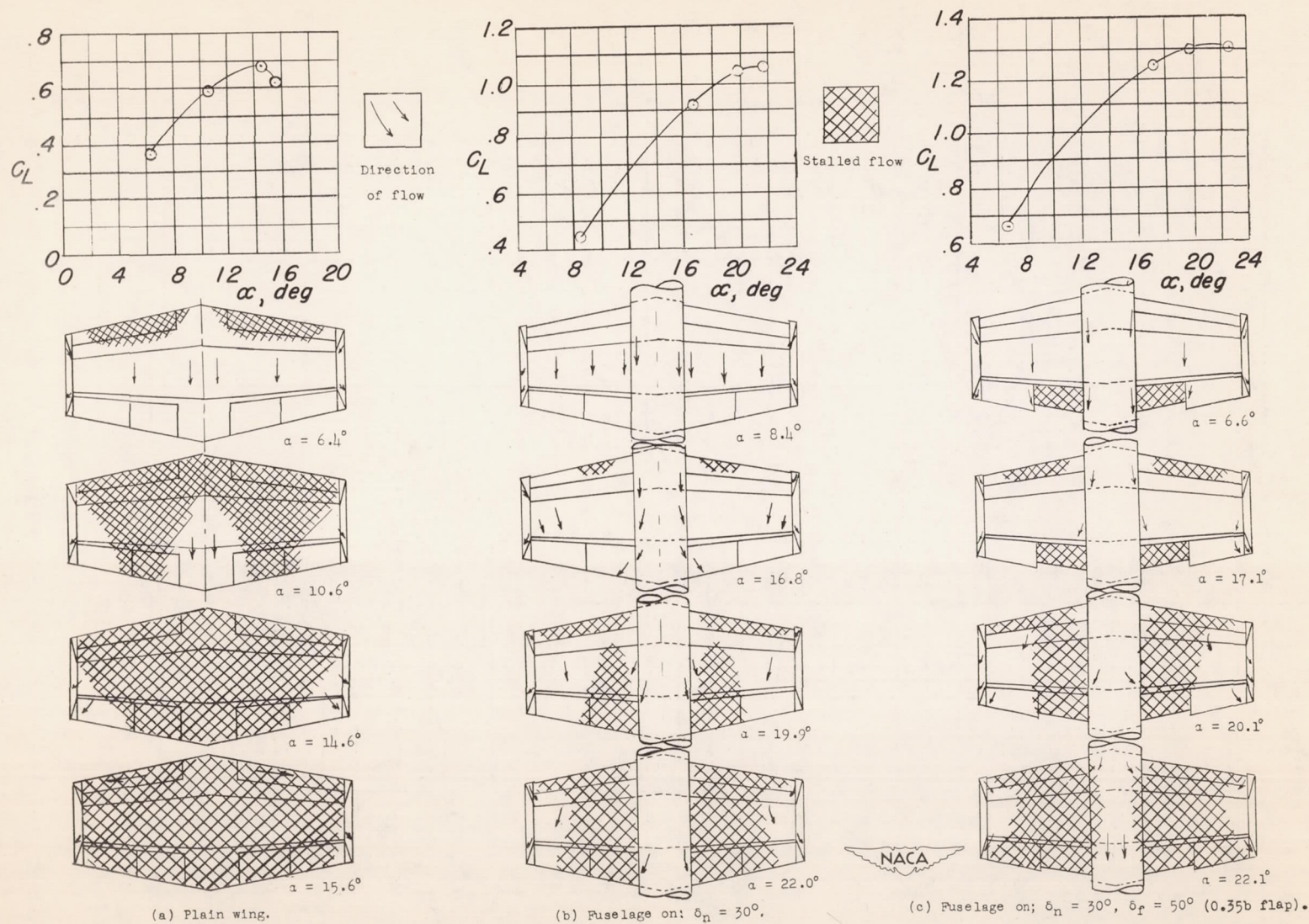
Figure 5.- Stalling patterns of the hexagonal wing model with and without a fuselage and deflected flaps.
