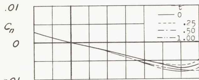
(a) Plain wing, blunt ailerons ( 0.40b/2 ).
