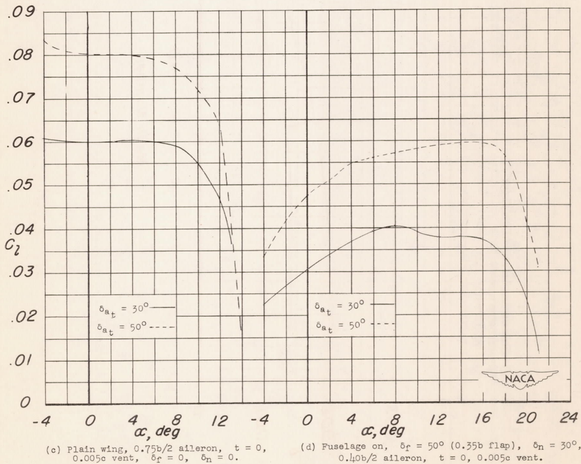
Figure 19.- Rolling-moment coefficients for total aileron deflections of 30^\circ and 50^\circ .
