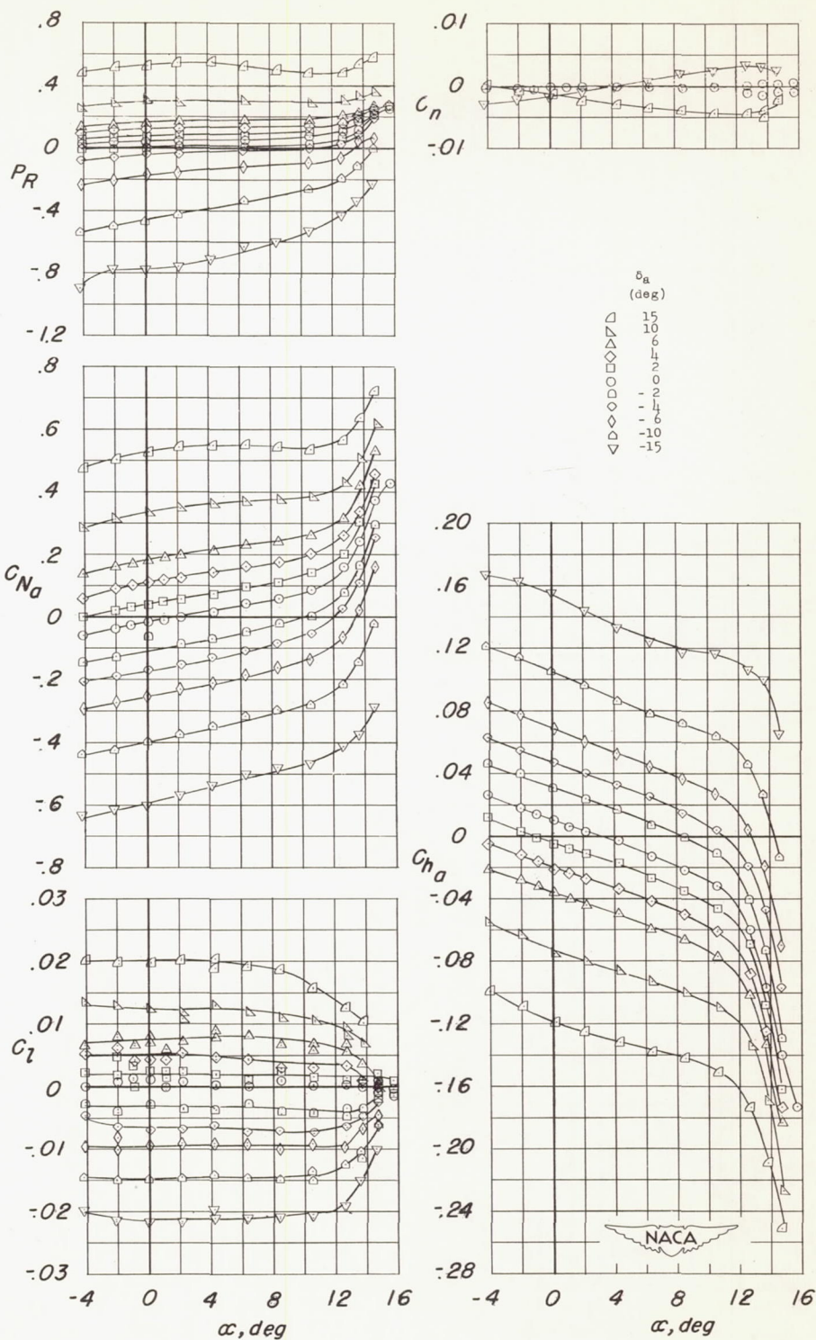
Figure 8.- Variation of P_R , C_{N\alpha} , C_l , C_n , and C_{ha} with \alpha ; plain wing, 0.40b/2 aileron, t = 0.50 , 0.001c vent, \delta_f = 0 , \delta_n = 0 .
