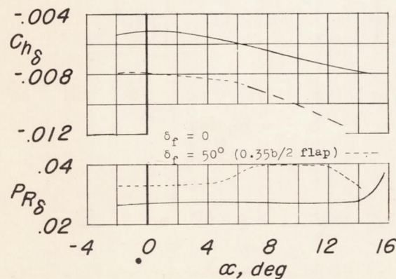
(c) Effect of 0.35b flap; fuselage on, 0.40b/2 aileron, t = 0 , 0.005c.
