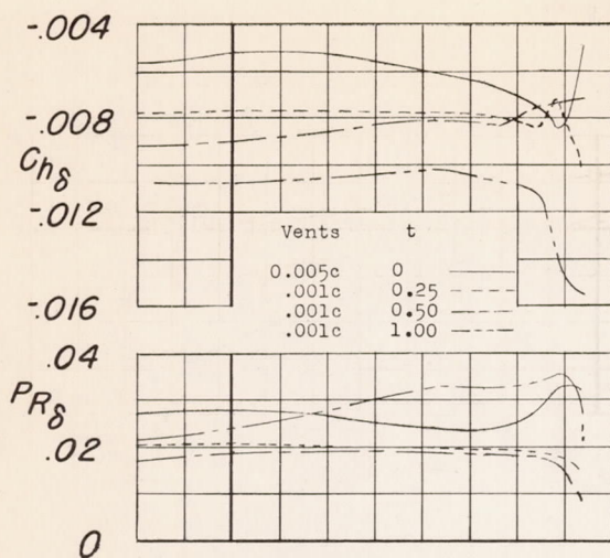
(a) Effect of blunt ailerons; plain wing, 0.40b/2 ailerons.
