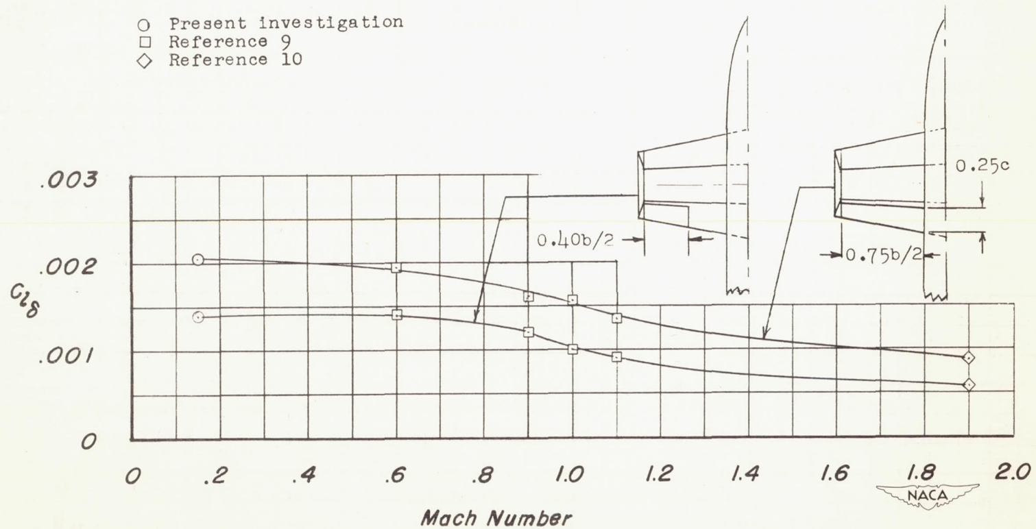
Figure 18.- Variation of aileron effectiveness parameter C_{l\delta} with Mach number. Reynolds number varies from 10^6 to 7.6 \times 10^6 .
