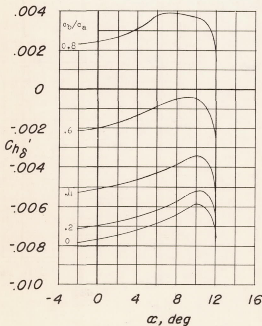
\delta_n = 0 , fuselage on, 0.40b/2 aileron, \delta_r = 50^\circ (0.35b flap)
