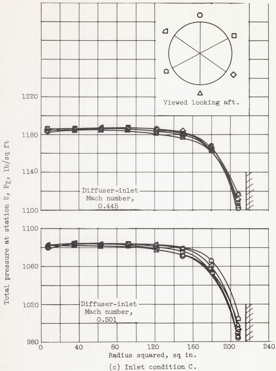
Figure 10. - Concluded. Diffuser-inlet total-pressure profiles. (Station 2.)
