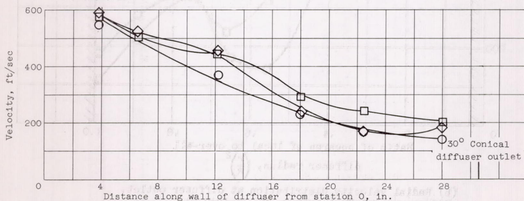
(c) Longitudinal velocity distribution along wall of diffuser. Diffuser-inlet Mach number, M_2 , 0.46 \pm 0.01 .
