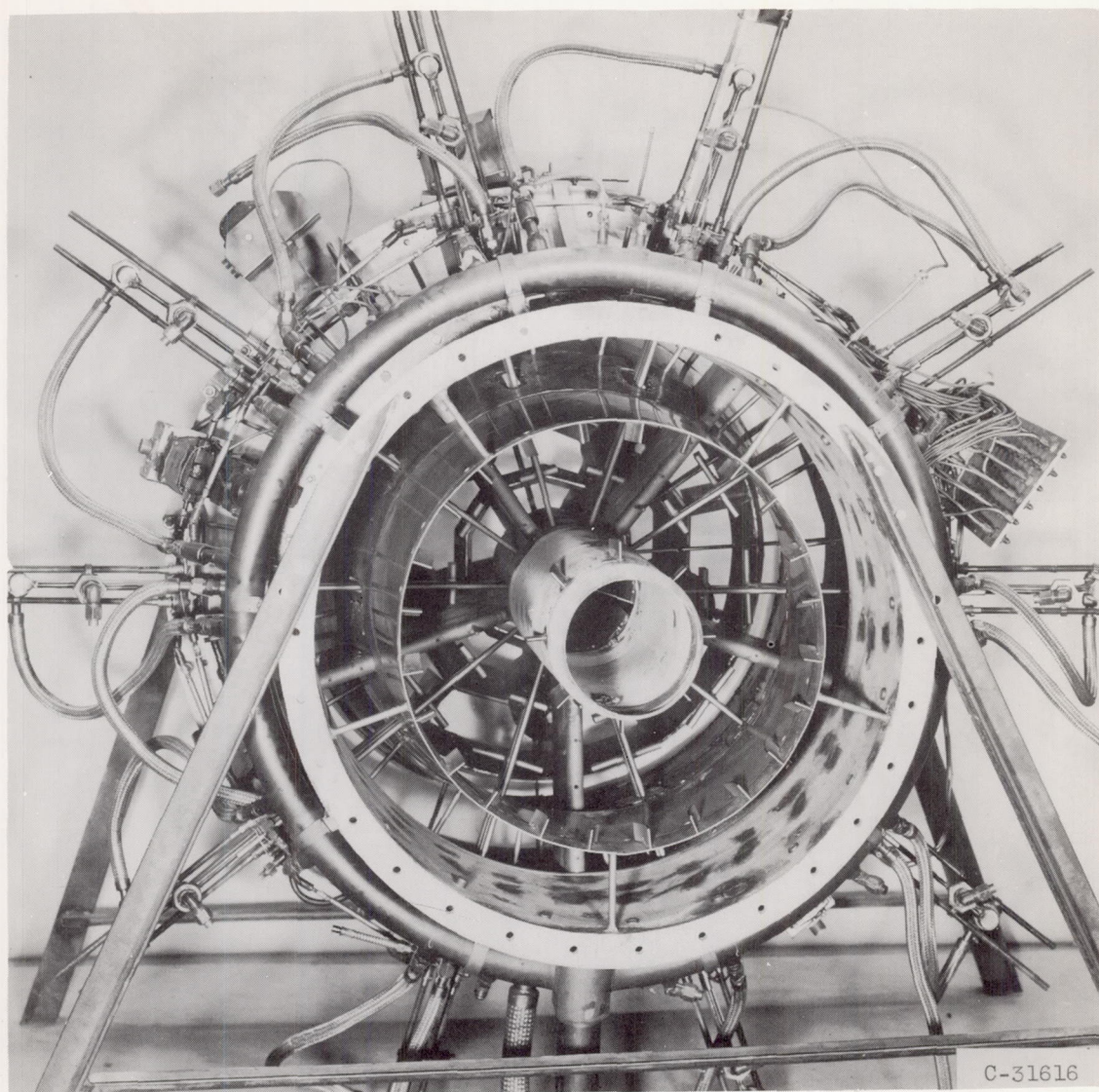
(b) Typical installation (upstream view).
