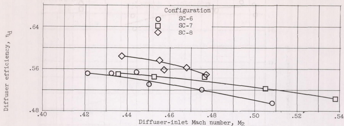
(a) Variation of diffuser efficiency with diffuser-inlet Mach number.
