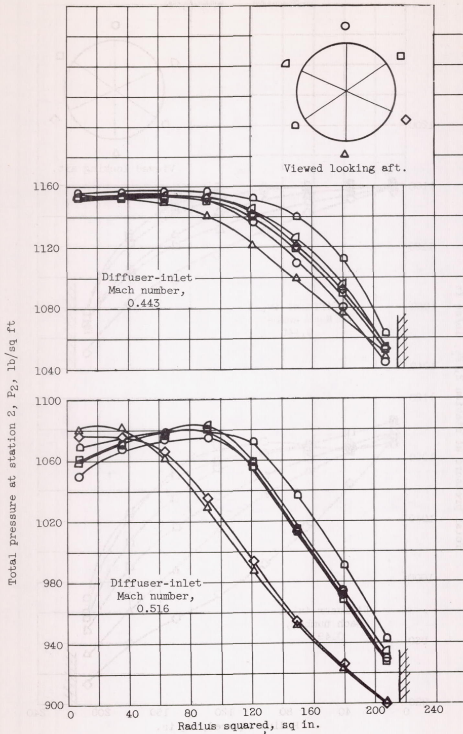
Figure 10. - Continued. Diffuser-inlet total-pressure profiles. (Station 2.)
