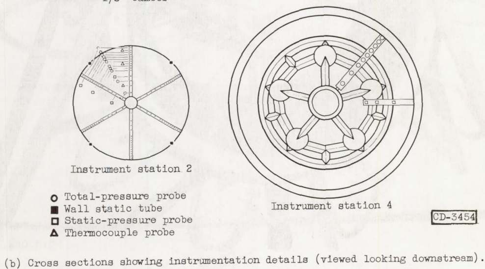
Figure 4. - Engine modifications and diffuser instrumentation.
