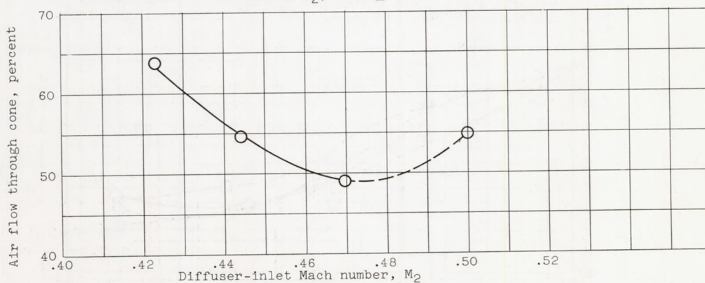
(c) Effect of diffuser-inlet Mach number on air flow through splitter cone.
