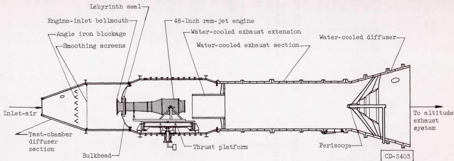
Figure 1. - 48-Inch ram-jet engine in 14-foot-diameter altitude chamber.
