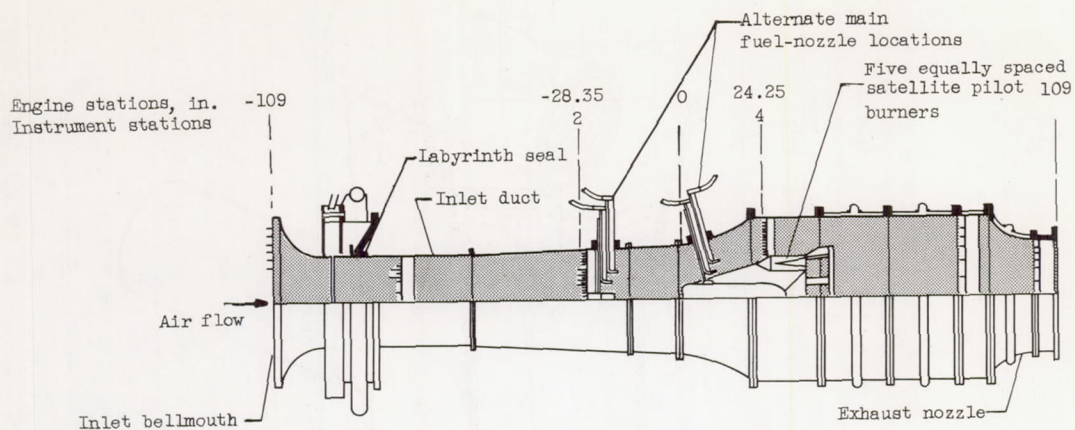
(a) Engine with inlet ducting.
