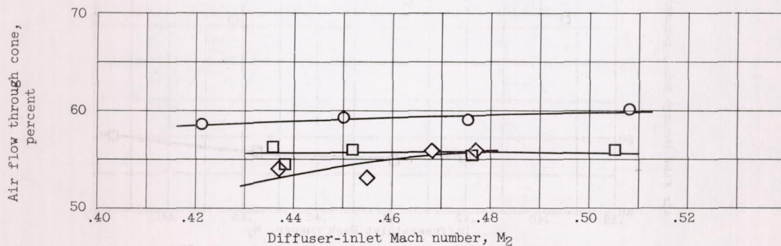
(c) Effect of diffuser-inlet Mach number on air flow through splitter cone.
