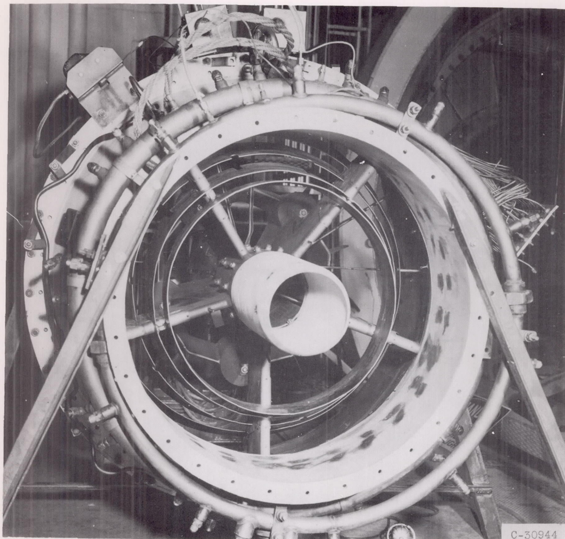
(c) Typical installation (upstream view).
