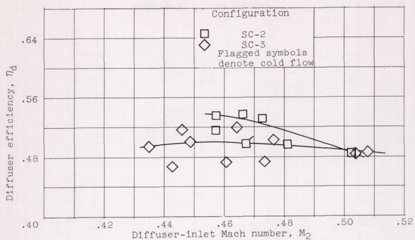
(a) Variation of diffuser efficiency with diffuser-inlet Mach number.
