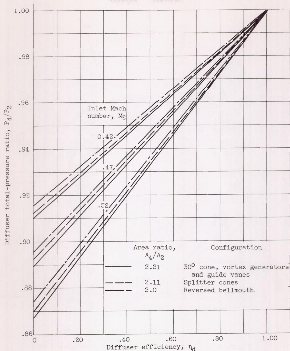
Figure 9. - Variation of diffuser total-pressure ratio with diffuser efficiency for various diffuser Mach numbers and area ratios.
