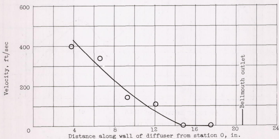
(c) Longitudinal velocity distribution along wall of diffuser. Diffuser-inlet Mach number, M_2 , 0.46 \pm 0.01 .
