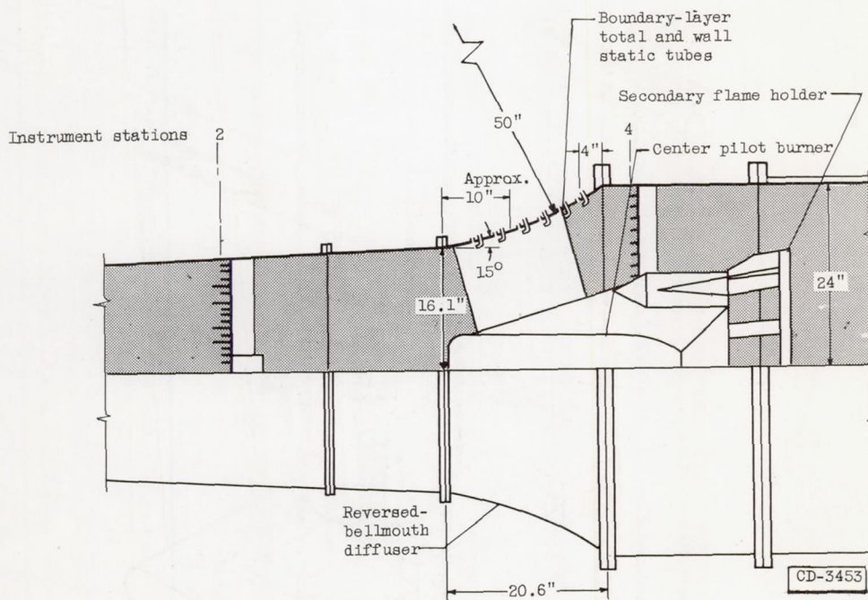
(b) Diffuser section showing flame holder and instrumentation.
