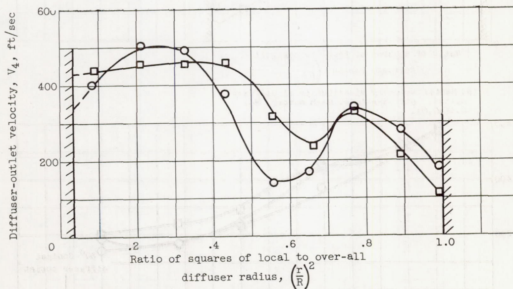
(b) Radial velocity distribution at diffuser outlet. Diffuser-inlet Mach number, M_2 , 0.46 \pm 0.01 .
