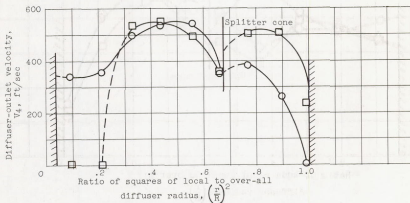
(b) Radial velocity distribution at diffuser outlet. Diffuser-inlet Mach number, M_2 , 0.46 \pm 0.01 .
