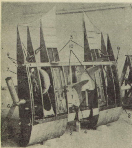
Figure 11.-The center section is built as a separate unit. 1, An adjustable seat sliding on runners. 2, The starboard wing fuel tank. 3, Small lockers for tools and log books. 4, A control column, working the push rods which leave the wing at 5, where they end in rubber buffers. 6, The elbow joint upon which the wing folds. 7, A landing gear wheel retracted. 8 and 9, The wing root spar bolts. 10, The center attachment point of the fuselage. "Flight"
