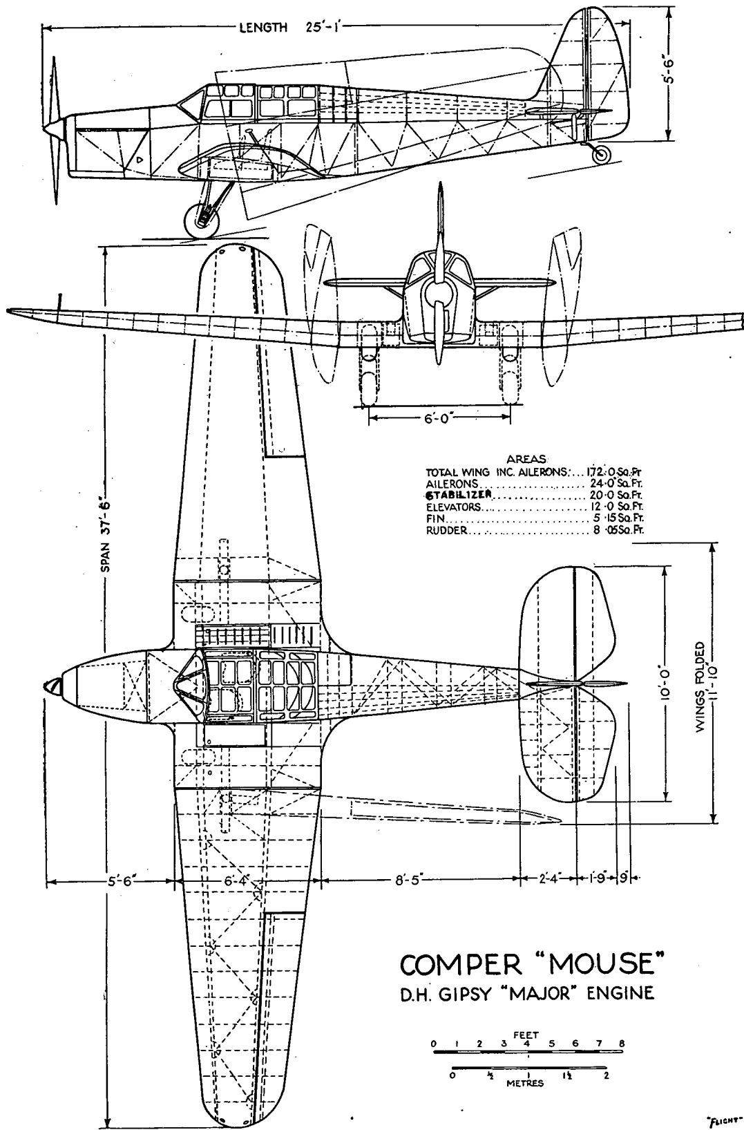
Fig.1-General arrangement drawings of the Comper "Mouse" airplane.
