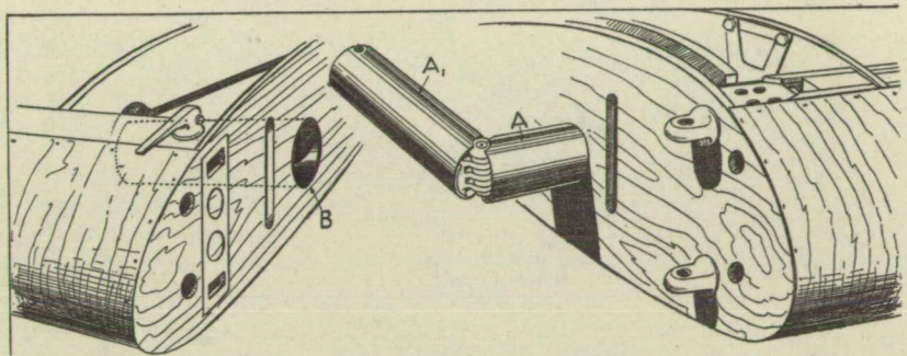
Figure 9.—These three sketches show how the wing folds. The jointed tube A is anchored in the center section and passes through the tube B. "Flight"
