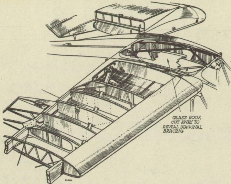
Figure 3.-The wings and center section of the D.H.85 Leopard Moth airplane
