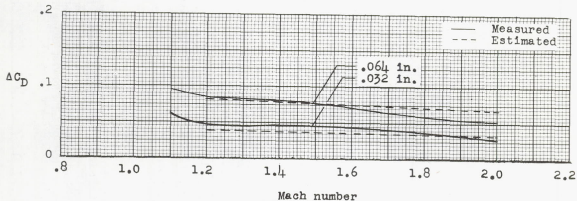
(a) Forward-facing lap joints.
