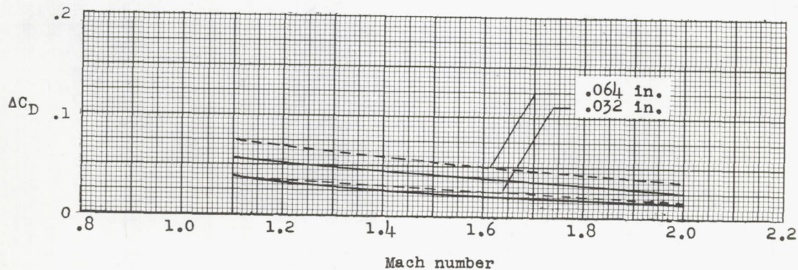
(b) Backward-facing lap joints.
