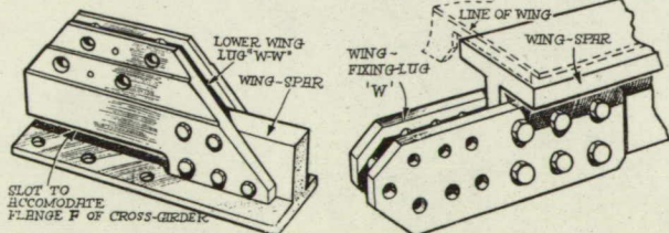
Figures 6 and 7.- Details and assembly of portions of wing structure of the Empire flying boat.
