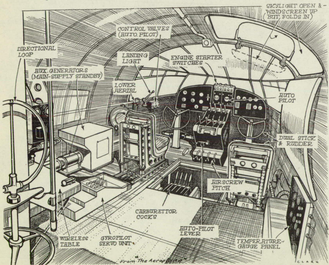
Figure 15.- The Pilots' cabin or the "Captains Bridge" on the Empire
