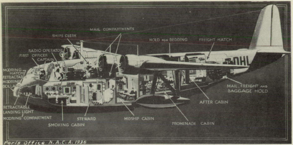
Figure 10.- Short Empire Boat (internal arrangements)
