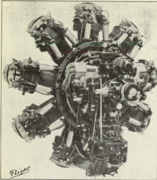
Figure 13.- The Pegasus Xc radial engine. More than 3600 hp. is delivered by four of these engines, to the finely pitched blades of the D.H. variable-pitch propeller, in the take-off.
