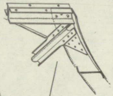
Figures 4, 5.- Details of hull and step of the Empire flying boat.
