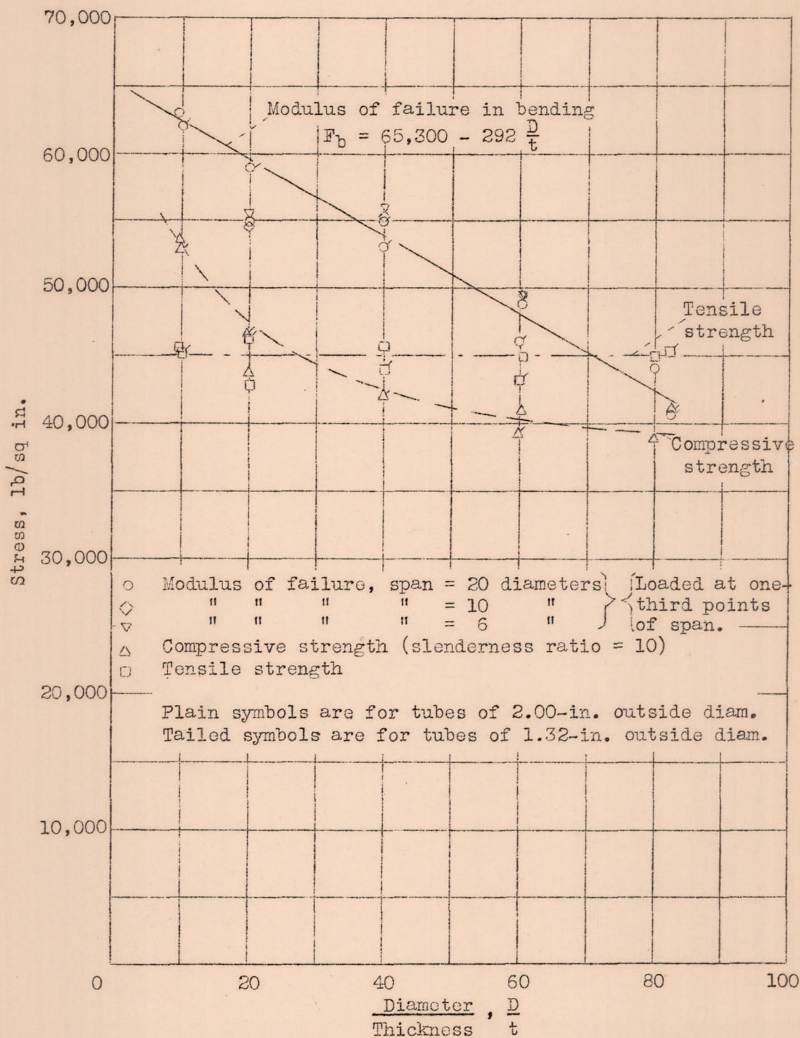
Figure 2.- Modulus of failure in bending and the mechanical properties of 6LS-T round tubing. Beams loaded at one-third points of span.
