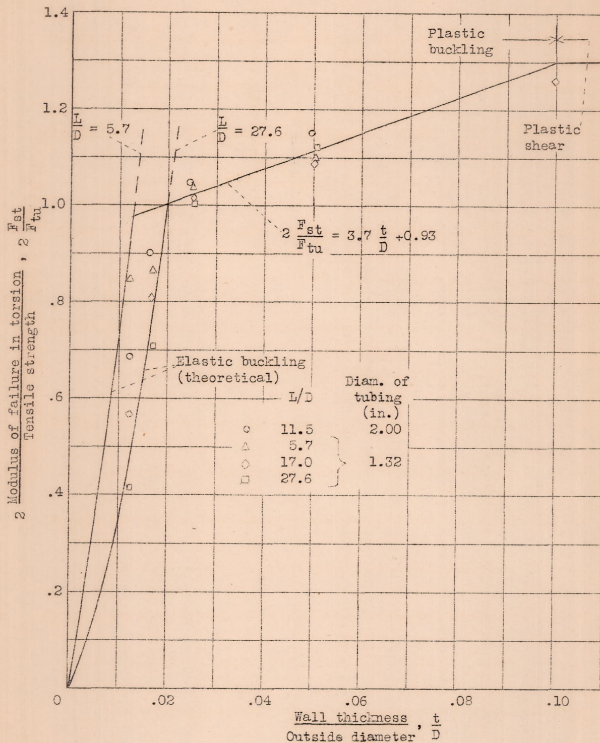
Figure 5.- Modulus of failure in torsion for aluminum-alloy round tubing.
