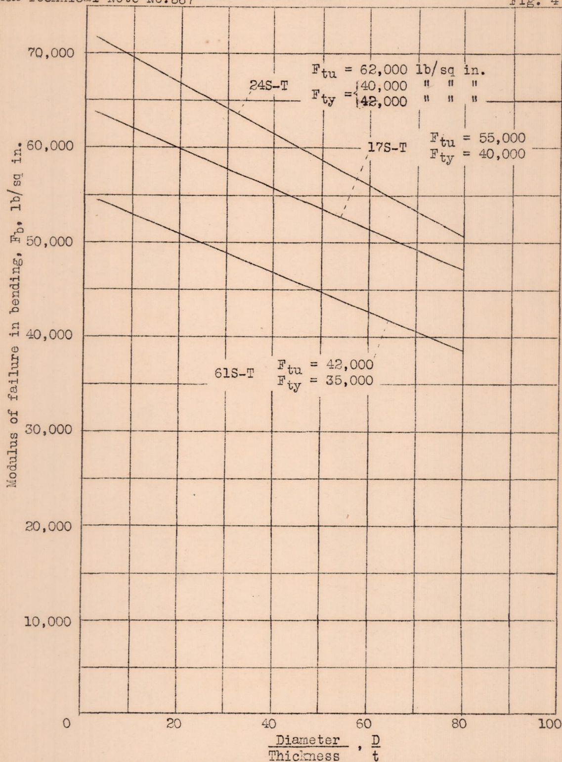
Figure 4.- Modulus of failure in bending of aluminum-alloy round tubing. Beams loaded at one-third points of span; tubes supported against local failure at loading points. (Data for 17S-T and 24S-T tubing are taken from fig. 5-6 of reference 1.)
