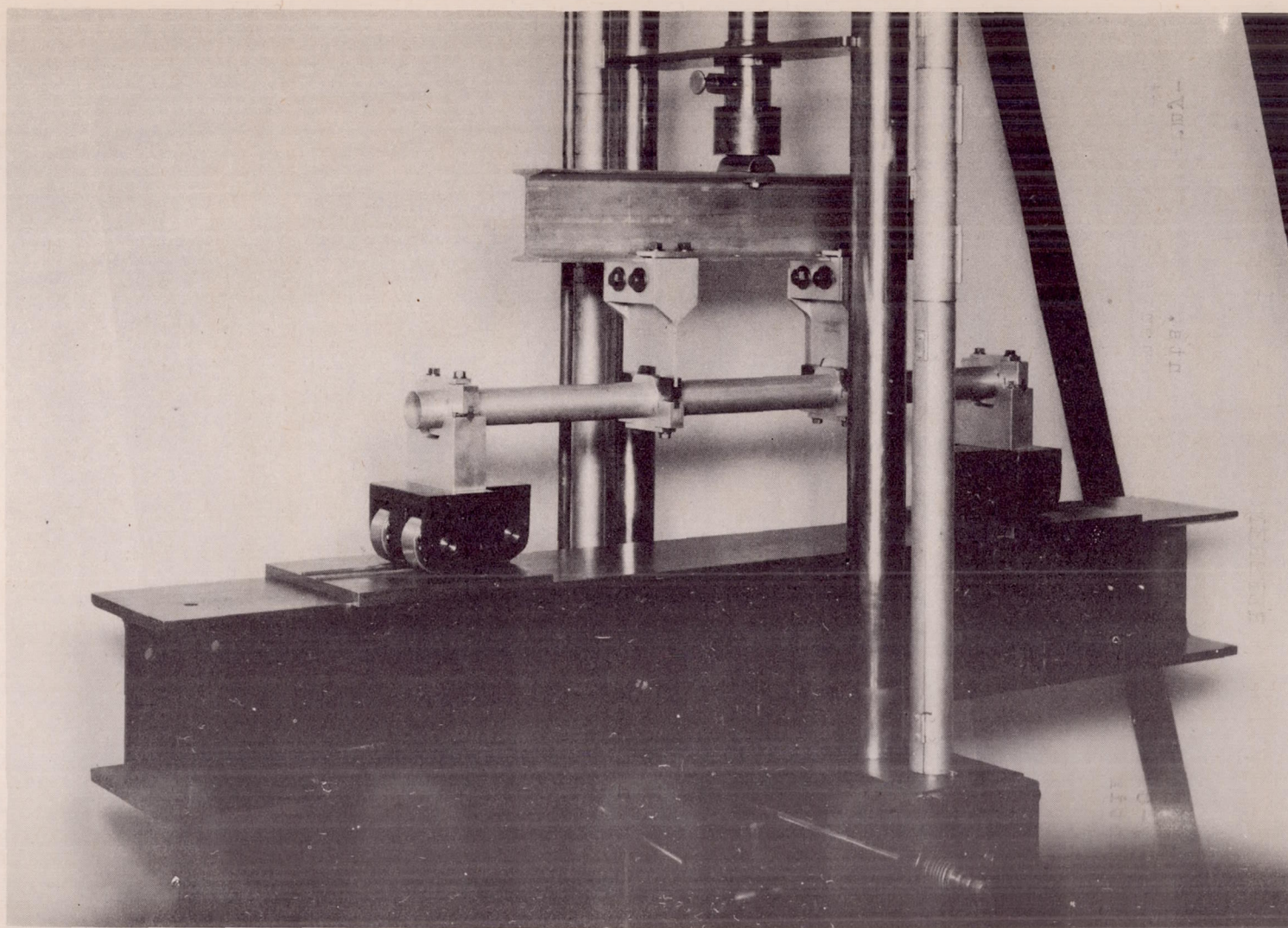
Figure 1.- Method of loading beam specimens on the neutral axis at the one-third points of the span.
