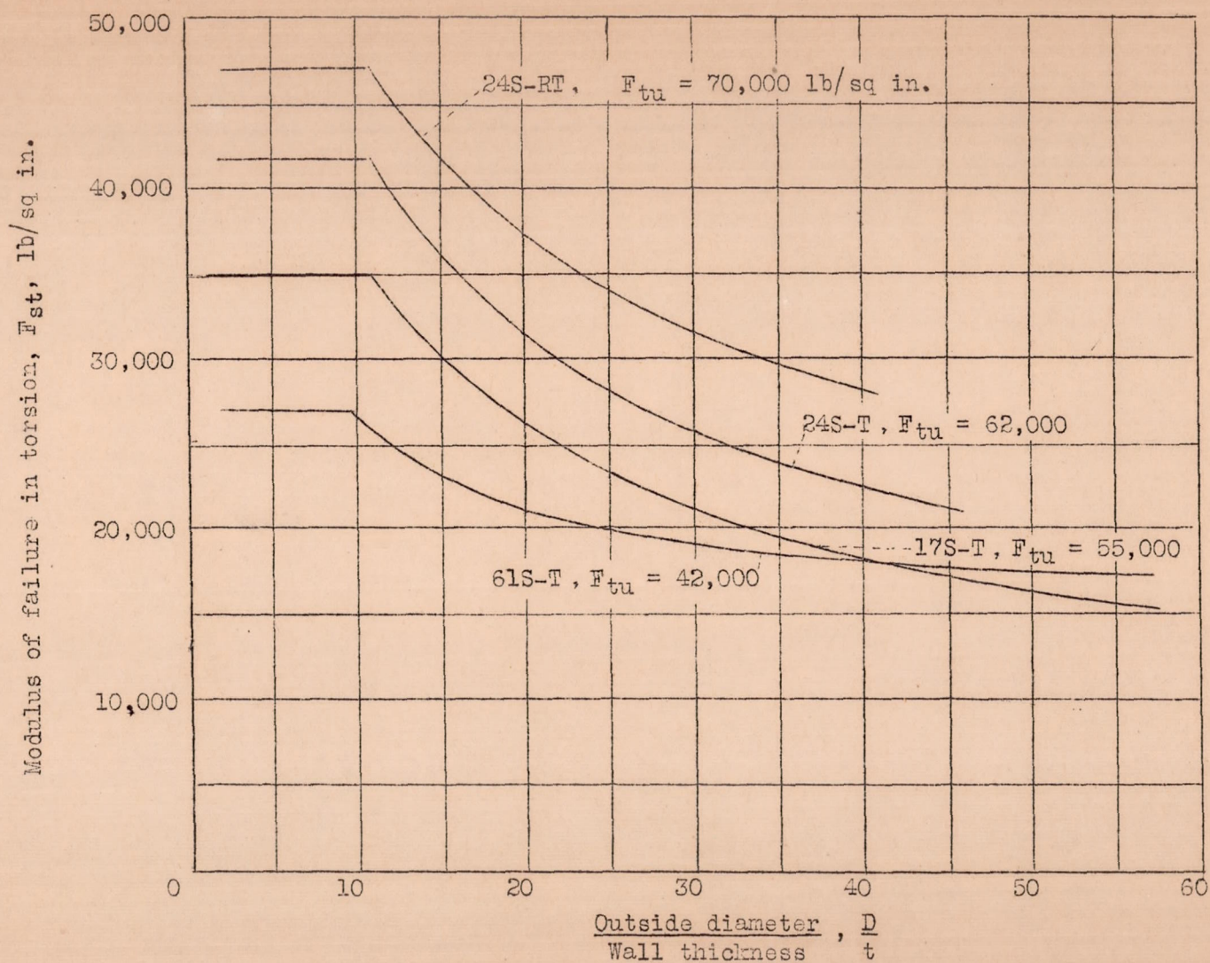
Figure 8.-- Moduli of failure in torsion against D/t ratios for aluminum-alloy round tubing. (Curves for 24S-RT, 24S-T, and 17S-T tubings are taken from fig. 5-7 of ref. 1.)
