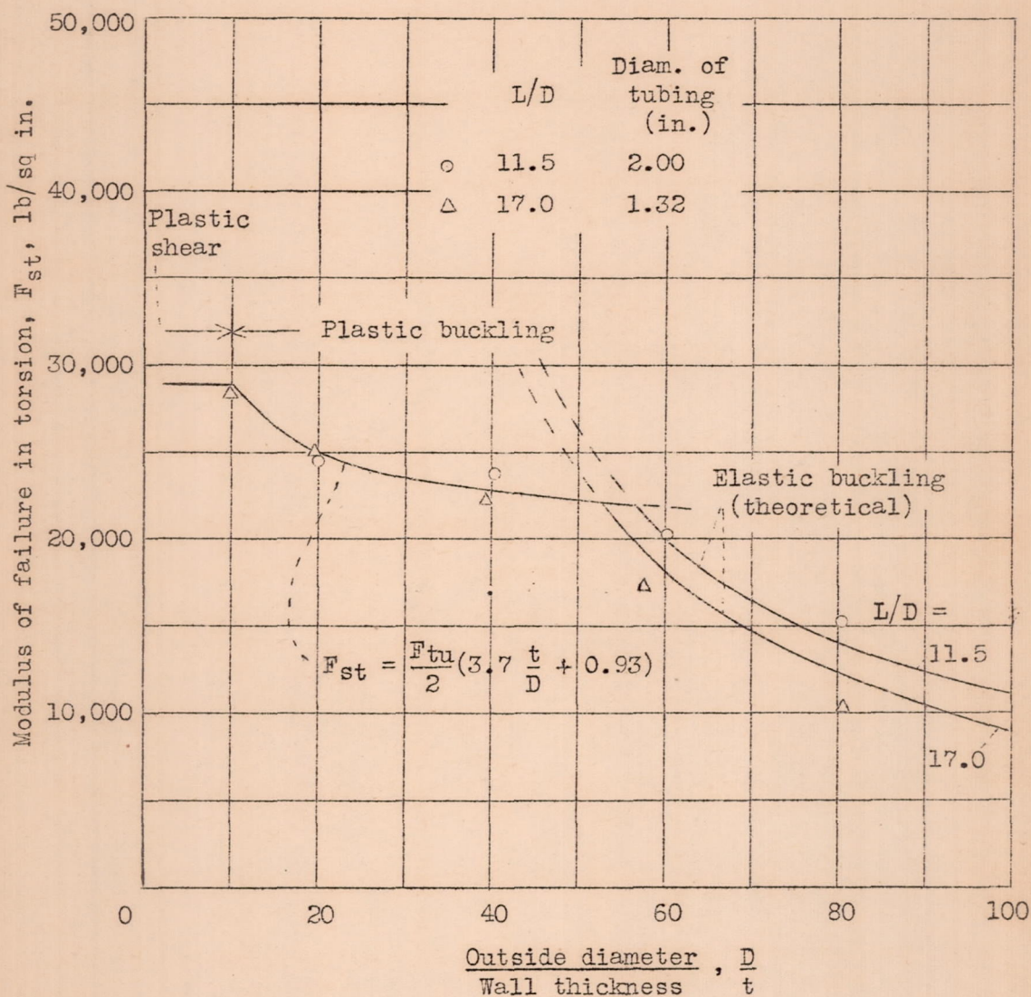
Figure 7.- Moduli of failure in torsion against D/t ratios for aluminum-alloy round tubing.
