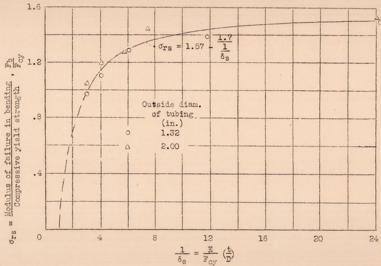
Figure 3.- Modulus of failure data from beam tests.
