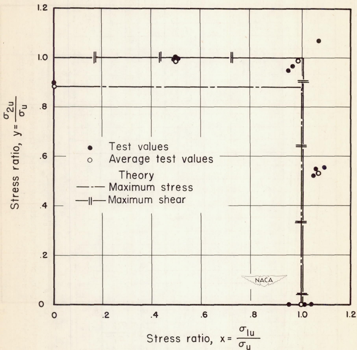
Figure 11.- Comparison of nominal biaxial ultimate stresses with values from maximum-stress theory.
