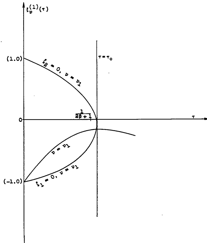
Figure 16.- The behavior of the integral-curve; i_v^{(1)}(\tau) .
