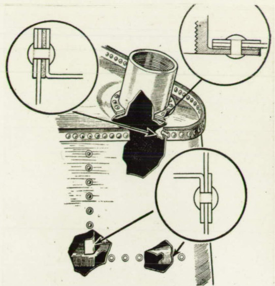
Fig. 7 Poite riveted duralumin fuel tank. Upper left, Top and bottom joints: sheet of varnished paper between the end and an exterior reinforcing strip of duralumin. Upper right, Attachment of cocks, necks, outlets, etc: interposed paper ring and duralumin reinforcing ring. Below, Attachment of partitions, each rivet provided with a washer. Rivets very close. Thickness of walls exaggerated for sake of clearness.
