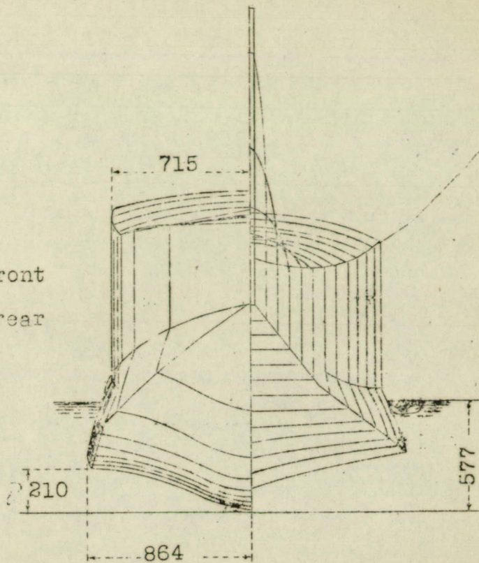
Fig. 4 Hull lines of LeO 194.
