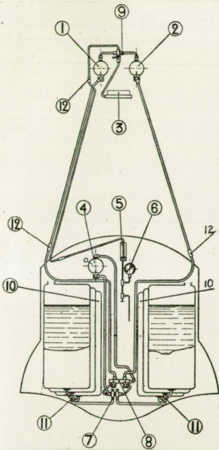
Fig. 6 Liore- Jupiter Fuel system. 1, 2 Self- regulating pump; 3, Car- buretor of 420 HP eng., "Jupiter"; 4, Hand pump; 5, Damper with plunging tube; 6, Fuel-pres- sure gauge; 7, Simple mani- fold with 2 cocks and 3 connections; 8, Manifold with 2 flap valves; 9, Cocks 1/4 turn with 4 branch- es; 10, Fuel tanks; 11, Cross branches; 12, Flexible metal connections
