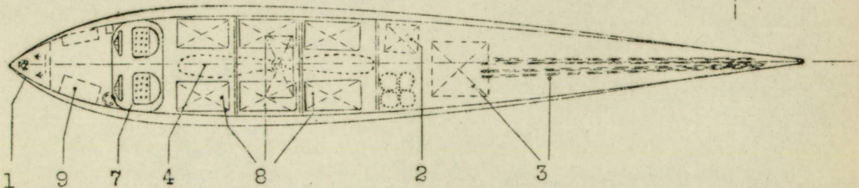
Fig. 5 Hull of LeO 194 - Left, section through pilot cockpit. Right, section through tanks. Bottom, plan view of hull.
