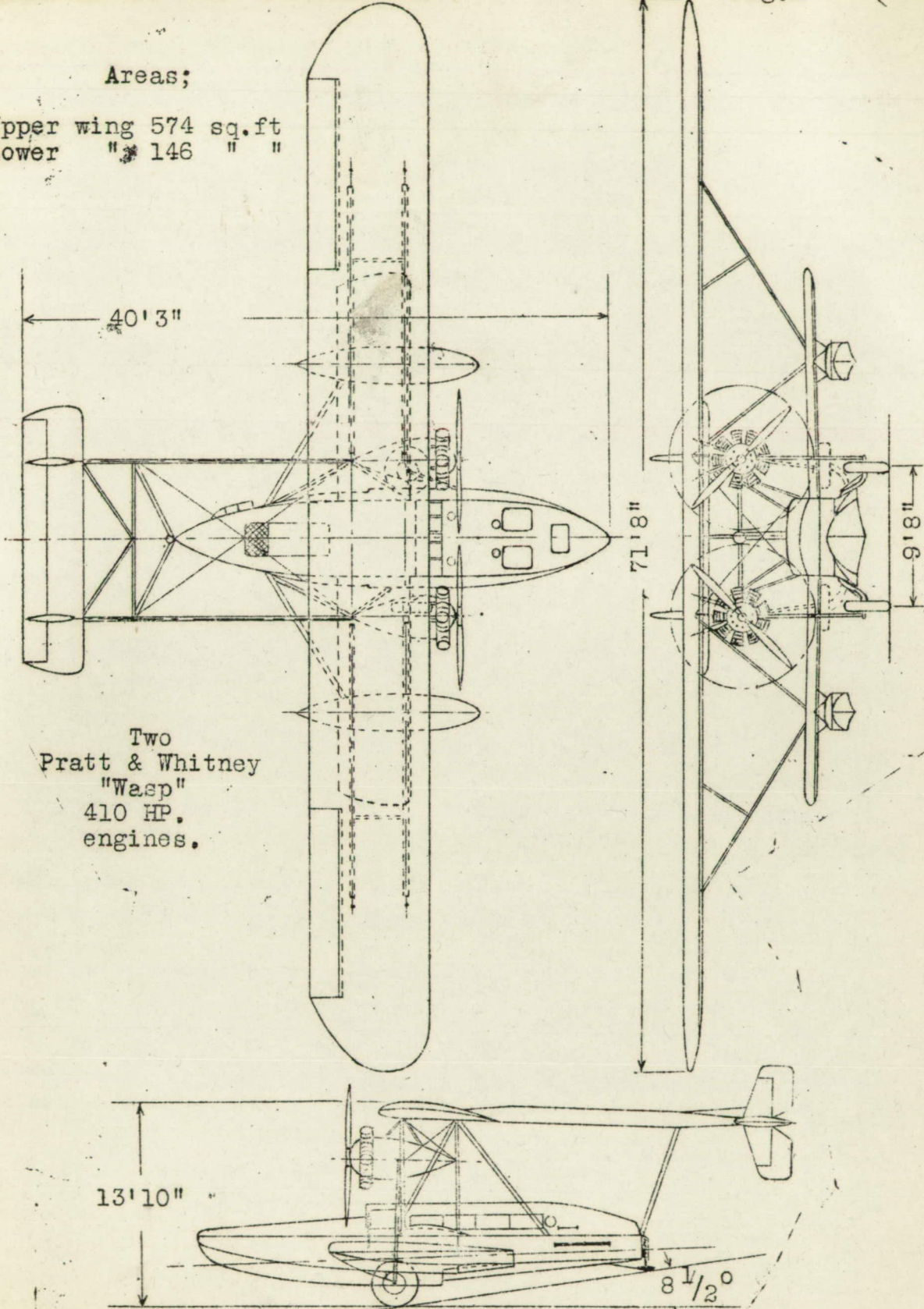
Fig.1 Sikorsky twin-motor amphibian flying boat Model 1928.
