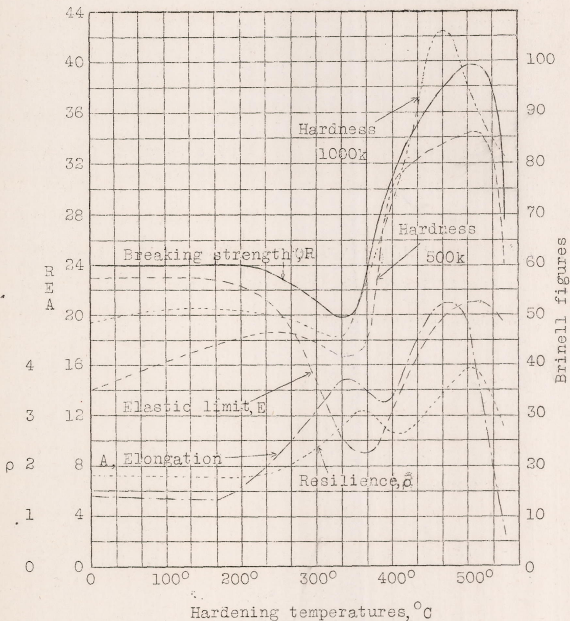
Fig.1 Variations in the mechanical properties of Duralumin plotted against the temperatures of hardening.
