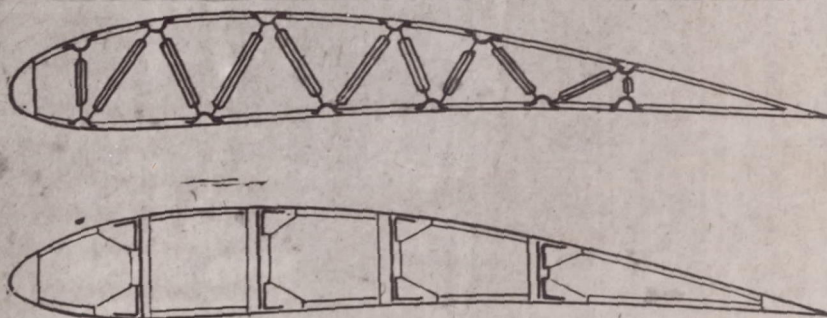
Fig.11 Wings with multiple spars (Dyle & Bacalan).
