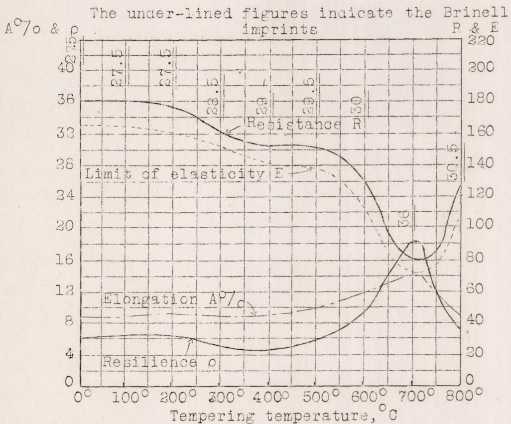
Fig.4 Holtzer steel CN 12, hardened in air at 950°C. Variation of mechanical characteristics plotted against the tempering temperatures.
