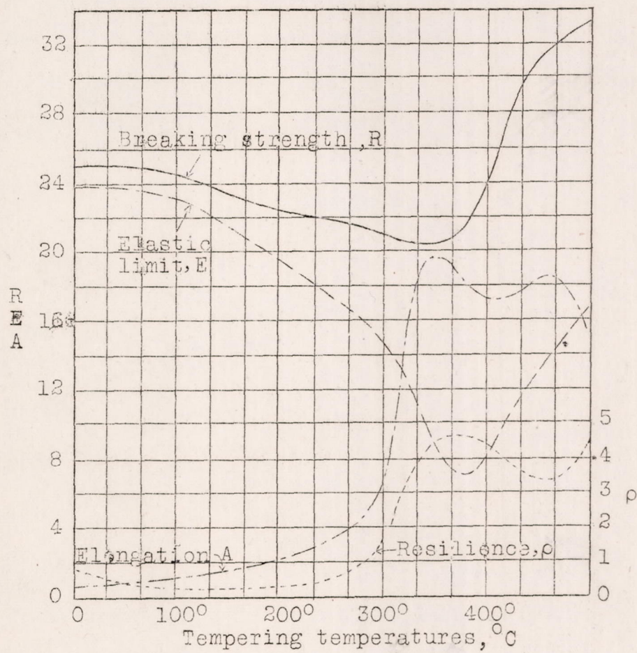
Fig.2 Variation in the mechanical properties of Duralumin plotted against the tempering temperatures.
