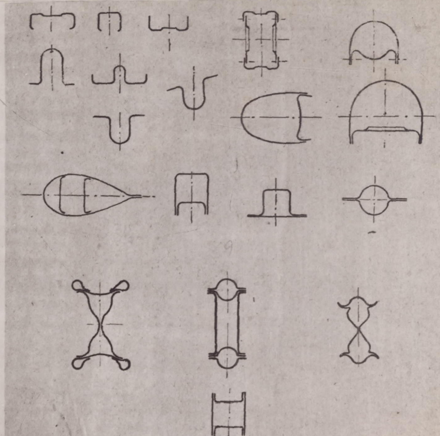
Fig.9 Various structural sections (Dornier, British, Dyle and Bacalan).
