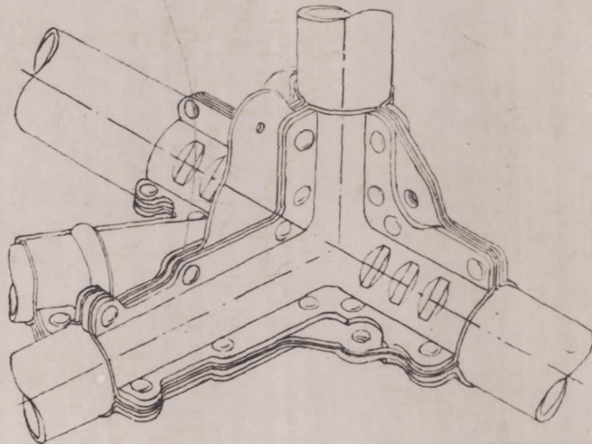
Fig.5 S.E.C.M. assembly by stamped pieces.
