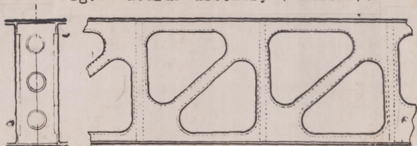
Fig.8 Open-work steel box-spar (Dyle & Bacalan airplane).
