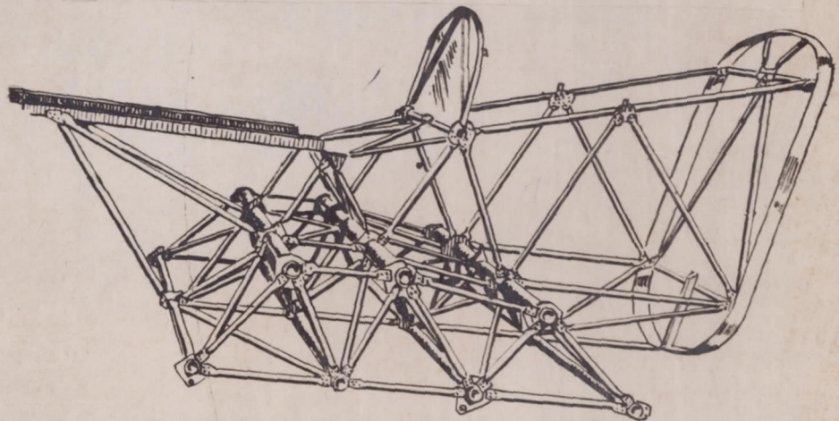
Fig.7 Tubular assembly (Junkers).
