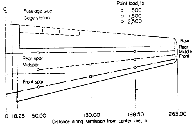
FIGURE 4.—Loading points for structure A.
