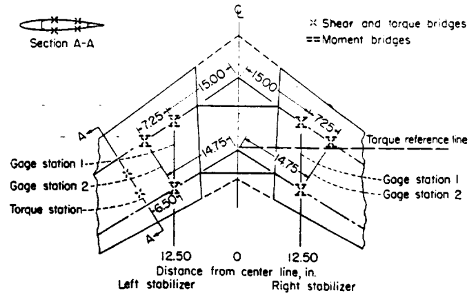
FIGURE 3.—Strain-gauge bridge locations for structure B. (All dimensions are in inches.)
