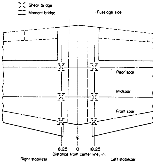
FIGURE 2.—Strain-gauge bridge locations for structure A.
