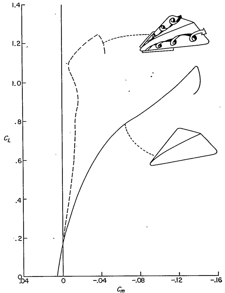
FIGURE 9.—An example of the reduction of the longitudinal stability and out-of-trim pitching moment of a delta wing ( \Delta_{LE} = 60^\circ ) by the leading-edge vortex flow resulting from leading-edge separation. (Data obtained from ref. 56.)
