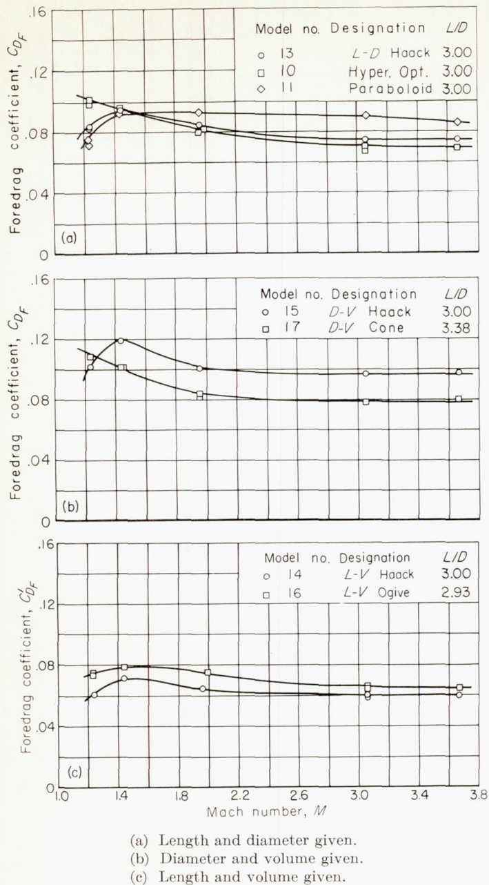
FIGURE 12.—Comparison of foredrag of Haack models with other models having the same two specified parameters.
