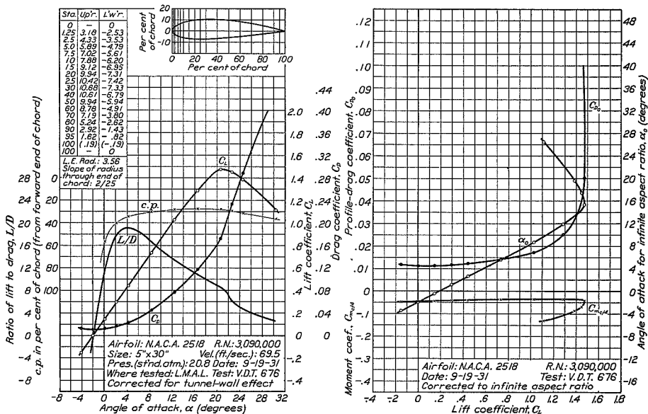
FIGURE 26.—N.A.C.A. 2518 airfoil.
