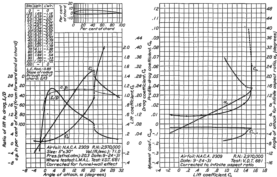
FIGURE 13.—N.A.C.A. 2309 airfoil.
