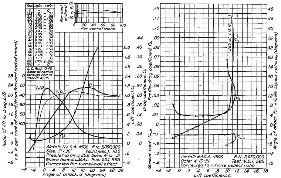
FIGURE 43.—N.A.C.A. 4506 airfoil.
