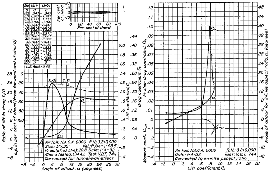
FIGURE 4.—N.A.C.A. 0006 airfoil.
