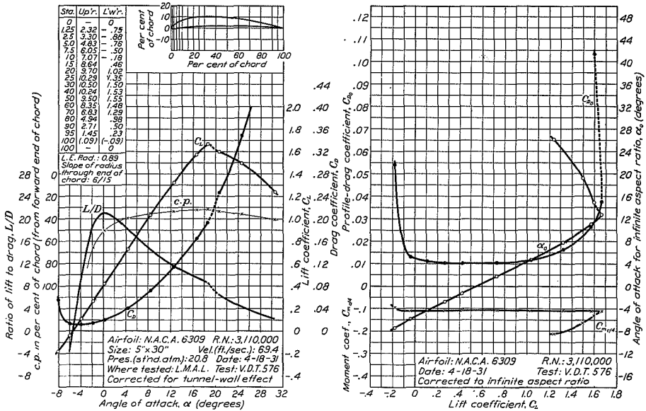
FIGURE 63.—N.A.C.A. 6309 airfoil.
