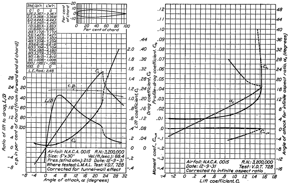
FIGURE 7.—N.A.C.A. 0015 airfoil.
