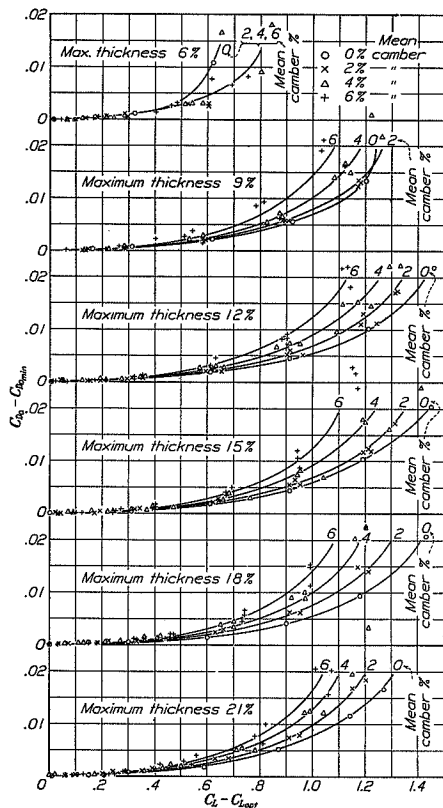
FIGURE 94.—Additional profile drag as a function of C_l - C_{l_{cpt}} . Results are for airfoils having normal camber positions (0.3c to 0.5c).
