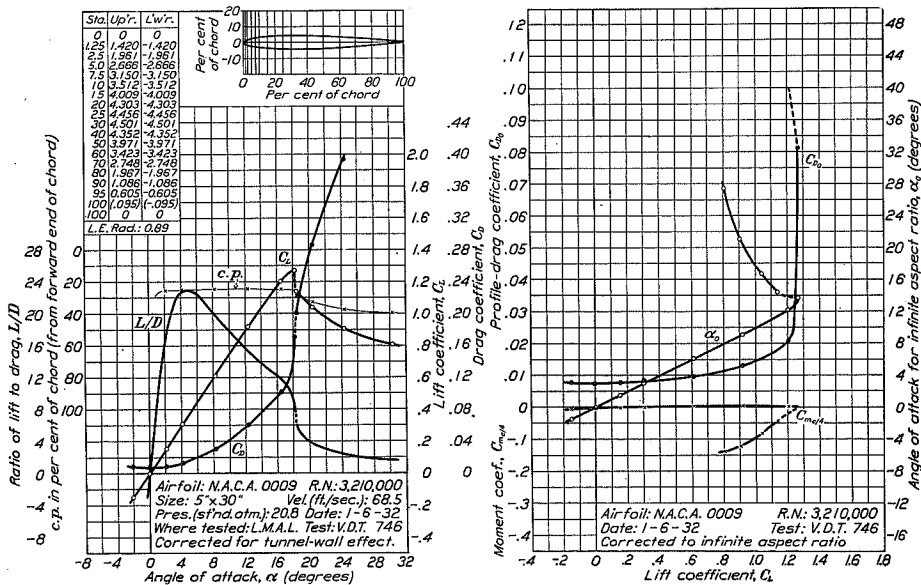
FIGURE 5.—N.A.C.A. 0009 airfoil.
