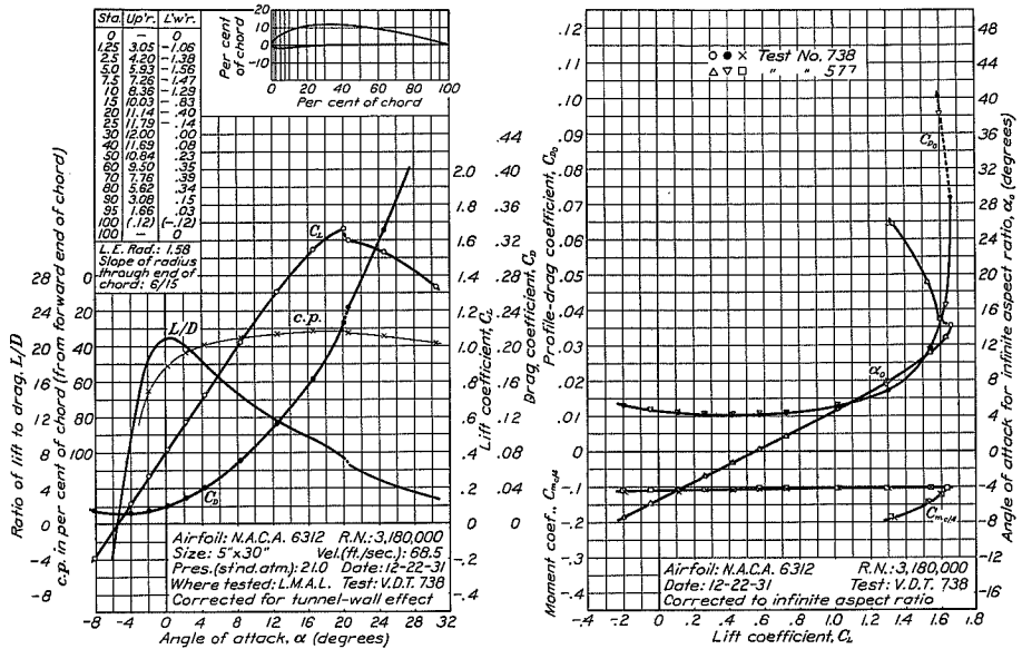
FIGURE 64.—N.A.C.A. 6312 airfoil.
