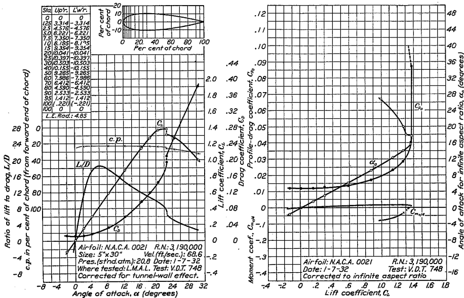
FIGURE 9.—N.A.C.A. 0021 airfoil.
