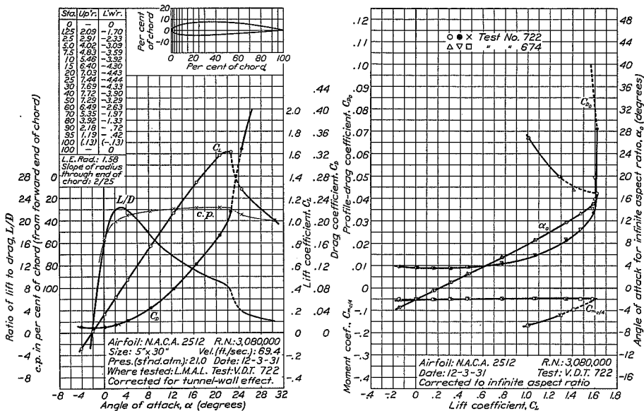
FIGURE 24.—N.A.C.A. 2512 airfoil.
