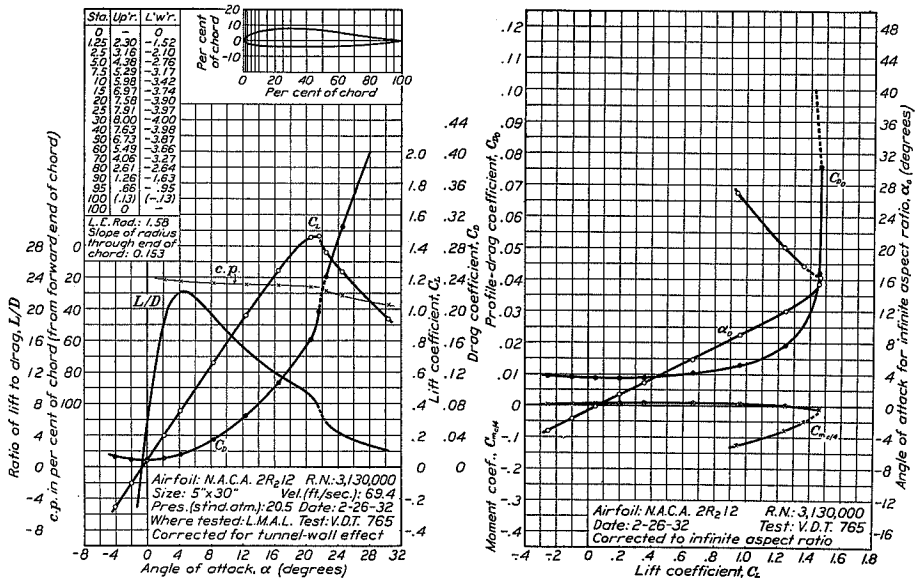
FIGURE 79.—N.A.C.A. 2R212 airfoil.
