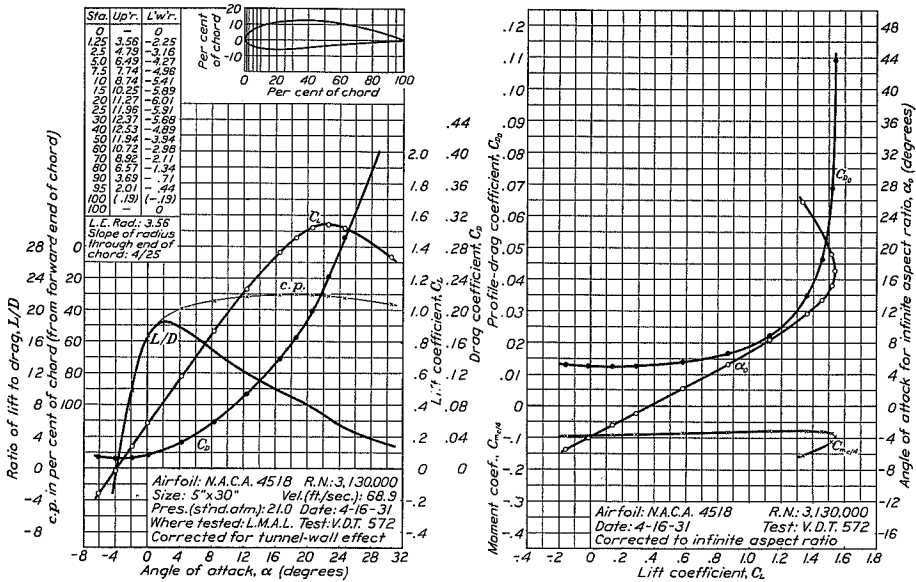
FIGURE 47.—N.A.C.A. 4518 airfoil.
