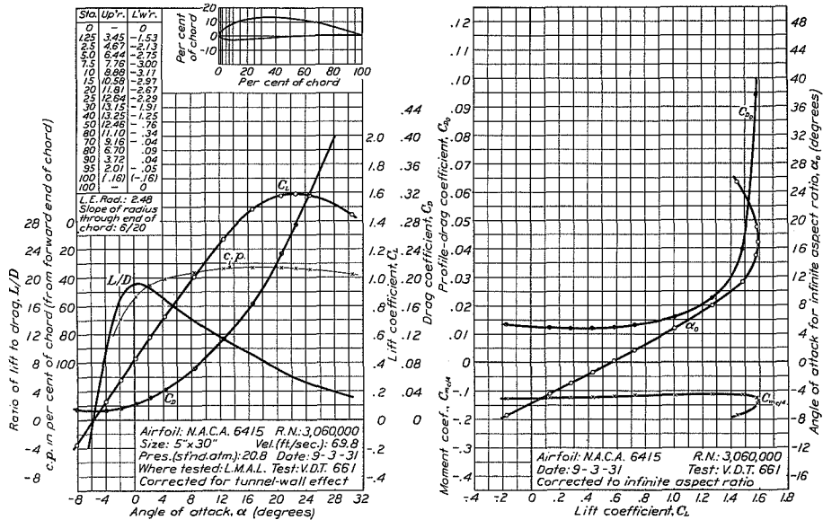
FIGURE 61.—N.A.C.A. 6415 airfoil.
