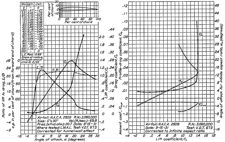
FIGURE 23.—N.A.C.A. 2509 airfoil.
