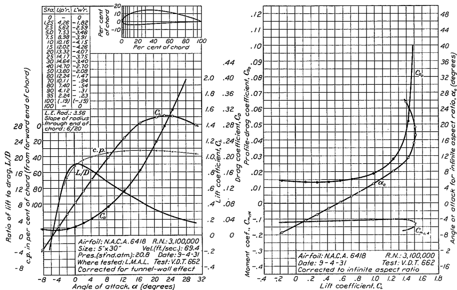
FIGURE 62.—N.A.C.A. 6418 airfoil.
