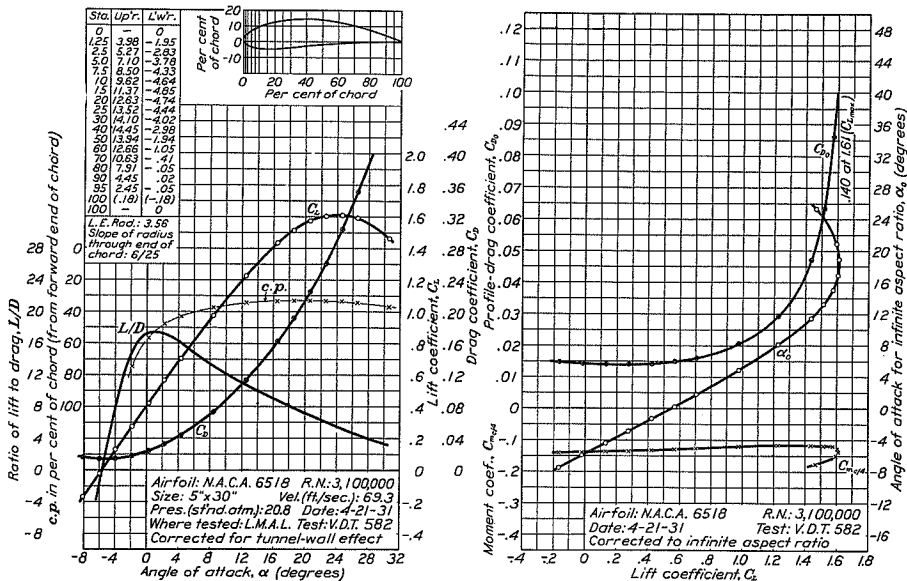
FIGURE 68.—N.A.C.A. 6518 airfoil.
