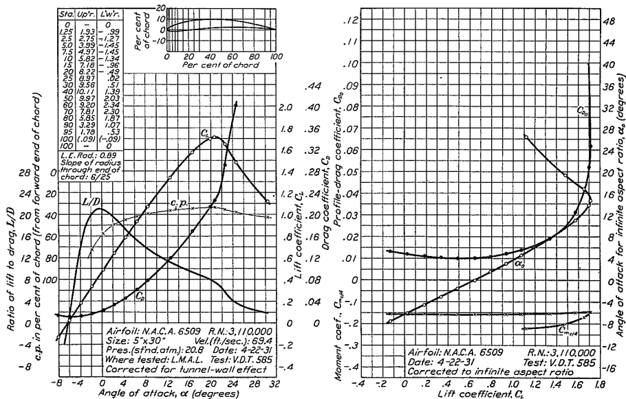
FIGURE 65.—N.A.C.A. 6509 airfoil.
