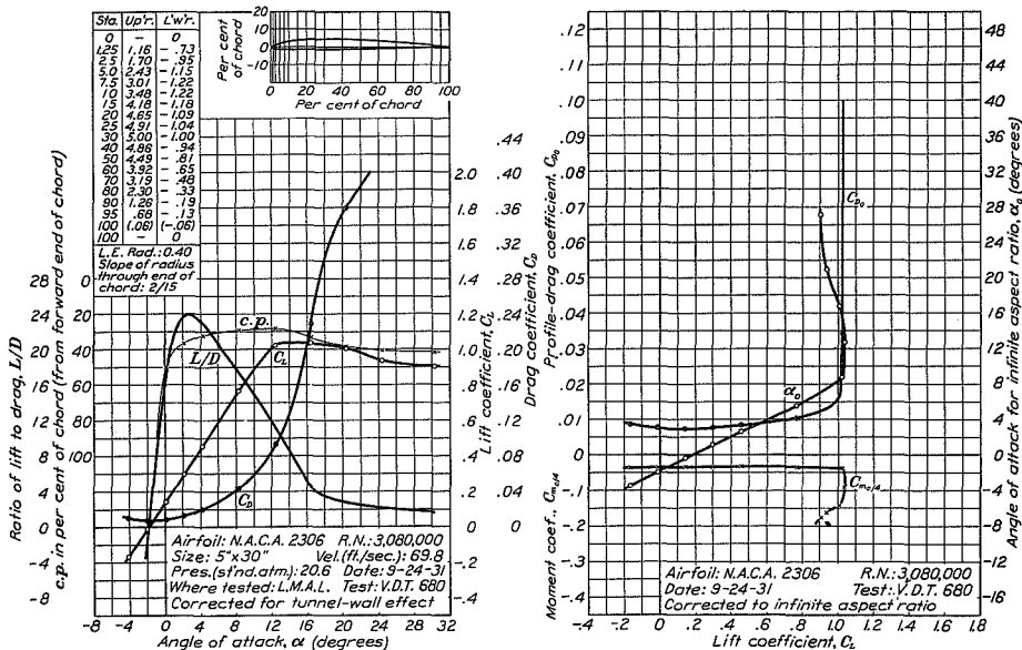
FIGURE 12.—N.A.C.A. 2306 airfoil.
