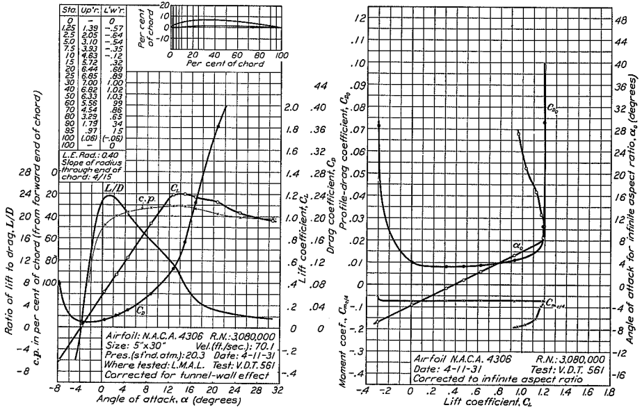
FIGURE 31.—N.A.C.A. 4306 airfoil.
