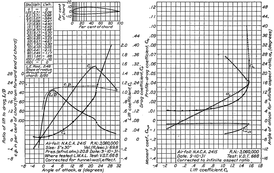
FIGURE 19.—N.A.C.A. 2415 airfoil.
