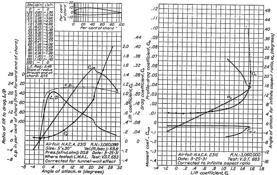
FIGURE 15.—N.A.C.A. 2315 airfoil.
