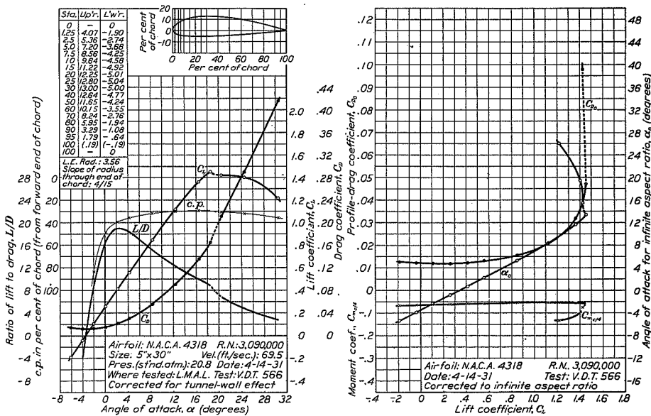
FIGURE 35.—N.A.C.A. 4318 airfoil.
