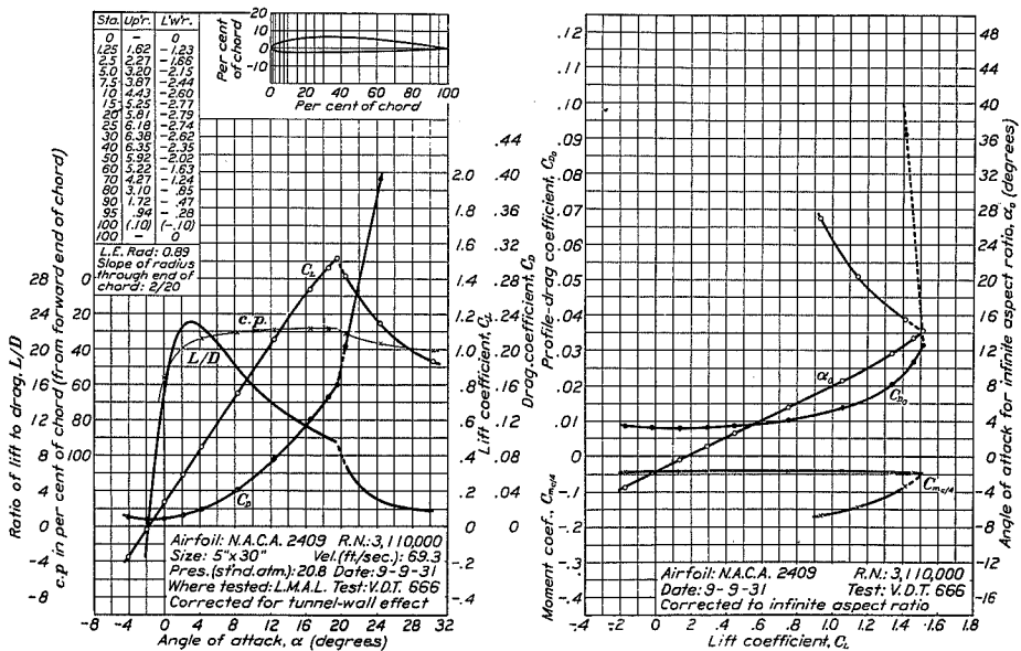
FIGURE 17.—N.A.C.A. 2409 airfoil.
