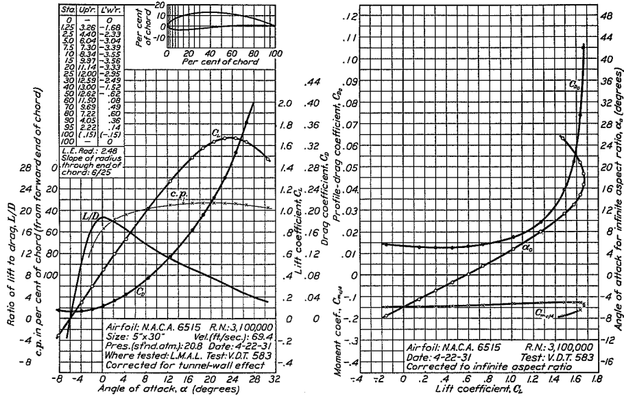
FIGURE 67.—N.A.C.A. 6515 airfoil.
