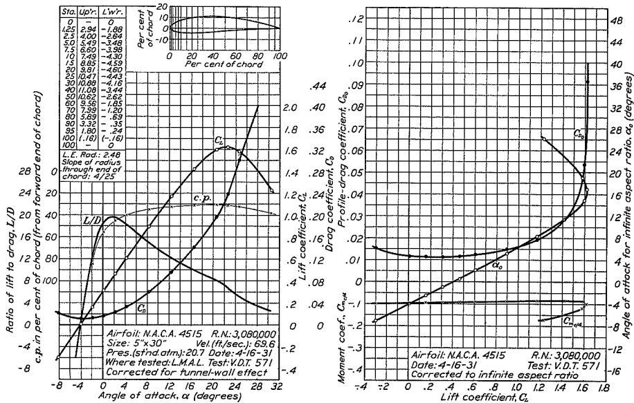
FIGURE 46.—N.A.C.A. 4515 airfoil.
