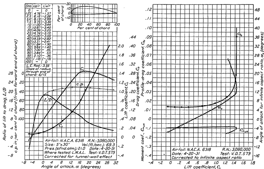
FIGURE 56.—N.A.C.A. 6318 airfoil.
