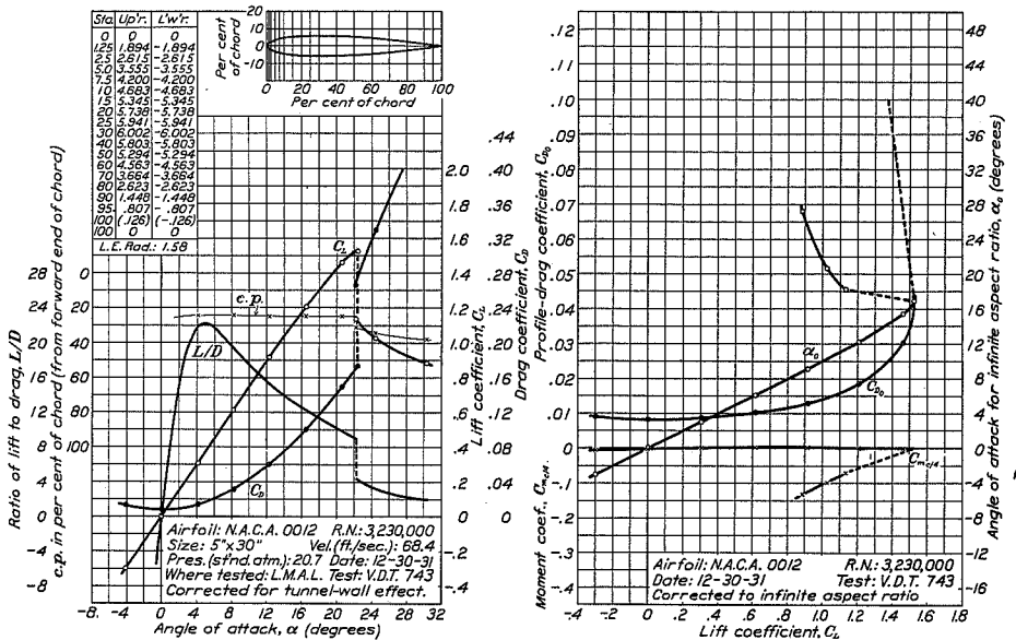
FIGURE 6.—N.A.C.A. 0012 airfoil.
