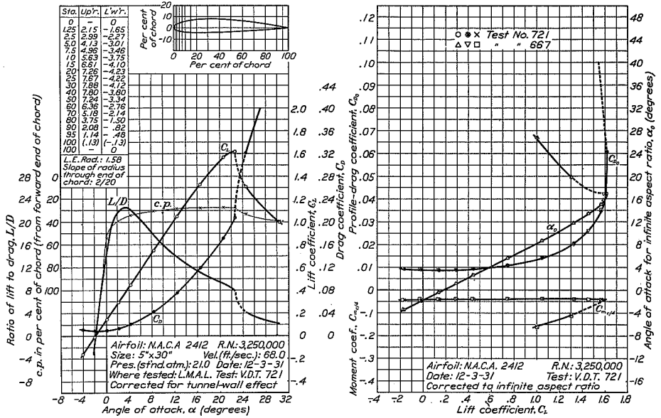
FIGURE 18.—N.A.C.A. 2412 airfoil.
