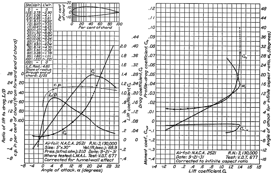
FIGURE 27.—N.A.C.A. 2521 airfoil.
