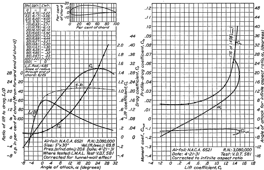
FIGURE 66.—N.A.C.A. 6521 airfoil.
