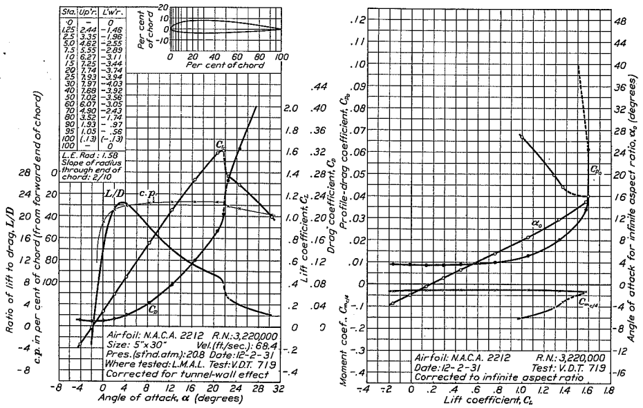
FIGURE 11.—N.A.C.A. 2212 airfoil.
