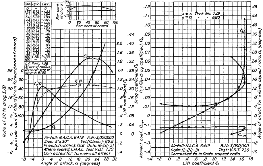
FIGURE 60.—N.A.C.A. 6412 airfoil.
