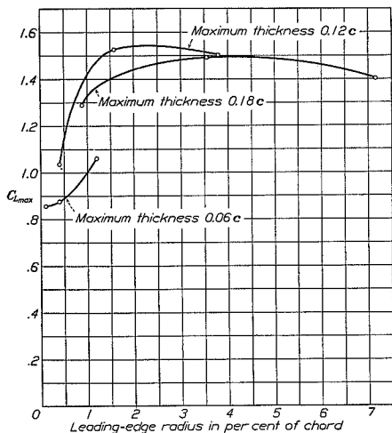
FIGURE 97.—Variation of maximum lift with nose radius.
