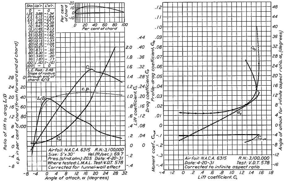
FIGURE 65.—N.A.C.A. 6315 airfoil.
