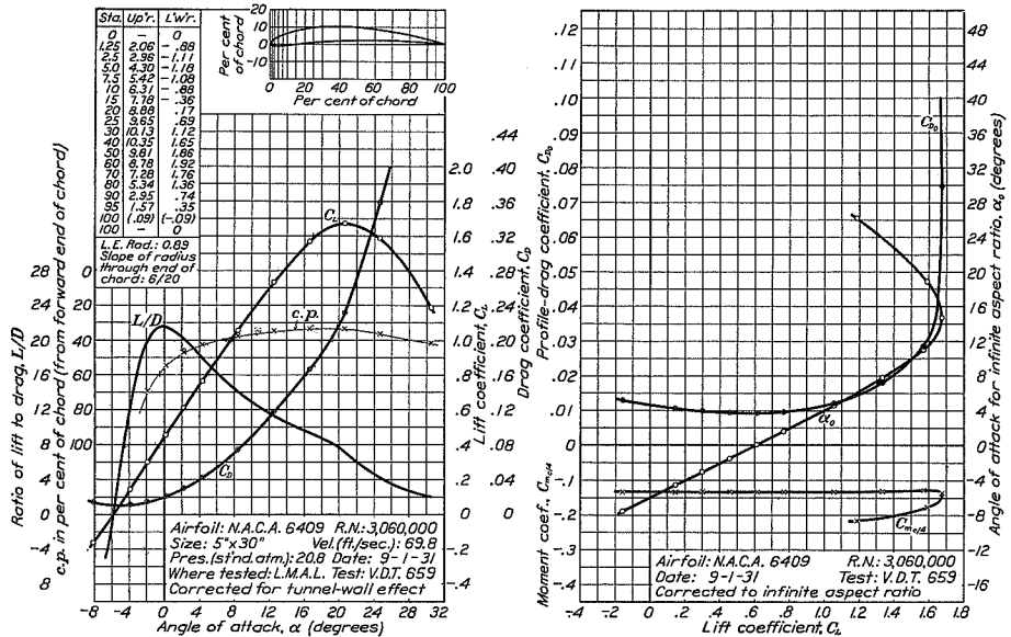
FIGURE 59.—N.A.C.A. 6409 airfoil.
