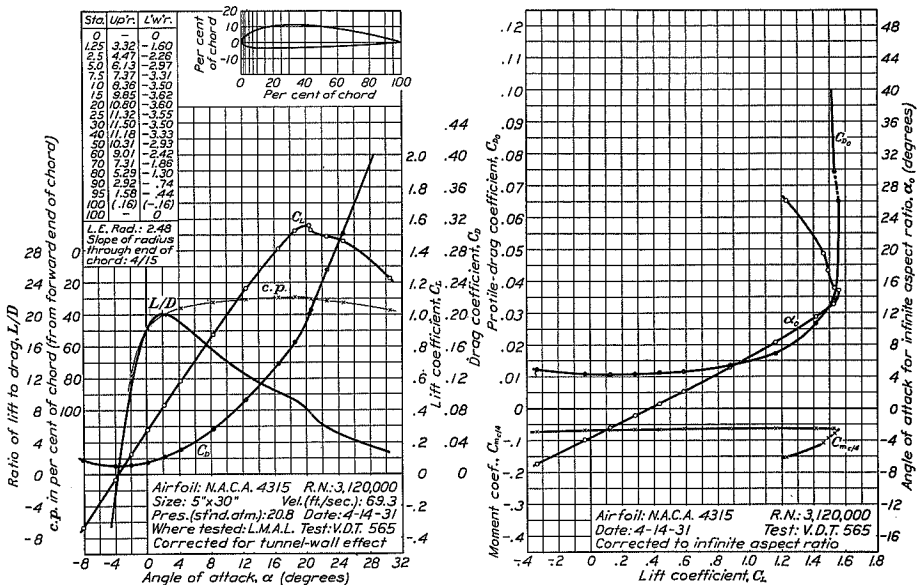
FIGURE 34.—N.A.C.A. 4315 airfoil.
