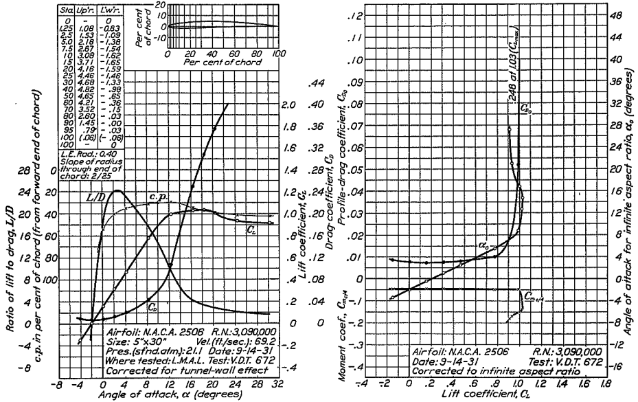
FIGURE 22.—N.A.C.A. 2506 airfoil.
