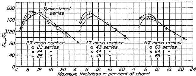
FIGURE 96.—Variation of C_{l_{max}}/C_{d_{pmin}} with thickness.
