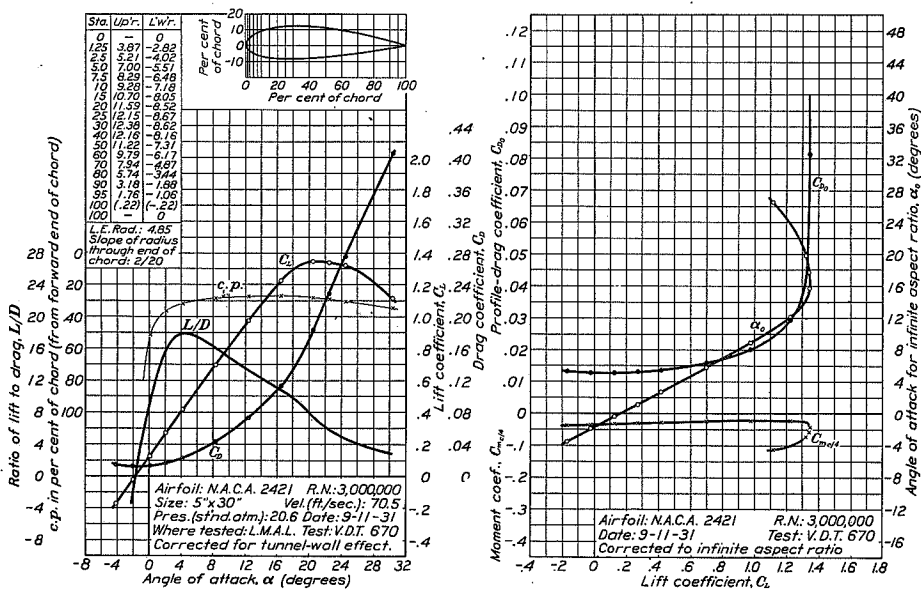
FIGURE 21.—N.A.C.A. 2421 airfoil.
