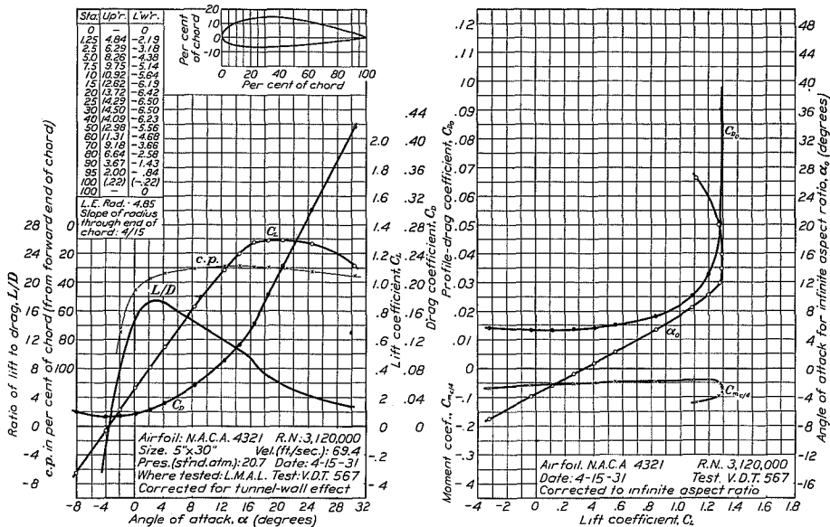
FIGURE 36.—N.A.C.A. 4321 airfoil.
