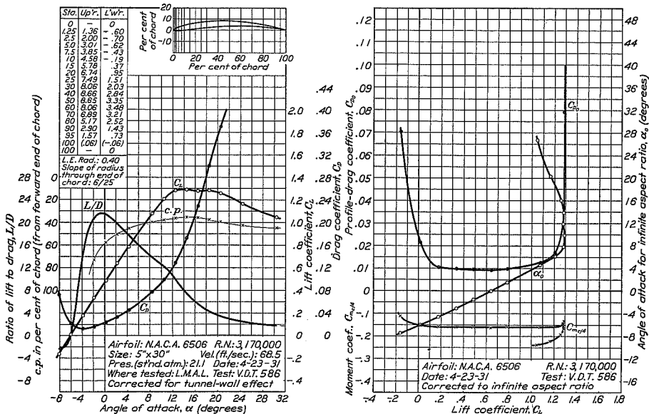
FIGURE 64.—N.A.C.A. 6506 airfoil.
