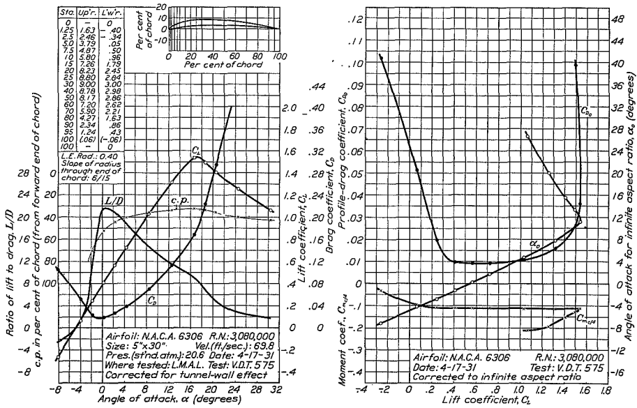
FIGURE 62.—N.A.C.A. 6306 airfoil.
