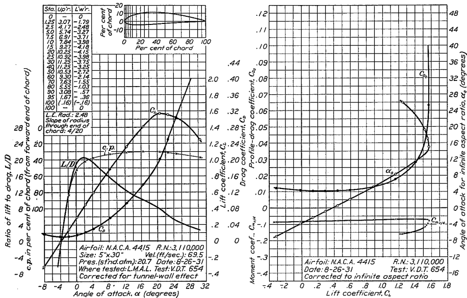
FIGURE 40.—N.A.C.A. 4415 airfoil.
