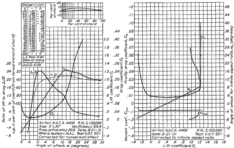
FIGURE 37.—N.A.C.A. 4406 airfoil.
