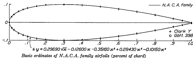
FIGURE 1.—Thickness variation.
