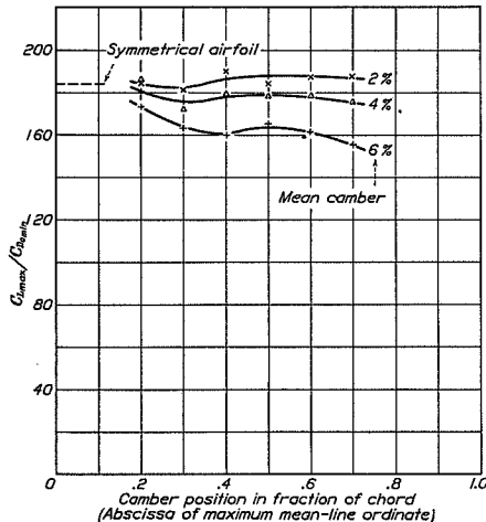
FIGURE 95.—Variation of C_{l_{max}}/C_{d_{pmin}} with camber. Results are for 12 percent thick airfoils.
