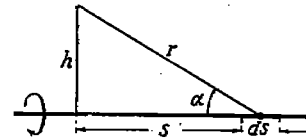
FIG. 4.—Velocity-field due to infinite rectilinear vortex.
