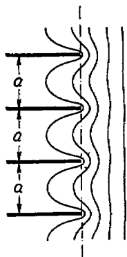
FIG. 60.—Conformal transformation
