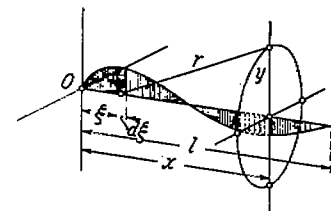
FIG. 8.—Explanation of quantities used in calculation of streamline shapes. Abscissae: Position of source. Ordinates: Intensity of source per unit length, i. e. f(\xi) .
