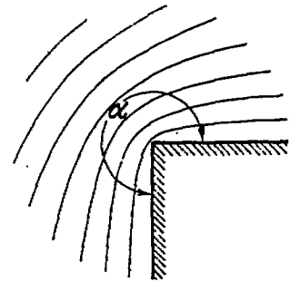
FIG. 7.—Uniplanar flow around plane walls making an angle 270^\circ with each other.
