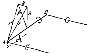
FIG. 41.—Curvature of wing-profile at its middle point due to velocities caused by transverse and tip vortices.
