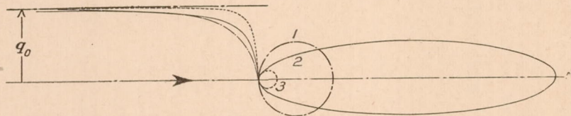
FIG. 19.—Superposed graphs of axial flow speed before three endless cylinders 1, 2, and 3 (3 osculating 2), each fixed transverse to an infinite stream of inviscid liquid. At great distance flow speed is q_0 .
