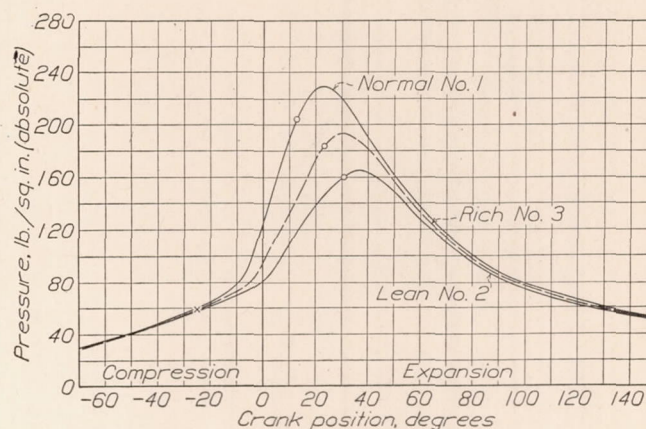
FIGURE 19.—Effect of mixture ratio
