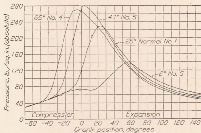
FIGURE 20.—Effect of spark advance
