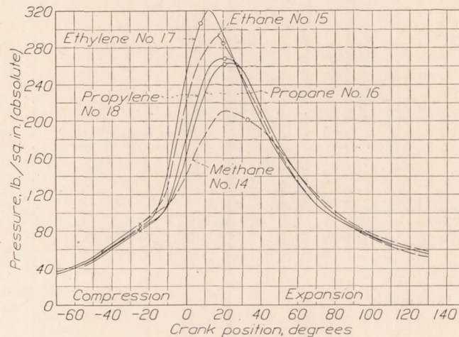
FIGURE 26.—Effect of fuel
