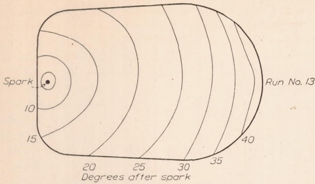
FIGURE 6.—Flame diagram. Normal run. Compression ratio 5 to 1
