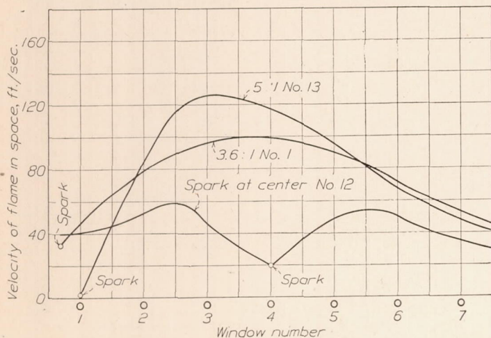
FIGURE 17.—Velocity-displacement diagrams
