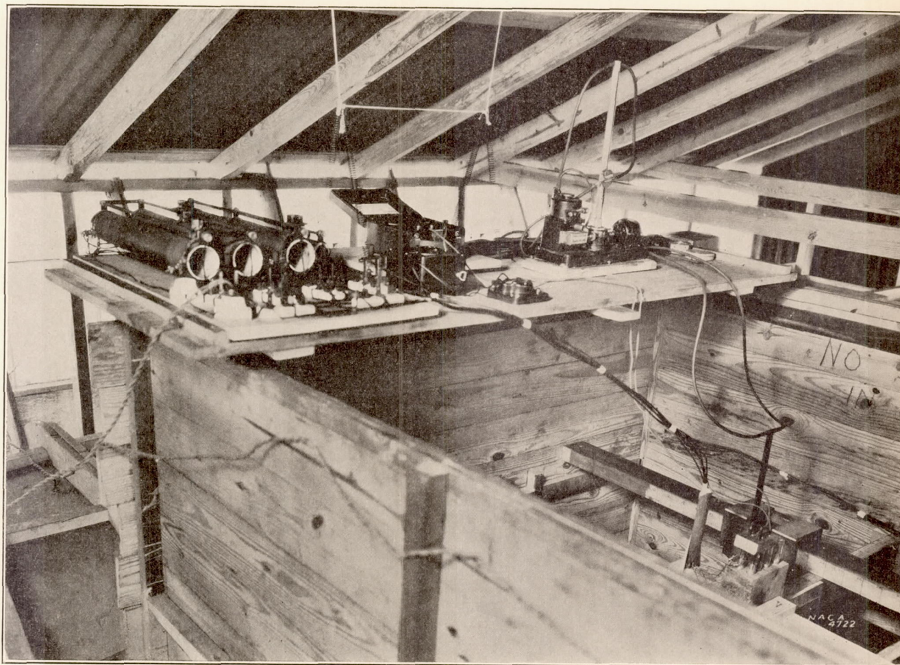
FIGURE 4.—Control group of wind tunnel set-up
