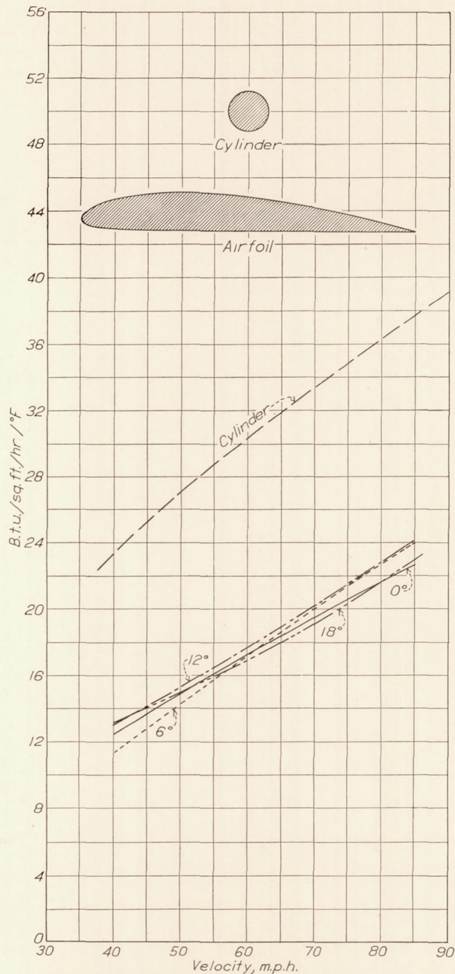
FIGURE 14.—Rate of heat transmission from the entire airfoil and the cylinder
