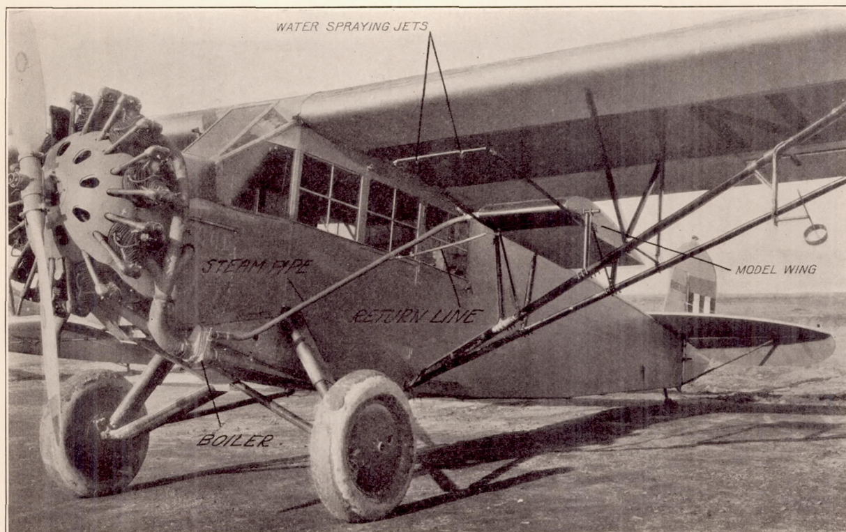
FIGURE 24.—Experimental installation on airplane
