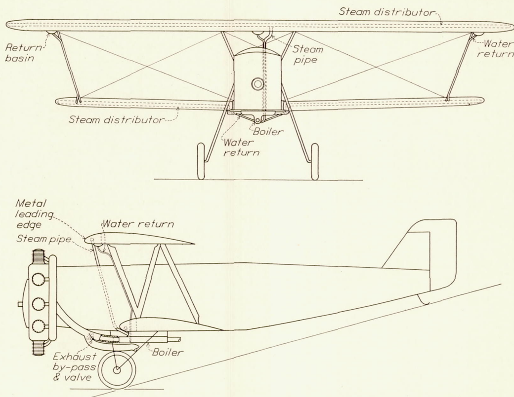
FIGURE 26.—Diagram of suggested layout for biplane installation
