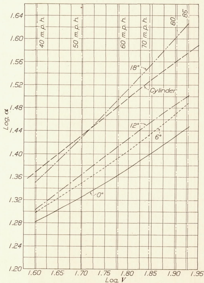
FIGURE 16.—Log \alpha versus log velocity V for section 1 and the cylinder, where \alpha =B. t. u./sq. ft./hr./° F. and V =m. p. h.
