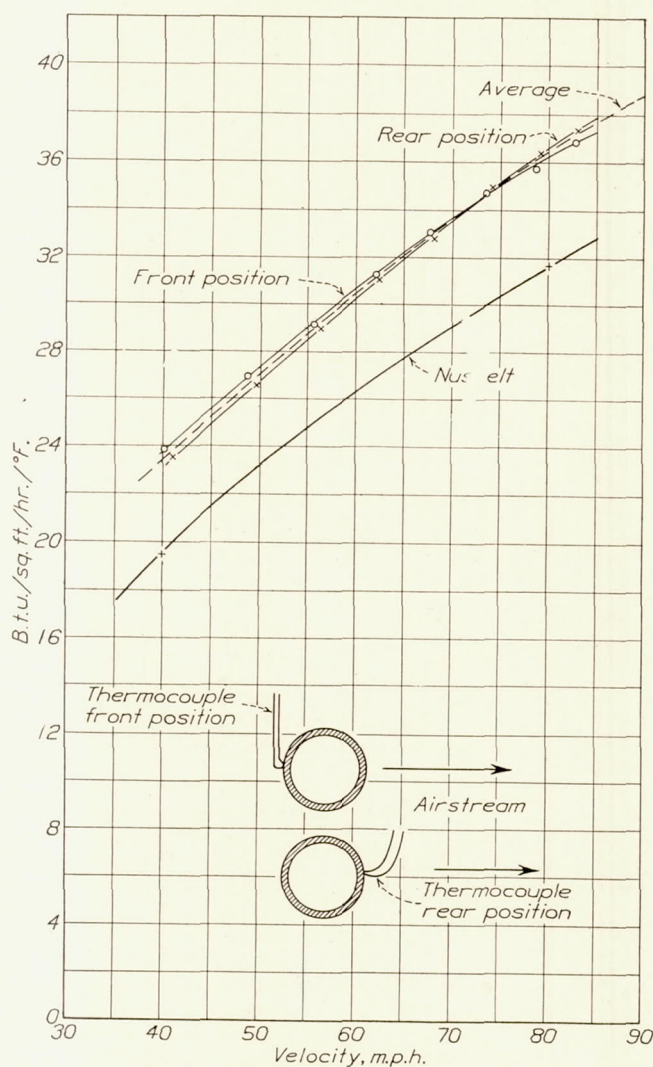
FIGURE 9.—Rate of heat transmission for cylinder ( 1\frac{3}{8} in. O. D.). Lower curve shows values calculated from formula by Nusselt
