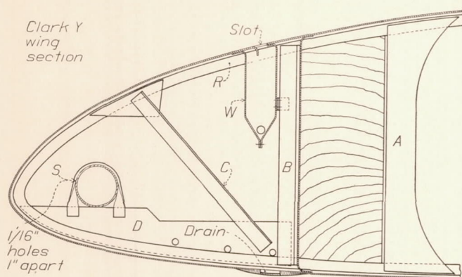
FIGURE 27.—Diagrammatic design of vapor-heated leading edge
