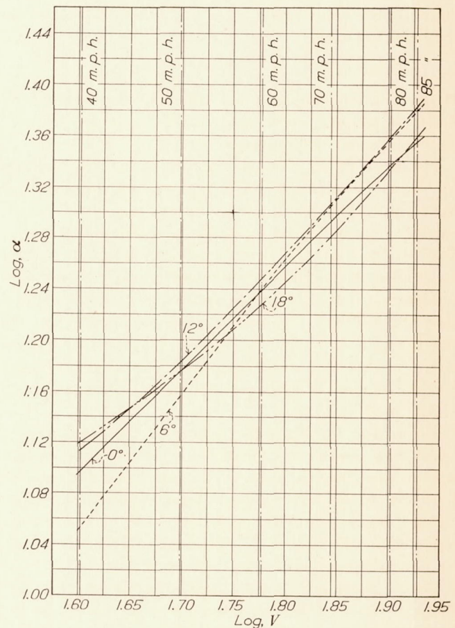
FIGURE 17.—Log \alpha versus log velocity V for the entire airfoil, where \alpha =B. t. u./sq. ft./hr./° F. V =m. p. h.
