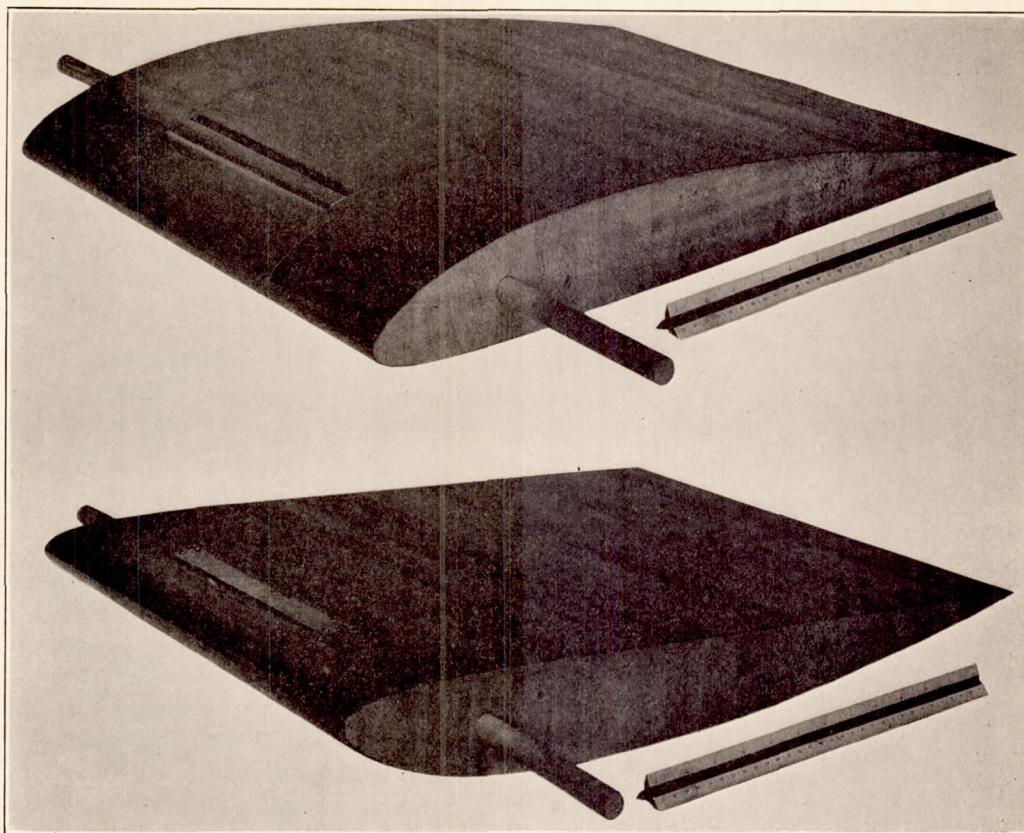
FIGURE 18.—Model for experiments on rain-catch slots
