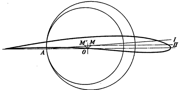
FIGURE 24.—The Joukowski airfoil \rho=0.10 , \delta=45^\circ
