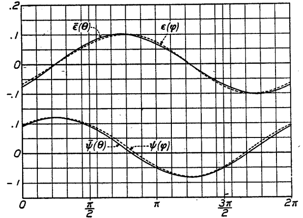
FIGURE 25.—The \epsilon(\theta) and \psi(\theta) curves for the airfoil in Figure 24
