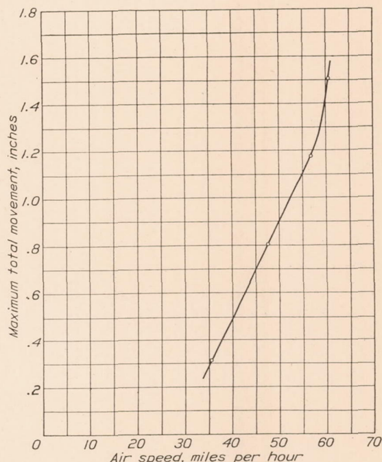
FIGURE 28.—Variation in stabilizer-tip movements with changes in air speed. Power off. McDonnell airplane in original condition. Angle of attack (corrected for tunnel effect), 3.7^\circ below \alpha_{C_{L_{max}}} .
