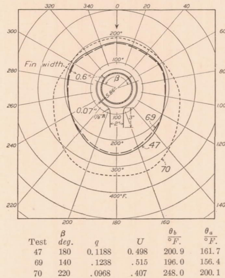
FIGURE 15.—Effect of the entrance angle of a shell baffle on the temperature distribution and heat-transfer coefficients. Cylinder 3.
